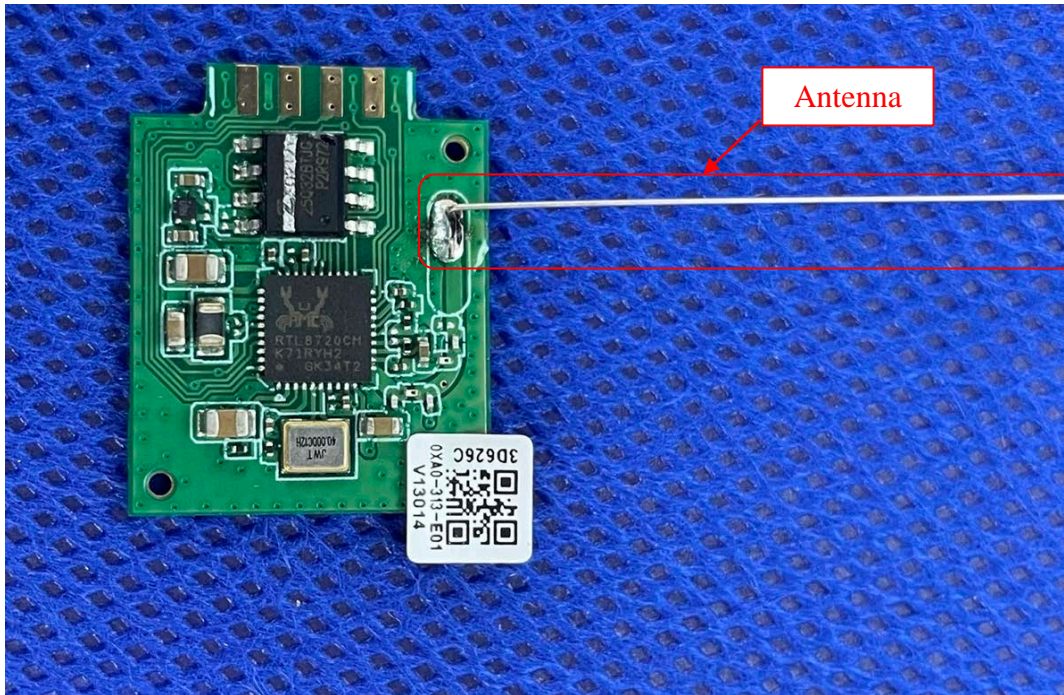
FIGURE 6 LED LAMP (M/N: CLEDA2116CD) CHIP&CRYSTAL ON RFBORAD
