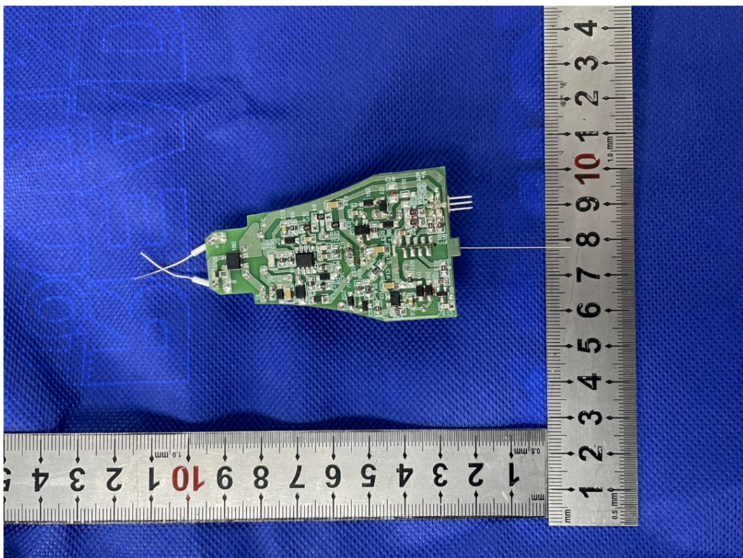
FIGURE 2 LED LAMP (M/N: CLEDA2116CD) MAIN BOARD FRONT
