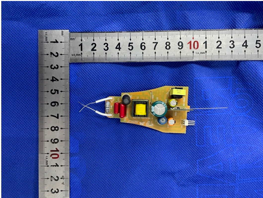
FIGURE 4 LED LAMP (M/N: CLEDA2116CD) RF BORAD FRONT
