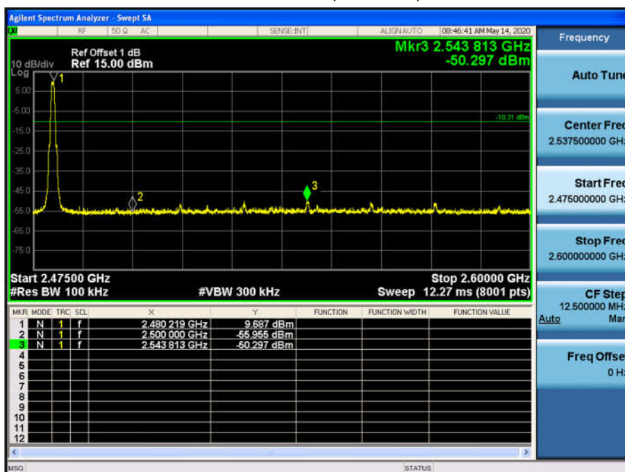
Mode 2 CH39(2480MHz)
