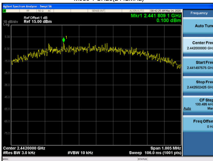
Mode 1 CH20(2442MHz)
