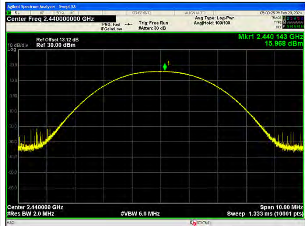
Peak Power NVNT 512K 2440MHz Ant1
