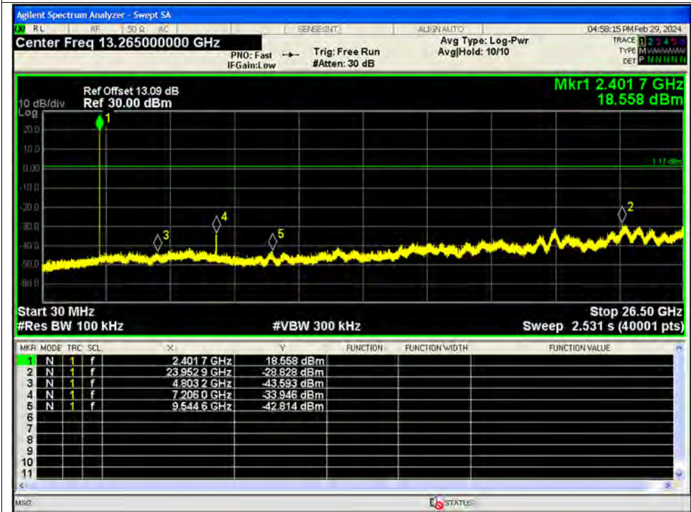
Tx. Spurious NVNT 512K 2402MHz Ant1 Emission
