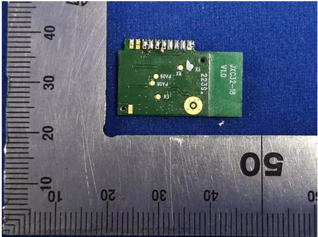
FIGURE 9 DIRECT CONNECT FULL COLOR A19 (M/N: CLEDA199CD1) RBOARD BACK
