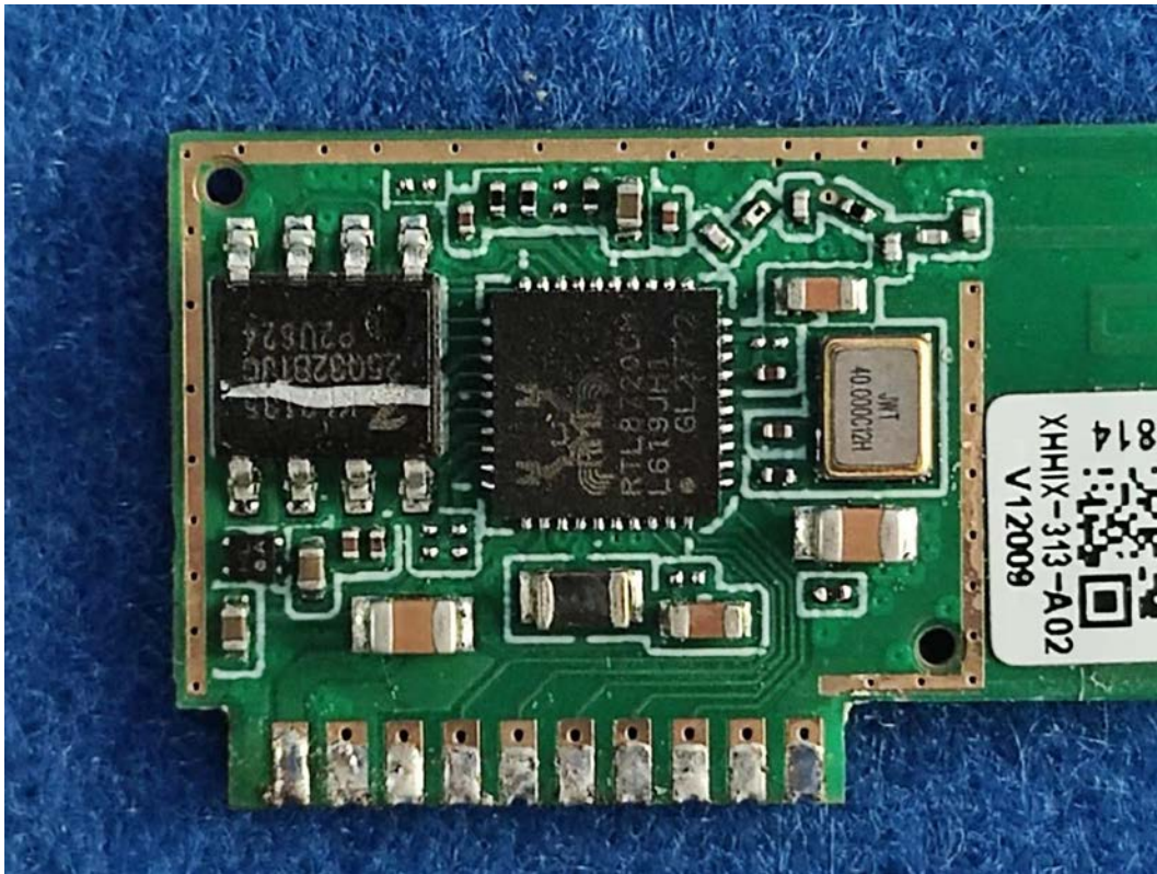
FIGURE 7 DIRECT CONNECT FULL COLOR A19 (M/N: CLEDA199CD1) (HVIN: CLEDA199CD1D) CHIP&CRYSTAL ON RBOARD
