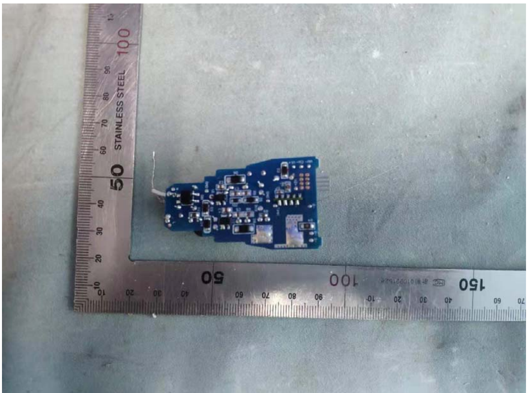
FIGURE 5 DIRECT CONNECT FULL COLOR A19 (M/N: CLEDA199CD1) MAIN BOARD (SOLDERED SIDE)
