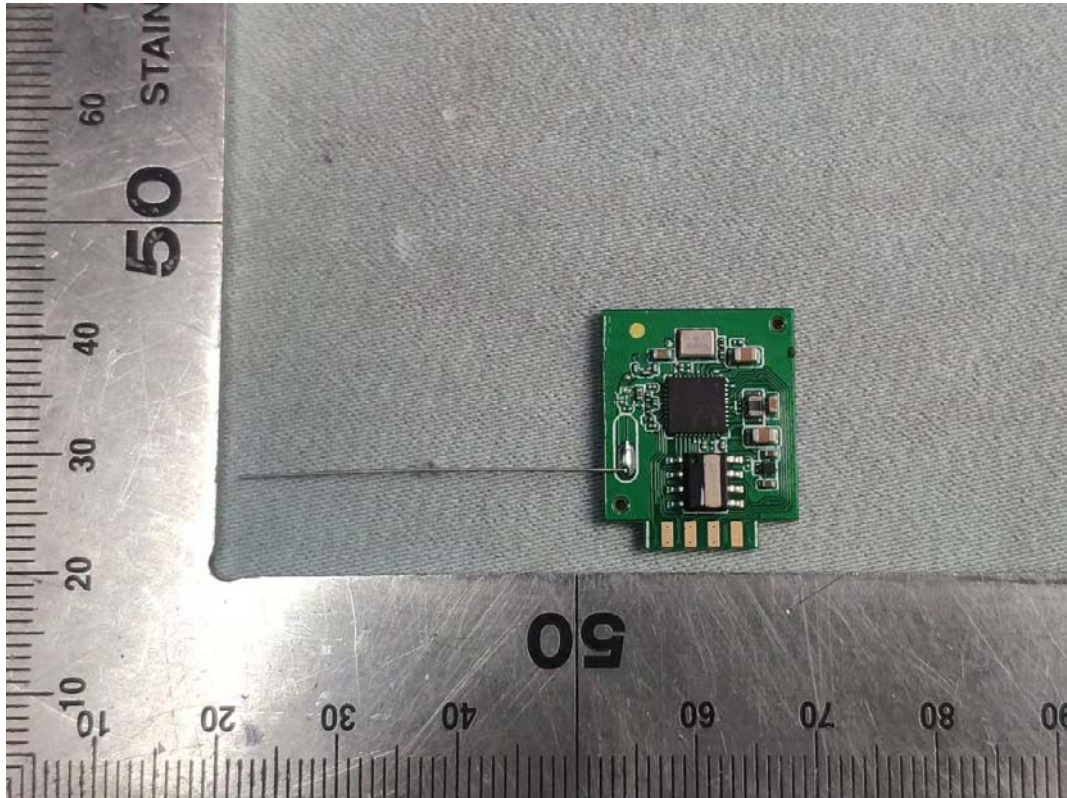
FIGURE 7 DIRECT CONNECT FULL COLOR A19 (M/N: CLEDA199CD1) RF BOARD (BACK SIDE)
