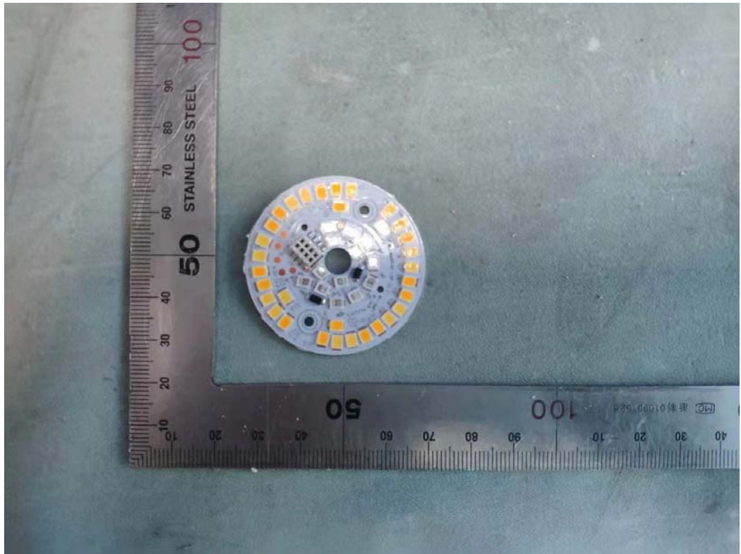
FIGURE 2 DIRECT CONNECT FULL COLOR A19 (M/N: CLEDA199CD1) LED (FRONT)
