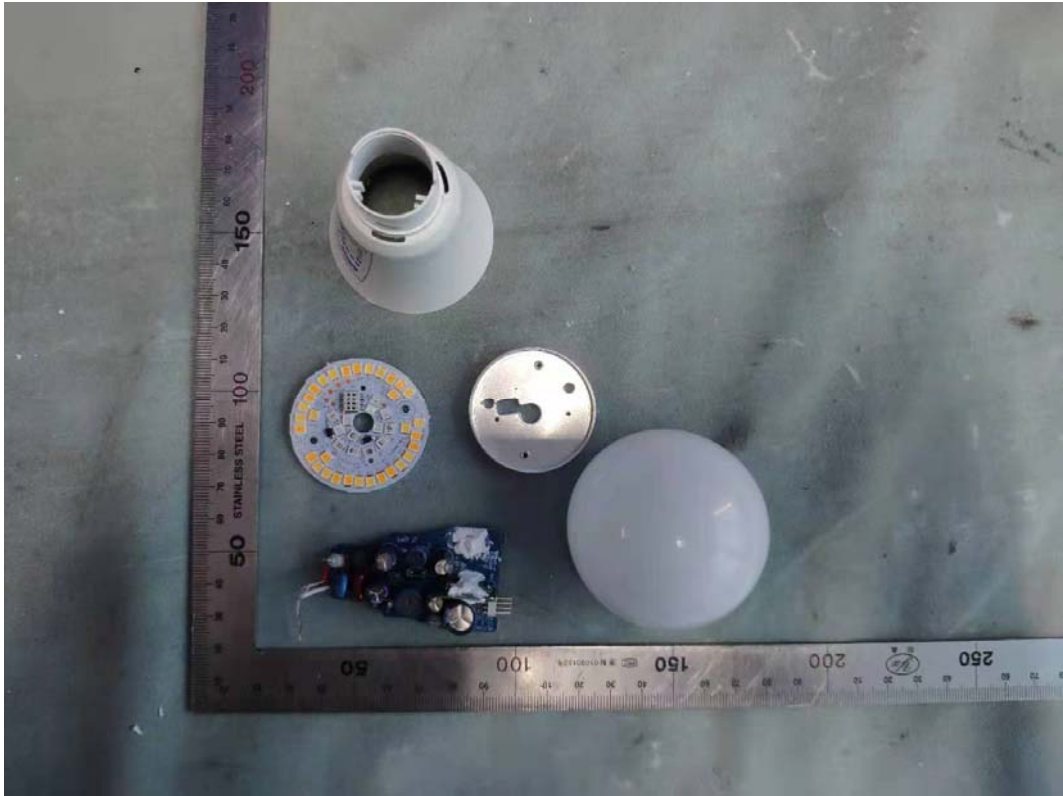
FIGURE 1 DIRECT CONNECT FULL COLOR A19 (M/N: CLEDA199CD1) GENERAL APPEARANCE (COVER REMOVED)
