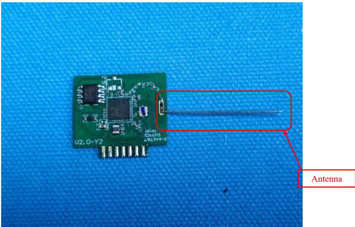
FIGURE 8 DUAL MODE FULL COLOR A19 (M/N: CLEDA199CD1) RF BOARD (COMPONENT SIDE)
