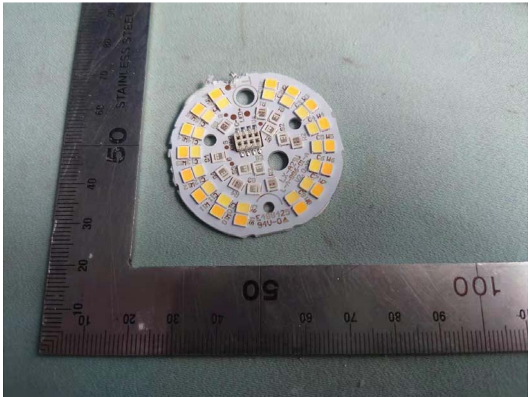
FIGURE 3 DUAL MODE FULL COLOR A19 (M/N: CLEDA199CD1) LED (FRONT)
