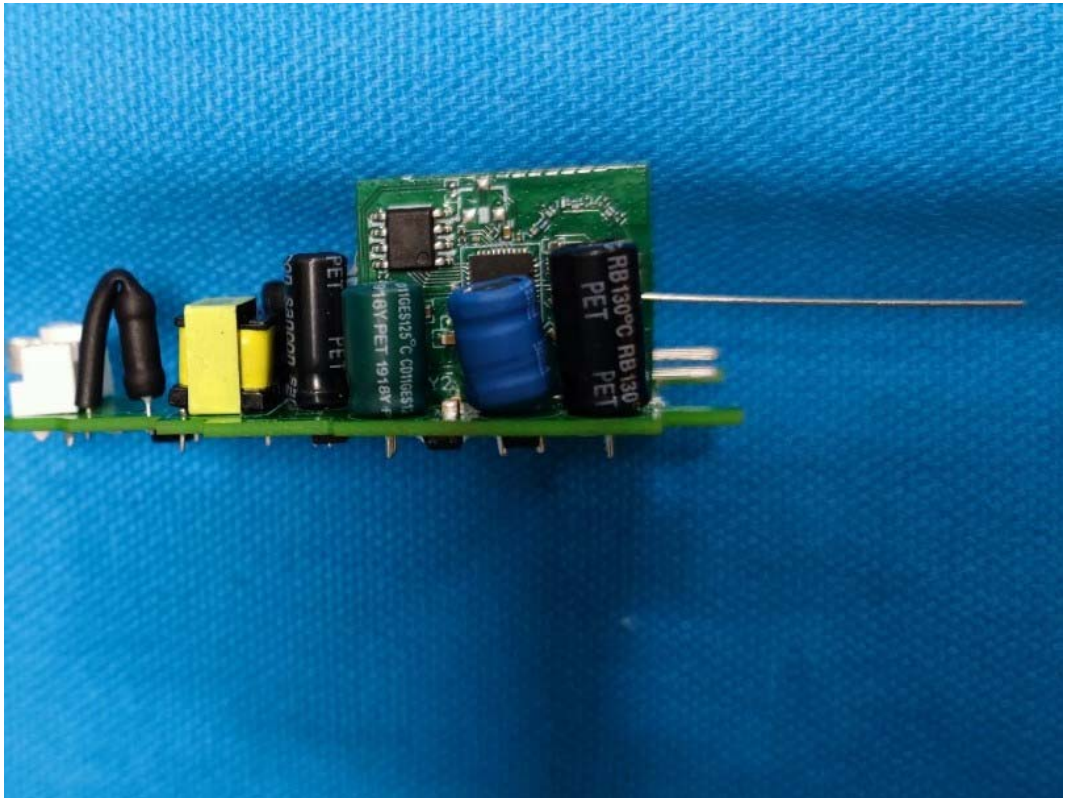
FIGURE 8 DUAL MODE FULL COLOR A19 (M/N: CLEDA199CD1) RF BOARD (COMPONENT SIDE)
