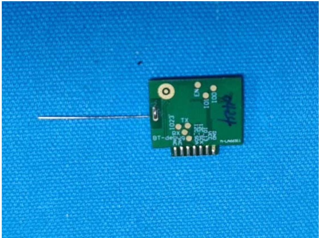
FIGURE 9 DUAL MODE FULL COLOR A19 (M/N: CLEDA199CD1) RF BOARD (SOLDERED SIDE)
