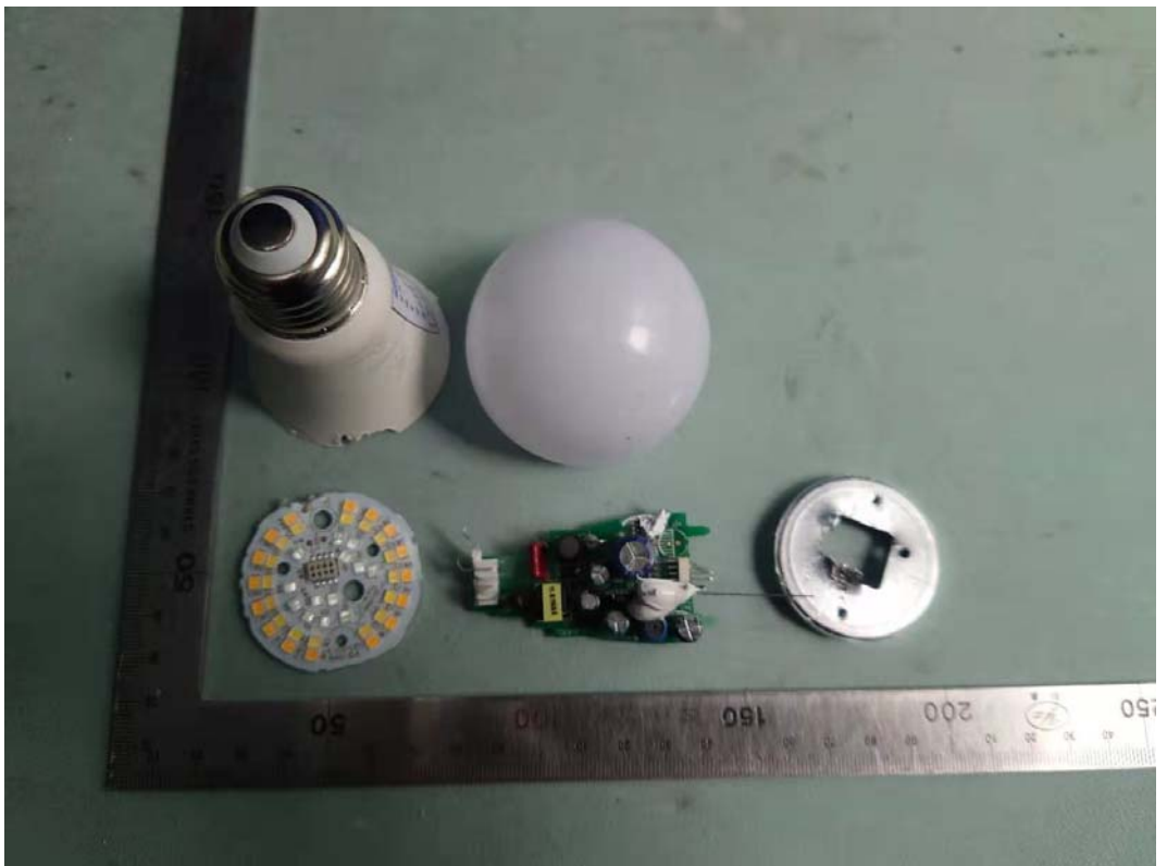
FIGURE 2 DUAL MODE FULL COLOR A19 (M/N: CLEDA199CD1) GENERAL APPEARANCE (COVER REMOVED)
