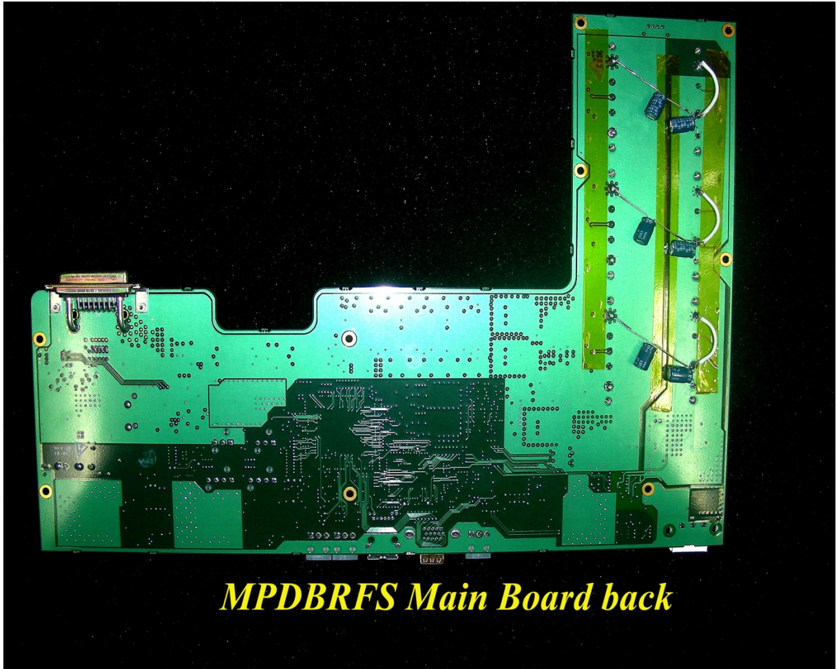
PCB Back
