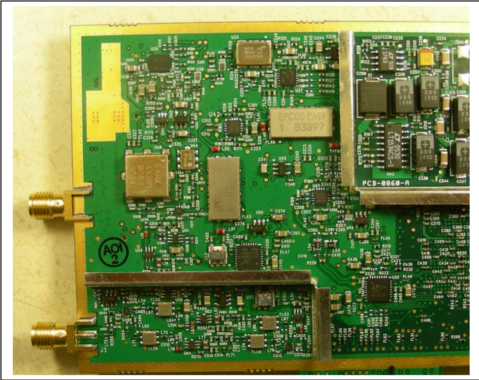
MCRB PCB Front
