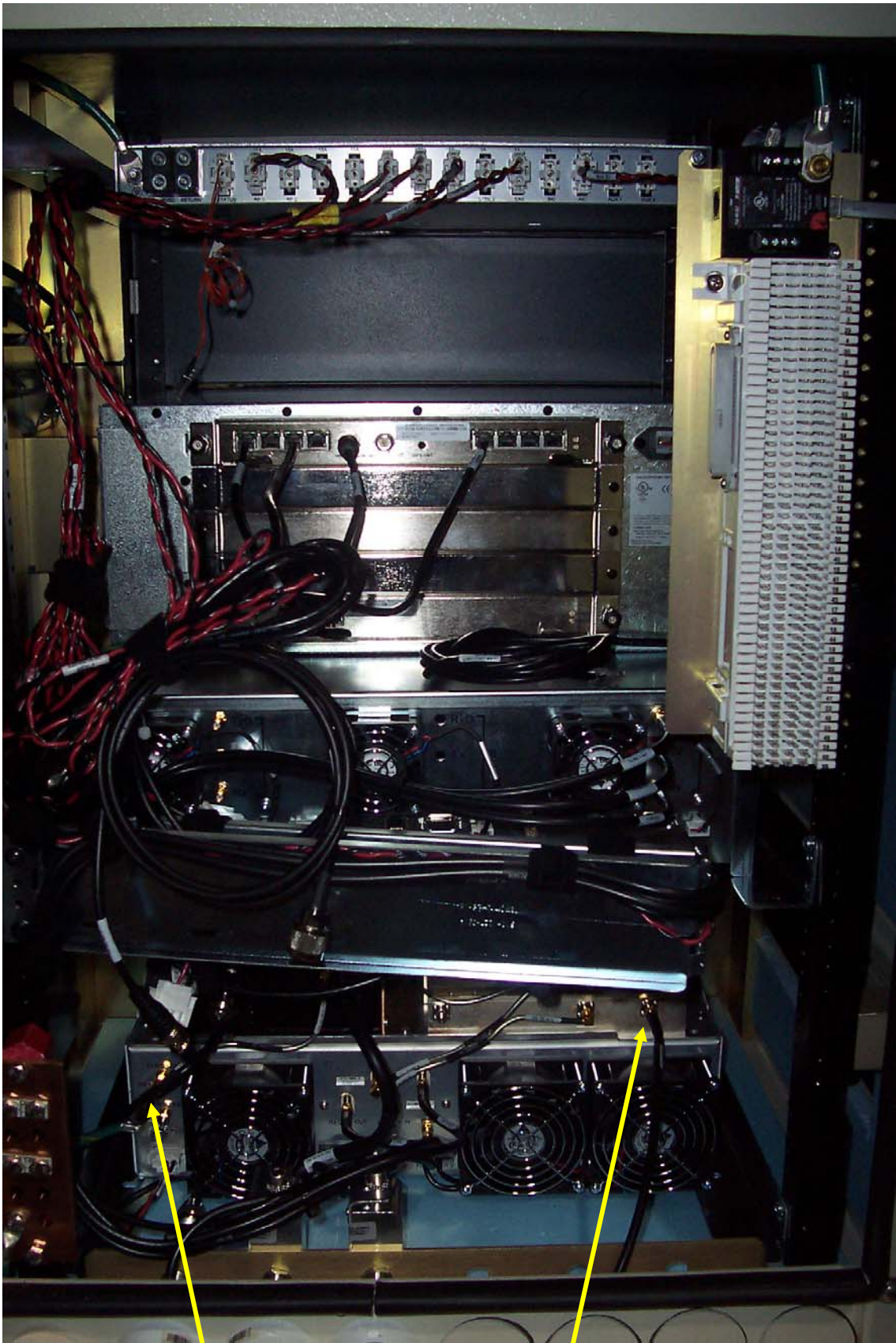
Transmit signal in from Radio in RBS 800 MHz Transmit signal out to Antenna
