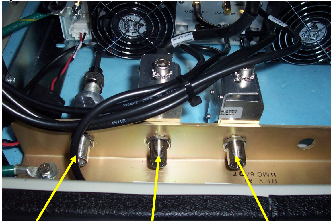
Transmit antenna port Receive Antenna Port Receive Div. Antenna Port
