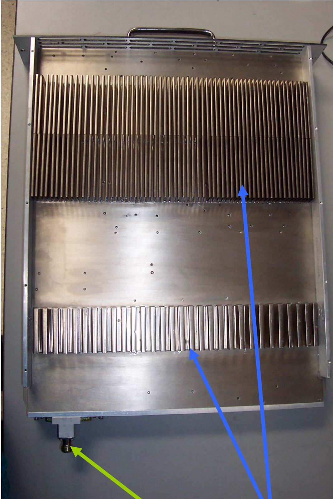
PA Top Vertical View
