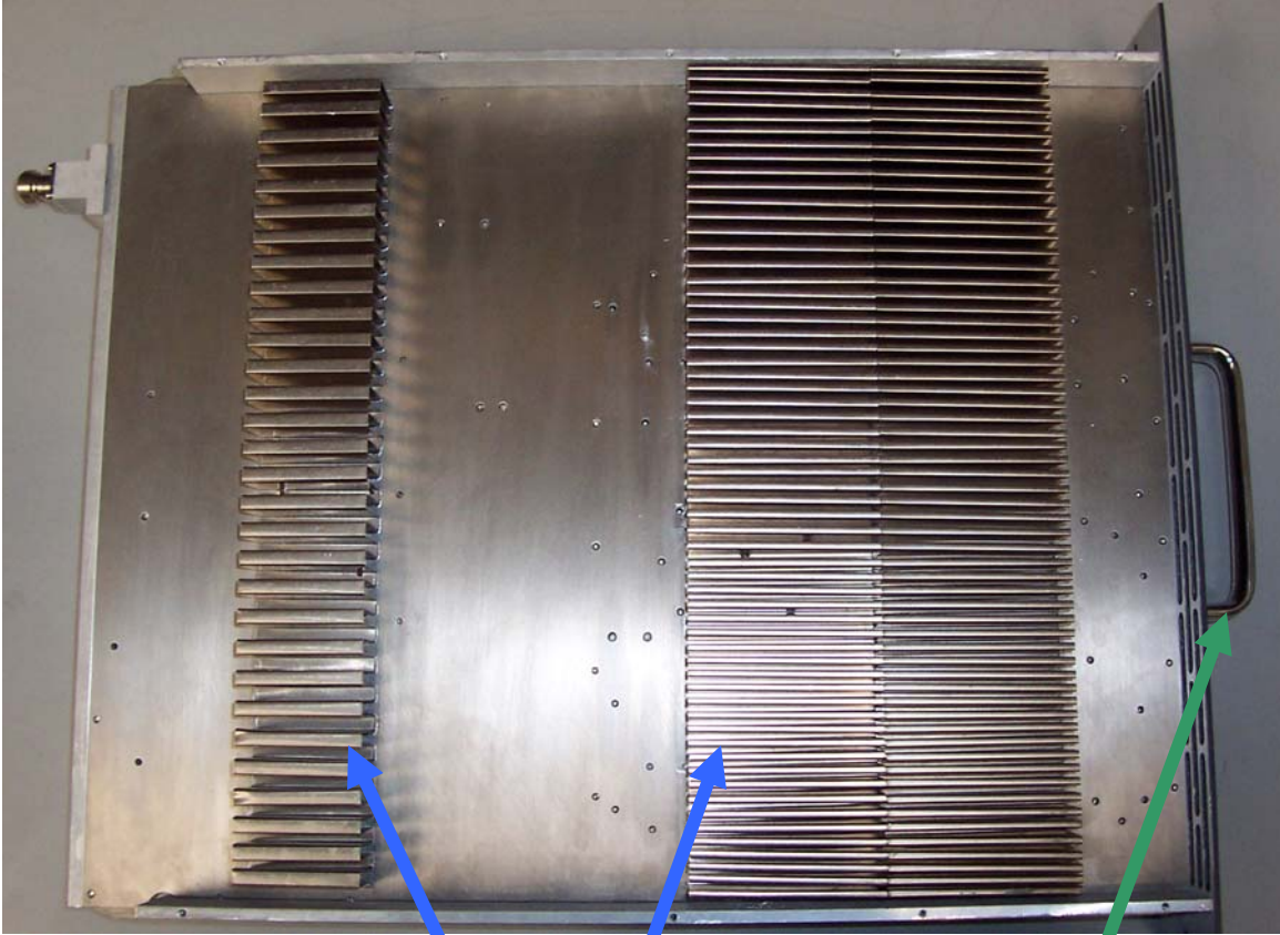
PA Top Horizontal View
