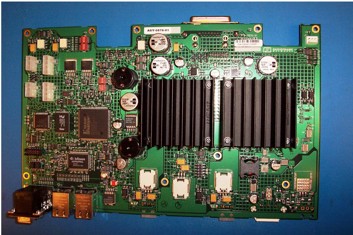
PCB Front
