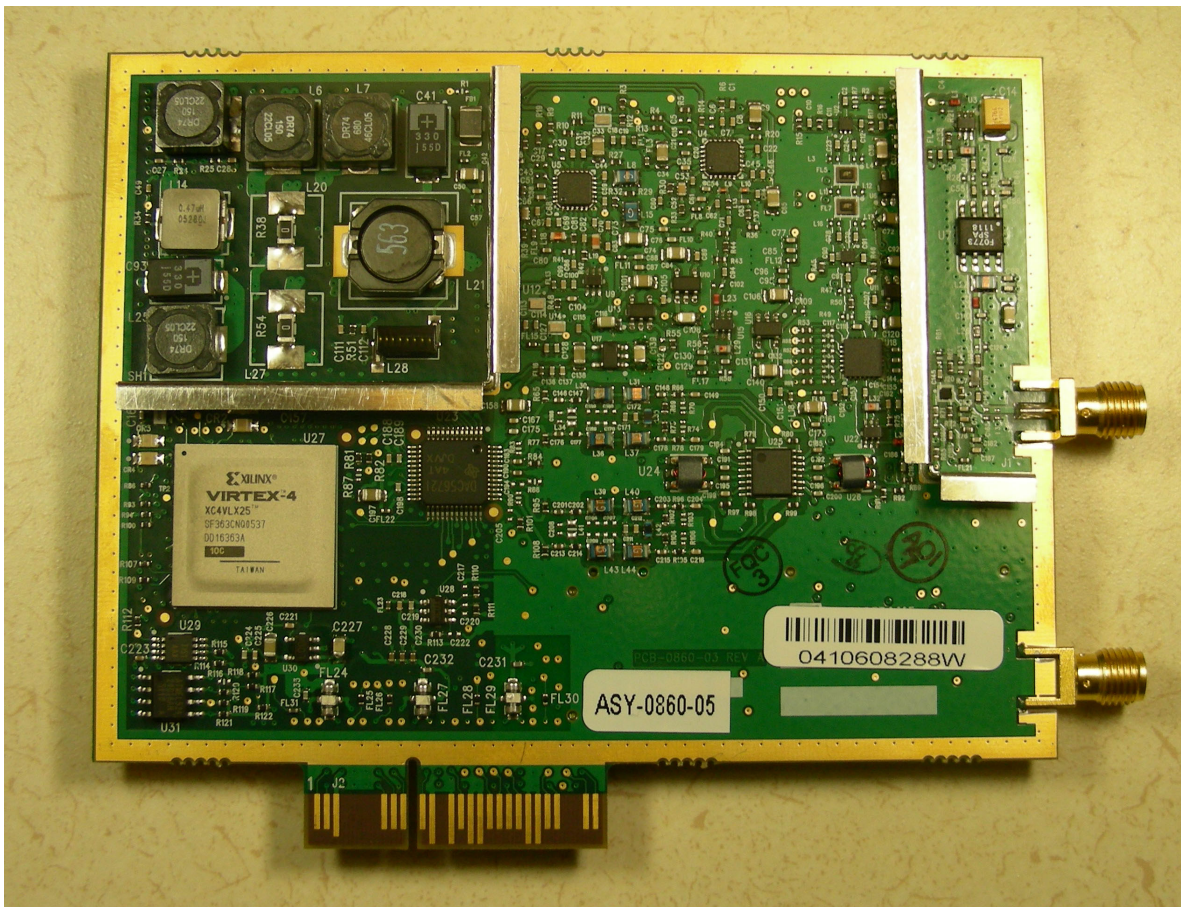
MCRB PCB Back
