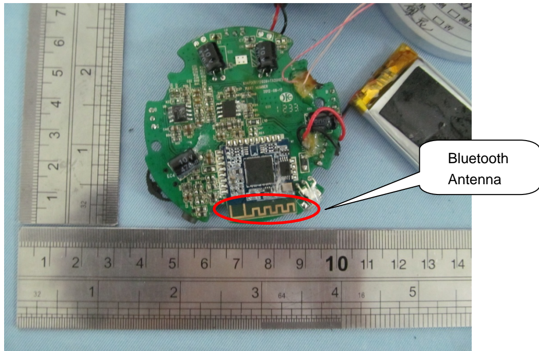
BACK VIEW OF PCB-1
