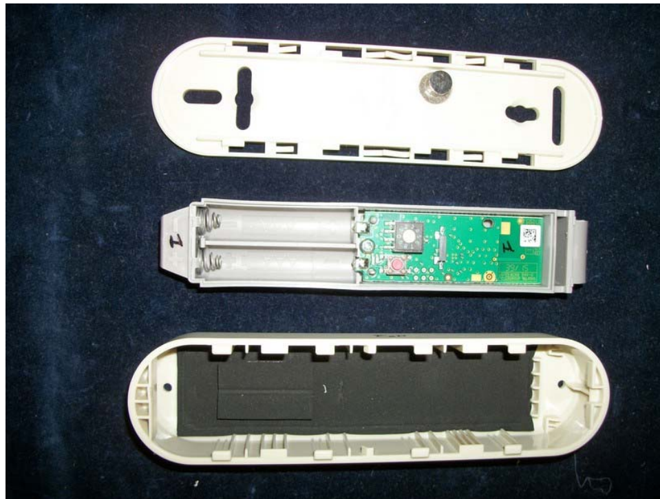
Figure 7.3 Internal View
