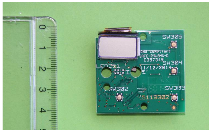
Figure 7.5 Foil Side (5 Channel, 2008776)
