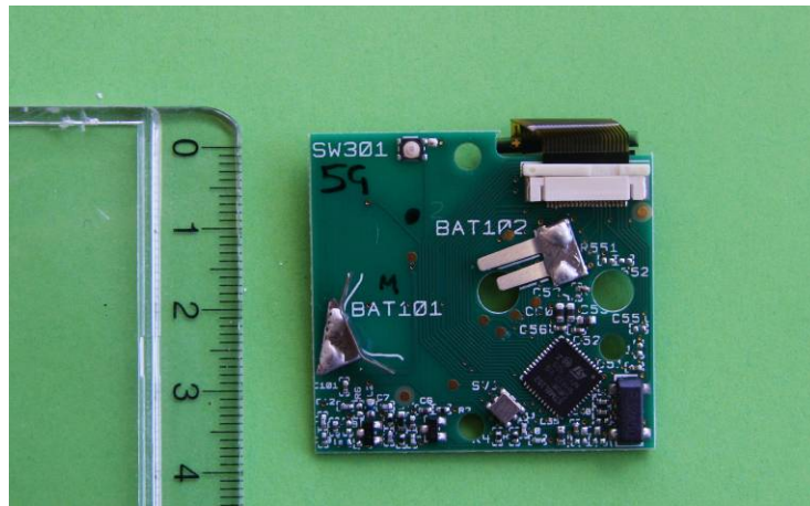
Figure 7.4 Component Side (5 Channel, 2008776)
