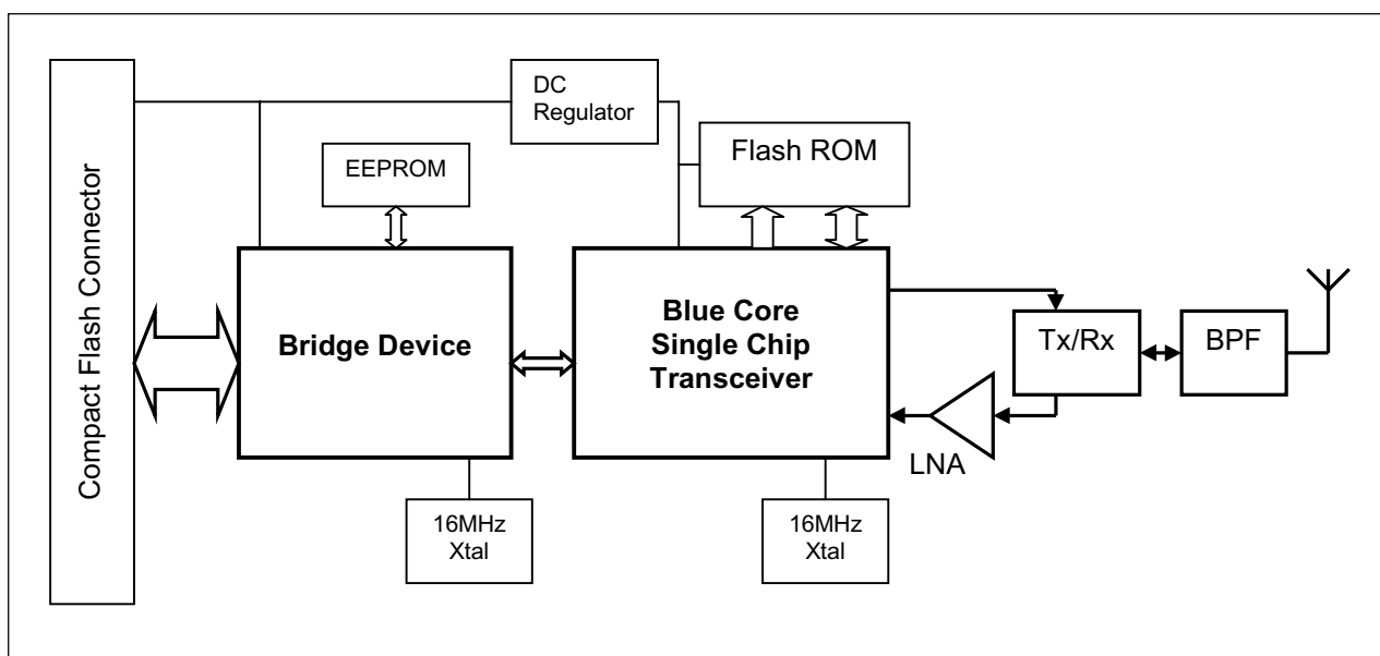
Figure 1: Block Diagram
