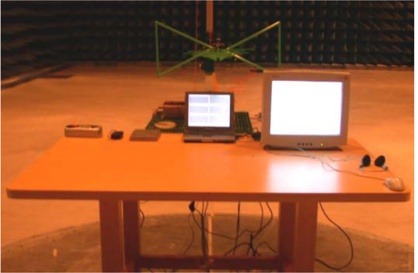
Test Setup photos
