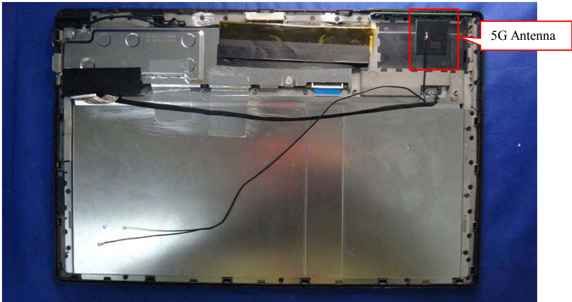
(22) EUT Photo
