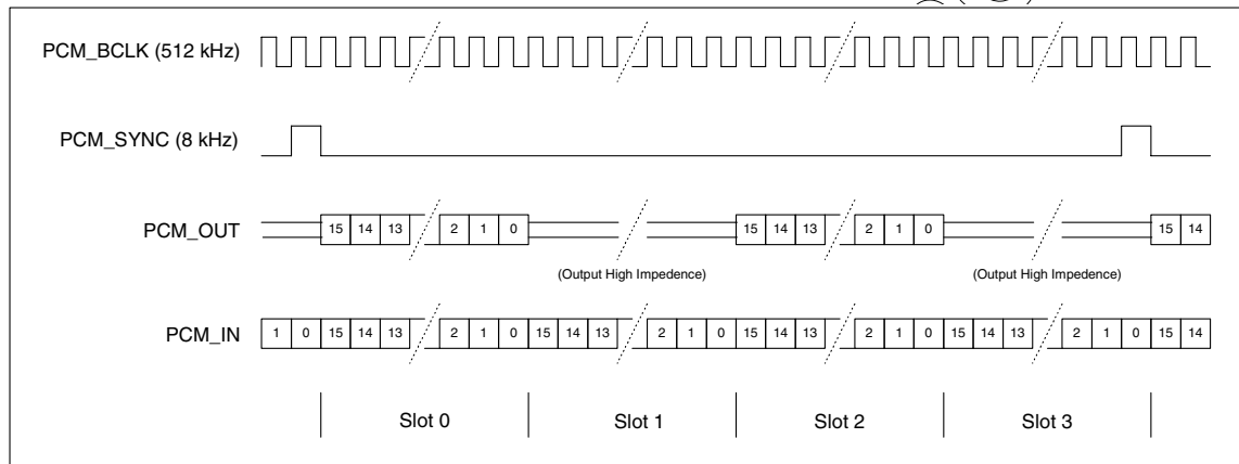
Figure 30: PCM Time Slots Example
