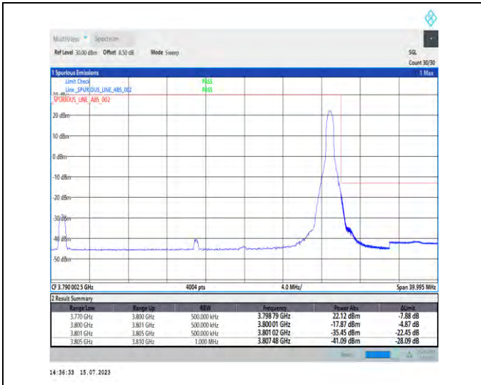
1-N78-3700-3800-PC1-30-30-H-2-DFT-PI2BPSK-Edge_1RB_Right-1@77-Ant1-1--PASS-see graph
