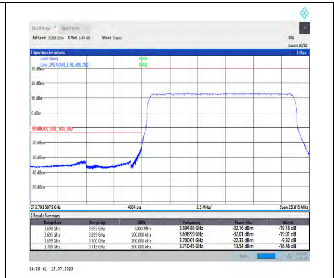
1-N78-3700-3800-PC1-30-15-L-3-DFT-PI2BPSK-Outer_Full-36@0-Ant1-1--PASS-see graph
