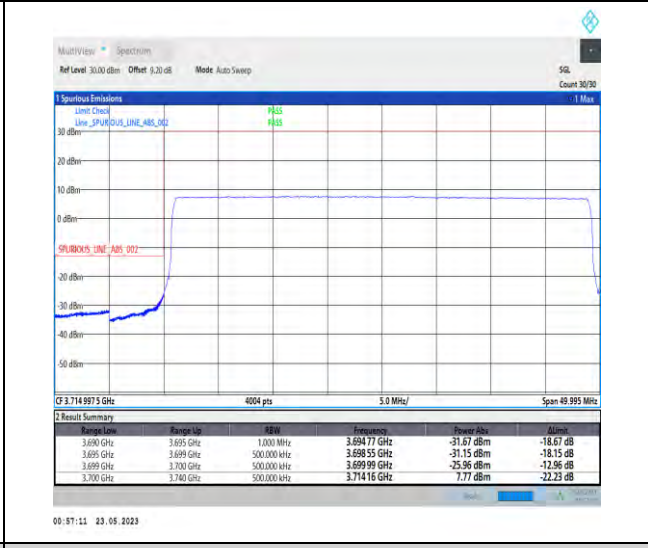
1-N78-3700-3800-PC1-30-40-L-6-CP-QPSK-Outer_Full-106@0-Ant1-1--PASS-see graph
