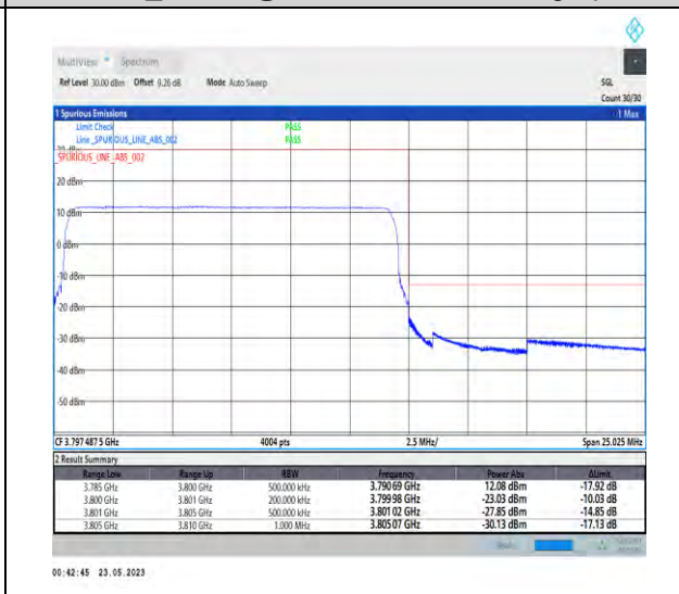
1-N78-3700-3800-PC1-30-15-H-6-CP-QPSK-Outer_Full-38@0-Ant1-1--PASS-see graph
