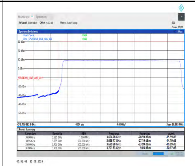
1-N78-3700-3800-PC1-30-30-L-6-CP-QPSK-Outer_Full-78@0-Ant1-1--PASS-see graph
