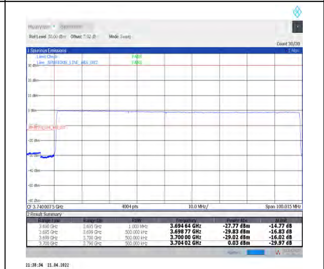
1-N78-3700-3800--30-90-L-6-CP-QPSK-Outer_Ful_I-245@0-Ant1-PASS-see graph
