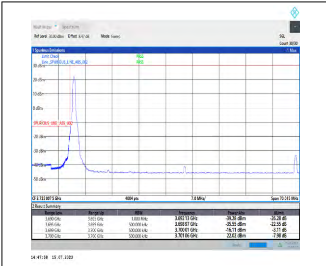
1-N78-3700-3800-PC1-30-60-L-1-DFT-PI2BPSK-Edge_1_RB_Left-1@0-Ant1-1--PASS-see graph
