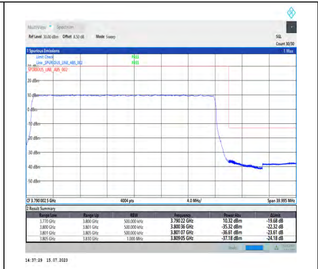
1-N78-3700-3800-PC1-30-30-H-3-DFT-PI2BPSK-Outer_Full-75@0-Ant1-1--PASS-see graph
