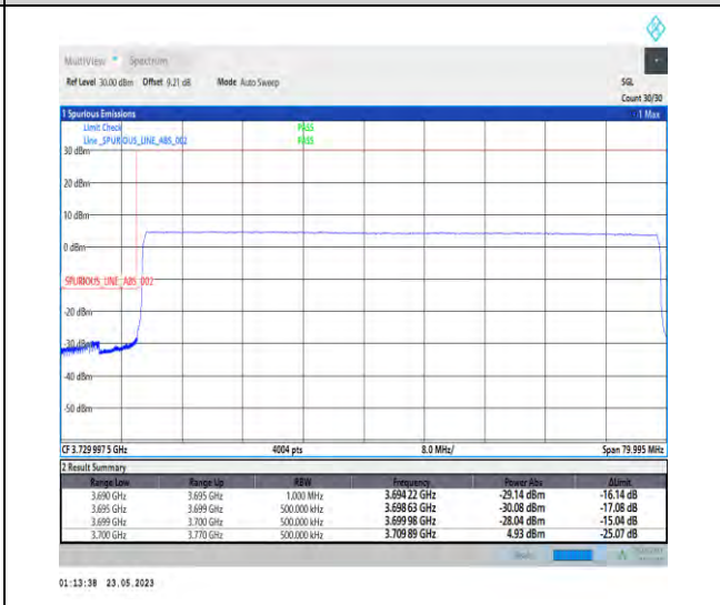
1-N78-3700-3800-PC1-30-70-L-6-CP-QPSK-Outer_Full-189@0-Ant1-1--PASS-see graph
