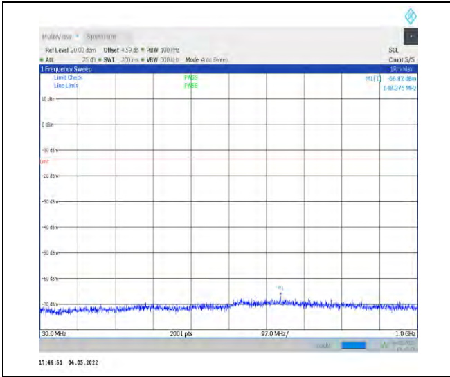
1-N78-3700-3800--30-100-M-1-DFT-PI2BPSK-Inner _1RB_Left-1@1-30-1000-Ant1--66.82--13-PASS
