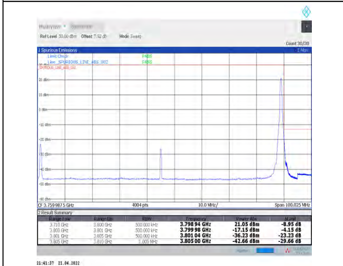
1-N78-3700-3800--30-90-H-5-CP-QPSK-Edge_1RB_Right-1@244-Ant1-PASS-see graph
