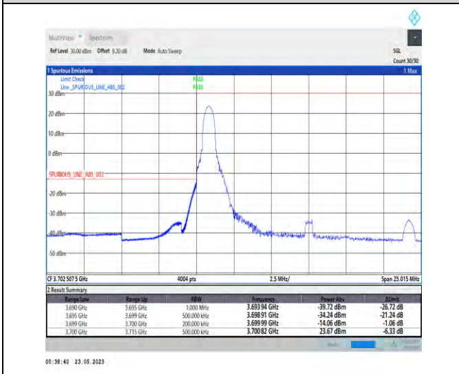
1-N78-3700-3800-PC1-30-15-L-4-CP-QPSK-Edge_1_RB_Left-1@0-Ant1-1--PASS-see graph
