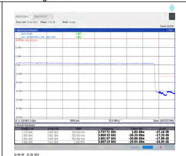
1-N78-3700-3800--30-90-H-3-DFT-PI2BPSK-Outer_Full-240@0-Ant1-PASS-see graph
