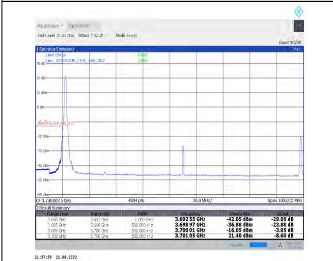
1-N78-3700-3800--30-90-L-4-CP-QPSK-Edge_1RB_L_eff-1@0-Ant1-PASS-see graph
