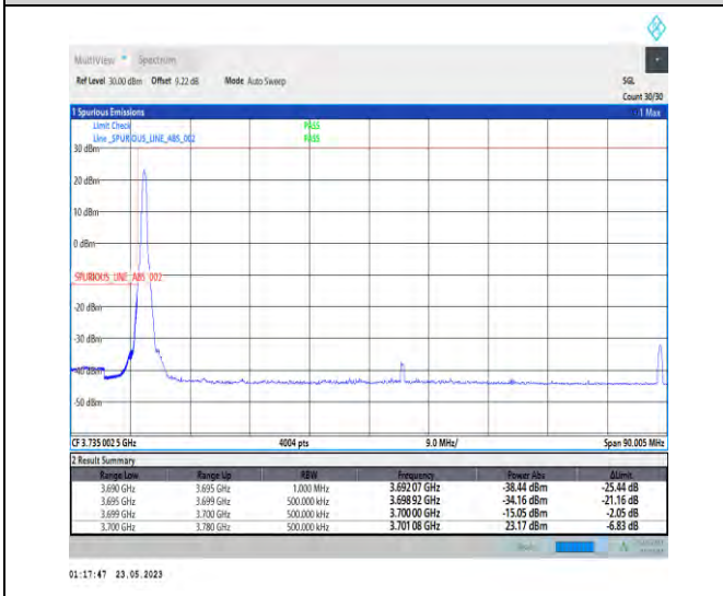
1-N78-3700-3800-PC1-30-80-L-4-CP-QPSK-Edge_1RB_Left-1@0-Ant1-1--PASS-see graph
