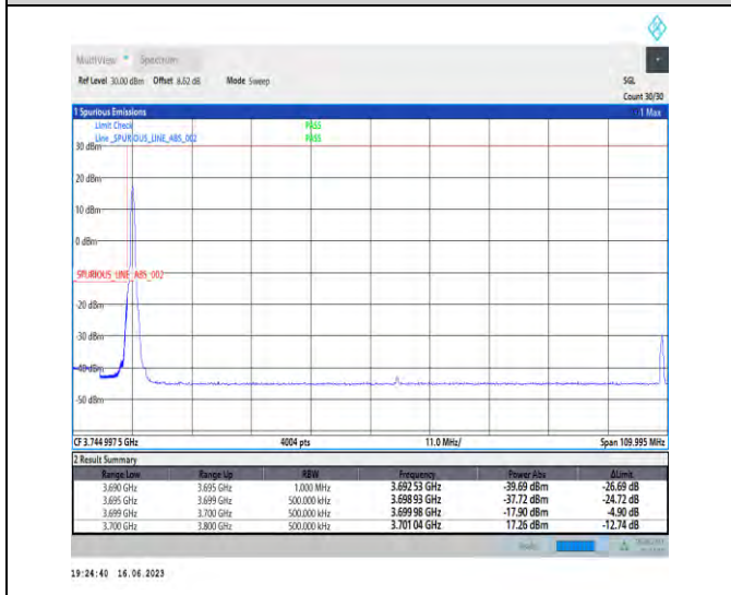
1-N78-3700-3800-PC1-30-100-L-4-CP-QPSK-Edge_1RB_Left-1@0-Ant1-1--PASS-see graph
