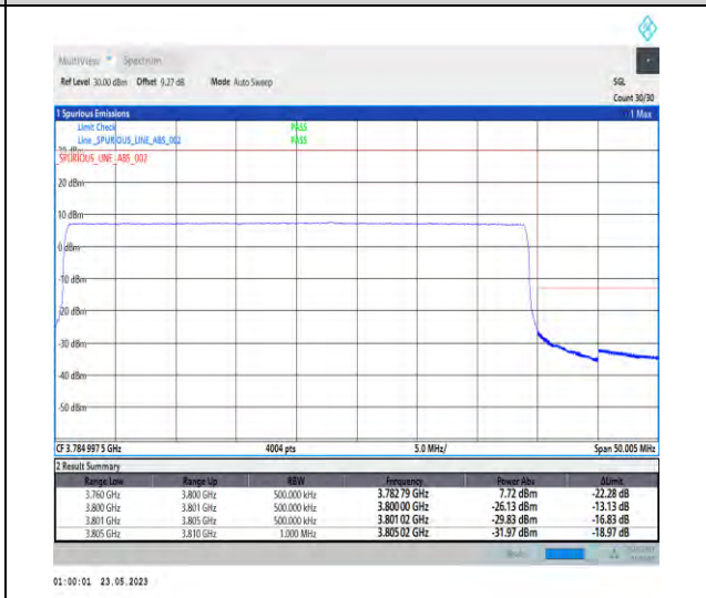
1-N78-3700-3800-PC1-30-40-H-6-CP-QPSK-Outer_Full-106@0-Ant1-1--PASS-see graph
