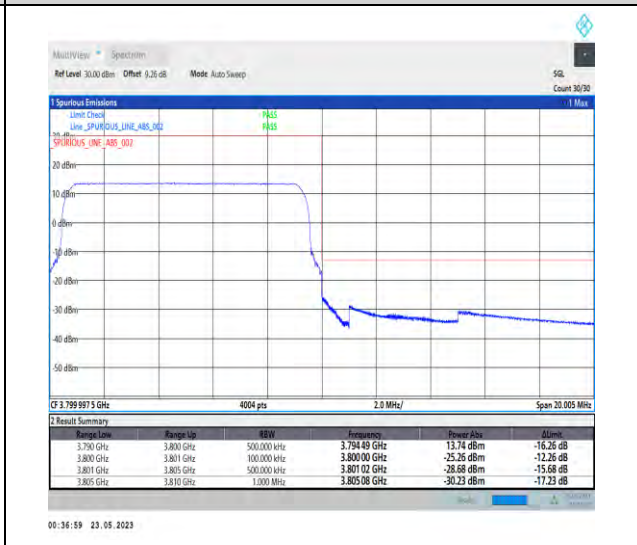
1-N78-3700-3800-PC1-30-10-H-6-CP-QPSK-Outer_Full-24@0-Ant1-1--PASS-see graph
