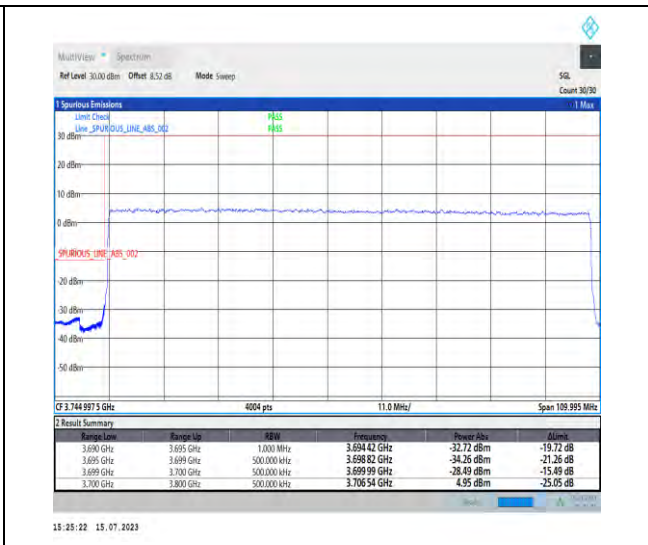
1-N78-3700-3800-PC1-30-100-L-3-DFT-PI2BPSK-Outer_Full-270@0-Ant1-1--PASS-see graph
