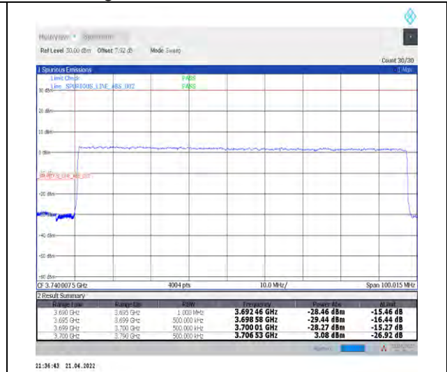
1-N78-3700-3800--30-90-L-3-DFT-PI2BPSK-Outer_Full-240@0-Ant1-PASS-see graph
