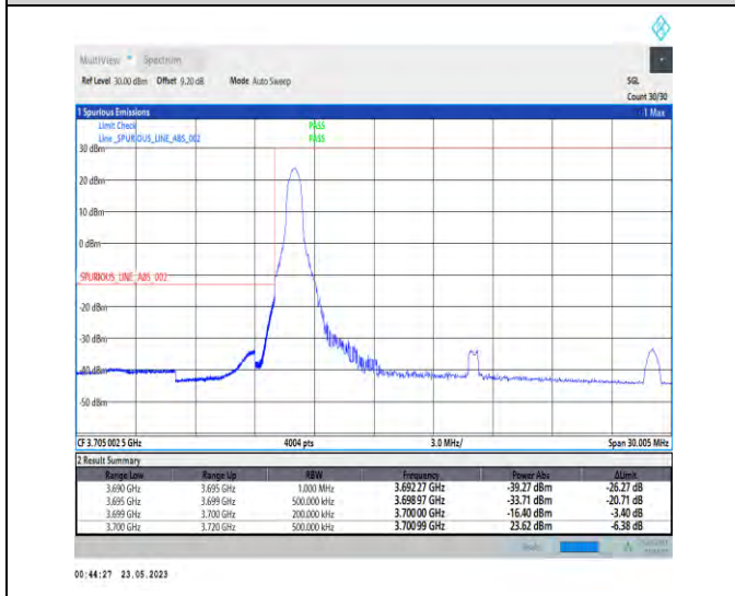
1-N78-3700-3800-PC1-30-20-L-4-CP-QPSK-Edge_1_RB_Left-1@0-Ant1-1--PASS-see graph
