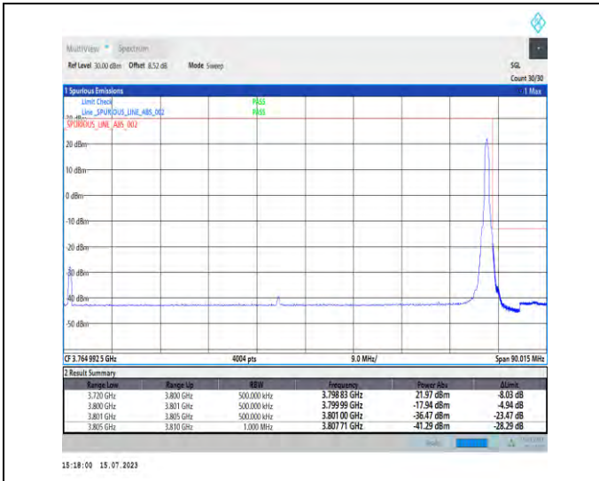
1-N78-3700-3800-PC1-30-80-H-2-DFT-PI2BPSK-Edge_1RB_Right-1@216-Ant1-1--PASS-see graph
