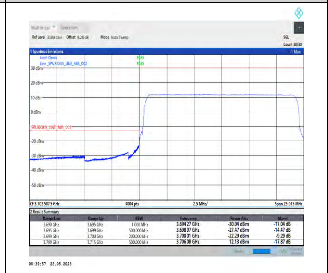
1-N78-3700-3800-PC1-30-15-L-6-CP-QPSK-Outer_Full-38@0-Ant1-1--PASS-see graph
