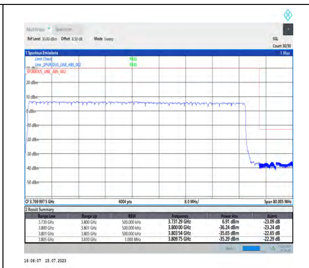
1-N78-3700-3800-PC1-30-70-H-3-DFT-PI2BPSK-Outer_Full-180@0-Ant1-1--PASS-see graph
