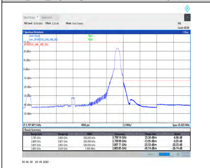
1-N78-3700-3800-PC1-30-15-H-5-CP-QPSK-Edge_1RB_Right-1@37-Ant1-1--PASS-see graph
