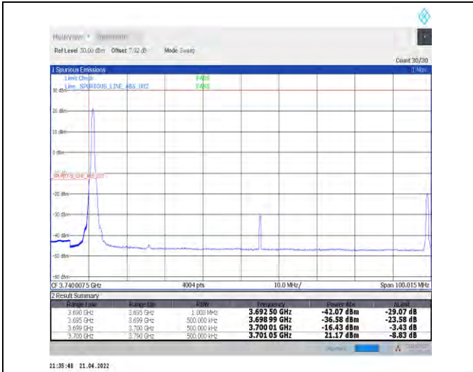
1-N78-3700-3800--30-90-L-1-DFT-PI2BPSK-Edge_1R_B_Left-1@0-Ant1-PASS-see graph
