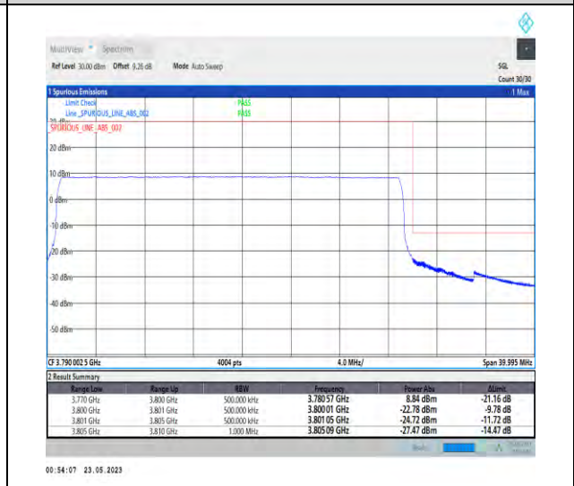
1-N78-3700-3800-PC1-30-30-H-6-CP-QPSK-Outer_Full-78@0-Ant1-1--PASS-see graph
