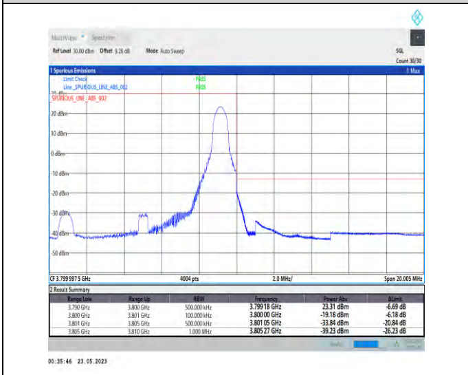
1-N78-3700-3800-PC1-30-10-H-5-CP-QPSK-Edge_1RB_Right-1@23-Ant1-1--PASS-see graph
