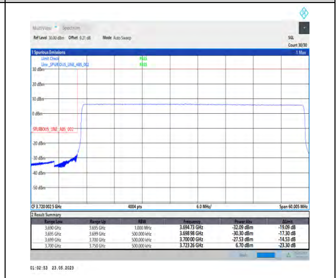
1-N78-3700-3800-PC1-30-50-L-6-CP-QPSK-Outer_Full-133@0-Ant1-1--PASS-see graph
