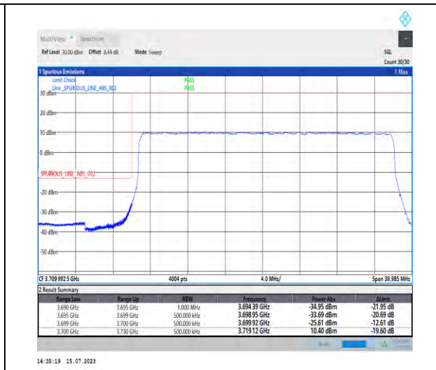
1-N78-3700-3800-PC1-30-30-L-3-DFT-PI2BPSK-Outer_Full-75@0-Ant1-1--PASS-see graph
