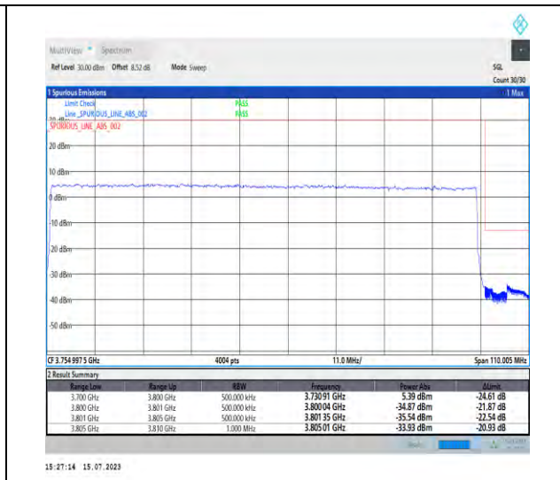
1-N78-3700-3800-PC1-30-100-H-3-DFT-PI2BPSK-Outer_Full-270@0-Ant1-1--PASS-see graph
