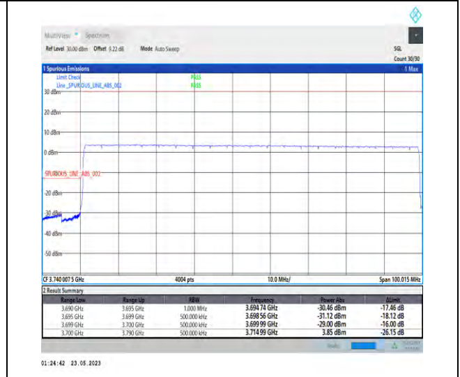
1-N78-3700-3800-PC1-30-90-L-6-CP-QPSK-Outer_Full-245@0-Ant1-1--PASS-see graph
