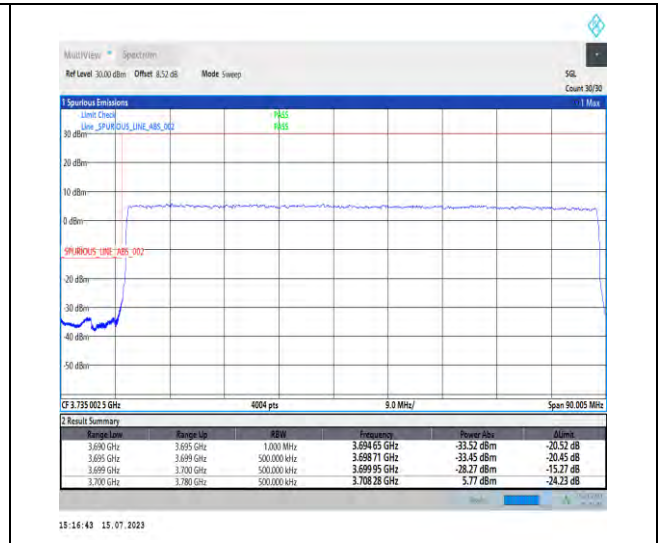
1-N78-3700-3800-PC1-30-80-L-3-DFT-PI2BPSK-Outer_Full-216@0-Ant1-1--PASS-see graph
