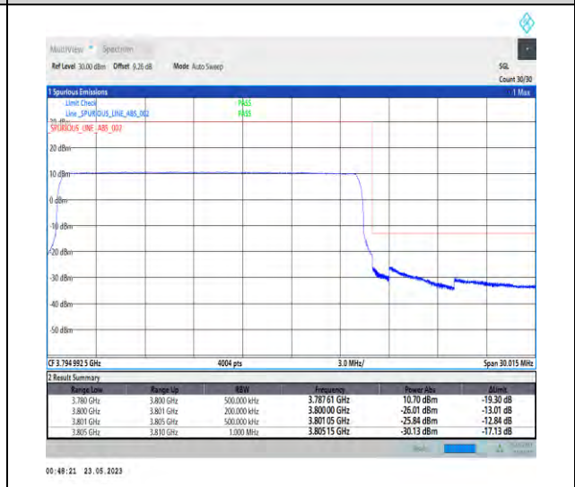
1-N78-3700-3800-PC1-30-20-H-6-CP-QPSK-Outer_Full-51@0-Ant1-1--PASS-see graph
