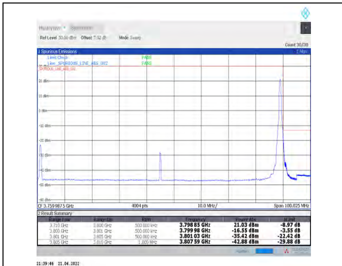
1-N78-3700-3800--30-90-H-2-DFT-PI2BPSK-Edge_1R_B_Right-1@244-Ant1-PASS-see graph
