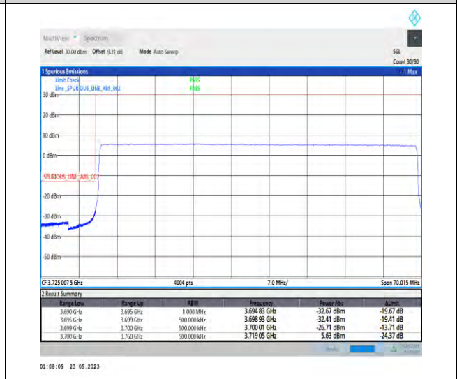
1-N78-3700-3800-PC1-30-60-L-6-CP-QPSK-Outer_Full-162@0-Ant1-1--PASS-see graph
