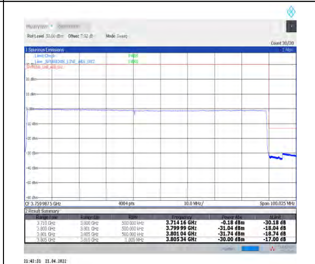
1-N78-3700-3800--30-90-H-6-CP-QPSK-Outer_Full-245@0-Ant1-PASS-see graph
