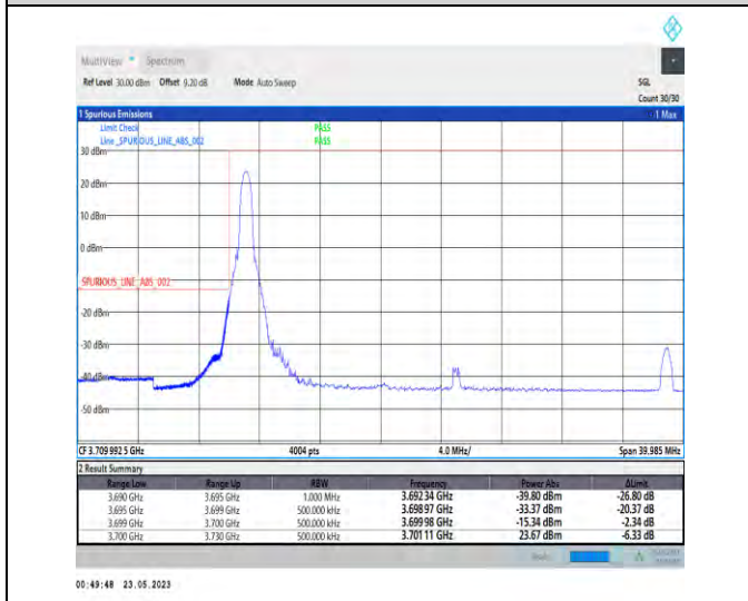
1-N78-3700-3800-PC1-30-30-L-4-CP-QPSK-Edge_1_RB_Left-1@0-Ant1-1--PASS-see graph
