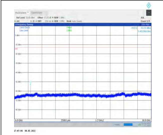
1-N78-3700-3800--30-100-M-1-DFT-PI2BPSK-Inner _1RB_Left-1@1-6000-18000-Ant1--53.72--13-PASS
