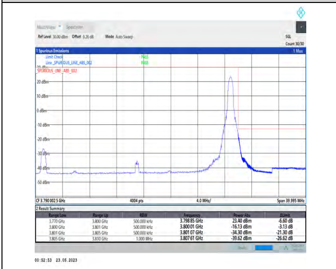
1-N78-3700-3800-PC1-30-30-H-5-CP-QPSK-Edge_1R_B_Right-1@77-Ant1-1--PASS-see graph
