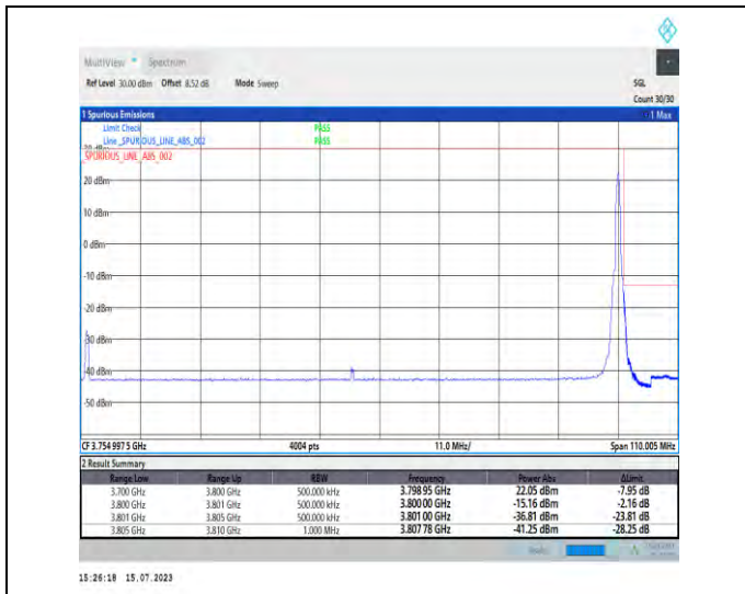
1-N78-3700-3800-PC1-30-100-H-2-DFT-PI2BPSK-Edge_e_1RB_Right-1@272-Ant1-1--PASS-see graph
