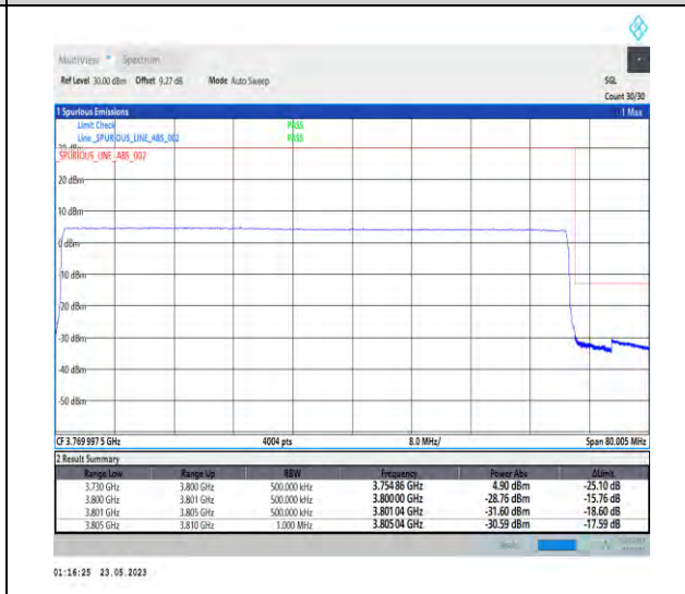
1-N78-3700-3800-PC1-30-70-H-6-CP-QPSK-Outer_Full-189@0-Ant1-1--PASS-see graph
