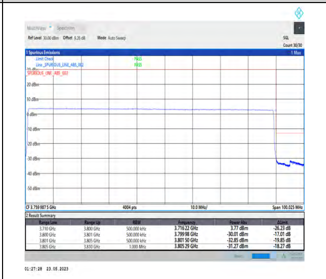
1-N78-3700-3800-PC1-30-90-H-6-CP-QPSK-Outer_Full-245@0-Ant1-1--PASS-see graph
