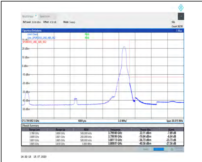
1-N78-3700-3800-PC1-30-20-H-2-DFT-PI2BPSK-Edge_1RB_Right-1@50-Ant1-1--PASS-see graph
