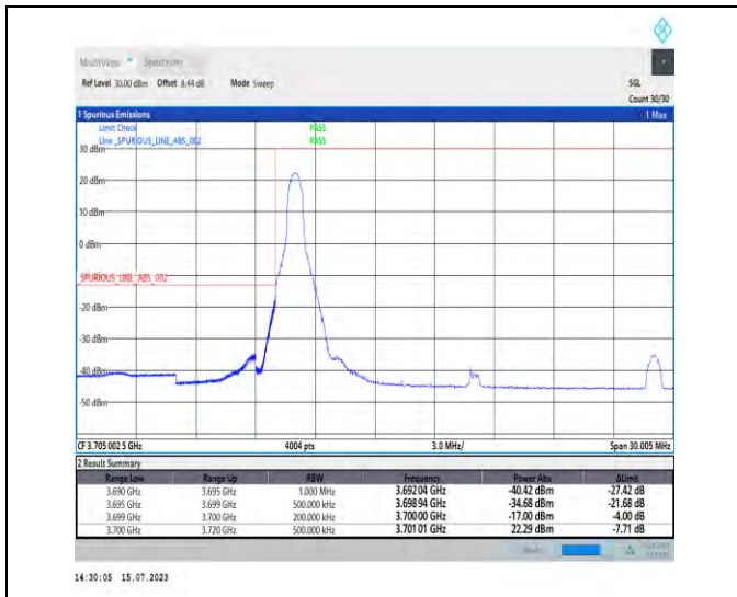
1-N78-3700-3800-PC1-30-20-L-1-DFT-PI2BPSK-Edge_1_RB_Left-1@0-Ant1-1--PASS-see graph
