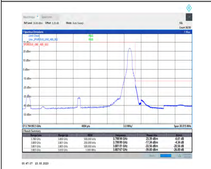
1-N78-3700-3800-PC1-30-20-H-5-CP-QPSK-Edge_1RB_Right-1@50-Ant1-1--PASS-see graph
