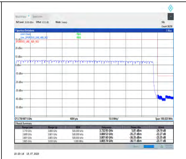
1-N78-3700-3800-PC1-30-90-H-3-DFT-PI2BPSK-Outer_Full-240@0-Ant1-1--PASS-see graph
