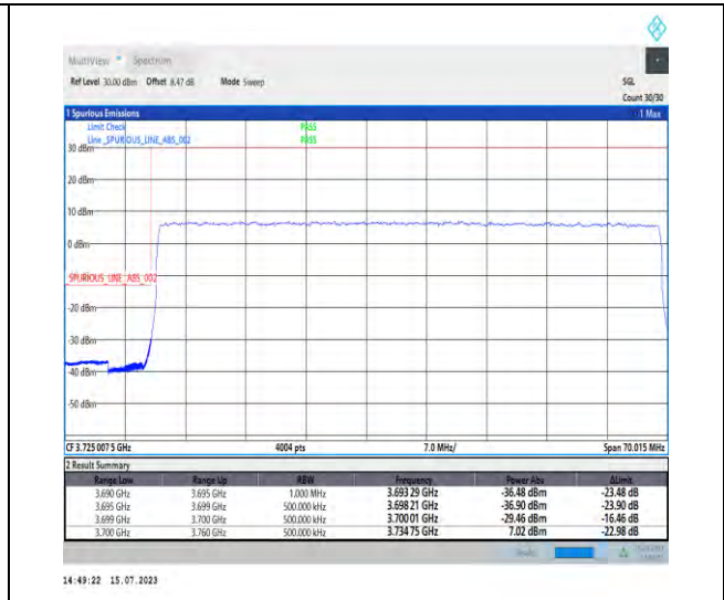
1-N78-3700-3800-PC1-30-60-L-3-DFT-PI2BPSK-Outer_Full-162@0-Ant1-1--PASS-see graph
