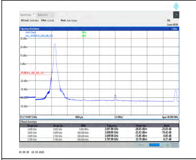
1-N78-3700-3800-PC1-30-40-L-4-CP-QPSK-Edge_1_RB_Left-1@0-Ant1-1--PASS-see graph
