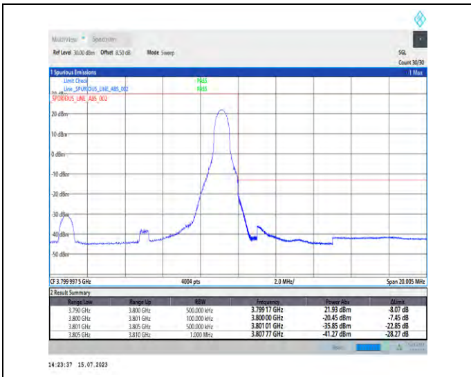
1-N78-3700-3800-PC1-30-10-H-2-DFT-PI2BPSK-Edge_1RB_Right-1@23-Ant1-1--PASS-see graph
