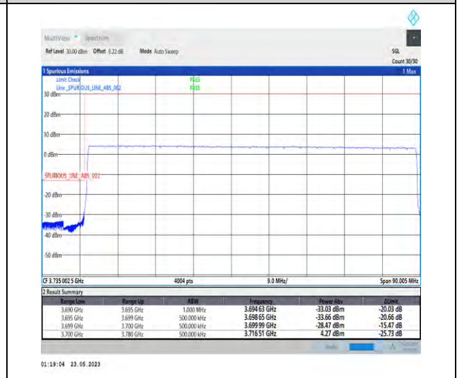
1-N78-3700-3800-PC1-30-80-L-6-CP-QPSK-Outer_Full-217@0-Ant1-1--PASS-see graph
