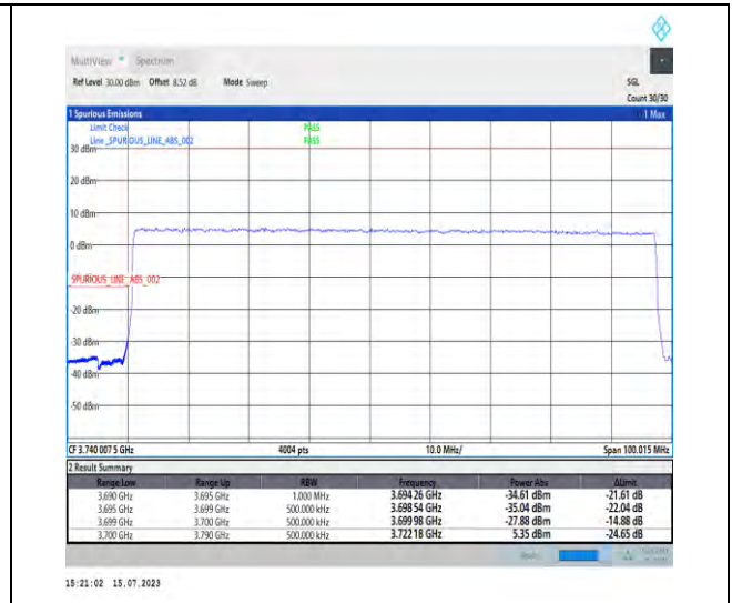
1-N78-3700-3800-PC1-30-90-L-3-DFT-PI2BPSK-Outer_Full-240@0-Ant1-1--PASS-see graph
