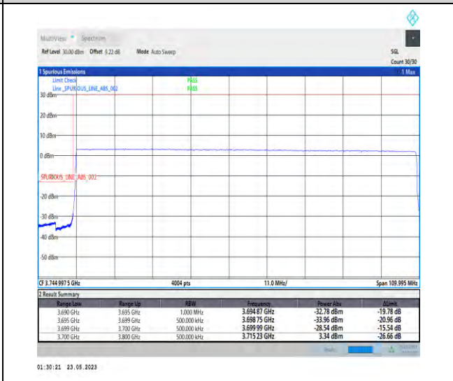
1-N78-3700-3800-PC1-30-100-L-6-CP-QPSK-Outer_Full-273@0-Ant1-1--PASS-see graph
