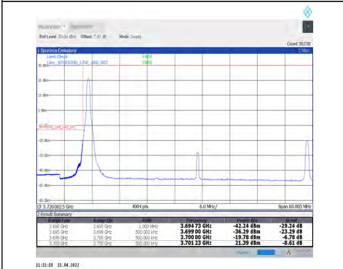
1-N78-3700-3800--30-50-L-4-CP-QPSK-Edge_1RB_L_eff-1@0-Ant1-PASS-see graph
