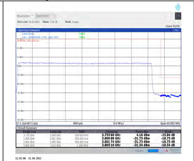
1-N78-3700-3800--30-70-H-3-DFT-PI2BPSK-Outer_Full-180@0-Ant1-PASS-see graph
