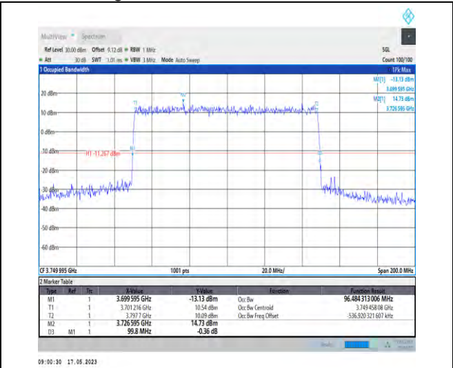
1-N78-3700-3800-PC1-30-100-L-4-DFT-64QAM-Out er_Full-270@0-Ant1-96.484-99.800-≤100-PASS
