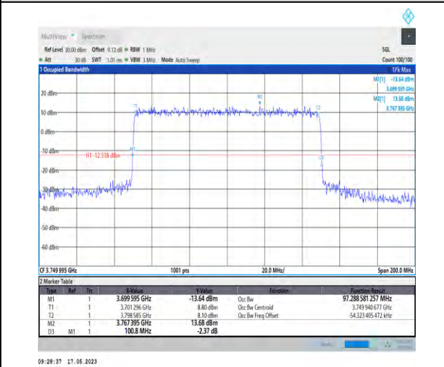
1-N78-3700-3800-PC1-30-100-H-8-CP-64QAM-Outer_Full-273@0-Ant1-97.289-100.800-≤100-PASS
