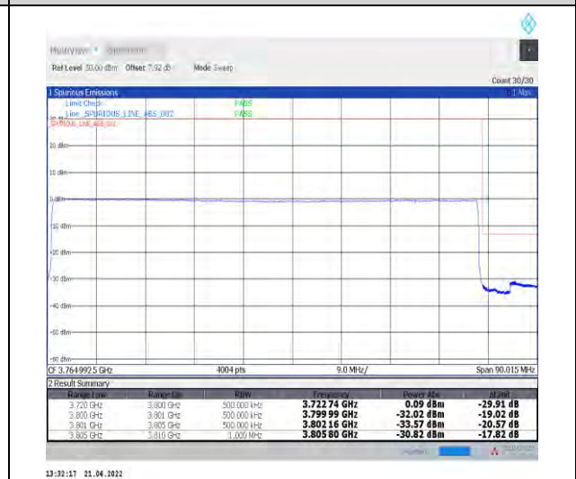
1-N78-3700-3800--30-80-H-6-CP-QPSK-Outer_Fu ll-217@0-Ant1-PASS-see graph
