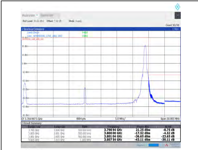
1-N78-3700-3800--30-40-H-2-DFT-PI2BPSK-Edge_1R_B_Right-1@105-Ant1-PASS-see graph
