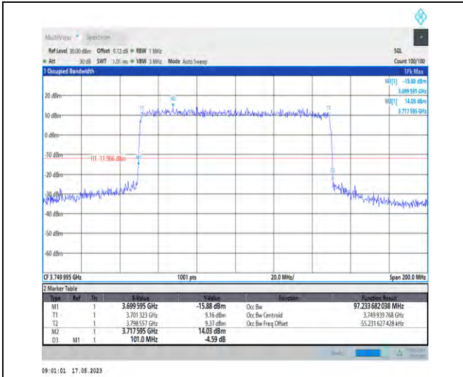
1-N78-3700-3800-PC1-30-100-L-7-CP-16QAM-Outer_Full-273@0-Ant1-97.234-101.000-≤100-PASS
