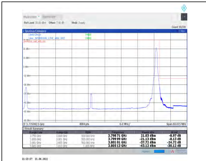
1-N78-3700-3800--30-50-H-2-DFT-PI2BPSK-Edge_1R_B_Right-1@132-Ant1-PASS-see graph
