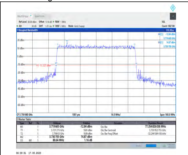
1-N78-3700-3800-PC1-30-80-H-8-CP-64QAM-Outer_Full-217@0-Ant1-77.355-80.640-<math>\leq 80</math>-PASS
