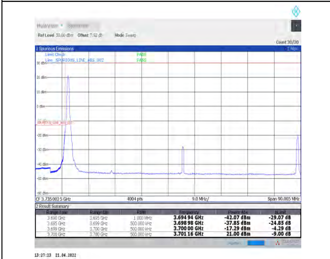
1-N78-3700-3800--30-80-L-4-CP-QPSK-Edge_1RB_L_eff-1@0-Ant1-PASS-see graph
