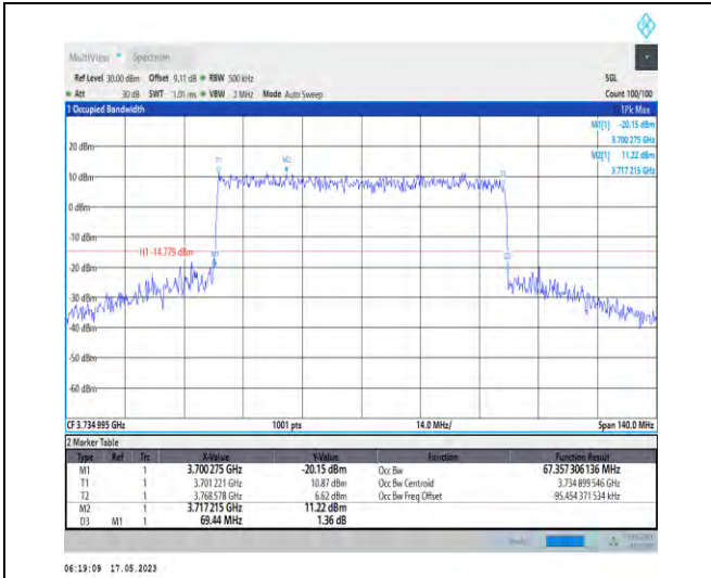
1-N78-3700-3800-PC1-30-70-L-8-CP-64QAM-Outer_Full-189@0-Ant1-67.357-69.440-≤70-PASS
