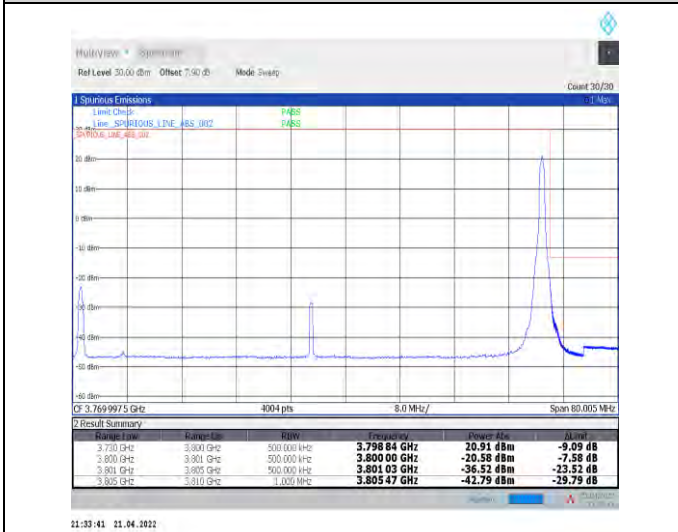
1-N78-3700-3800--30-70-H-5-CP-QPSK-Edge_1RB_Right-1@188-Ant1-PASS-see graph
