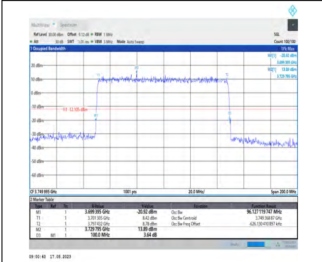
1-N78-3700-3800-PC1-30-100-L-5-DFT-256QAM-Out er_Full-270@0-Ant1-96.127-100.000-≤100-PASS
