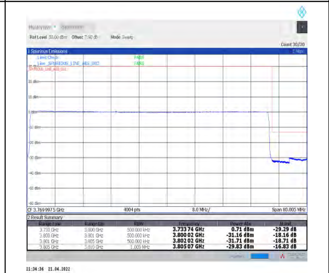
1-N78-3700-3800--30-70-H-6-CP-QPSK-Outer_Full-189@0-Ant1-PASS-see graph
