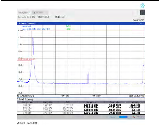
1-N78-3700-3800--30-80-L-1-DFT-PI2BPSK-Edge_1R_B_Left-1@0-Ant1-PASS-see graph
