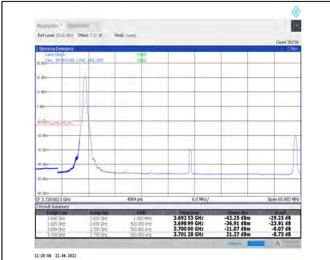
1-N78-3700-3800--30-50-L-1-DFT-PI2BPSK-Edge_1R_B_Left-1@0-Ant1-PASS-see graph
