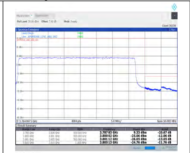
1-N78-3700-3800--30-40-H-3-DFT-PI2BPSK-Outer_Full-100@0-Ant1-PASS-see graph
