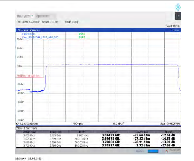
1-N78-3700-3800--30-50-L-6-CP-QPSK-Outer_Ful_I-133@0-Ant1-PASS-see graph
