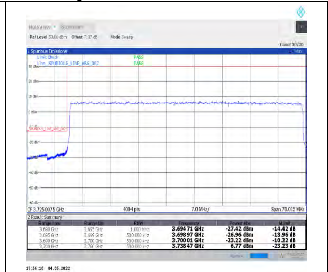
1-N78-3700-3800--30-60-L-3-DFT-PI2BPSK-Outer_Full-162@0-Ant1-PASS-see graph
