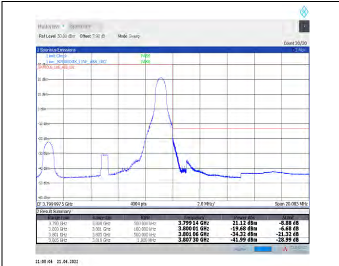
1-N78-3700-3800--30-10-H-2-DFT-PI2BPSK-Edge_1R_B_Right-1@23-Ant1-PASS-see graph
