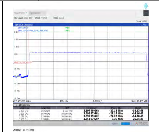
1-N78-3700-3800--30-80-L-3-DFT-PI2BPSK-Outer_Full-216@0-Ant1-PASS-see graph
