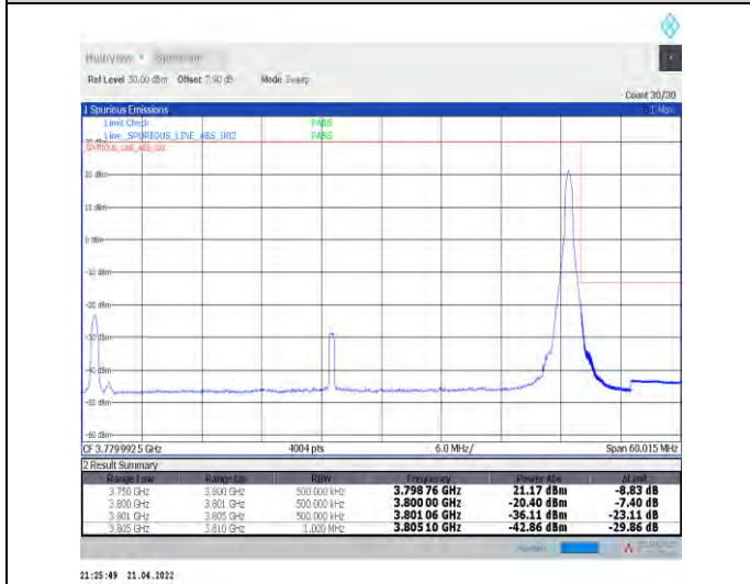
1-N78-3700-3800--30-50-H-5-CP-QPSK-Edge_1RB_R ight-1@132-Ant1-PASS-see graph
