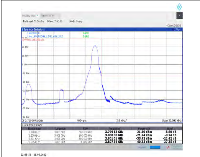
1-N78-3700-3800--30-10-H-5-CP-QPSK-Edge_1RB_R ight-1@23-Ant1-PASS-see graph
