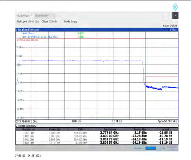
1-N78-3700-3800--30-40-H-6-CP-QPSK-Outer_Fu ll-106@0-Ant1-PASS-see graph
