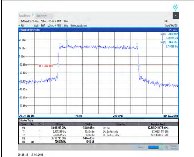
1-N78-3700-3800-PC1-30-100-H-7-CP-16QAM-Outer_Full-273@0-Ant1-97.303-100.800-≤100-PASS
