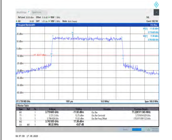
1-N78-3700-3800-PC1-30-80-H-1-DFT-QPSK-Outer_Full-216@0-Ant1-77.229-80.320-≤80-PASS
