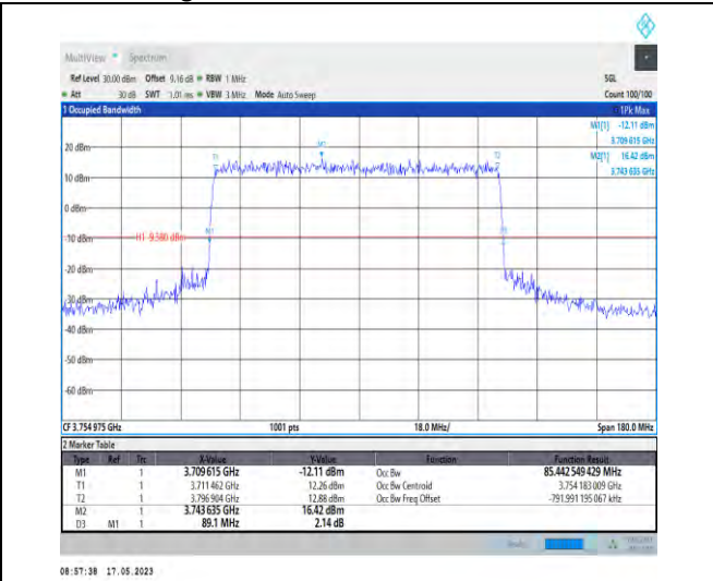
1-N78-3700-3800-PC1-30-90-H-1-DFT-QPSK-Outer_Full-240@0-Ant1-85.443-89.100-≤90-PASS
