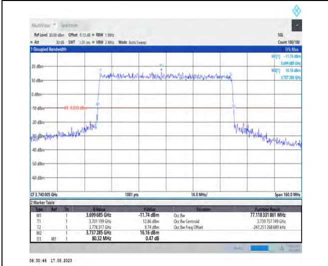
1-N78-3700-3800-PC1-30-80-L-3-DFT-16QAM-Outer_Full-216@0-Ant1-77.118-80.320-≤80-PASS
