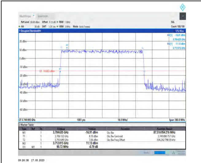
1-N78-3700-3800-PC1-30-90-M-9-CP-256QAM-Outer_Full-245@0-Ant1-87.517-90.720-≤90-PASS
