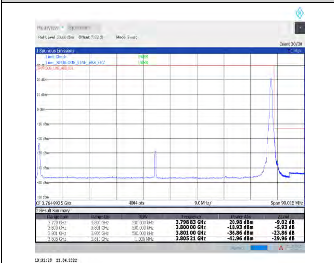
1-N78-3700-3800--30-80-H-5-CP-QPSK-Edge_1RB_R ight-1@216-Ant1-PASS-see graph
