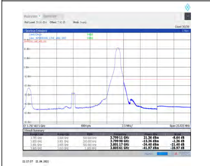
1-N78-3700-3800--30-15-H-5-CP-QPSK-Edge_1RB_R ight-1@37-Ant1-PASS-see graph
