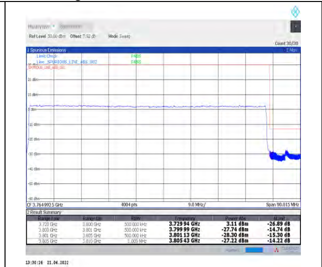
1-N78-3700-3800--30-80-H-3-DFT-PI2BPSK-Outer_Full-216@0-Ant1-PASS-see graph
