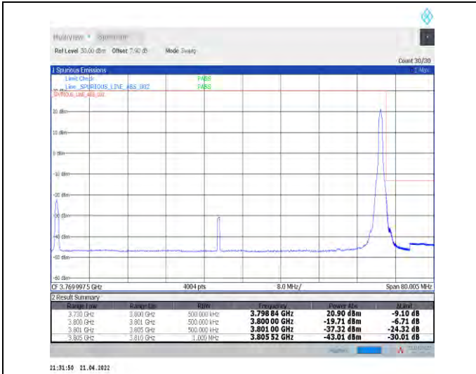
1-N78-3700-3800--30-70-H-2-DFT-PI2BPSK-Edge_1R_B_Right-1@188-Ant1-PASS-see graph
