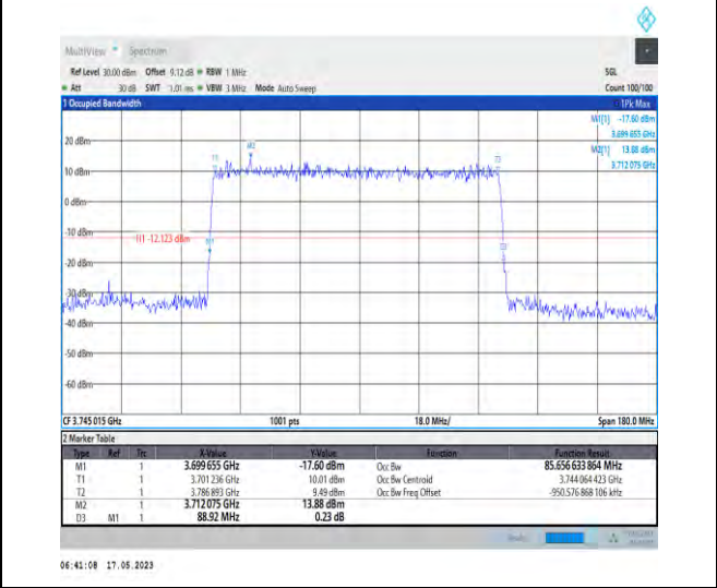
1-N78-3700-3800-PC1-30-90-L-5-DFT-256QAM-Outer_Full-240@0-Ant1-85.657-88.920-<90-PASS
