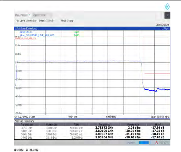
1-N78-3700-3800--30-50-H-6-CP-QPSK-Outer_Fu ll-133@0-Ant1-PASS-see graph
