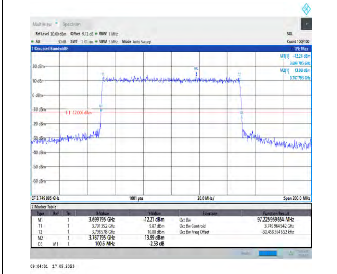
1-N78-3700-3800-PC1-30-100-M-8-CP-64QAM-Outer_Full-273@0-Ant1-97.226-100.600-≤100-PASS
