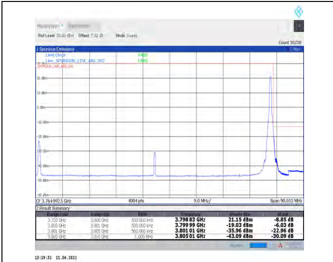
1-N78-3700-3800--30-80-H-2-DFT-PI2BPSK-Edge_1R_B_Right-1@216-Ant1-PASS-see graph
