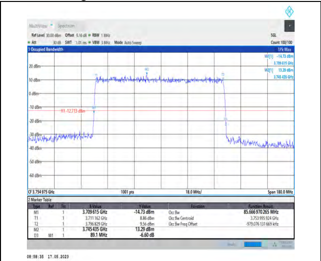
1-N78-3700-3800-PC1-30-90-H-5-DFT-256QAM-Outer_Full-240@0-Ant1-85.667-89.100-≤90-PASS
