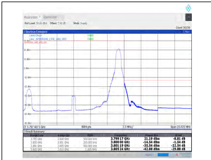
1-N78-3700-3800--30-15-H-2-DFT-PI2BPSK-Edge_1R_B_Right-1@37-Ant1-PASS-see graph
