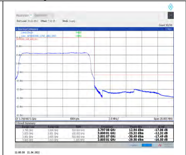
1-N78-3700-3800--30-10-H-3-DFT-PI2BPSK-Outer_Full-24@0-Ant1-PASS-see graph
