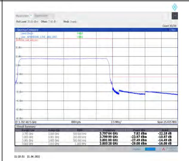
1-N78-3700-3800--30-15-H-6-CP-QPSK-Outer_Fu ll-38@0-Ant1-PASS-see graph
