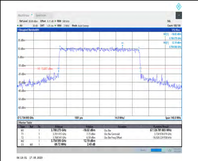
1-N78-3700-3800-PC1-30-70-L-7-CP-16QAM-Outer_Full-189@0-Ant1-67.127-69.720-≤70-PASS
