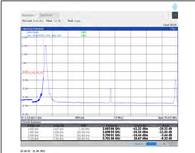
1-N78-3700-3800--30-60-L-1-DFT-PI2BPSK-Edge_1R_B_Left-1@0-Ant1-PASS-see graph
