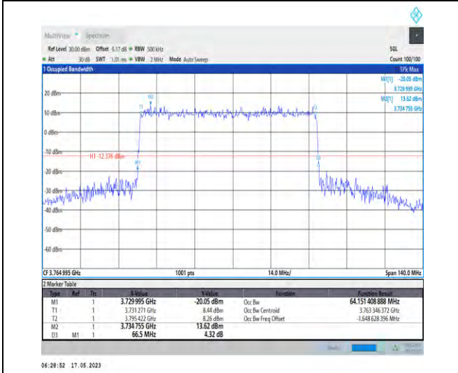
1-N78-3700-3800-PC1-30-70-H-4-DFT-64QAM-Outer_Full-180@0-Ant1-64.151-66.500-≤70-PASS
