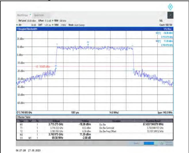
1-N78-3700-3800-PC1-30-70-M-8-CP-64QAM-Outer _Full-189@0-Ant1-67.433-69.580-≤70-PASS
