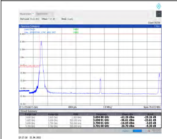
1-N78-3700-3800--30-60-L-4-CP-QPSK-Edge_1RB_L_eff-1@0-Ant1-PASS-see graph
