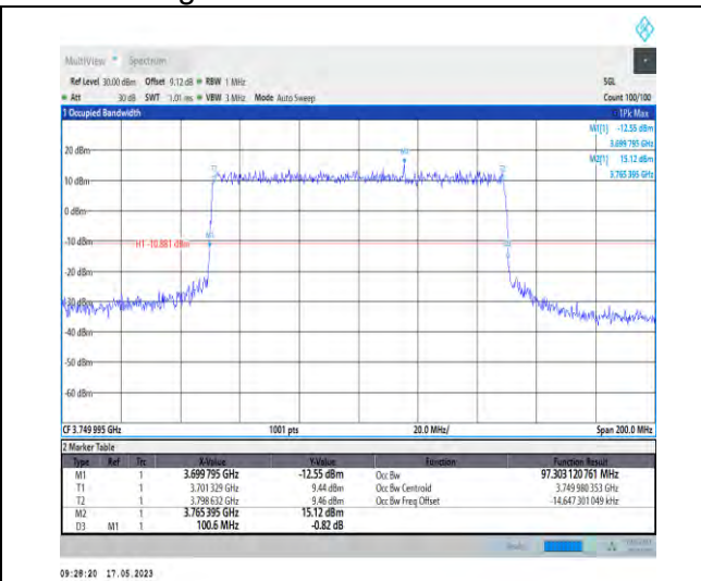
1-N78-3700-3800-PC1-30-100-H-6-CP-QPSK-Outer_Full-273@0-Ant1-97.303-100.600-≤100-PASS
