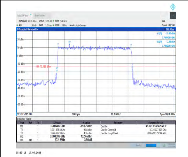
1-N78-3700-3800-PC1-30-50-L-5-DFT-256QAM-Out er_Full-128@0-Ant1-45.701-47.400-<math>\leq 50</math>-PASS
