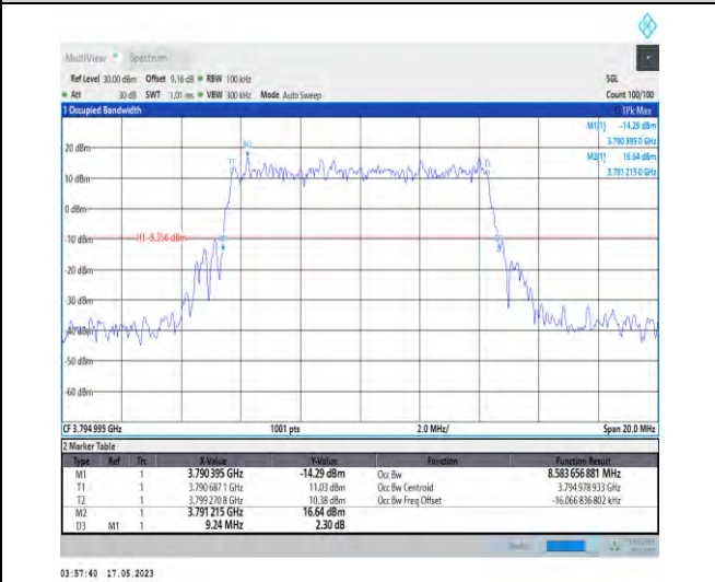
1-N78-3700-3800-PC1-30-10-H-2-DFT-PI2BPSK-Outer_Full-24@0-Ant1-8.584-9.240-≤10-PASS
