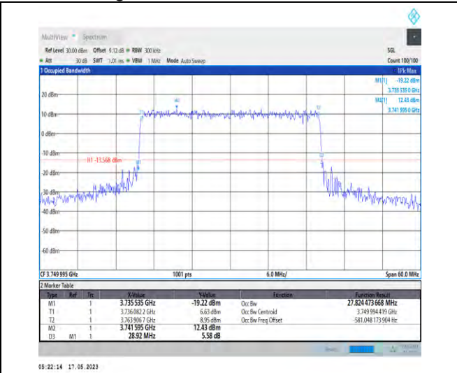
1-N78-3700-3800-PC1-30-30-M-8-CP-64QAM-Outer _Full-78@0-Ant1-27.824-28.920-≤30-PASS
