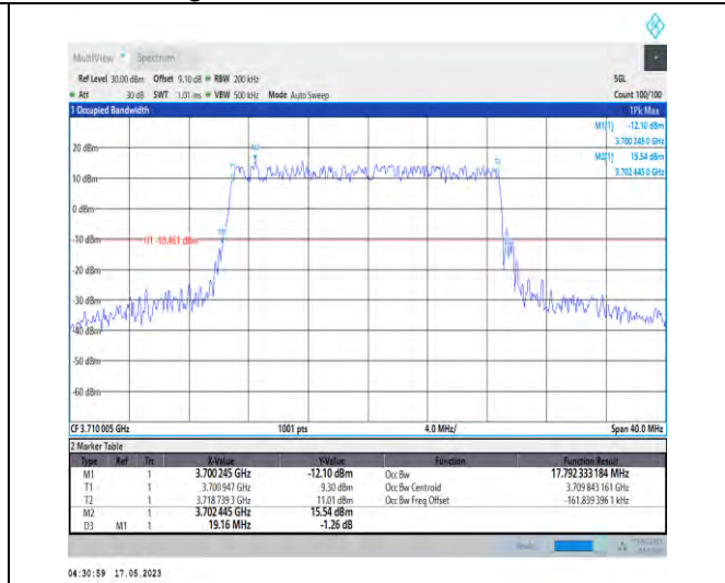
1-N78-3700-3800-PC1-30-20-L-4-DFT-64QAM-Outer_Full-50@0-Ant1-17.792-19.160-≤20-PASS
