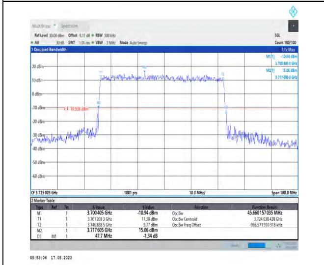
1-N78-3700-3800-PC1-30-50-L-4-DFT-64QAM-Out er_Full-128@0-Ant1-45.66-47.700-<math>\leq 50</math>-PASS
