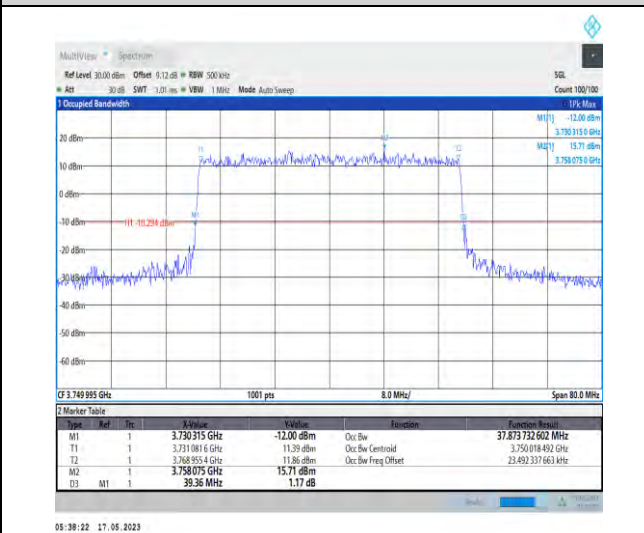
1-N78-3700-3800-PC1-30-40-M-7-CP-16QAM-Outer_Full-106@0-Ant1-37.874-39.360-≤40-PASS
