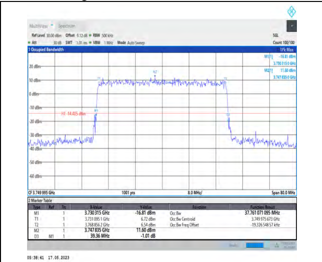
1-N78-3700-3800-PC1-30-40-M-9-CP-256QAM-Outer_Full-106@0-Ant1-37.761-39.360-≤40-PASS
