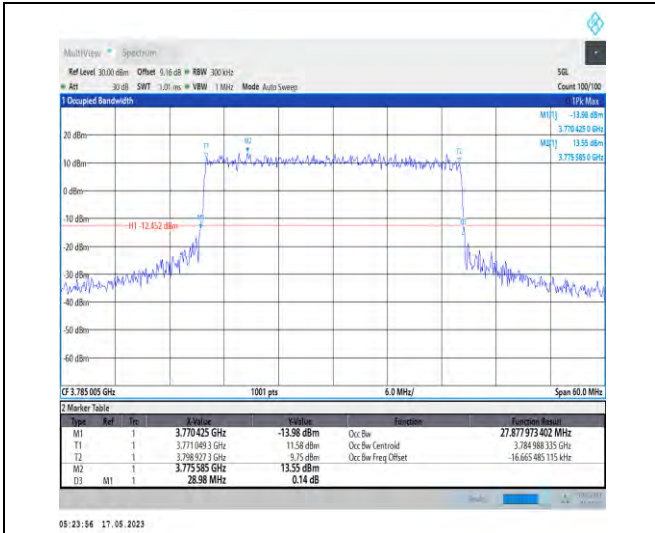
1-N78-3700-3800-PC1-30-30-H-6-CP-QPSK-Outer_Full-78@0-Ant1-27.878-28.980-≤30-PASS
