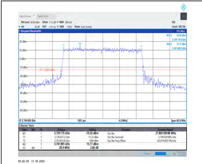
1-N78-3700-3800-PC1-30-30-M-7-CP-16QAM-Outer _Full-78@0-Ant1-27.806-29.400-≤30-PASS
