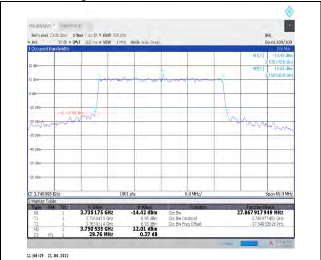
1-N78-3700-3800--30-30-M-8-CP-64QAM-Outer_Ful I-78@0-Ant1-27.868-29.760-<30-PASS
