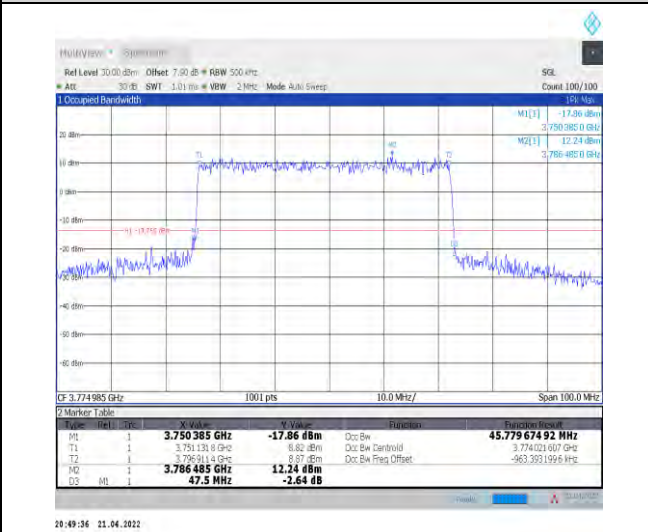
1-N78-3700-3800--30-50-H-3-DFT-16QAM-Outer_Full-128@0-Ant1-45.78-47.500-≤50-PASS
