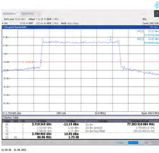
1-N78-3700-3800--30-80-H-1-DFT-QPSK-Outer_Full -216@0-Ant1-77.304-80.960-<math>\leq 80</math>-PASS
