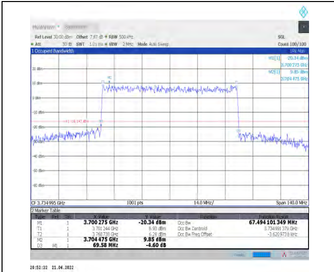
1-N78-3700-3800--30-70-L-8-CP-64QAM-Outer_Full -189@0-Ant1-67.494-69.580-≤70-PASS
