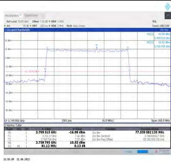
1-N78-3700-3800--30-80-M-9-CP-256QAM-Outer_Full -217@0-Ant1-77.54-81.120-<math>\leq 80</math>-PASS
