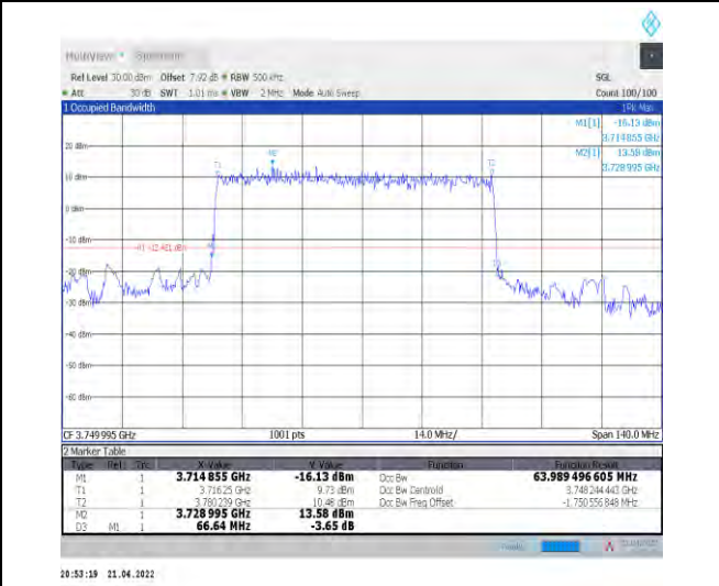
1-N78-3700-3800--30-70-M-2-DFT-PI2BPSK-Outer_Full Full-180@0-Ant1-63.989-66.640-≤70-PASS
