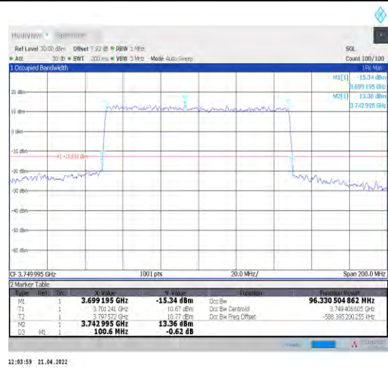
1-N78-3700-3800--30-100-L-4-DFT-64QAM-Outer_F ull-270@0-Ant1-96.331-100.600-≤100-PASS
