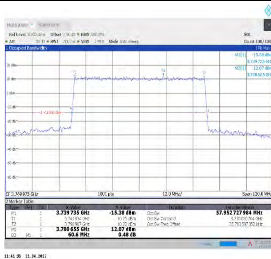
1-N78-3700-3800--30-60-H-4-DFT-64QAM-Outer_Fu ll-162@0-Ant1-57.953-60.600-≤60-PASS
