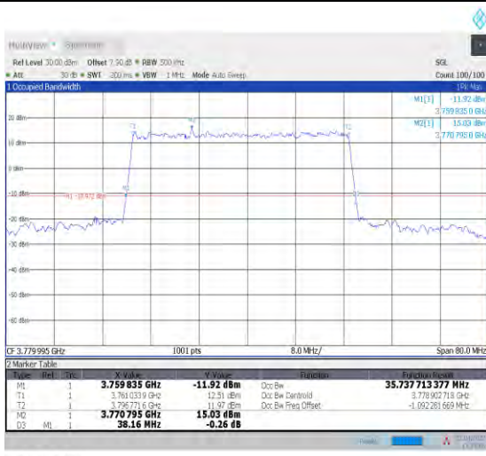
1-N78-3700-3800--30-40-H-3-DFT-16QAM-Outer_Fu II-100@0-Ant1-35.738-38.160-<math>\leq 40</math>-PASS
