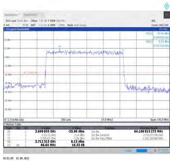
1-N78-3700-3800--30-70-L-5-DFT-256QAM-Outer_Full ull-180@0-Ant1-64.107-66.640-≤70-PASS
