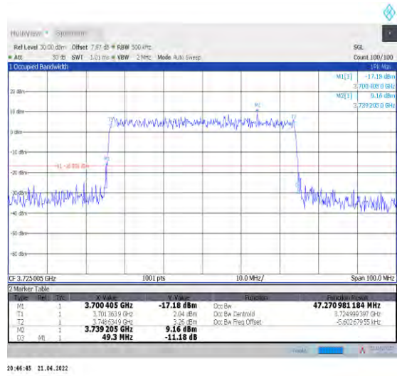
1-N78-3700-3800--30-50-L-9-CP-256QAM-Outer_Fu ll-133@0-Ant1-47.271-49.300-≤50-PASS
