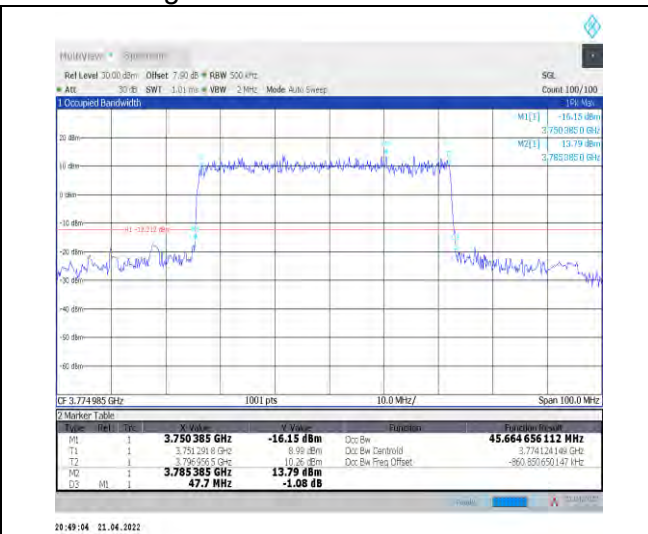
1-N78-3700-3800--30-50-H-1-DFT-QPSK-Outer_Full-128@0-Ant1-45.665-47.700-≤50-PASS
