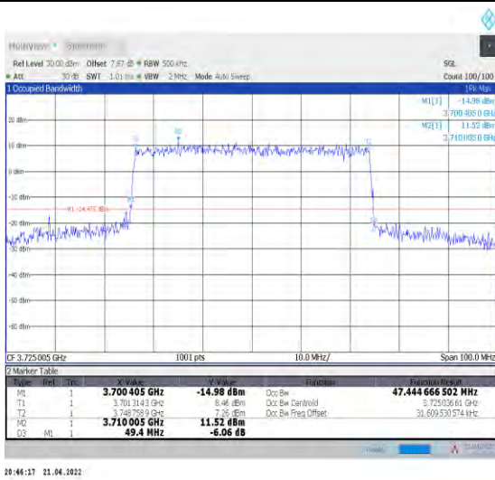
1-N78-3700-3800--30-50-L-6-CP-QPSK-Outer_Full-1 33@0-Ant1-47.445-49.400-≤50-PASS
