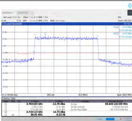
1-N78-3700-3800--30-90-M-1-DFT-QPSK-Outer_Full -240@0-Ant1-85.635-88.920-≤90-PASS
