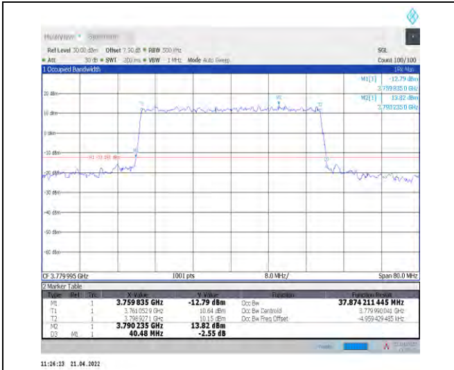
1-N78-3700-3800--30-40-H-7-CP-16QAM-Outer_Full -106@0-Ant1-37.874-40.480-≤40-PASS
