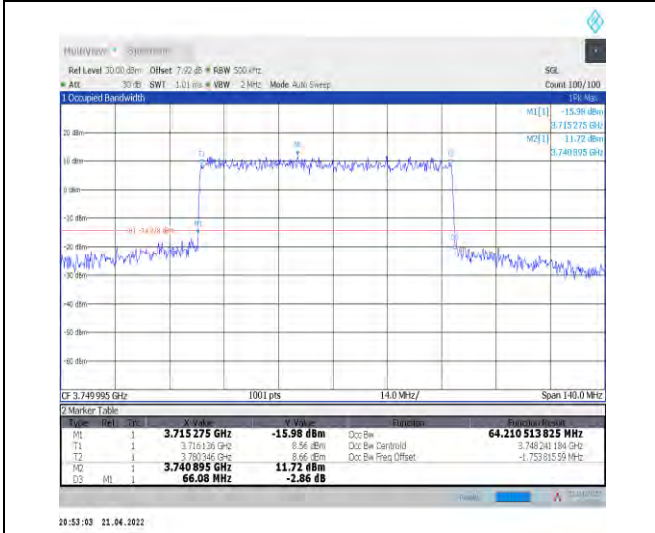
1-N78-3700-3800--30-70-M-1-DFT-QPSK-Outer_Full -180@0-Ant1-64.211-66.080-≤70-PASS
