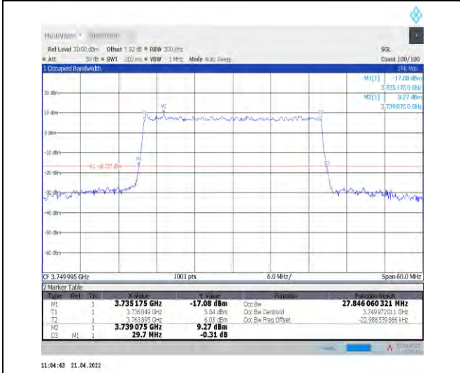
1-N78-3700-3800--30-30-M-9-CP-256QAM-Outer_F ull-78@0-Ant1-27.846-29.700-<30-PASS
