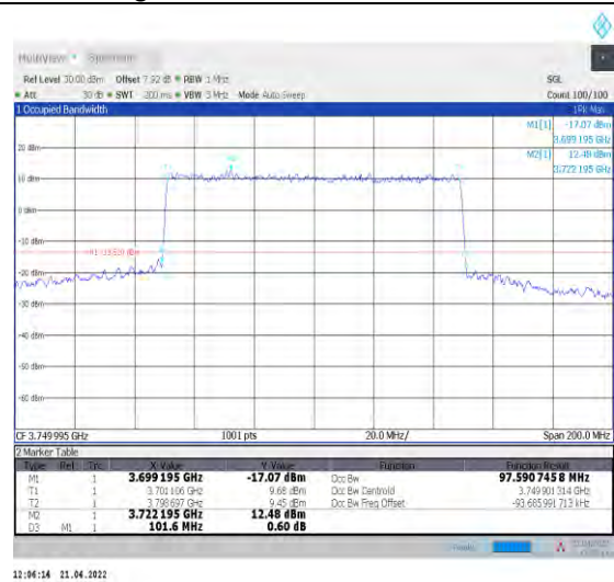
1-N78-3700-3800--30-100-L-8-CP-64QAM-Outer_Fu Il-273@0-Ant1-97.591-101.600-≤100-PASS
