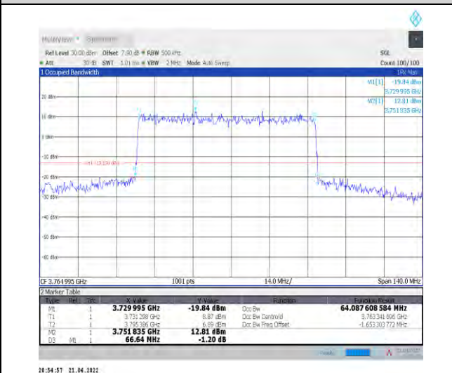
1-N78-3700-3800--30-70-H-1-DFT-QPSK-Outer_Full -180@0-Ant1-64.088-66.640-≤70-PASS
