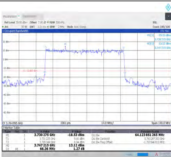
1-N78-3700-3800--30-70-H-2-DFT-PI2BPSK-Outer_Full-180@0-Ant1-64.124-66.360-≤70-PASS
