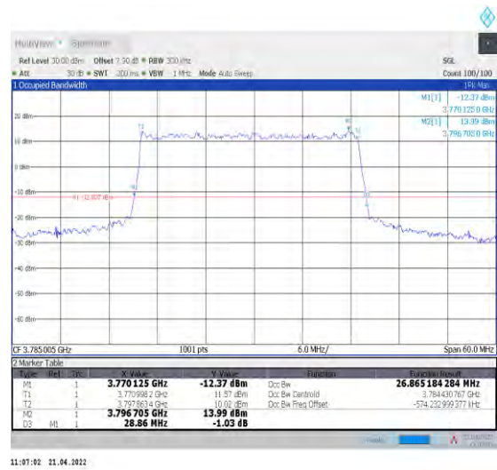
1-N78-3700-3800--30-30-H-3-DFT-16QAM-Outer_Fu II-75@0-Ant1-26.865-28.860-<math>\leq</math>30-PASS
