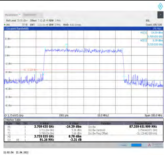
1-N78-3700-3800--30-90-H-9-CP-256QAM-Outer_Full-245@0-Ant1-87.359-91.260-<math>\leq 90</math>-PASS
