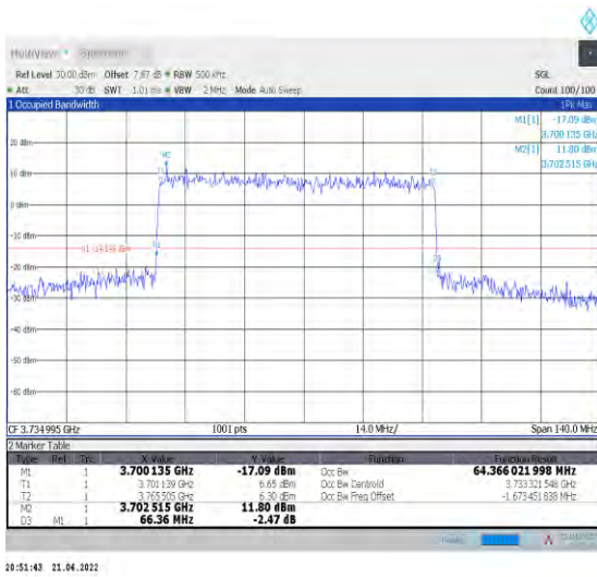
1-N78-3700-3800--30-70-L-4-DFT-64QAM-Outer_Full I-180@0-Ant1-64.366-66.360-≤70-PASS
