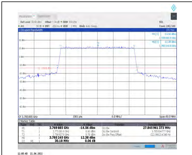
1-N78-3700-3800--30-30-H-6-CP-QPSK-Outer_Full-78@0-Ant1-27.846-30.180-≤30-PASS
