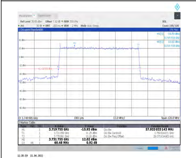
1-N78-3700-3800--30-60-M-4-DFT-64QAM-Outer_Full-162@0-Ant1-57.933-60.480-≤60-PASS
