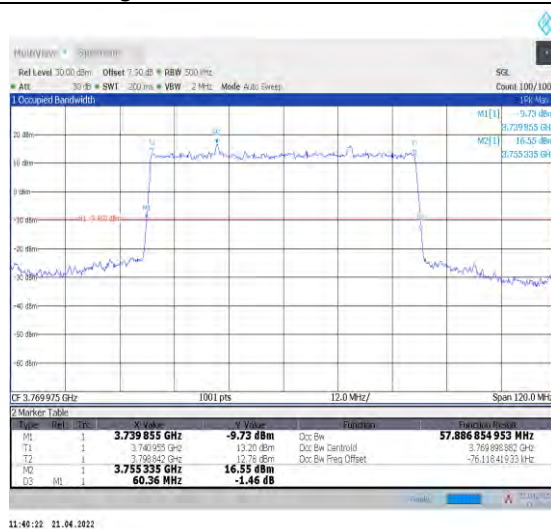
1-N78-3700-3800--30-60-H-2-DFT-PI2BPSK-Outer_Full Full-162@0-Ant1-57.887-60.360-≤60-PASS
