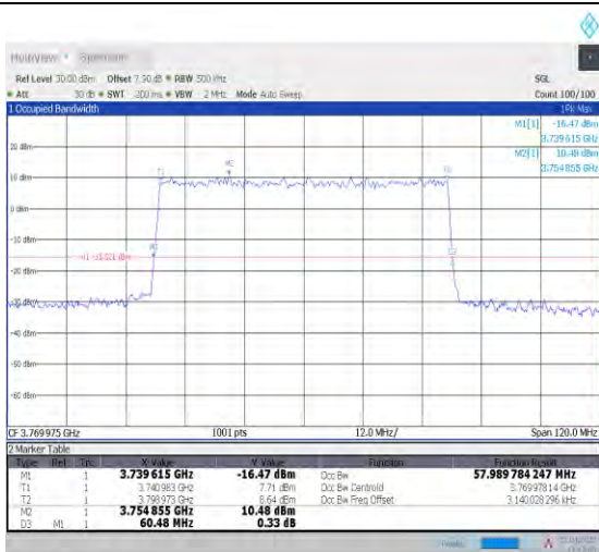
1-N78-3700-3800--30-60-H-5-DFT-256QAM-Outer_Full-162@0-Ant1-57.99-60.480-≤60-PASS
