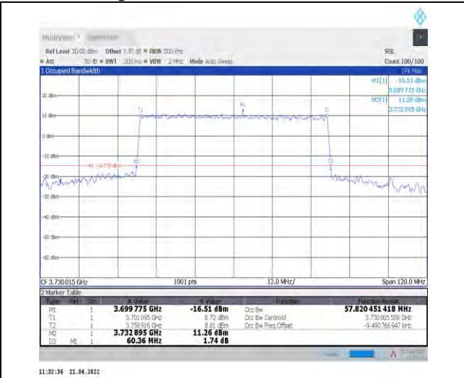
1-N78-3700-3800--30-60-L-8-CP-64QAM-Outer_Full -162@0-Ant1-57.82-60.360-≤60-PASS
