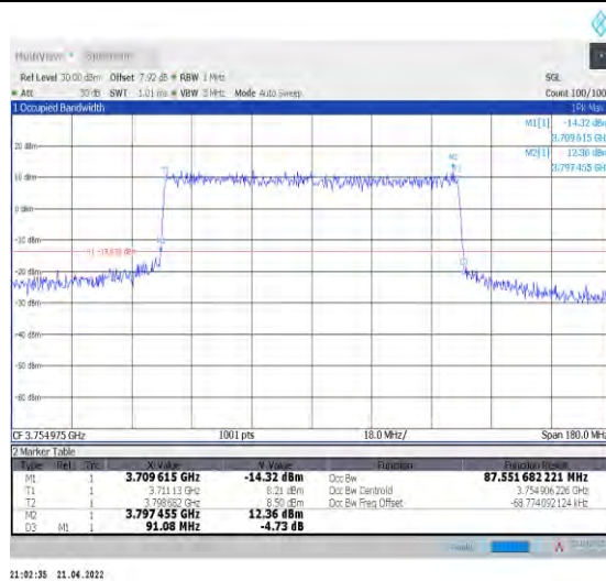
1-N78-3700-3800--30-90-H-7-CP-16QAM-Outer_Full-245@0-Ant1-87.552-91.080-≤90-PASS
