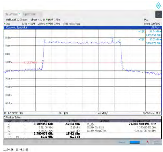
1-N78-3700-3800--30-80-M-1-DFT-QPSK-Outer_Full-216@0-Ant1-77.304-80.800-≤80-PASS
