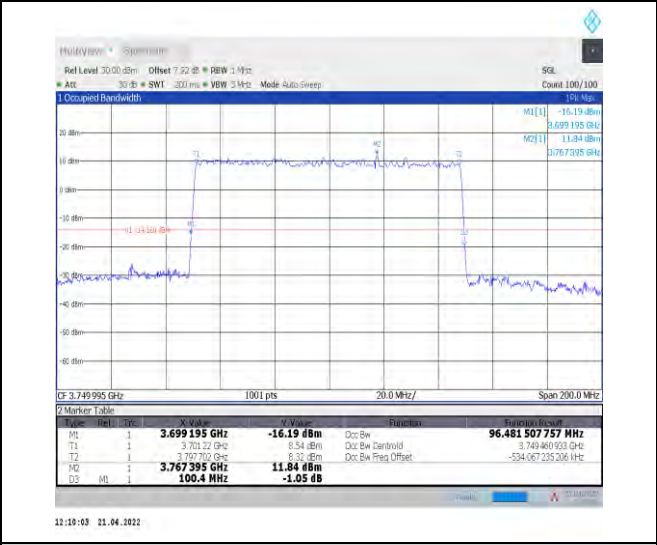
1-N78-3700-3800--30-100-M-5-DFT-256QAM-Outer_Full-270@0-Ant1-96.482-100.400-≤100-PASS
