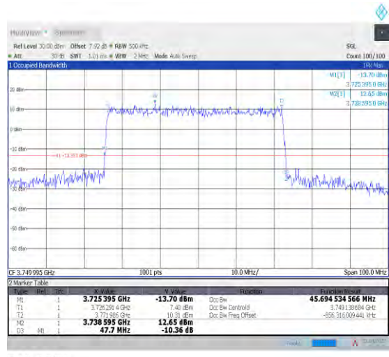
1-N78-3700-3800--30-50-M-4-DFT-64QAM-Outer_Full ull-128@0-Ant1-45.695-47.700-≤50-PASS
