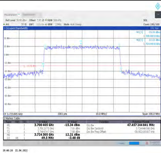
1-N78-3700-3800--30-50-L-7-CP-16QAM-Outer_Full -133@0-Ant1-47.457-49.500-≤50-PASS
