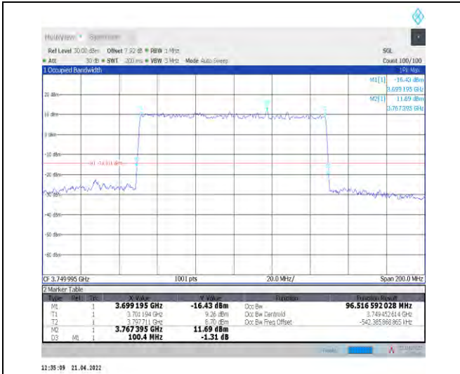
1-N78-3700-3800--30-100-H-5-DFT-256QAM-Outer_Full-270@0-Ant1-96.517-100.400-≤100-PASS
