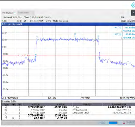
1-N78-3700-3800--30-50-M-1-DFT-QPSK-Outer_Full -128@0-Ant1-45.766-47.600-≤50-PASS
