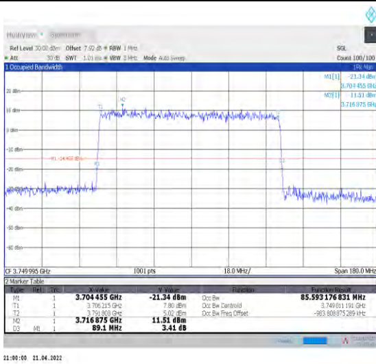
1-N78-3700-3800--30-90-M-5-DFT-256QAM-Outer_Full-240@0-Ant1-85.593-89.100-<math>\leq 90</math>-PASS
