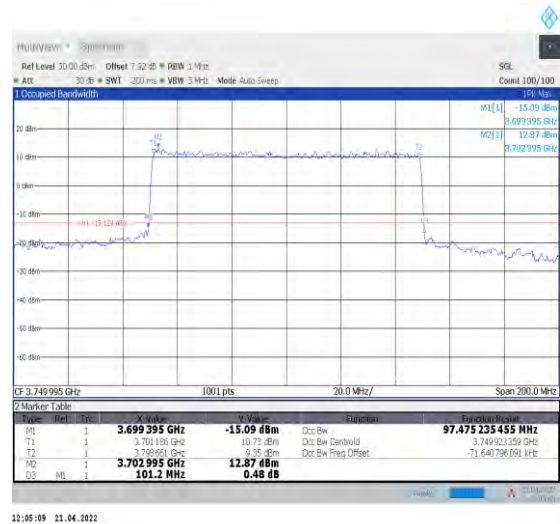
1-N78-3700-3800--30-100-L-6-CP-QPSK-Outer_F ull-273@0-Ant1-97.475-101.200-≤100-PASS
