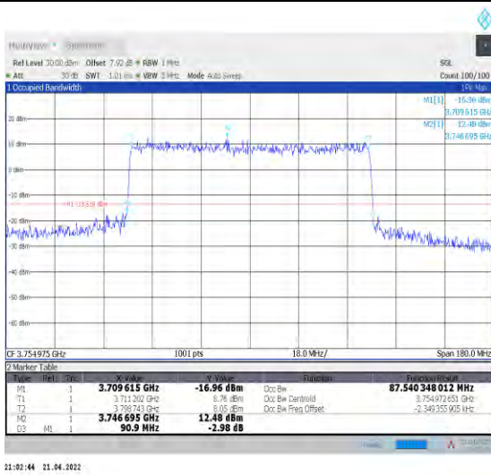
1-N78-3700-3800--30-90-H-8-CP-64QAM-Outer_Full -245@0-Ant1-87.54-90.900-<math>\leq 90</math>-PASS
