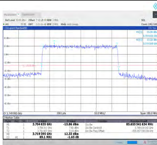
1-N78-3700-3800--30-90-M-2-DFT-PI2BPSK-Outer_Full Full-240@0-Ant1-85.644-89.100-≤90-PASS
