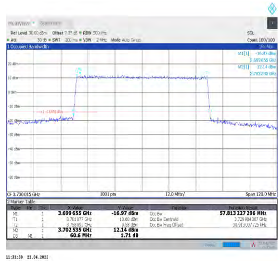
1-N78-3700-3800--30-60-L-6-CP-QPSK-Outer_Full- 162@0-Ant1-57.813-60.600-≤60-PASS
