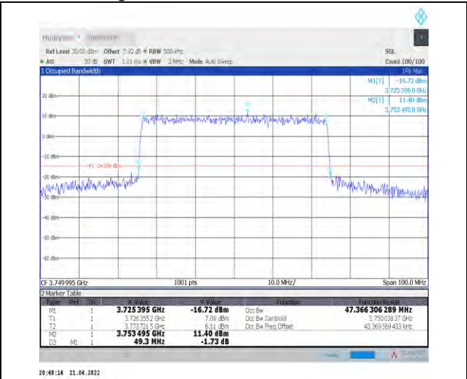
1-N78-3700-3800--30-50-M-6-CP-QPSK-Outer_Full-133@0-Ant1-47.366-49.300-<math>\leq 50</math>-PASS
