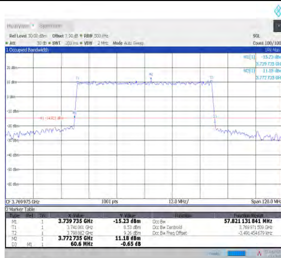
1-N78-3700-3800--30-60-H-6-CP-QPSK-Outer_Full-162@0-Ant1-57.832-60.600-≤60-PASS
