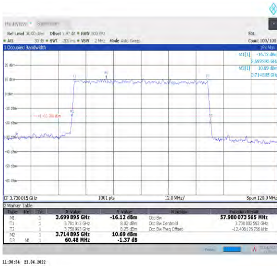
1-N78-3700-3800--30-60-L-5-DFT-256QAM-Outer_F ull-162@0-Ant1-57.98-60.480-≤60-PASS
