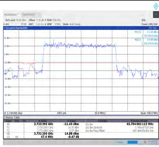
1-N78-3700-3800--30-50-M-2-DFT-PI2BPSK-Outer_Full Full-128@0-Ant1-45.704-47.400-≤50-PASS
