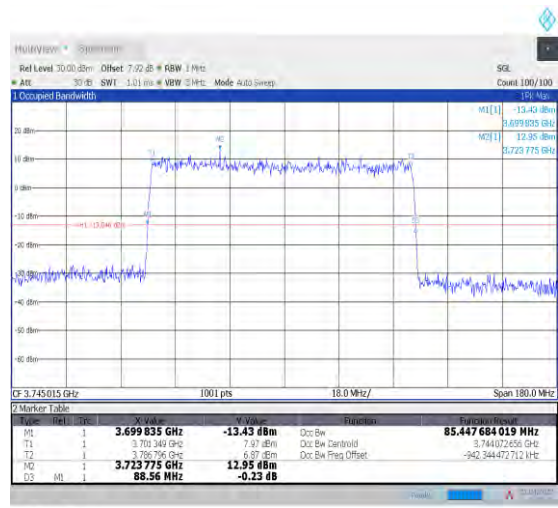
1-N78-3700-3800--30-90-L-3-DFT-16QAM-Outer_Full-240@0-Ant1-85.615-88.740-≤90-PASS
