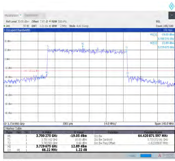
1-N78-3700-3800--30-70-L-1-DFT-QPSK-Outer_Full-180@0-Ant1-64.421-66.220-≤70-PASS
