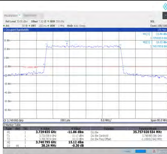
1-N78-3700-3800--30-40-M-1-DFT-QPSK-Outer_Full -100@0-Ant1-35.766-38.240-≤40-PASS
