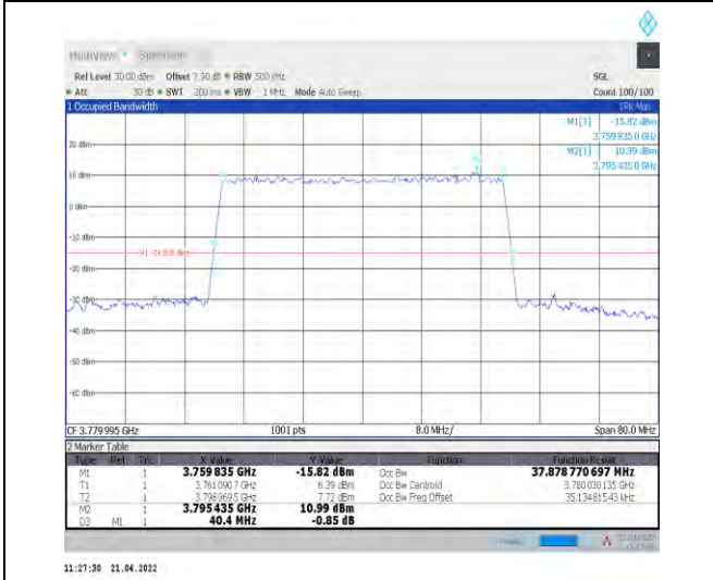
1-N78-3700-3800--30-40-H-9-CP-256QAM-Outer_Fu II-106@0-Ant1-37.879-40.400-≤40-PASS
