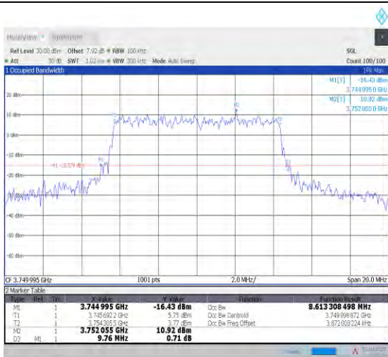
1-N78-3700-3800--30-10-M-8-CP-64QAM-Outer_Full -24@0-Ant1-8.613-9.760-≤10-PASS
