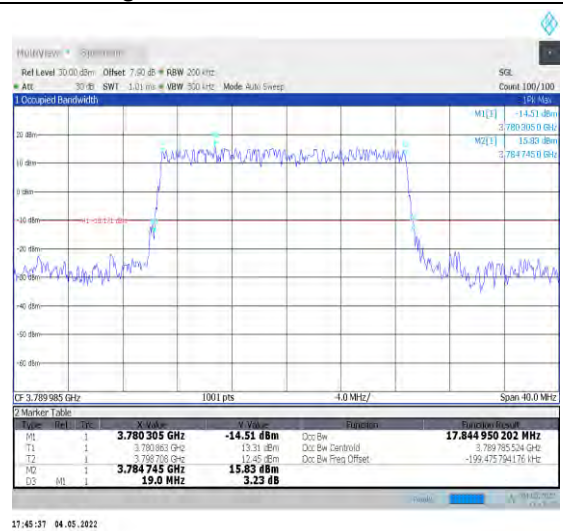
1-N78-3700-3800--30-20-H-2-DFT-PI2BPSK-Outer_Full Full-50@0-Ant1-17.845-19.000-≤20-PASS
