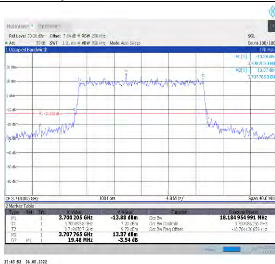
1-N78-3700-3800--30-20-L-8-CP-64QAM-Outer_Full -51@0-Ant1-18.185-19.480-≤20-PASS
