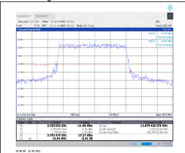
1-N78-3700-3800--30-15-H-1-DFT-QPSK-Outer_Full-36@0-Ant1-12.879-14.040-≤15-PASS
