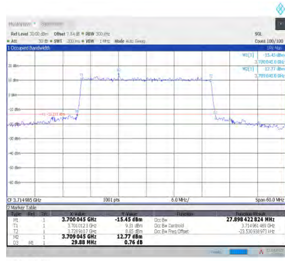
1-N78-3700-3800--30-30-L-7-CP-16QAM-Outer_Full-78@0-Ant1-27.898-29.880-<math>\leq</math>30-PASS
