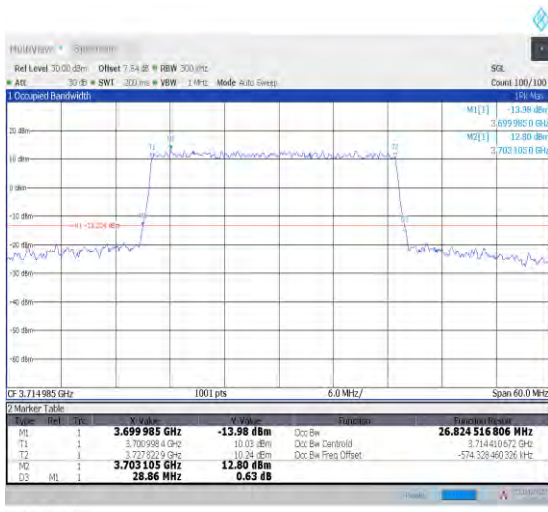
1-N78-3700-3800--30-30-L-4-DFT-64QAM-Outer_Full-75@0-Ant1-26.825-28.860-<math>\leq</math>30-PASS
