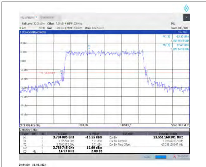
1-N78-3700-3800--30-15-H-8-CP-64QAM-Outer_Full -38@0-Ant1-13.551-14.970-≤15-PASS
