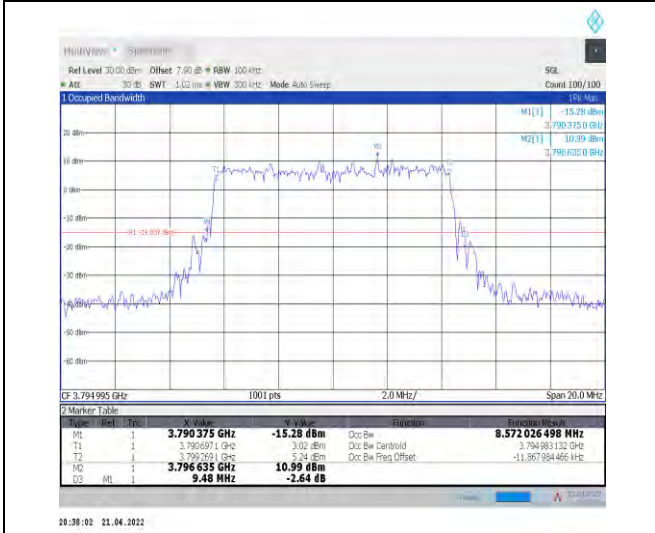
1-N78-3700-3800--30-10-H-5-DFT-256QAM-Outer_Full-24@0-Ant1-8.572-9.480-≤10-PASS
