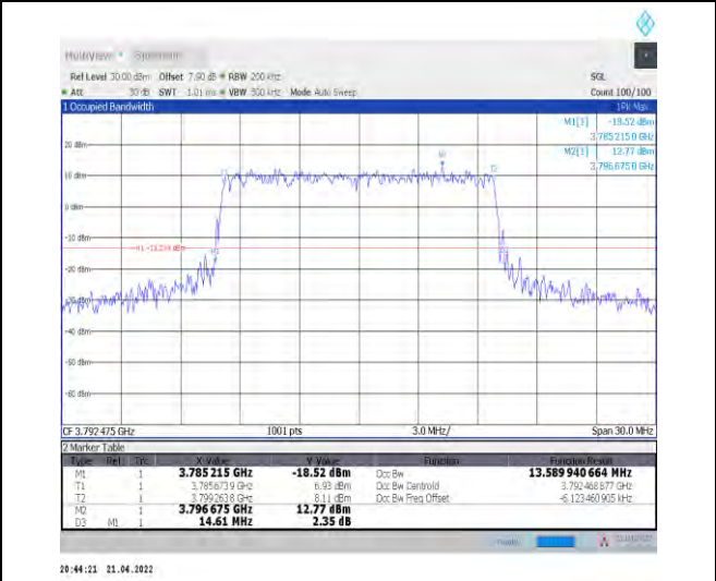
1-N78-3700-3800--30-15-H-7-CP-16QAM-Outer_Full-38@0-Ant1-13.59-14.610-≤15-PASS
