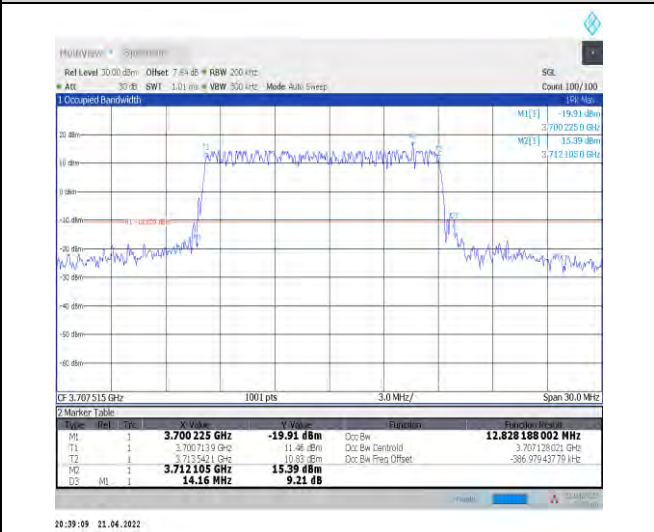
1-N78-3700-3800--30-15-L-1-DFT-QPSK-Outer_Full- 36@0-Ant1-12.828-14.160-≤15-PASS
