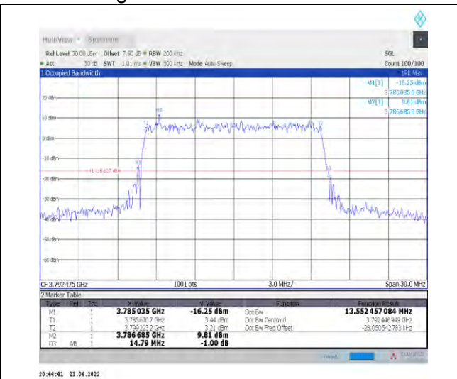
1-N78-3700-3800--30-15-H-9-CP-256QAM-Outer_Full -38@0-Ant1-13.552-14.790-≤15-PASS
