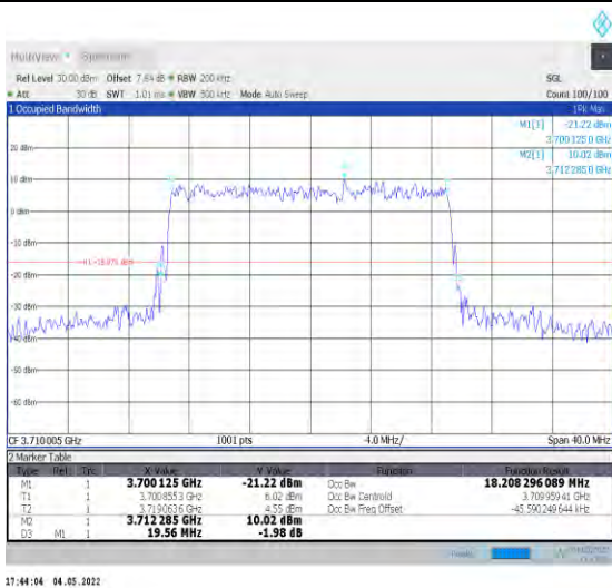
1-N78-3700-3800--30-20-L-9-CP-256QAM-Outer_Fu II-51@0-Ant1-18.208-19.560-≤20-PASS
