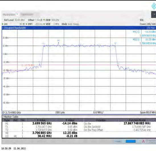
1-N78-3700-3800--30-30-L-8-CP-64QAM-Outer_Full -78@0-Ant1-27.868-30.420-<30-PASS
