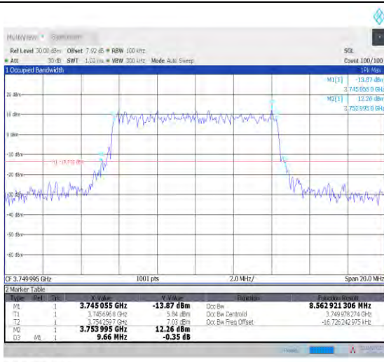
1-N78-3700-3800--30-10-M-4-DFT-64QAM-Outer_Full-24@0-Ant1-8.563-9.660-≤10-PASS
