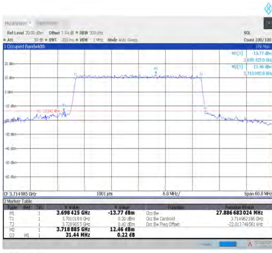
1-N78-3700-3800--30-30-L-6-CP-QPSK-Outer_Full-78@0-Ant1-27.887-31.440-<math>\leq</math>30-PASS
