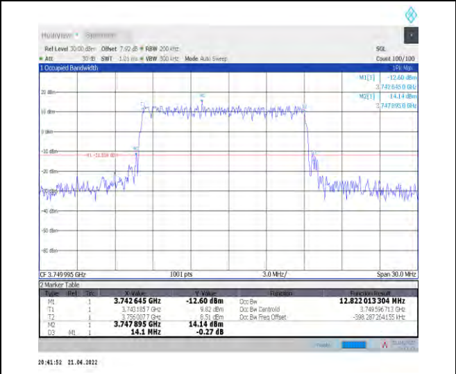
1-N78-3700-3800--30-15-M-4-DFT-64QAM-Outer_Full Full-36@0-Ant1-12.822-14.100-≤15-PASS
