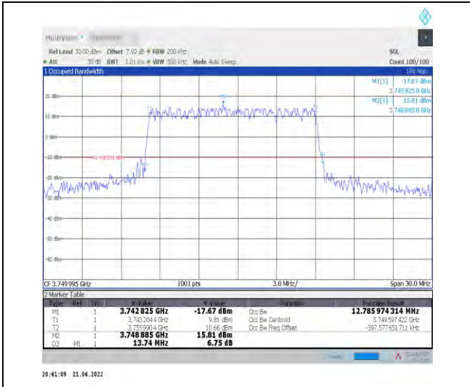
1-N78-3700-3800--30-15-M-1-DFT-QPSK-Outer_Full -36@0-Ant1-12.786-13.740-≤15-PASS
