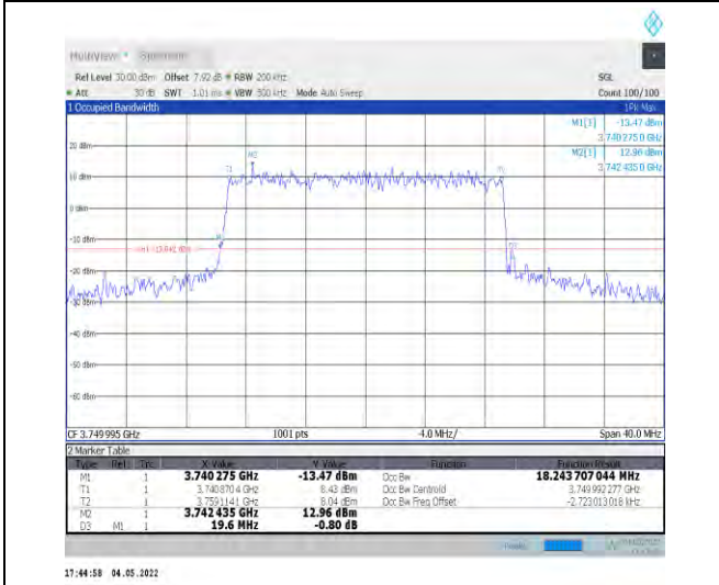
1-N78-3700-3800--30-20-M-8-CP-64QAM-Outer_Full-51@0-Ant1-18.244-19.600-<math>\leq 20</math>-PASS
