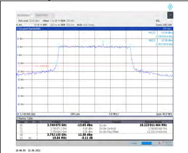
1-N78-3700-3800--30-20-M-7-CP-16QAM-Outer_Full-51@0-Ant1-18.223-19.840-<math>\leq 20</math>-PASS
