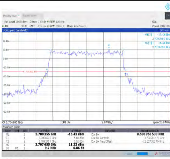
1-N78-3700-3800--30-10-L-5-DFT-256QAM-Outer_Full-24@0-Ant1-8.581-9.200-<=10-PASS
