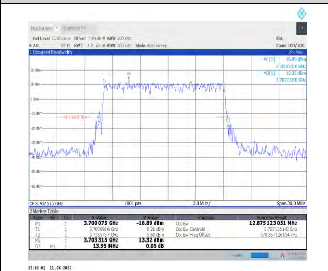
1-N78-3700-3800--30-15-L-5-DFT-256QAM-Outer_Full-36@0-Ant1-12.875-13.950-≤15-PASS
