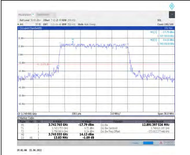
1-N78-3700-3800--30-15-M-3-DFT-16QAM-Outer_Full Full-36@0-Ant1-12.891-13.830-≤15-PASS
