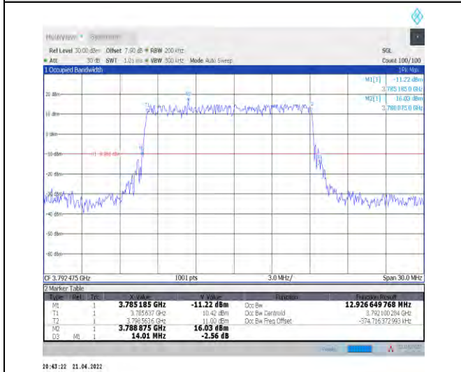
1-N78-3700-3800--30-15-H-2-DFT-PI2BPSK-Outer_Full-36@0-Ant1-12.927-14.010-≤15-PASS
