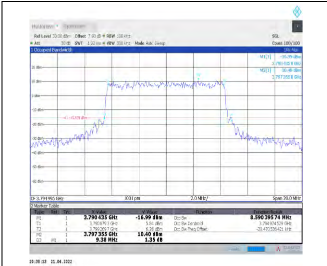
1-N78-3700-3800--30-10-H-7-CP-16QAM-Outer_Full -24@0-Ant1-8.59-9.380-≤10-PASS
