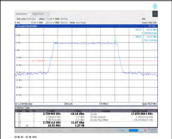
1-N78-3700-3800--30-20-M-5-DFT-256QAM-Outer_Full-50@0-Ant1-17.871-19.520-≤20-PASS
