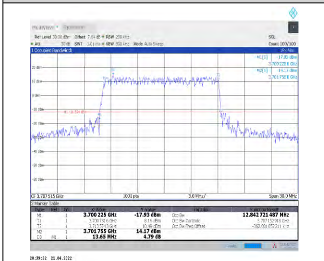
1-N78-3700-3800--30-15-L-4-DFT-64QAM-Outer_Full-36@0-Ant1-12.843-13.650-≤15-PASS
