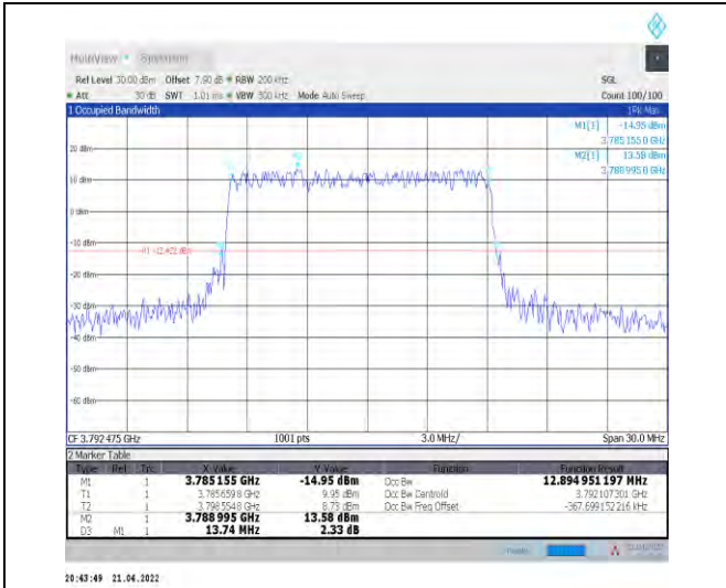
1-N78-3700-3800--30-15-H-4-DFT-64QAM-Outer_Fu II-36@0-Ant1-12.895-13.740-≤15-PASS
