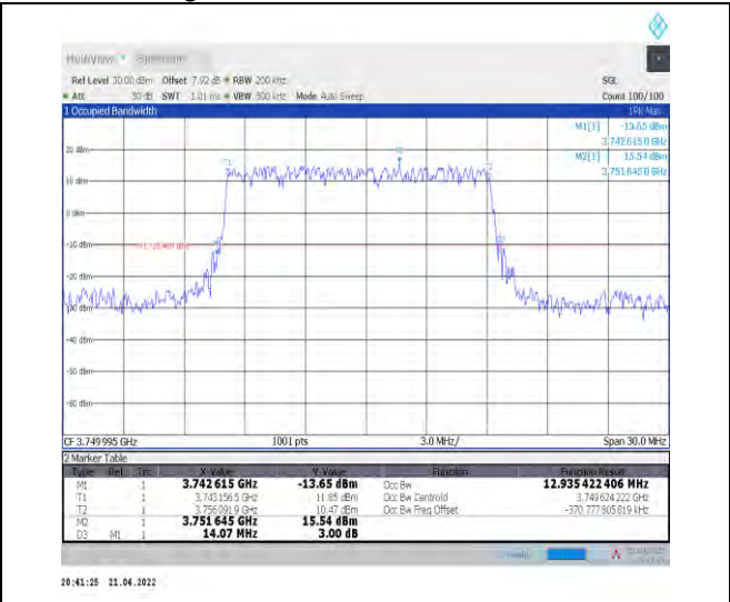
1-N78-3700-3800--30-15-M-2-DFT-PI2BPSK-Outer_Full Full-36@0-Ant1-12.935-14.070-≤15-PASS
