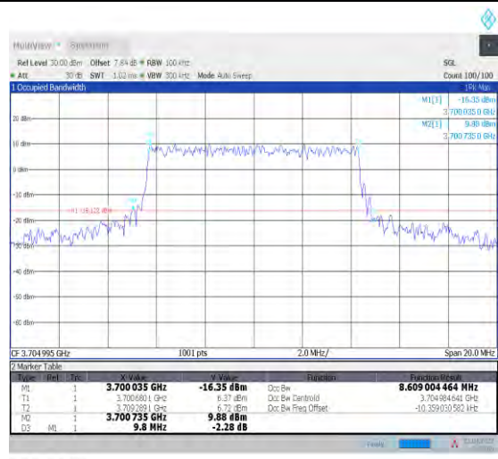
1-N78-3700-3800--30-10-L-6-CP-QPSK-Outer_Full-24@0-Ant1-8.609-9.800-<=10-PASS
