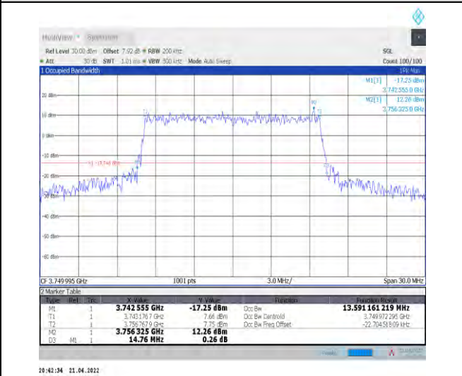
1-N78-3700-3800--30-15-M-8-CP-64QAM-Outer_Full-38@0-Ant1-13.591-14.760-≤15-PASS
