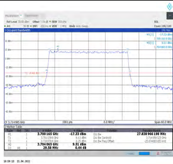
1-N78-3700-3800--30-30-L-9-CP-256QAM-Outer_Fu II-78@0-Ant1-27.839-29.580-<30-PASS
