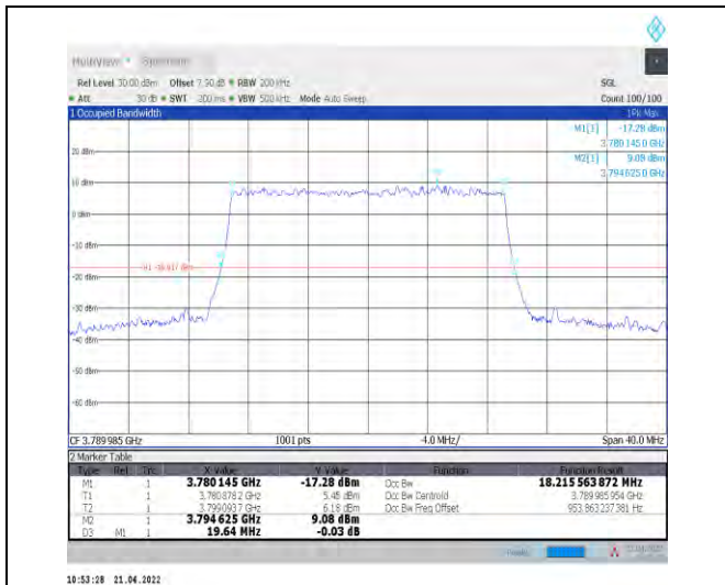
1-N78-3700-3800--30-20-H-9-CP-256QAM-Outer_Fu II-51@0-Ant1-18.216-19.640-≤20-PASS
