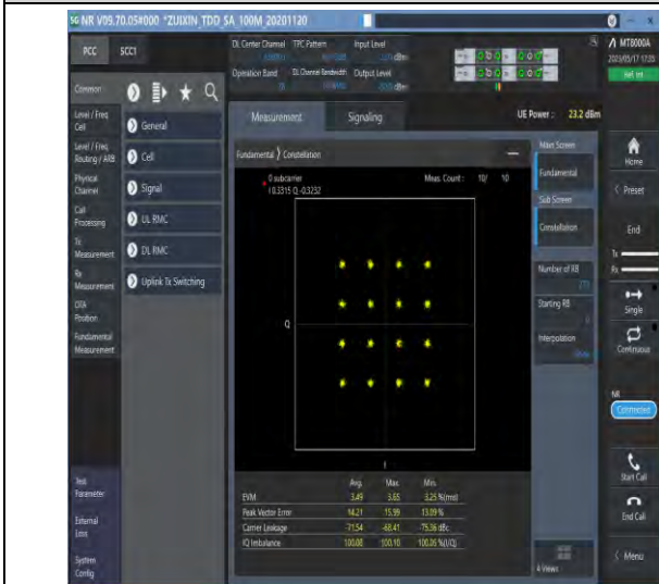
1-N78-3700-3800-PC1-30-100-M-7-CP-16QAM-Outer_Full-273@0-Ant1-see graph-PASS
