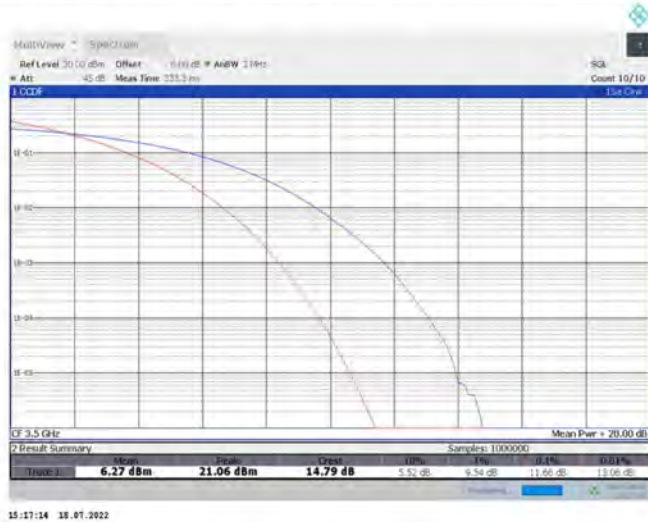
42-42-20MHz-20MHz-QPSK-QPSK-42491-42689-100RB#0-100RB#0
