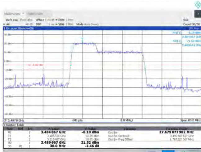
42-42-10MHz-20MHz-QPSK-QPSK-42496-42640-50RB#0-100RB#0
