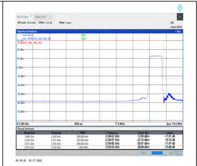
1-N78-3450-3550-PC1-30-15-H-3-DFT-PI2BPSK-Outer_Full-36@0-Ant1-1--PASS-see graph
