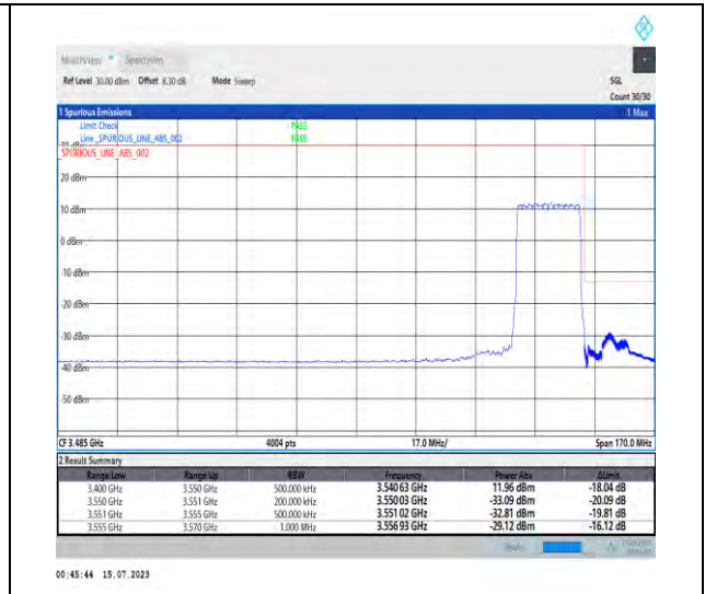
1-N78-3450-3550-PC1-30-20-H-3-DFT-PI2BPSK-Outer_Full-50@0-Ant1-1--PASS-see graph
