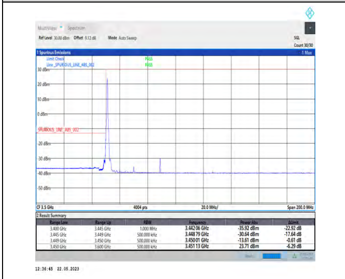
1-N78-3450-3550-PC1-30-40-L-4-CP-QPSK-Edge_1RB_Left-1@0-Ant1-1--PASS-see graph
