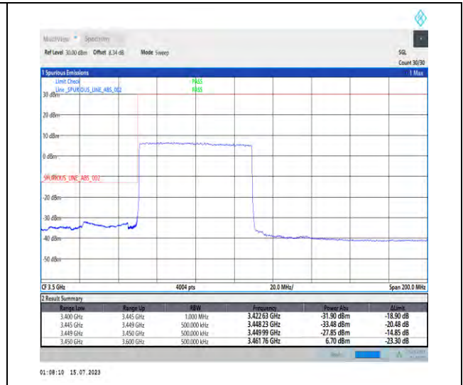
1-N78-3450-3550-PC1-30-60-L-3-DFT-PI2BPSK-Outer_Full-162@0-Ant1-1--PASS-see graph
