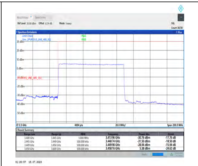
1-N78-3450-3550-PC1-30-80-L-3-DFT-PI2BPSK-Outer_Full-216@0-Ant1-1--PASS-see graph
