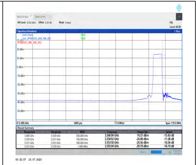
1-N78-3450-3550-PC1-30-10-H-3-DFT-PI2BPSK-Outer_Full-24@0-Ant1-1--PASS-see graph
