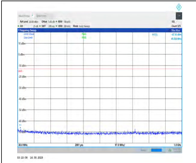
1-N78-3450-3550-PC1-30-100-M-1-DFT-PI2BPSK- Inner_1RB_Left-1@1-30-1000-Ant1-45.52--67.10--1- 3-PASS
