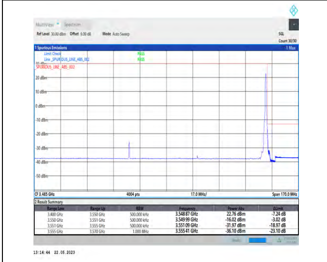
1-N78-3450-3550-PC1-30-90-H-5-CP-QPSK-Edge_1RB_Right-1@244-Ant1-1--PASS-see graph
