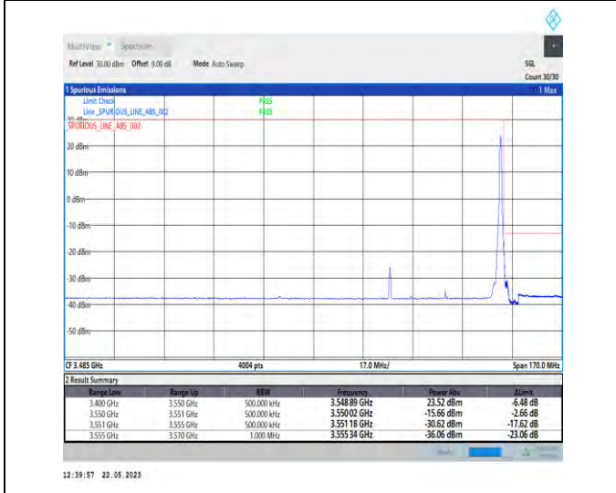
1-N78-3450-3550-PC1-30-40-H-5-CP-QPSK-Edge_1RB_Right-1@105-Ant1-1--PASS-see graph
