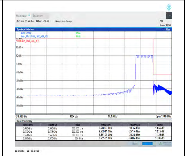
1-N78-3450-3550-PC1-30-20-H-6-CP-QPSK-Outer_Full-51@0-Ant1-1--PASS-see graph
