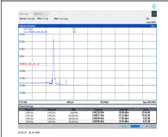
1-N78-3450-3550-PC1-30-20-L-4-CP-QPSK-Edge_1_RB_Left-1@0-Ant1-1--PASS-see graph
