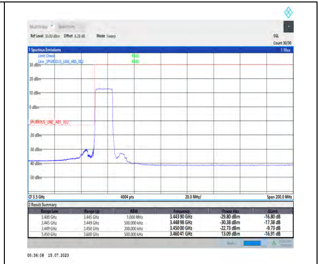
1-N78-3450-3550-PC1-30-15-L-3-DFT-PI2BPSK-Outer_Full-36@0-Ant1-1--PASS-see graph
