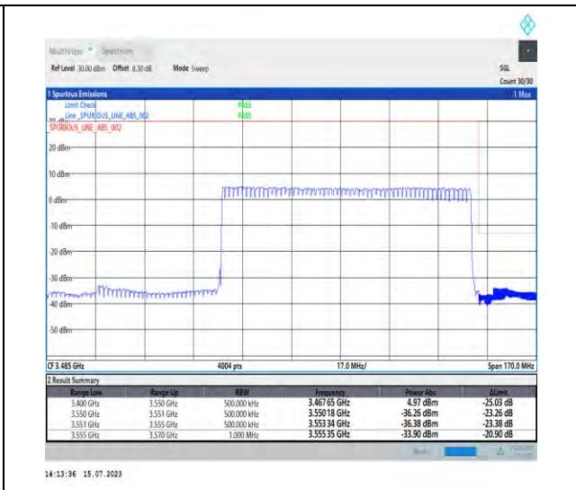
1-N78-3450-3550-PC1-30-90-H-3-DFT-PI2BPSK-Outer_Full-240@0-Ant1-1--PASS-see graph
