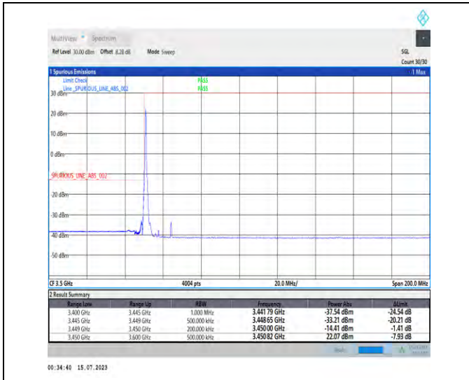
1-N78-3450-3550-PC1-30-15-L-1-DFT-PI2BPSK-Edge_1_RB_Left-1@0-Ant1-1--PASS-see graph
