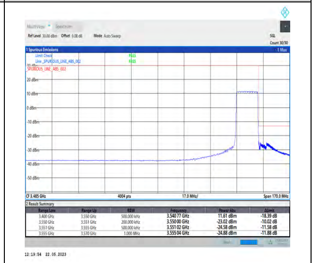
1-N78-3450-3550-PC1-30-15-H-6-CP-QPSK-Outer_Full-38@0-Ant1-1--PASS-see graph
