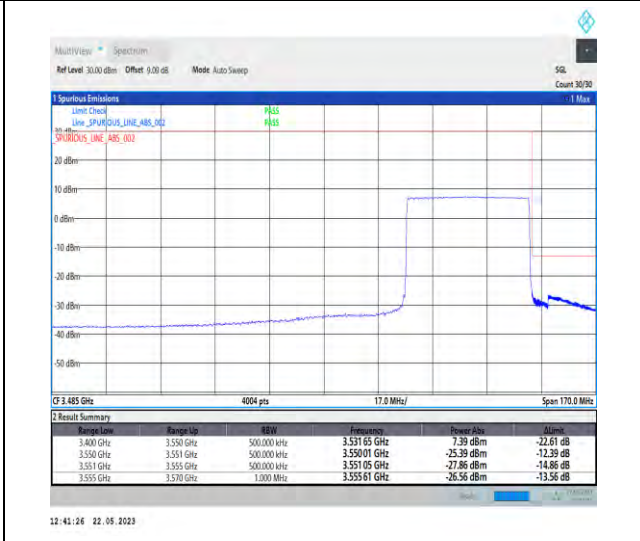
1-N78-3450-3550-PC1-30-40-H-6-CP-QPSK-Outer_Full-106@0-Ant1-1--PASS-see graph
