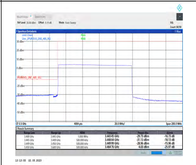
1-N78-3450-3550-PC1-30-90-L-6-CP-QPSK-Outer_Full-245@0-Ant1-1--PASS-see graph
