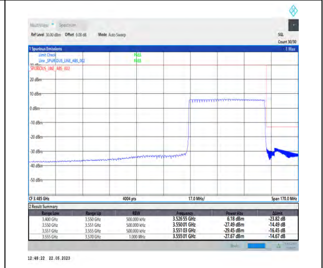
1-N78-3450-3550-PC1-30-50-H-6-CP-QPSK-Outer_Full-133@0-Ant1-1--PASS-see graph
