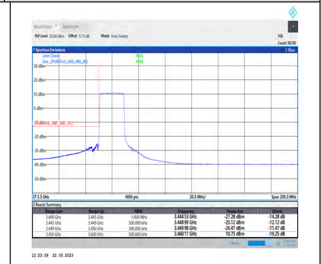
1-N78-3450-3550-PC1-30-20-L-6-CP-QPSK-Outer_Full-51@0-Ant1-1--PASS-see graph
