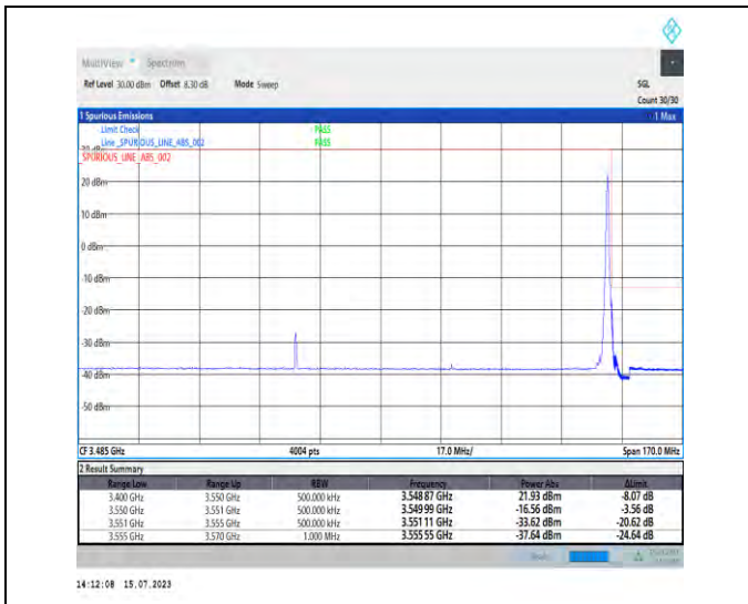
1-N78-3450-3550-PC1-30-90-H-2-DFT-PI2BPSK-Edge_1RB_Right-1@244-Ant1-1--PASS-see graph
