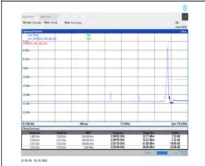
1-N78-3450-3550-PC1-30-60-H-5-CP-QPSK-Edge_1RB_Right-1@161-Ant1-1--PASS-see graph
