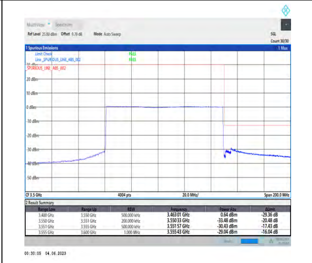
1-N78-3450-3550-PC1-30-90-H-6-CP-QPSK-Outer_Full-245@0-Ant1-1--PASS-see graph
