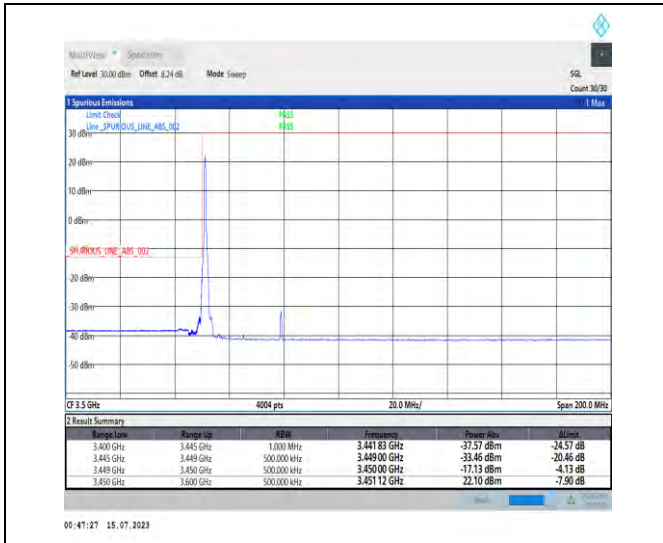
1-N78-3450-3550-PC1-30-30-L-1-DFT-PI2BPSK-Edge_e_1RB_Left-1@0-Ant1-1--PASS-see graph
