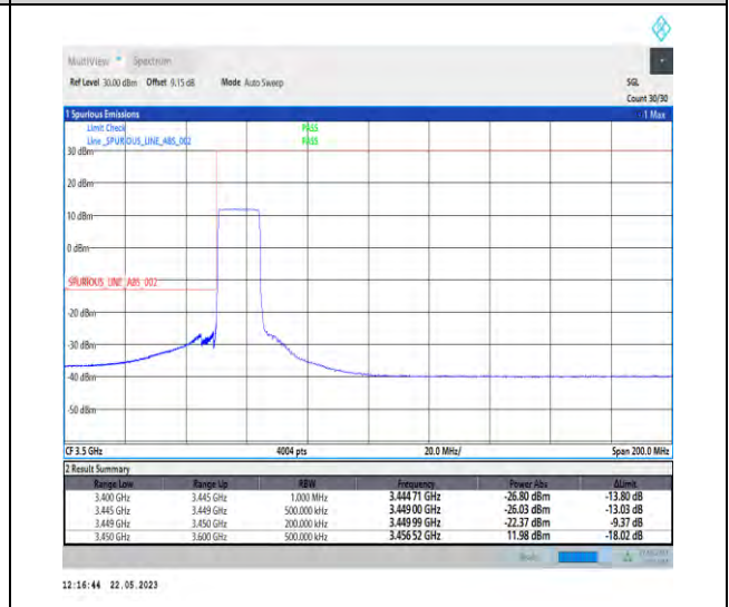
1-N78-3450-3550-PC1-30-15-L-6-CP-QPSK-Outer_Full-38@0-Ant1-1--PASS-see graph
