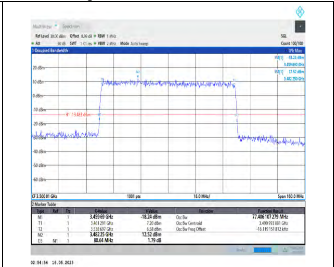
1-N78-3450-3550-PC1-30-80-M-9-CP-256QAM-Outer_Full-217@0-Ant1-77.406-80.640-≤80-PASS
