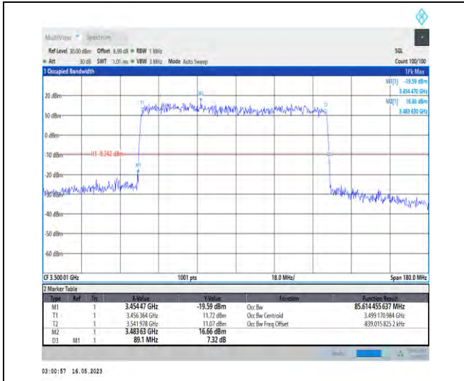
1-N78-3450-3550-PC1-30-90-M-1-DFT-QPSK-Outer_Full-240@0-Ant1-85.614-89.100-≤90-PASS
