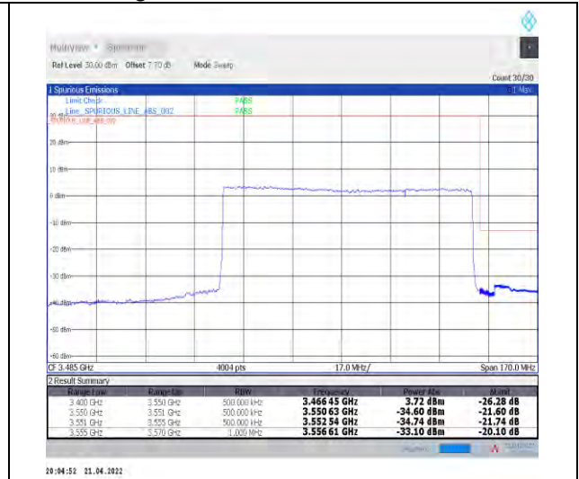
1-N78-3450-3550--30-90-H-3-DFT-PI2BPSK-Outer_Full-240@0-Ant1-PASS-see graph
