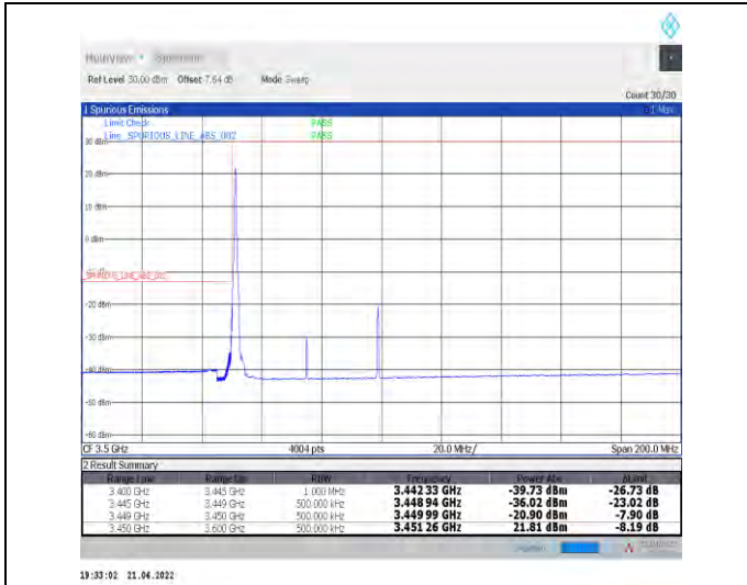
1-N78-3450-3550--30-50-L-1-DFT-PI2BPSK-Edge_1R_B_Left-1@0-Ant1-PASS-see graph
