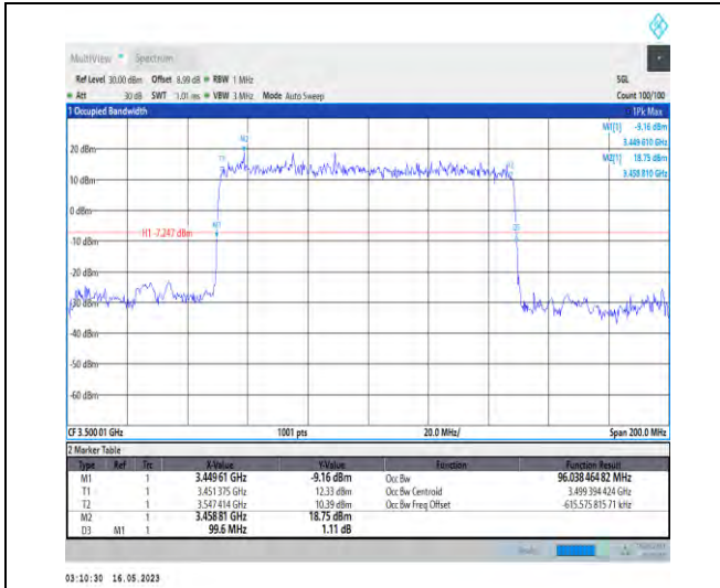
1-N78-3450-3550-PC1-30-100-M-2-DFT-PI2BPSK-Outer_Full-270@0-Ant1-96.038-99.600-≤100-PASS
