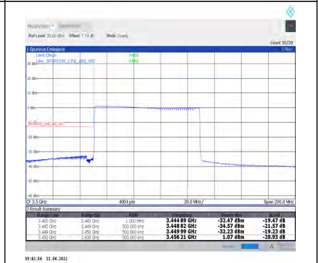
1-N78-3450-3550--30-80-L-6-CP-QPSK-Outer_Ful_I-217@0-Ant1-PASS-see graph
