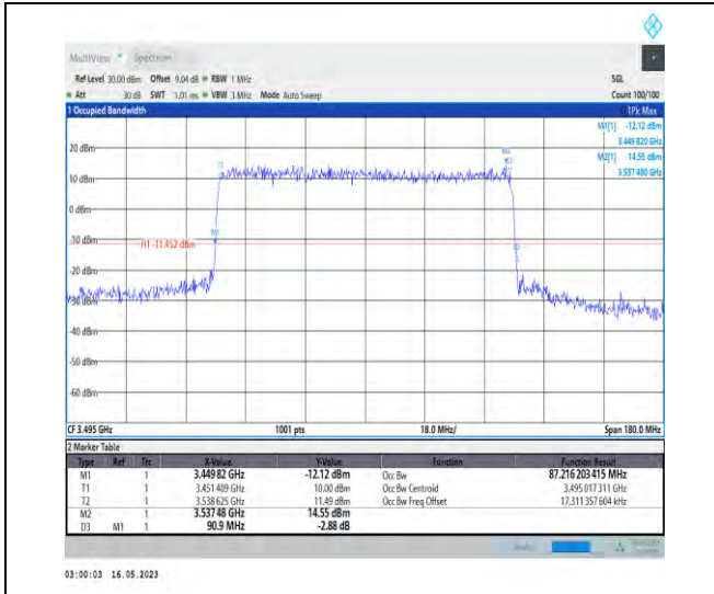
1-N78-3450-3550-PC1-30-90-L-6-CP-QPSK-Outer_Full-245@0-Ant1-87.216-90.900-<math>\leq 90</math>-PASS
