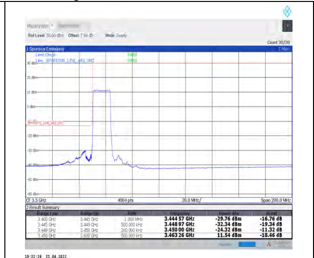
1-N78-3450-3550--30-15-L-3-DFT-PI2BPSK-Outer_Full-36@0-Ant1-PASS-see graph
