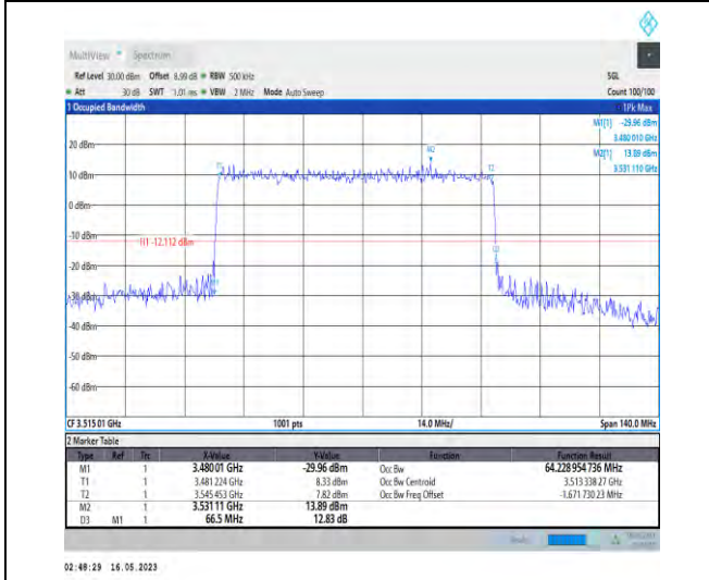
1-N78-3450-3550-PC1-30-70-H-4-DFT-64QAM-Outer_Full-180@0-Ant1-64.229-66.500-≤70-PASS
