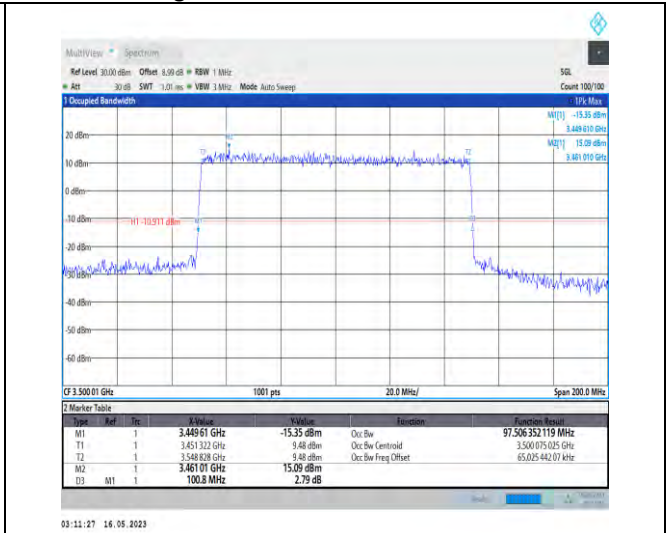
1-N78-3450-3550-PC1-30-100-M-7-CP-16QAM-Outer_Full-273@0-Ant1-97.506-100.800-≤100-PASS
