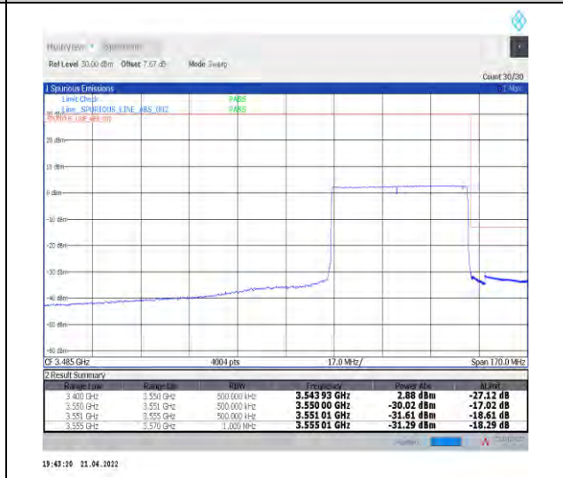
1-N78-3450-3550--30-50-H-6-CP-QPSK-Outer_Fu ll-133@0-Ant1-PASS-see graph
