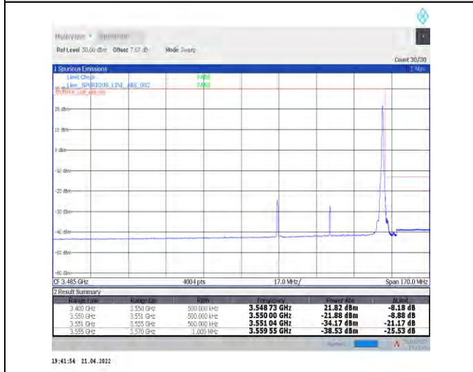
1-N78-3450-3550--30-50-H-5-CP-QPSK-Edge_1RB_R ight-1@132-Ant1-PASS-see graph
