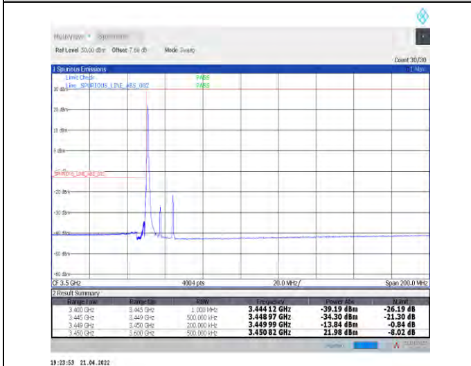
1-N78-3450-3550--30-15-L-4-CP-QPSK-Edge_1RB_L_eft-1@0-Ant1-PASS-see graph
