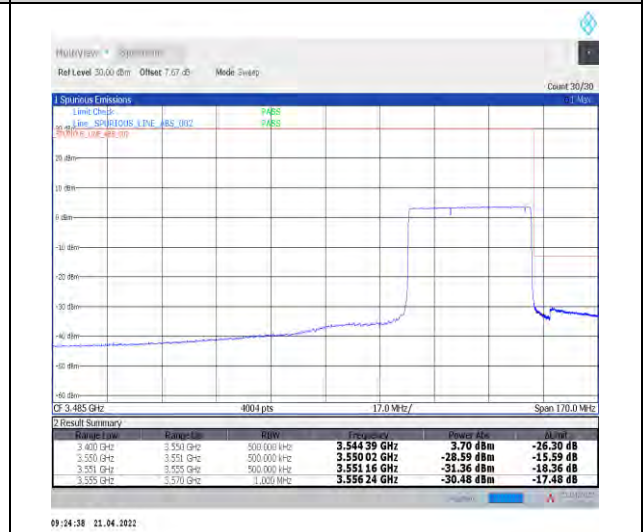
1-N78-3450-3550--30-40-H-6-CP-QPSK-Outer_Fu ll-106@0-Ant1-PASS-see graph
