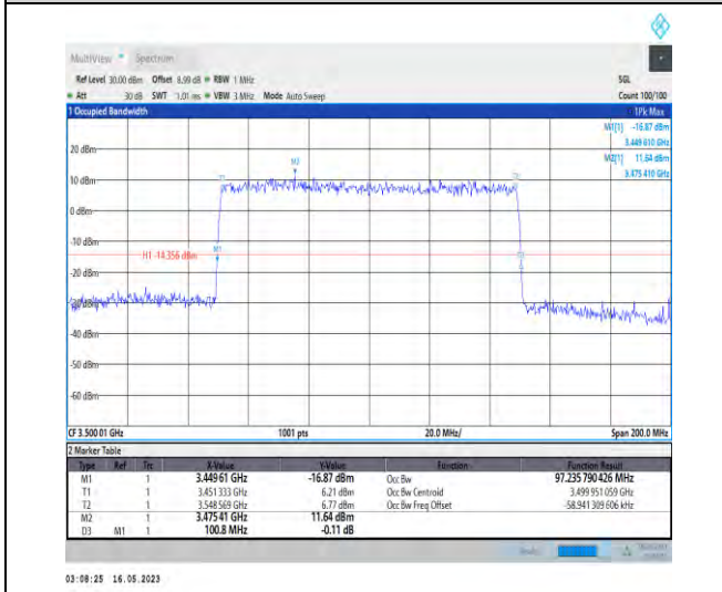
1-N78-3450-3550-PC1-30-100-L-9-CP-256QAM-Outer_Full-273@0-Ant1-97.236-100.800-≤100-PASS
