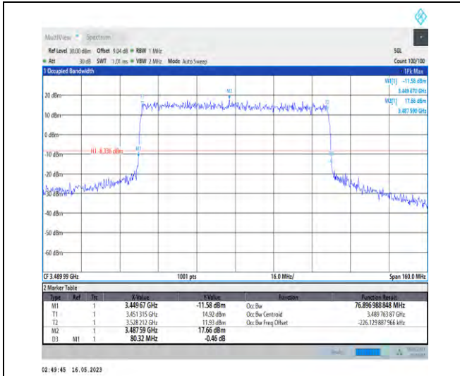
1-N78-3450-3550-PC1-30-80-L-1-DFT-QPSK-Outer_Full-216@0-Ant1-76.897-80.320-≤80-PASS
