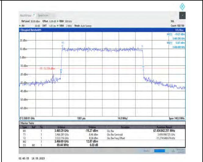
1-N78-3450-3550-PC1-30-70-M-6-CP-QPSK-Outer_Full-189@0-Ant1-67.435-69.440-≤70-PASS
