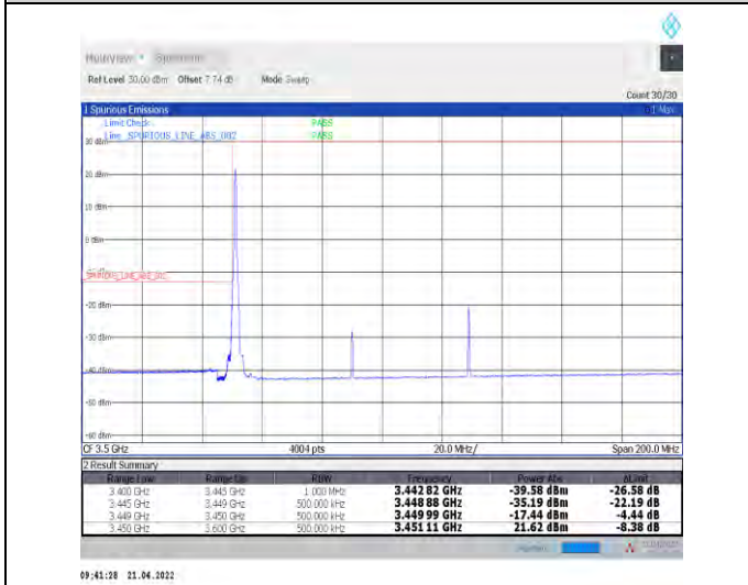
1-N78-3450-3550--30-80-L-4-CP-QPSK-Edge_1RB_L_eff-1@0-Ant1-PASS-see graph
