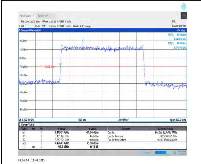
1-N78-3450-3550-PC1-30-100-M-4-DFT-64QAM-Outer_Full-270@0-Ant1-96.252-99.600-≤100-PASS
