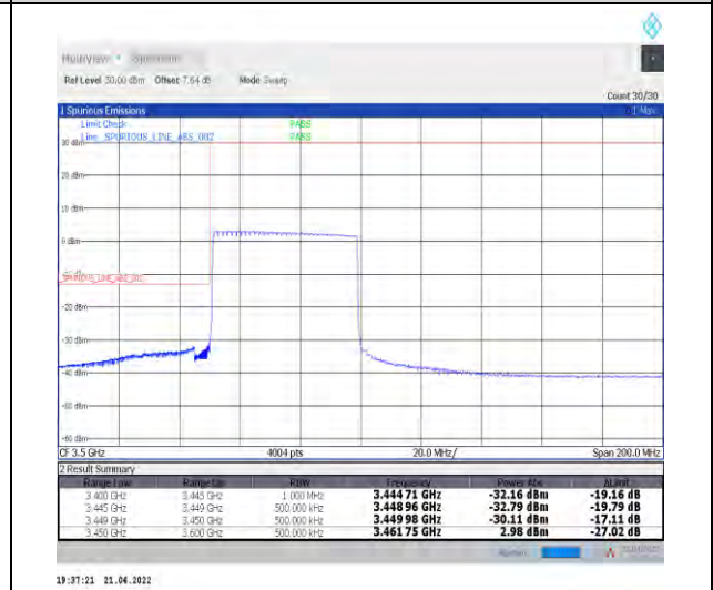
1-N78-3450-3550--30-50-L-6-CP-QPSK-Outer_Ful_I-133@0-Ant1-PASS-see graph
