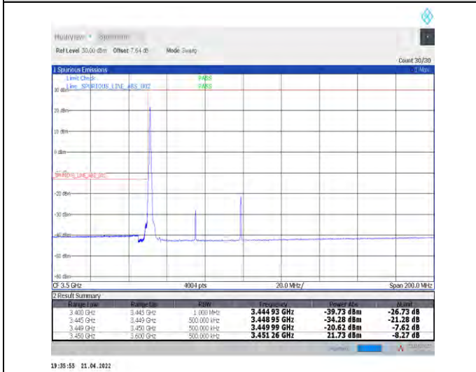
1-N78-3450-3550--30-50-L-4-CP-QPSK-Edge_1RB_L_eft-1@0-Ant1-PASS-see graph
