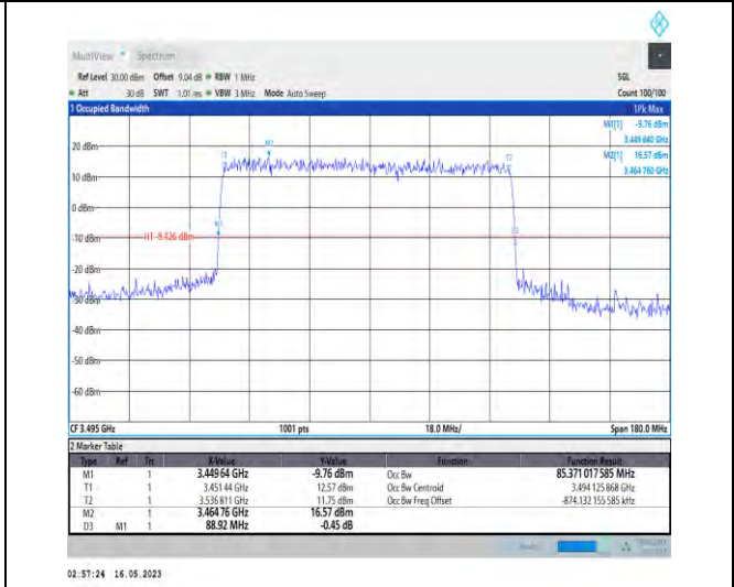
1-N78-3450-3550-PC1-30-90-L-1-DFT-QPSK-Outer_Full-240@0-Ant1-85.371-88.920-≤90-PASS
