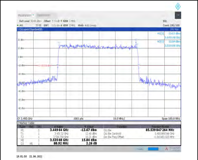
1-N78-3450-3550--30-90-L-1-DFT-QPSK-Outer_Full- 240@0-Ant1-85.54-88.920-≤90-PASS
