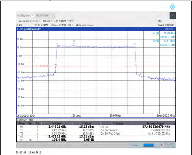
1-N78-3450-3550--30-100-L-8-CP-64QAM-Outer_Fu II-273@0-Ant1-97.481-101.400-≤100-PASS
