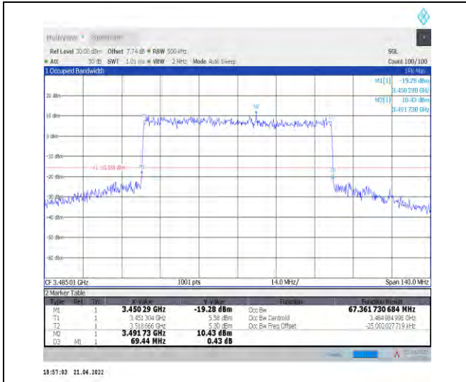
1-N78-3450-3550--30-70-L-8-CP-64QAM-Outer_Full -189@0-Ant1-67.362-69.440-≤70-PASS
