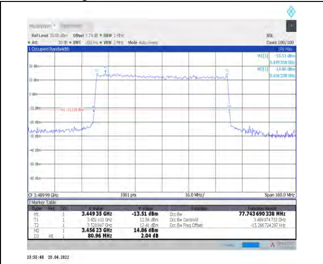
1-N78-3450-3550--30-80-L-6-CP-QPSK-Outer_Full-217@0-Ant1-77.744-80.960-<math>\leq 80</math>-PASS
