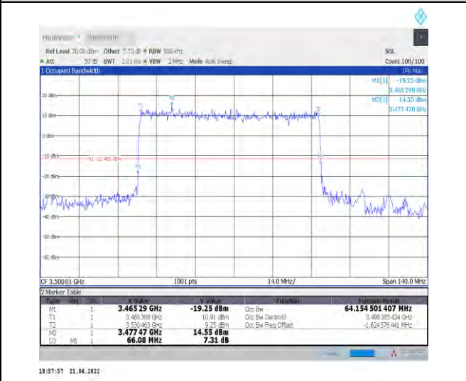
1-N78-3450-3550--30-70-M-2-DFT-PI2BPSK-Outer_Full Full-180@0-Ant1-64.155-66.080-≤70-PASS
