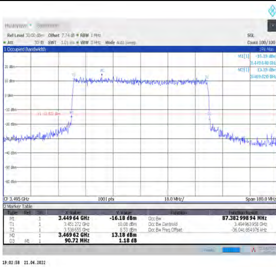
1-N78-3450-3550--30-90-L-6-CP-QPSK-Outer_Full-2 45@0-Ant1-87.383-90.720-<=90-PASS
