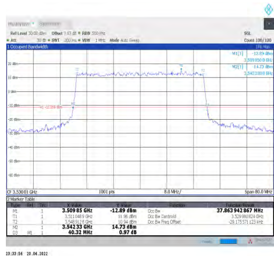
1-N78-3450-3550--30-40-H-6-CP-QPSK-Outer_Full-106@0-Ant1-37.864-40.320-≤40-PASS
