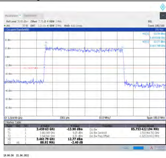
1-N78-3450-3550--30-90-H-5-DFT-256QAM-Outer_Full ull-240@0-Ant1-85.753-88.920-≤90-PASS
