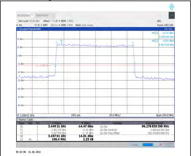
1-N78-3450-3550--30-100-L-4-DFT-64QAM-Outer_F ull-270@0-Ant1-96.279-100.400-≤100-PASS
