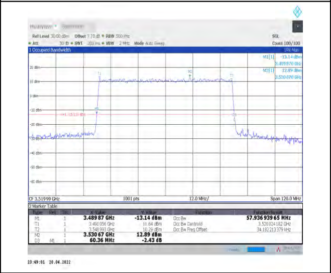
1-N78-3450-3550--30-60-H-4-DFT-64QAM-Outer_Fu II-162@0-Ant1-57.937-60.360-≤60-PASS
