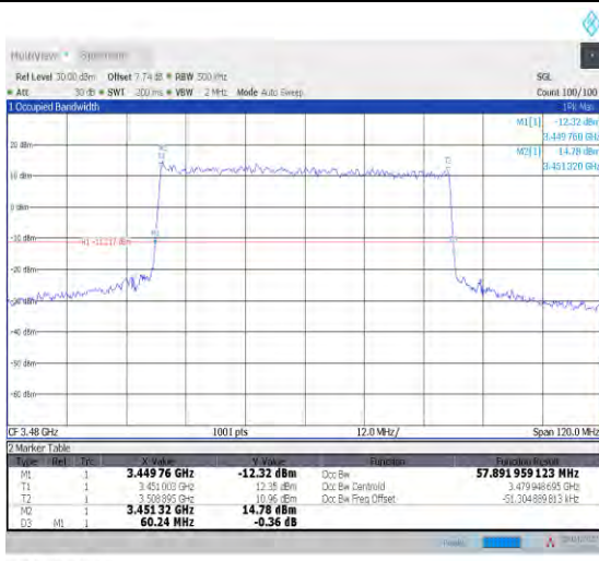
1-N78-3450-3550--30-60-L-3-DFT-16QAM-Outer_Ful I-162@0-Ant1-57.892-60.240-≤60-PASS
