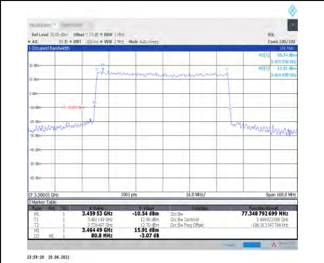
1-N78-3450-3550--30-80-M-3-DFT-16QAM-Outer_Full ull-216@0-Ant1-77.349-80.800≤80-PASS
