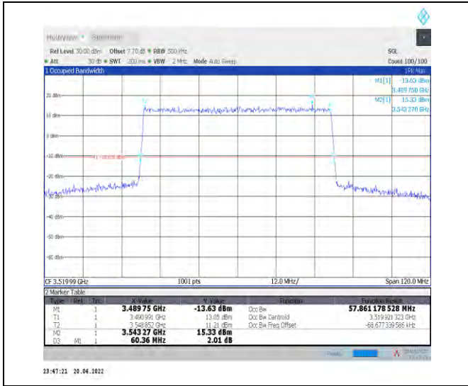
1-N78-3450-3550--30-60-H-1-DFT-QPSK-Outer_Full -162@0-Ant1-57.861-60.360-≤60-PASS
