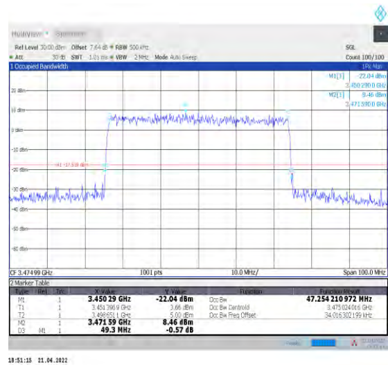
1-N78-3450-3550--30-50-L-9-CP-256QAM-Outer_Fu ll-133@0-Ant1-47.254-49.300-≤50-PASS
