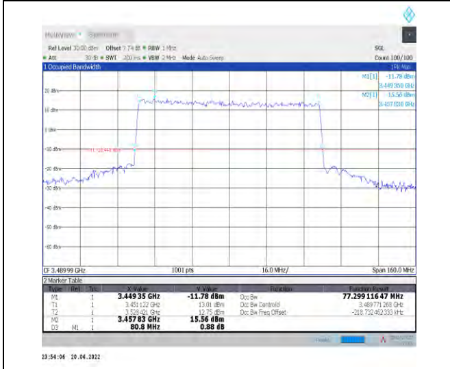
1-N78-3450-3550--30-80-L-3-DFT-16QAM-Outer_Ful-I-216@0-Ant1-77.299-80.800-≤80-PASS
