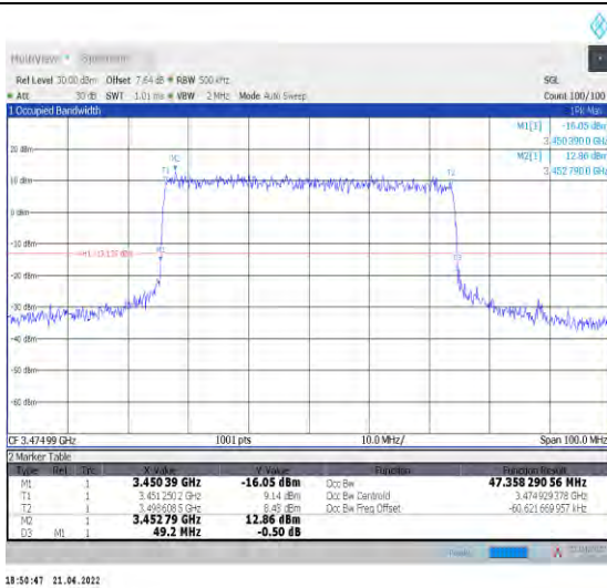
1-N78-3450-3550--30-50-L-6-CP-QPSK-Outer_Full-1 33@0-Ant1-47.358-49.200-≤50-PASS
