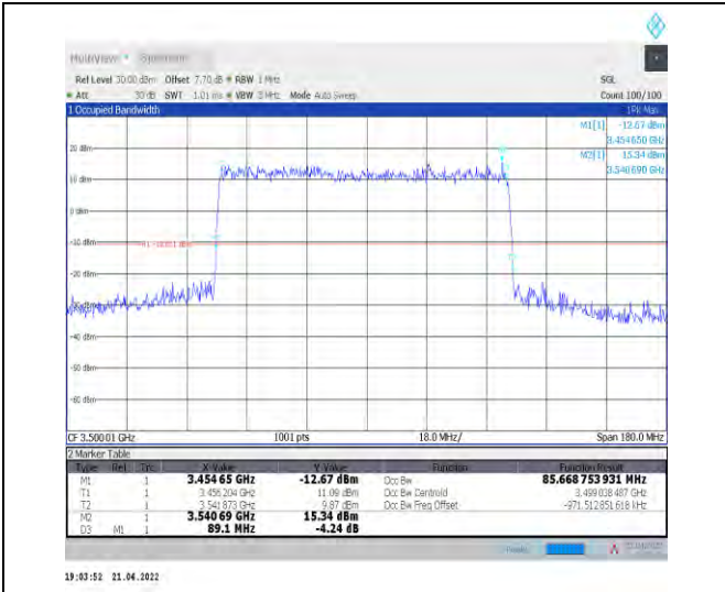
1-N78-3450-3550--30-90-M-1-DFT-QPSK-Outer_Full -240@0-Ant1-85.669-89.100-≤90-PASS
