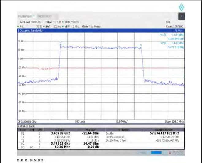
1-N78-3450-3550--30-60-M-1-DFT-QPSK-Outer_Full -162@0-Ant1-57.874-60.360-≤60-PASS
