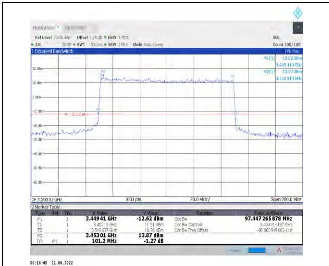
1-N78-3450-3550--30-100-M-6-CP-QPSK-Outer_Full -273@0-Ant1-97.447-101.200-≤100-PASS
