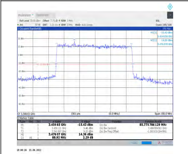
1-N78-3450-3550--30-90-M-3-DFT-16QAM-Outer_Full -240@0-Ant1-85.776-88.920-≤90-PASS
