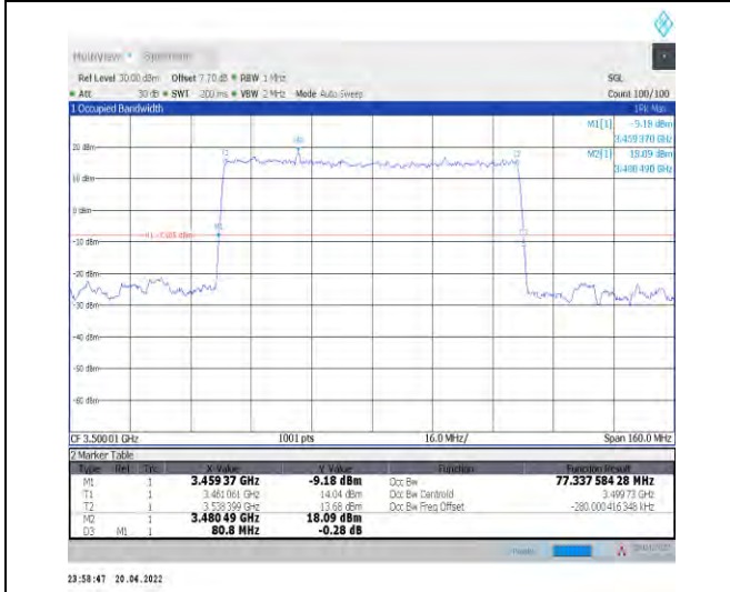
1-N78-3450-3550--30-80-M-2-DFT-PI2BPSK-Outer_Full Full-216@0-Ant1-77.338-80.800≤80-PASS
