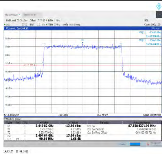
1-N78-3450-3550--30-90-L-7-CP-16QAM-Outer_Full -245@0-Ant1-87.558-90.540-<=90-PASS
