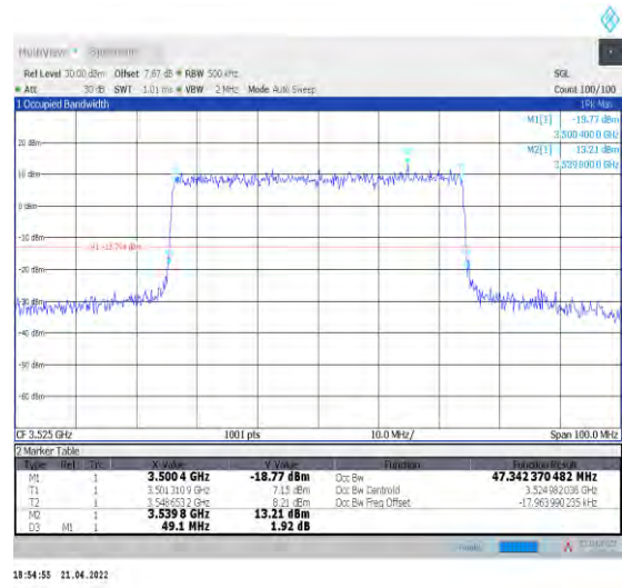
1-N78-3450-3550--30-50-H-7-CP-16QAM-Outer_Full -133@0-Ant1-47.342-49.100-≤50-PASS
