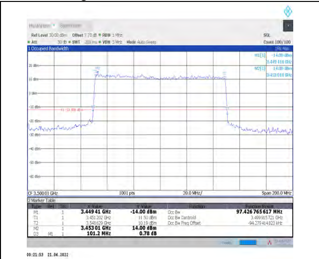
1-N78-3450-3550--30-100-H-6-CP-QPSK-Outer_Full-273@0-Ant1-97.427-101.200-≤100-PASS
