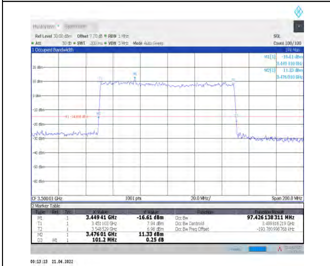
1-N78-3450-3550--30-100-L-9-CP-256QAM-Outer_F ull-273@0-Ant1-97.426-101.200-≤100-PASS
