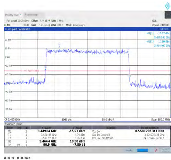
1-N78-3450-3550--30-90-L-9-CP-256QAM-Outer_Fu II-245@0-Ant1-87.58-90.900-<=90-PASS
