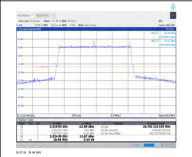
1-N78-3450-3550--30-30-H-5-DFT-256QAM-Outer_Full-75@0-Ant1-26.791-28.980-≤30-PASS
