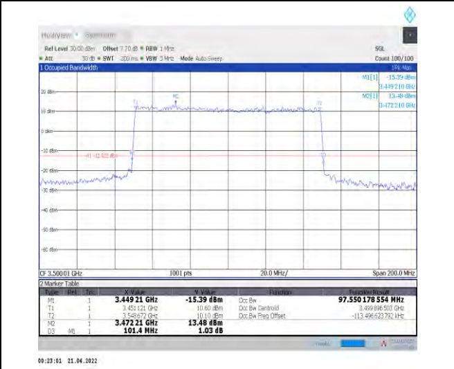
1-N78-3450-3550--30-100-H-8-CP-64QAM-Outer_Full-273@0-Ant1-97.55-101.400-≤100-PASS
