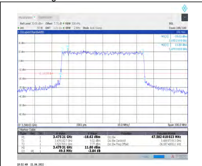
1-N78-3450-3550--30-50-M-6-CP-QPSK-Outer_Full-133@0-Ant1-47.582-49.500-≤50-PASS
