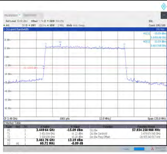
1-N78-3450-3550--30-60-L-4-DFT-64QAM-Outer_Fu II-162@0-Ant1-57.934-60.720-≤60-PASS
