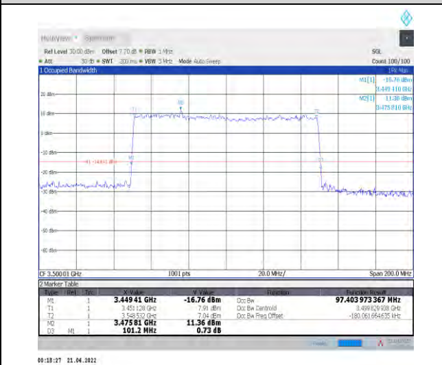
1-N78-3450-3550--30-100-M-9-CP-256QAM-Outer_Full -273@0-Ant1-97.404-101.200-≤100-PASS
