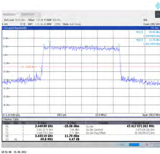
1-N78-3450-3550--30-50-L-8-CP-64QAM-Outer_Full -133@0-Ant1-47.418-49.800-≤50-PASS
