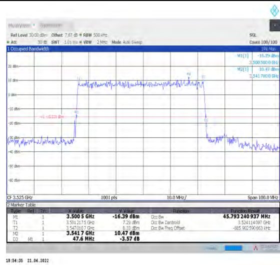
1-N78-3450-3550--30-50-H-5-DFT-256QAM-Outer_F ull-128@0-Ant1-45.793-47.600-≤50-PASS
