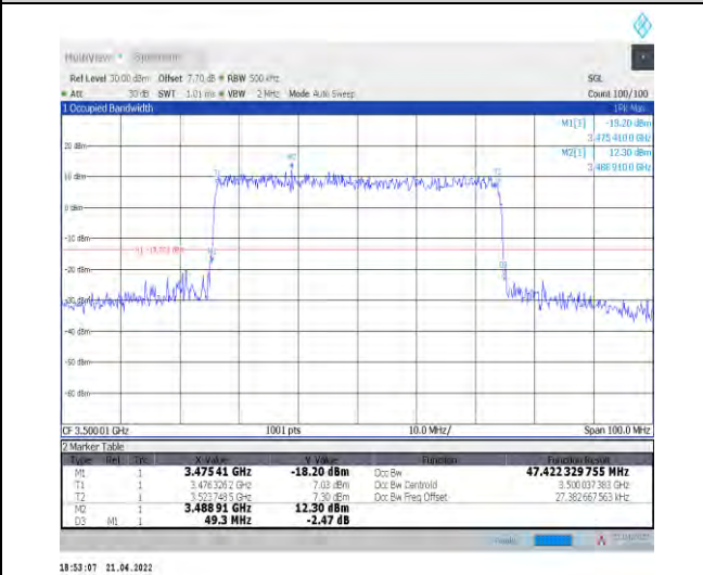
1-N78-3450-3550--30-50-M-8-CP-64QAM-Outer_Full-133@0-Ant1-47.422-49.300-≤50-PASS
