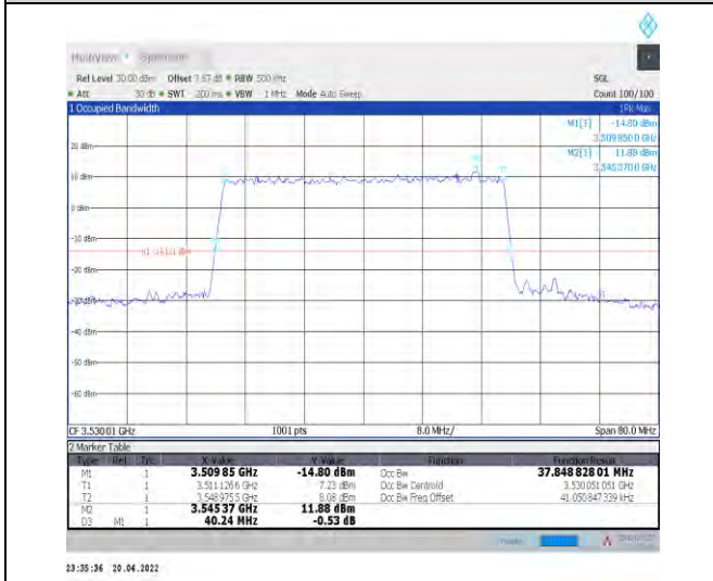
1-N78-3450-3550--30-40-H-9-CP-256QAM-Outer_Fu II-106@0-Ant1-37.849-40.240-≤40-PASS
