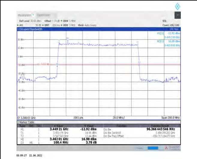
1-N78-3450-3550--30-100-L-2-DFT-PI2BPSK-Outer_Full Full-270@0-Ant1-96.366-100.400-≤100-PASS
