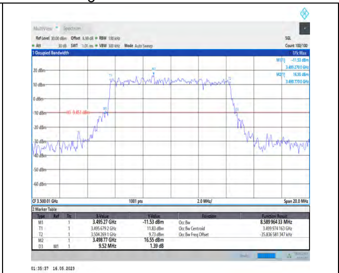
1-N78-3450-3550-PC1-30-10-M-1-DFT-QPSK-Outer_Full-24@0-Ant1-8.59-9.520-≤10-PASS
