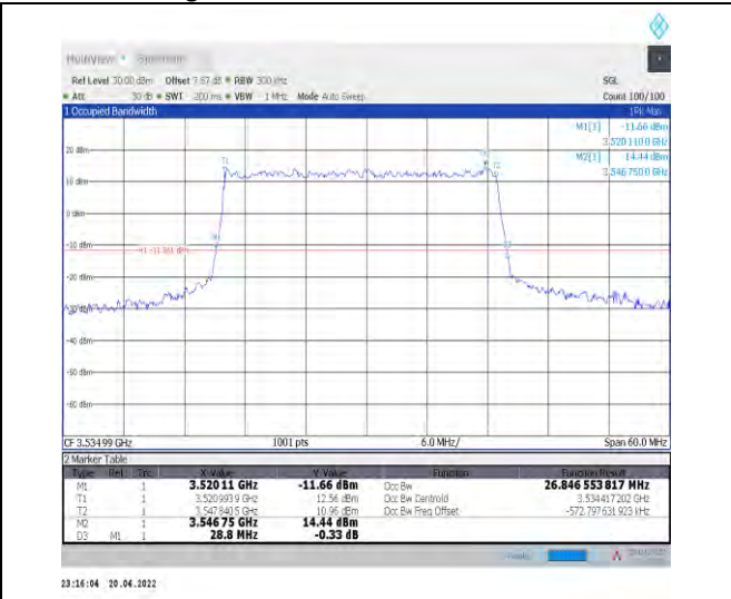
1-N78-3450-3550--30-30-H-3-DFT-16QAM-Outer_Fu II-75@0-Ant1-26.847-28.800-≤30-PASS
