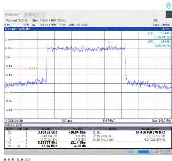
1-N78-3450-3550--30-70-H-1-DFT-QPSK-Outer_Full -180@0-Ant1-64.417-66.360-≤70-PASS
