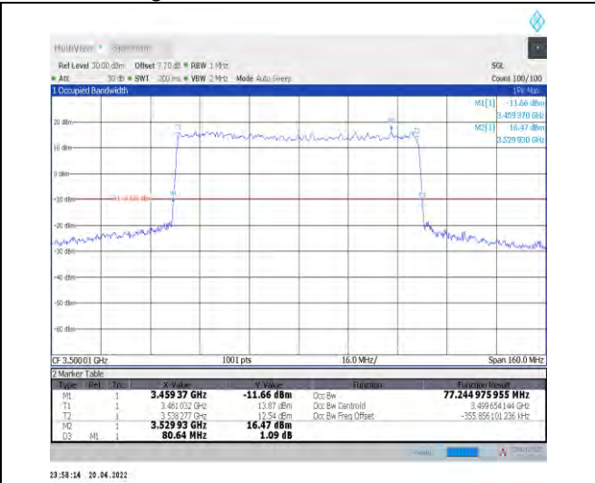
1-N78-3450-3550--30-80-M-1-DFT-QPSK-Outer_Full -216@0-Ant1-77.245-80.640≤80-PASS
