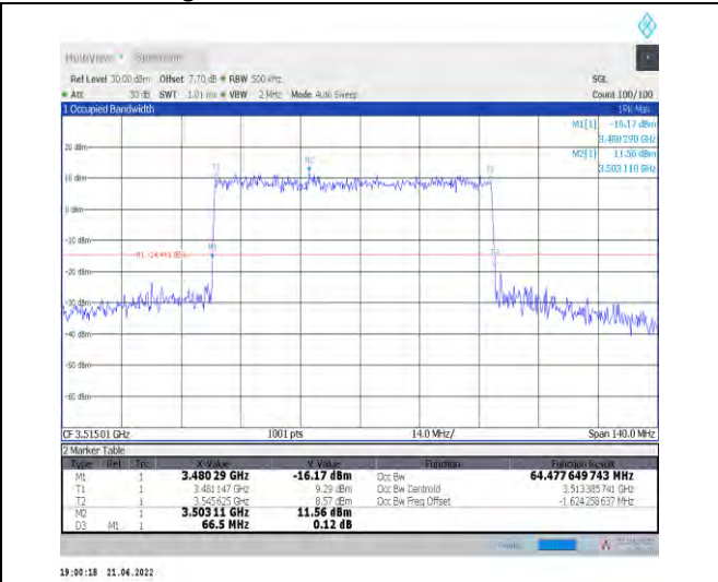
1-N78-3450-3550--30-70-H-3-DFT-16QAM-Outer_Fu II-180@0-Ant1-64.478-66.500-<=70-PASS
