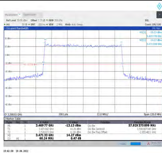
1-N78-3450-3550--30-60-M-3-DFT-16QAM-Outer_Full-162@0-Ant1-57.929-60.240-≤60-PASS
