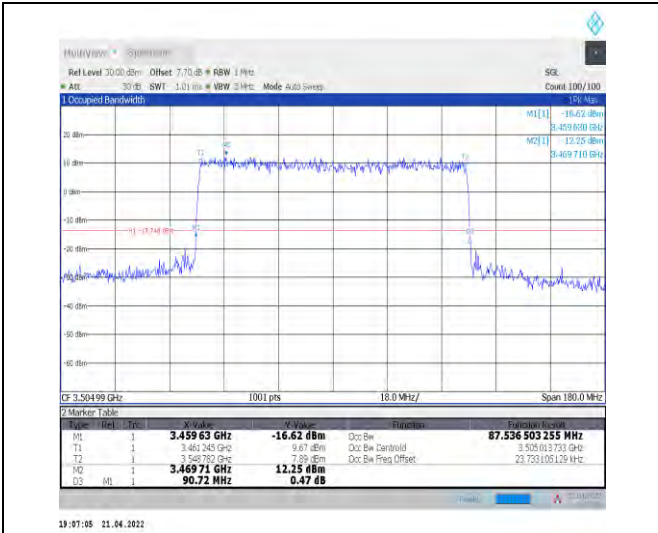
1-N78-3450-3550--30-90-H-8-CP-64QAM-Outer_Full -245@0-Ant1-87.537-90.720-≤90-PASS
