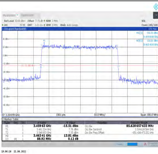
1-N78-3450-3550--30-90-H-4-DFT-64QAM-Outer_Fu ll-240@0-Ant1-85.629-88.920-≤90-PASS
