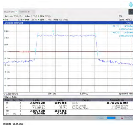
1-N78-3450-3550--30-40-M-3-DFT-16QAM-Outer_Full-100@0-Ant1-35.761-38.240-≤40-PASS
