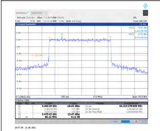
1-N78-3450-3550--30-70-M-1-DFT-QPSK-Outer_Full -180@0-Ant1-64.315-66.220-≤70-PASS
