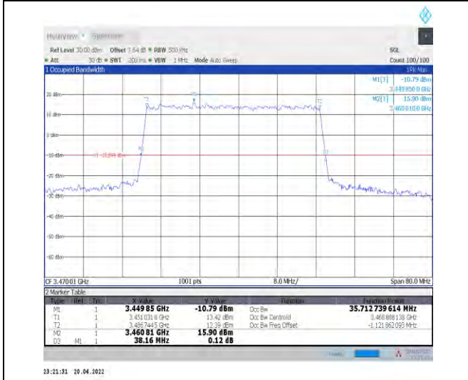
1-N78-3450-3550--30-40-L-3-DFT-16QAM-Outer_Ful-I-100@0-Ant1-35.713-38.160-≤40-PASS
