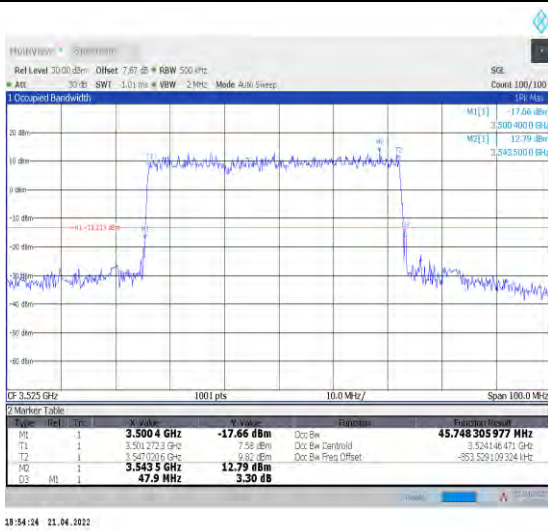
1-N78-3450-3550--30-50-H-4-DFT-64QAM-Outer_Fu ll-128@0-Ant1-45.748-47.900-≤50-PASS
