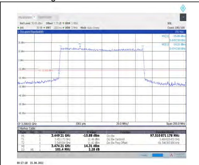
1-N78-3450-3550--30-100-M-7-CP-16QAM-Outer_Full -273@0-Ant1-97.511-101.400-≤100-PASS
