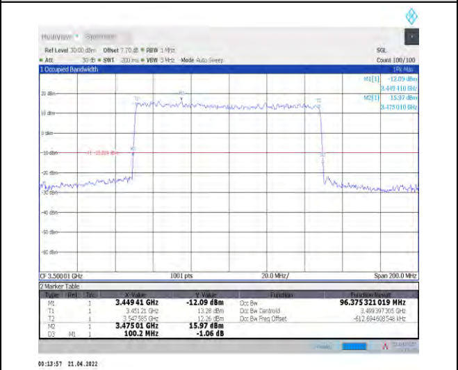
1-N78-3450-3550--30-100-M-1-DFT-QPSK-Outer_F ull-270@0-Ant1-96.375-100.200-≤100-PASS
