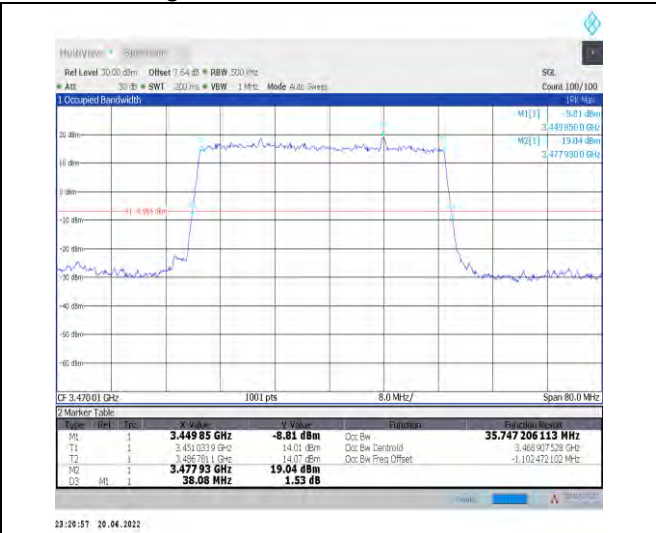
1-N78-3450-3550--30-40-L-2-DFT-PI2BPSK-Outer_Full-100@0-Ant1-35.747-38.080-≤40-PASS
