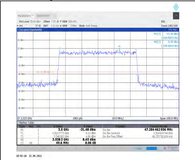
1-N78-3450-3550--30-50-H-9-CP-256QAM-Outer_Full-133@0-Ant1-47.284-49.600-≤50-PASS
