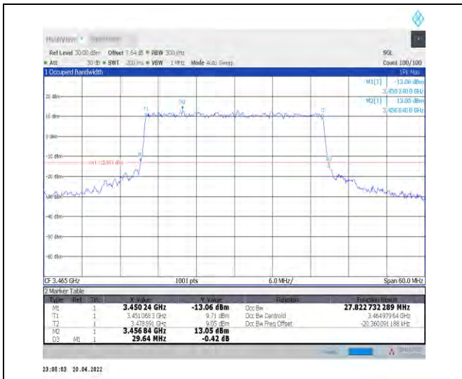
1-N78-3450-3550--30-30-L-8-CP-64QAM-Outer_Full -78@0-Ant1-27.823-29.640-<30-PASS
