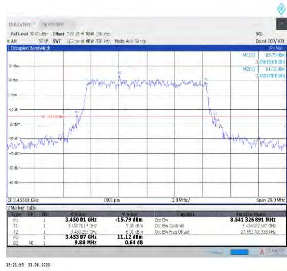
1-N78-3450-3550--30-10-L-8-CP-64QAM-Outer_Full-24@0-Ant1-8.541-9.880-≤10-PASS
