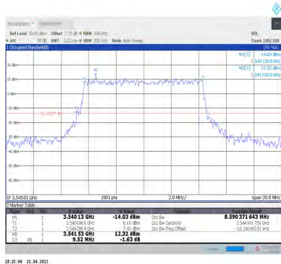
1-N78-3450-3550--30-10-H-6-CP-QPSK-Outer_Full- 24@0-Ant1-8.59-9.520-≤10-PASS
