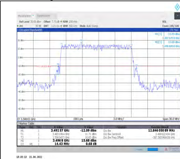
1-N78-3450-3550--30-15-M-2-DFT-PI2BPSK-Outer_Full Full-36@0-Ant1-12.846-14.430-≤15-PASS
