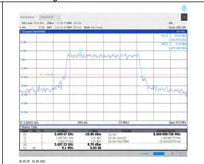
1-N78-3450-3550--30-10-M-9-CP-256QAM-Outer_Full-24@0-Ant1-8.567-9.100-<=10-PASS
