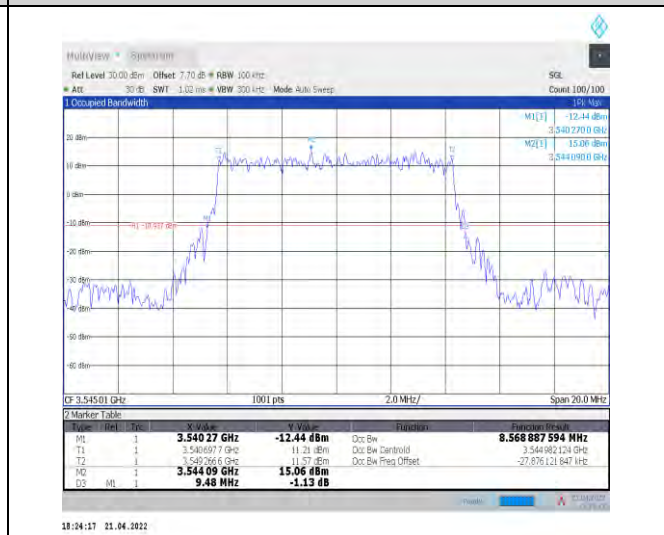
1-N78-3450-3550--30-10-H-2-DFT-PI2BPSK-Outer_Full-24@0-Ant1-8.569-9.480-<=10-PASS
