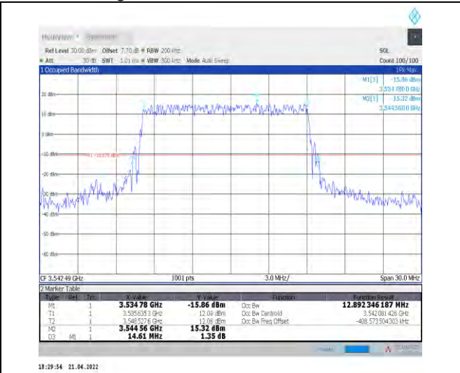
1-N78-3450-3550--30-15-H-1-DFT-QPSK-Outer_Full-36@0-Ant1-12.892-14.610-≤15-PASS
