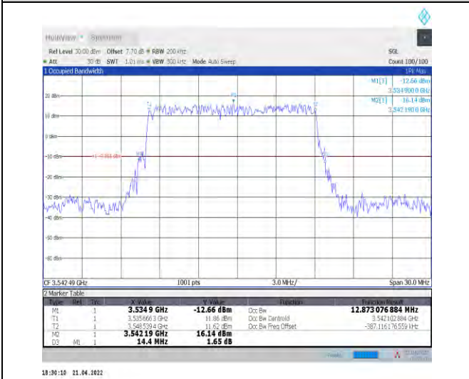
1-N78-3450-3550--30-15-H-2-DFT-PI2BPSK-Outer_Full-36@0-Ant1-12.873-14.400-≤15-PASS
