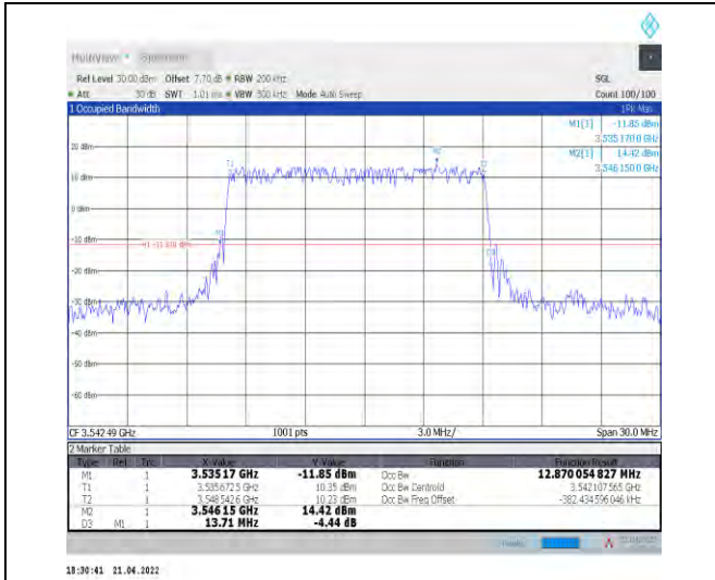
1-N78-3450-3550--30-15-H-4-DFT-64QAM-Outer_Fu ll-36@0-Ant1-12.87-13.710-≤15-PASS
