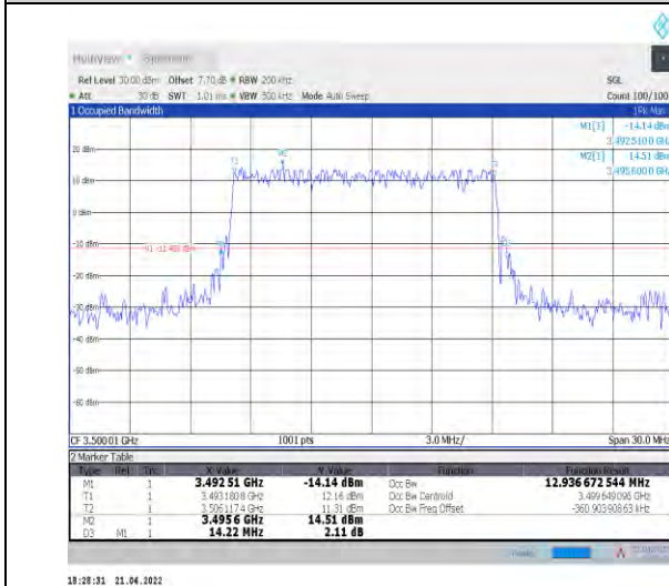
1-N78-3450-3550--30-15-M-3-DFT-16QAM-Outer_Full ull-36@0-Ant1-12.937-14.220-≤15-PASS
