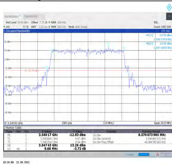
1-N78-3450-3550--30-10-H-4-DFT-64QAM-Outer_Fu Il-24@0-Ant1-8.57-9.680-≤10-PASS
