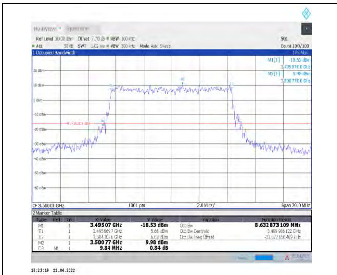
1-N78-3450-3550--30-10-M-8-CP-64QAM-Outer_Full -24@0-Ant1-8.633-9.840-<=10-PASS
