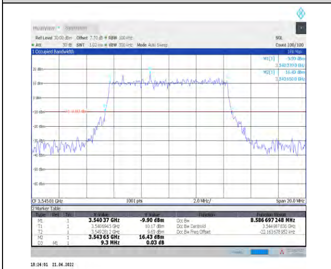
1-N78-3450-3550--30-10-H-1-DFT-QPSK-Outer_Full -24@0-Ant1-8.587-9.300-<=10-PASS
