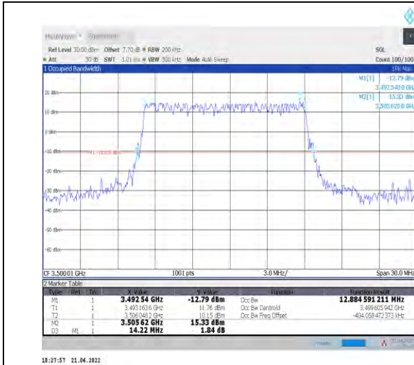
1-N78-3450-3550--30-15-M-1-DFT-QPSK-Outer_Full -36@0-Ant1-12.885-14.220-≤15-PASS
