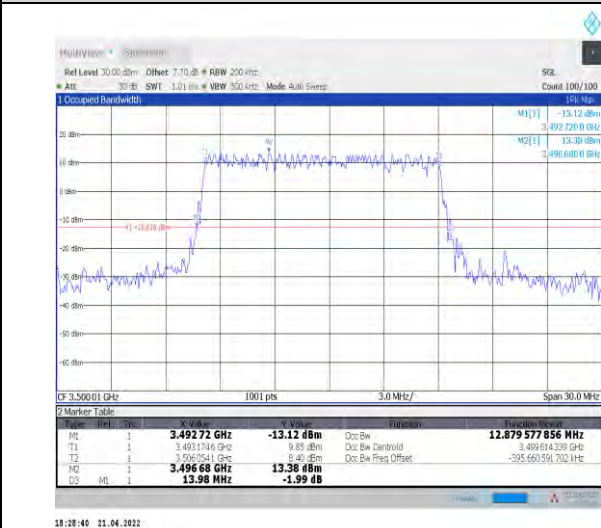
1-N78-3450-3550--30-15-M-4-DFT-64QAM-Outer_Full ull-36@0-Ant1-12.88-13.980-≤15-PASS
