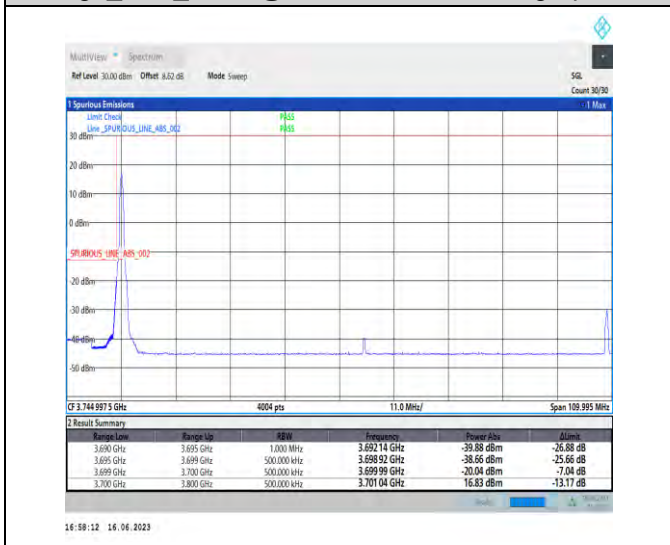
1-N77-3700-3980-PC1-30-100-L-4-CP-QPSK-Edge_1RB_Left-1@0-Ant1-1--PASS-see graph
