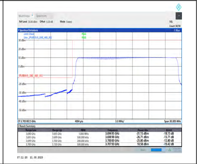
1-N77-3700-3980-PC1-30-20-L-6-CP-QPSK-Outer_Full-51@0-Ant1-1--PASS-see graph
