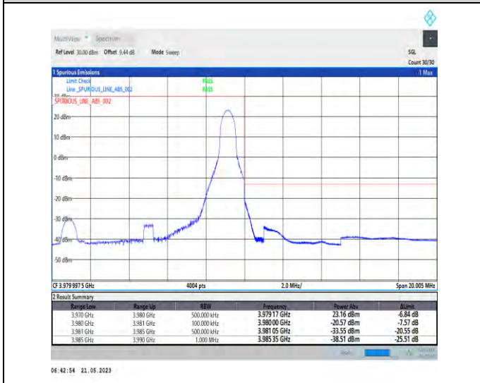
1-N77-3700-3980-PC1-30-10-H-5-CP-QPSK-Edge_1RB_Right-1@23-Ant1-1--PASS-see graph
