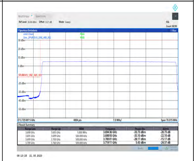
1-N77-3700-3980-PC1-30-60-L-6-CP-QPSK-Outer_Full-162@0-Ant1-1--PASS-see graph
