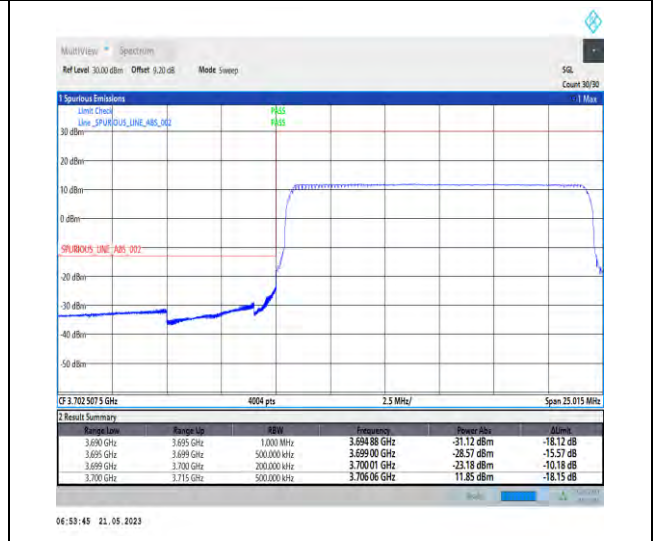
1-N77-3700-3980-PC1-30-15-L-6-CP-QPSK-Outer_Full-38@0-Ant1-1--PASS-see graph
