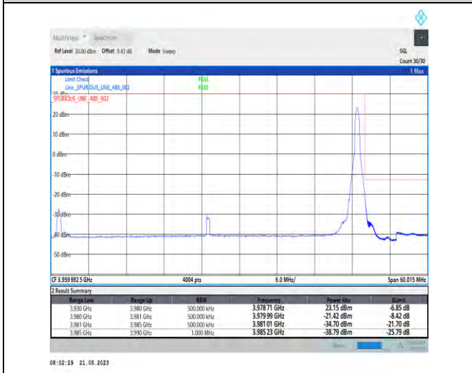
1-N77-3700-3980-PC1-30-50-H-5-CP-QPSK-Edge_1RB_Right-1@132-Ant1-1--PASS-see graph
