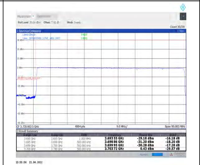
1-N77-3700-3980--30-80-L-6-CP-QPSK-Outer_Ful_I-217@0-Ant1-PASS-see graph
