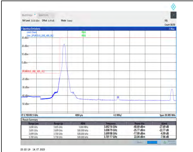
1-N77-3700-3980-PC1-30-30-L-1-DFT-PI2BPSK-Edge_1RB_Left-1@0-Ant1-1--PASS-see graph
