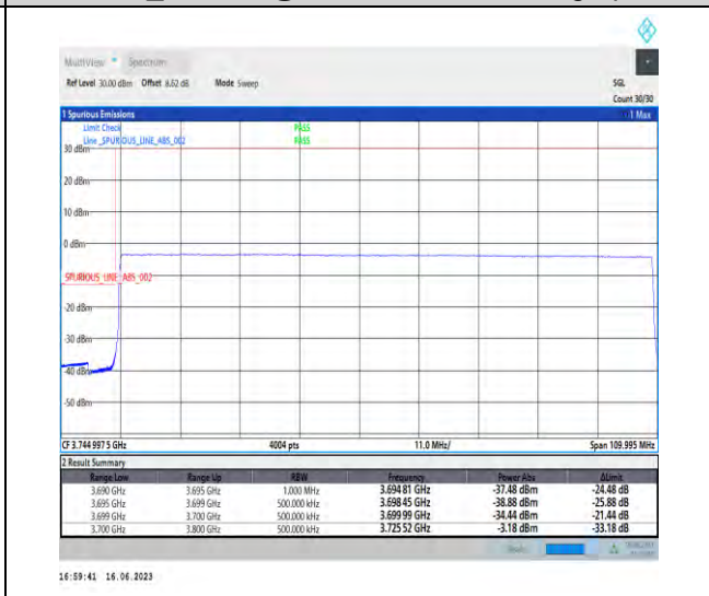
1-N77-3700-3980-PC1-30-100-L-6-CP-QPSK-Outer_Full-273@0-Ant1-1--PASS-see graph
