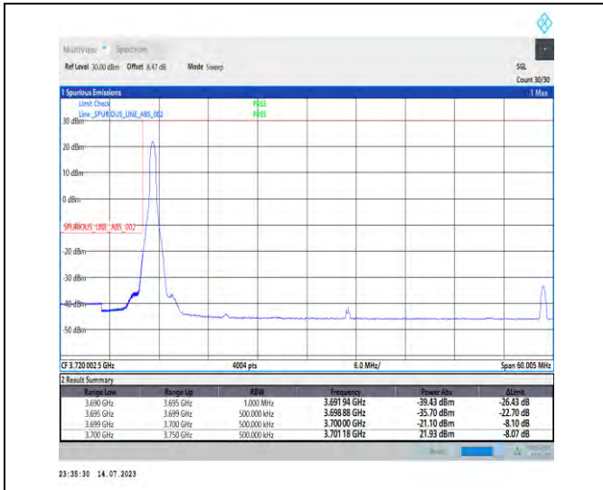
1-N77-3700-3980-PC1-30-50-L-1-DFT-PI2BPSK-Edge_1_RB_Left-1@0-Ant1-1--PASS-see graph
