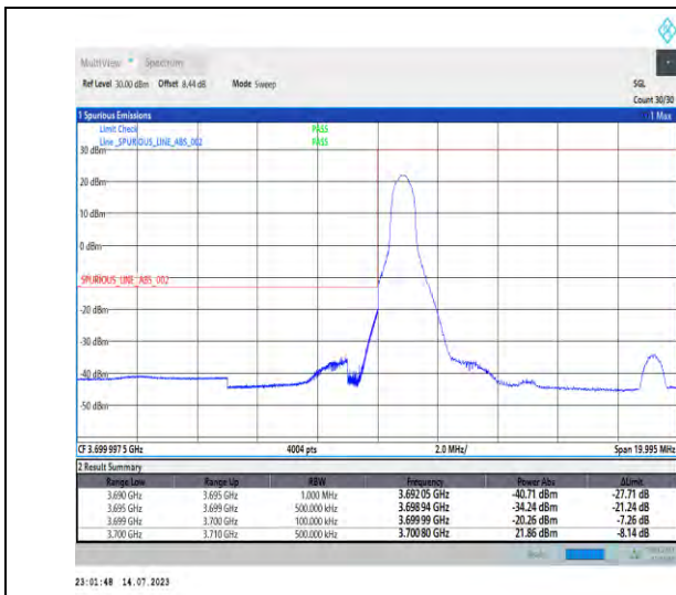
1-N77-3700-3980-PC1-30-10-L-1-DFT-PI2BPSK-Edge_e_1RB_Left-1@0-Ant1-1--PASS-see graph
