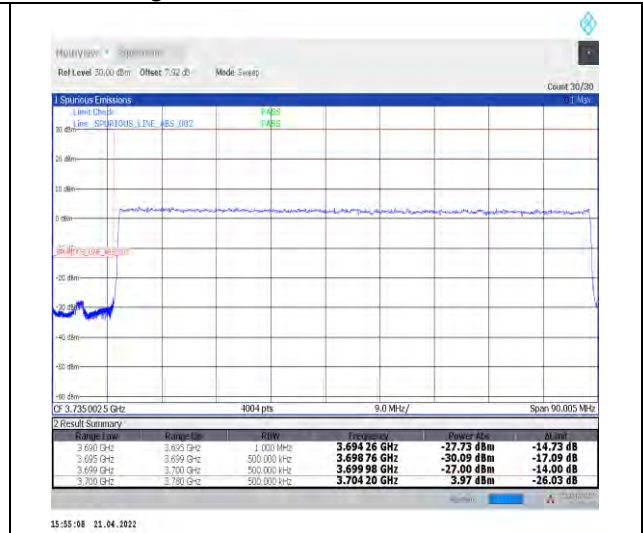
1-N77-3700-3980--30-80-L-3-DFT-PI2BPSK-Outer_Full-216@0-Ant1-PASS-see graph
