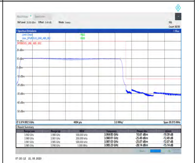
1-N77-3700-3980-PC1-30-20-H-6-CP-QPSK-Outer_Full-51@0-Ant1-1--PASS-see graph
