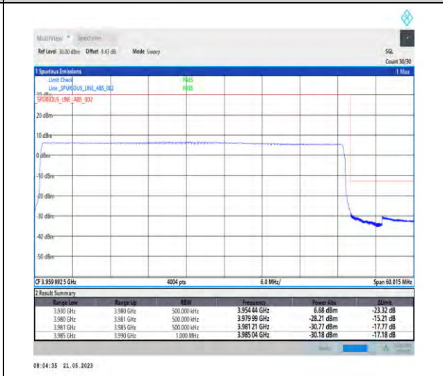
1-N77-3700-3980-PC1-30-50-H-6-CP-QPSK-Outer_Full-133@0-Ant1-1--PASS-see graph
