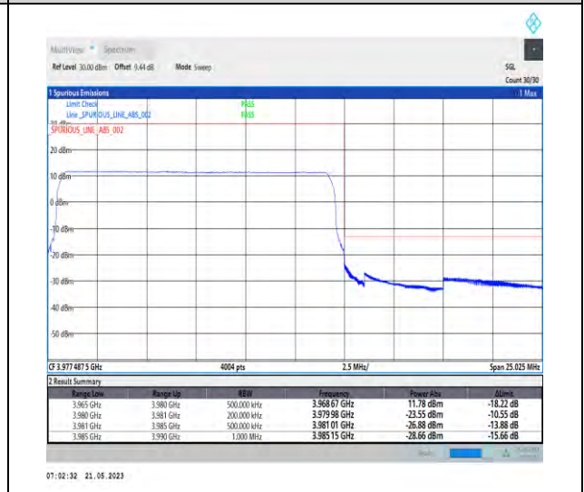
1-N77-3700-3980-PC1-30-15-H-6-CP-QPSK-Outer_Full-38@0-Ant1-1--PASS-see graph
