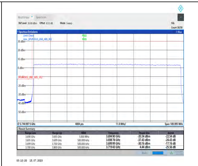
1-N77-3700-3980-PC1-30-100-L-3-DFT-PI2BPSK-Outer_Full-270@0-Ant1-1--PASS-see graph
