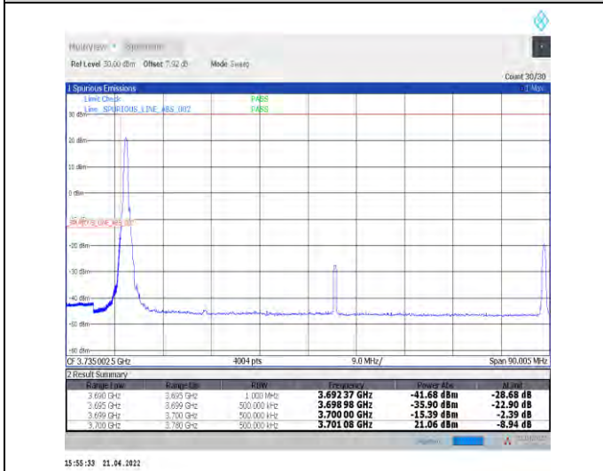
1-N77-3700-3980--30-80-L-4-CP-QPSK-Edge_1RB_L_eft-1@0-Ant1-PASS-see graph
