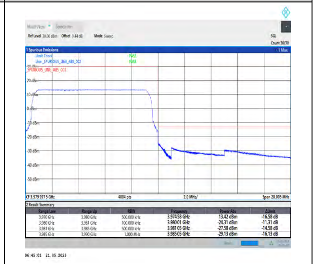
1-N77-3700-3980-PC1-30-10-H-6-CP-QPSK-Outer_Full-24@0-Ant1-1--PASS-see graph
