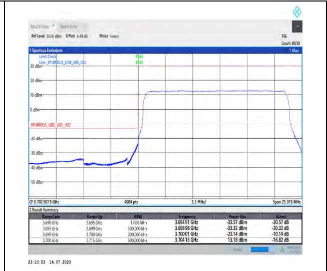
1-N77-3700-3980-PC1-30-15-L-3-DFT-PI2BPSK-Outer_Full-36@0-Ant1-1--PASS-see graph
