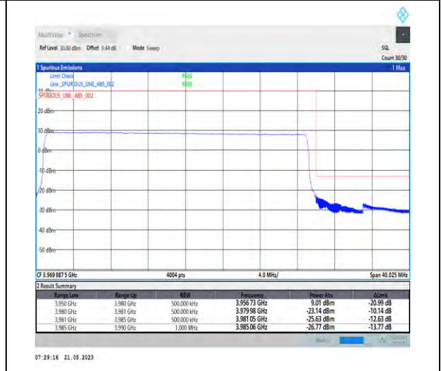
1-N77-3700-3980-PC1-30-30-H-6-CP-QPSK-Outer_Full-78@0-Ant1-1--PASS-see graph
