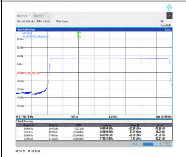
1-N77-3700-3980-PC1-30-40-L-6-CP-QPSK-Outer_Full-106@0-Ant1-1--PASS-see graph
