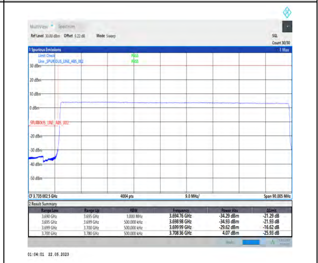
1-N77-3700-3980-PC1-30-80-L-6-CP-QPSK-Outer_Full-217@0-Ant1-1--PASS-see graph
