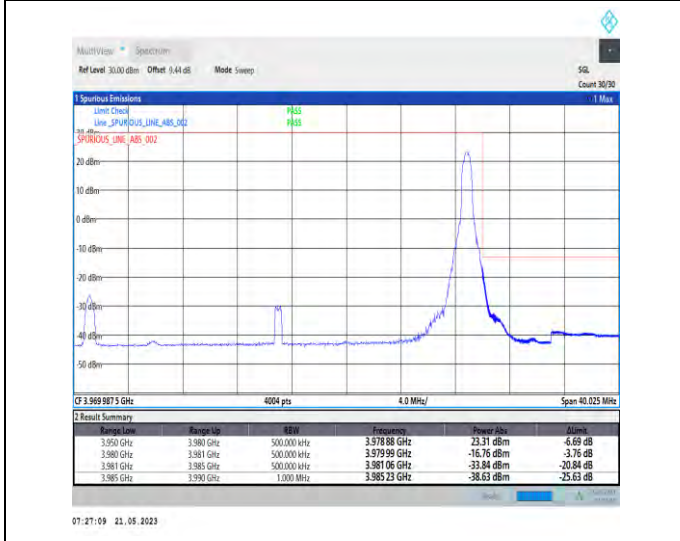
1-N77-3700-3980-PC1-30-30-H-5-CP-QPSK-Edge_1RB_Right-1@77-Ant1-1--PASS-see graph
