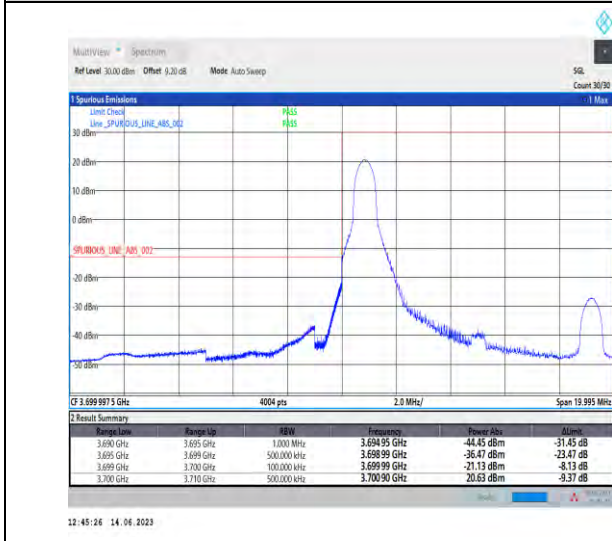
1-N77-3700-3980-PC1-30-10-L-4-CP-QPSK-Edge_1RB_Left-1@0-Ant1-1--PASS-see graph
