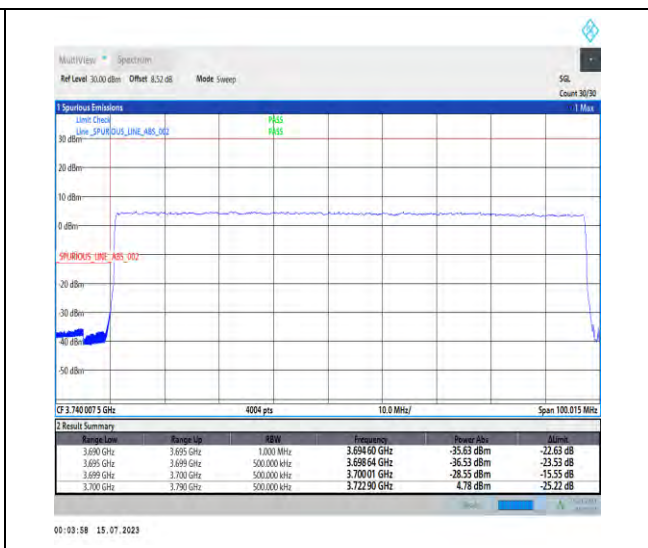
1-N77-3700-3980-PC1-30-90-L-3-DFT-PI2BPSK-Outer_Full-240@0-Ant1-1--PASS-see graph
