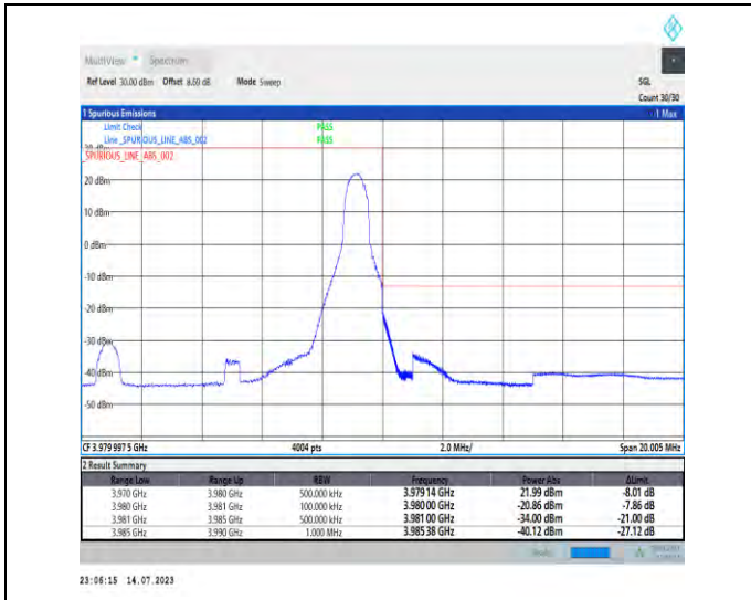
1-N77-3700-3980-PC1-30-10-H-2-DFT-PI2BPSK-Edge_1RB_Right-1@23-Ant1-1--PASS-see graph
