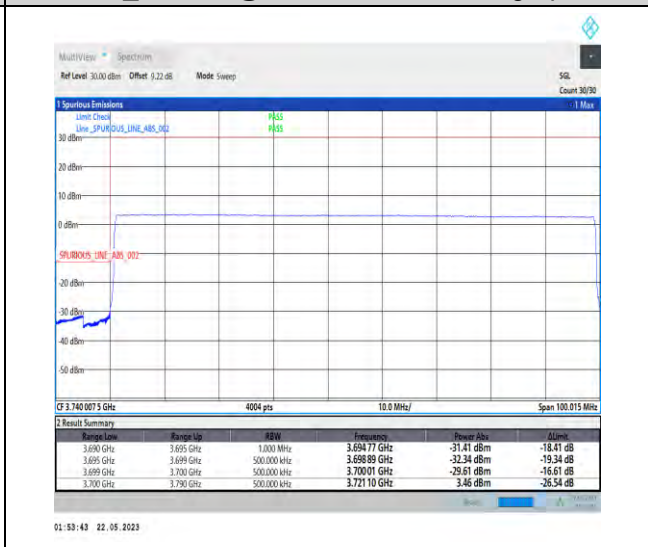
1-N77-3700-3980-PC1-30-90-L-6-CP-QPSK-Outer_Full-245@0-Ant1-1--PASS-see graph
