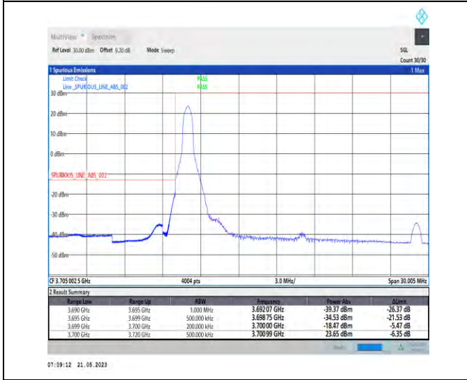
1-N77-3700-3980-PC1-30-20-L-4-CP-QPSK-Edge_1RB_Left-1@0-Ant1-1--PASS-see graph
