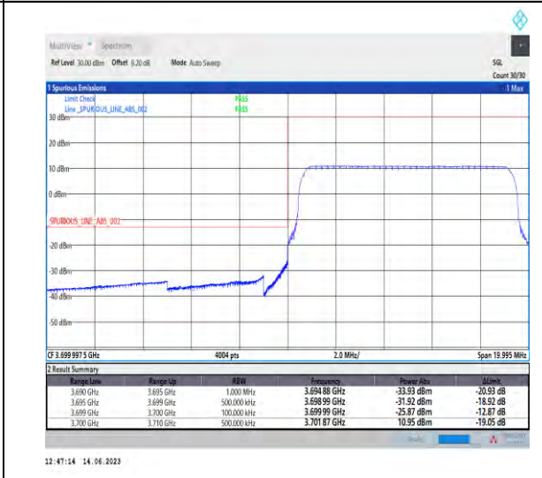
1-N77-3700-3980-PC1-30-10-L-6-CP-QPSK-Outer_Full-24@0-Ant1-1--PASS-see graph
