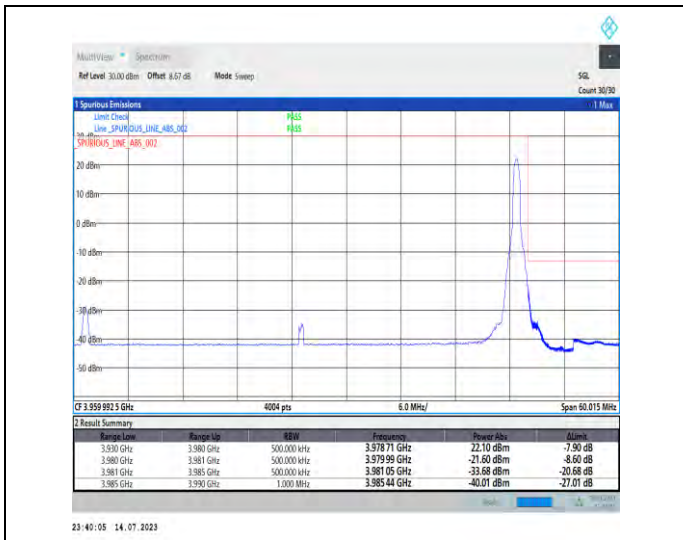
1-N77-3700-3980-PC1-30-50-H-2-DFT-PI2BPSK-Edge_1RB_Right-1@132-Ant1-1--PASS-see graph
