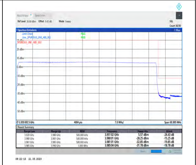
1-N77-3700-3980-PC1-30-60-H-6-CP-QPSK-Outer_Full-162@0-Ant1-1--PASS-see graph
