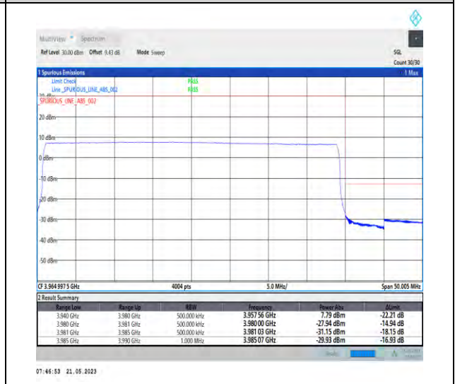
1-N77-3700-3980-PC1-30-40-H-6-CP-QPSK-Outer_Full-106@0-Ant1-1--PASS-see graph
