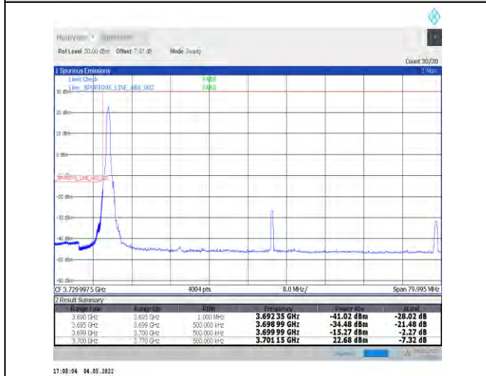
1-N77-3700-3980--30-70-L-4-CP-QPSK-Edge_1RB_L eft-1@0-Ant1-PASS-see graph
