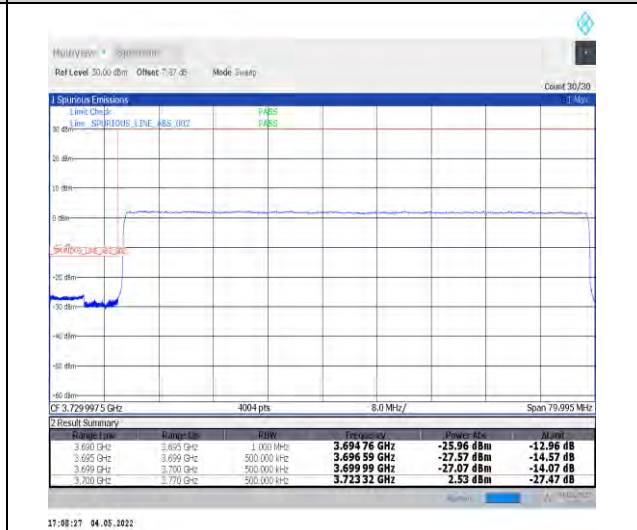
1-N77-3700-3980--30-70-L-6-CP-QPSK-Outer_Ful l-189@0-Ant1-PASS-see graph
