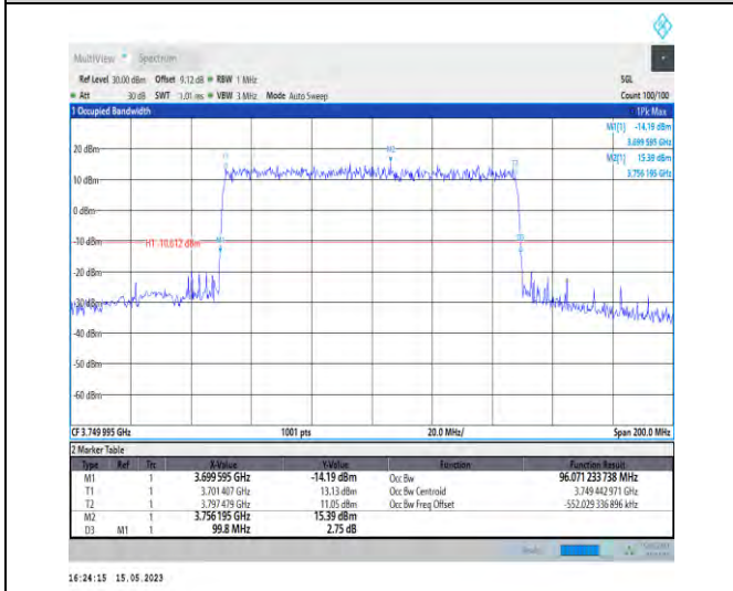
1-N77-3700-3980-PC1-30-100-L-1-DFT-QPSK-Outer_Full-270@0-Ant1-96.071-99.800-<=100-PASS
