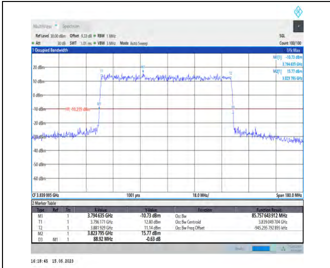
1-N77-3700-3980-PC1-30-90-M-1-DFT-QPSK-Outer_Full-240@0-Ant1-85.758-88.920-≤90-PASS
