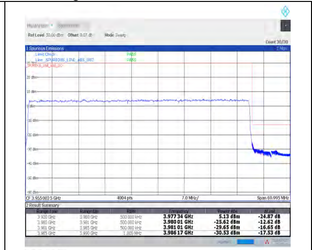
1-N77-3700-3980--30-60-H-3-DFT-PI2BPSK-Outer_Full-162@0-Ant1-PASS-see graph
