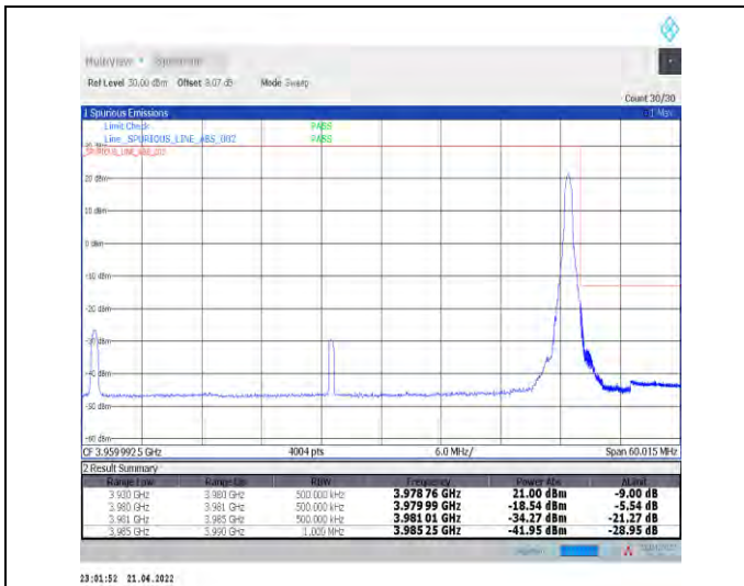
1-N77-3700-3980--30-50-H-2-DFT-PI2BPSK-Edge_1R_B_Right-1@132-Ant1-PASS-see graph
