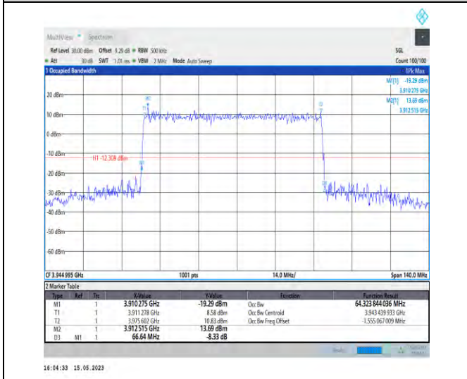
1-N77-3700-3980-PC1-30-70-H-4-DFT-64QAM-Out er_Full-180@0-Ant1-64.324-66.640-≤70-PASS
