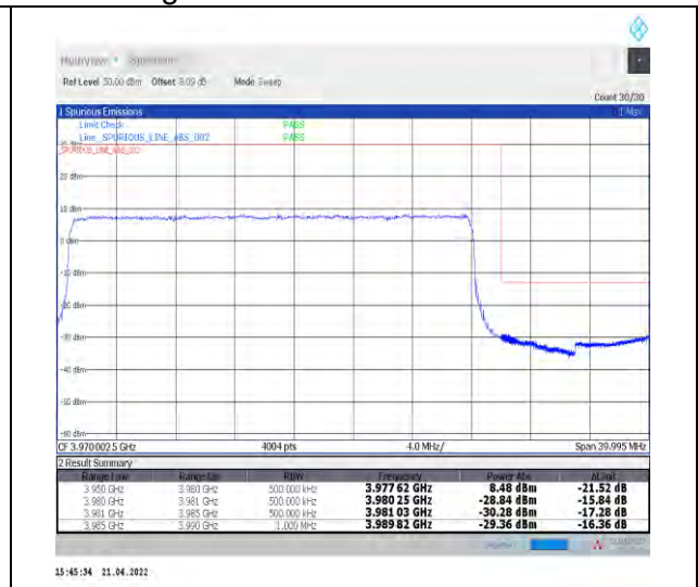
1-N77-3700-3980--30-30-H-3-DFT-PI2BPSK-Outer_Full-75@0-Ant1-PASS-see graph
