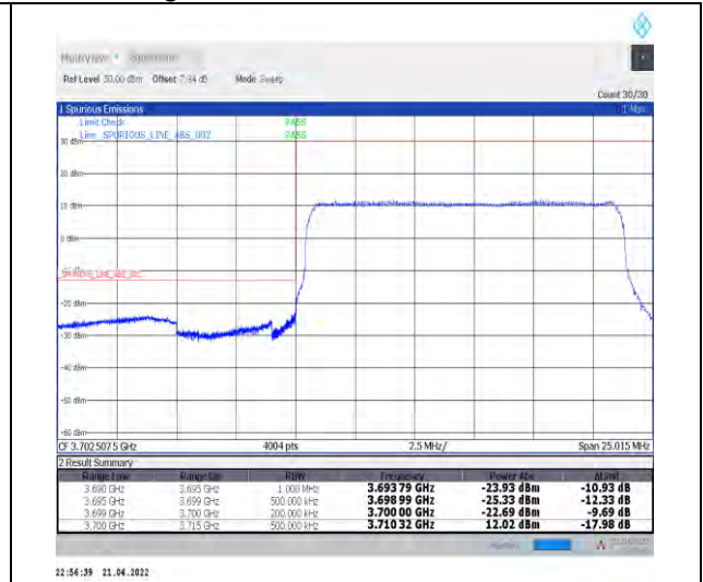
1-N77-3700-3980--30-15-L-3-DFT-PI2BPSK-Outer_Full-36@0-Ant1-PASS-see graph
