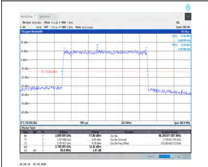
1-N77-3700-3980-PC1-30-100-L-5-DFT-256QAM-Out er_Full-270@0-Ant1-96.351-99.800-≤100-PASS
