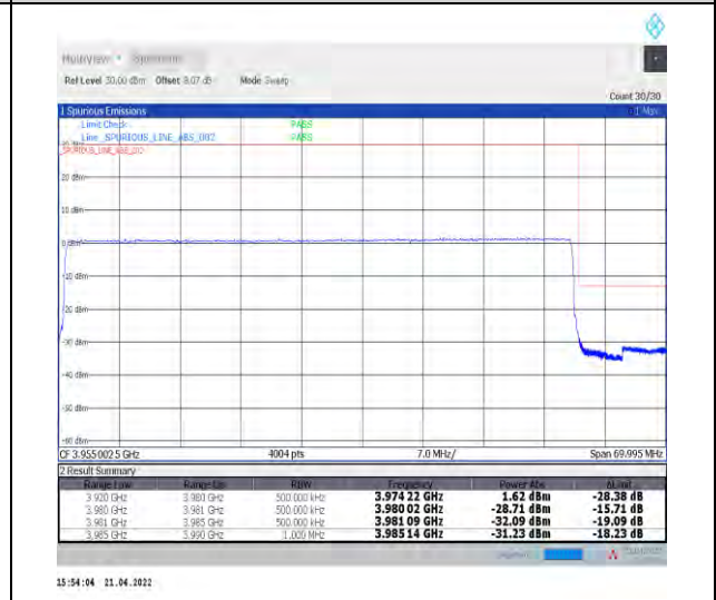
1-N77-3700-3980--30-60-H-6-CP-QPSK-Outer_Full-162@0-Ant1-PASS-see graph
