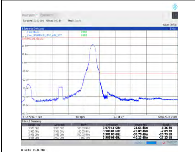
1-N77-3700-3980--30-10-H-5-CP-QPSK-Edge_1RB_Right-1@23-Ant1-PASS-see graph
