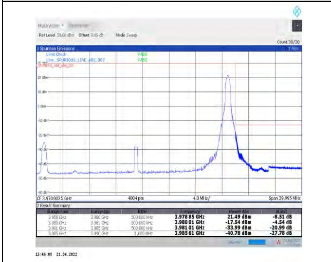
1-N77-3700-3980--30-30-H-5-CP-QPSK-Edge_1RB_Right-1@77-Ant1-PASS-see graph
