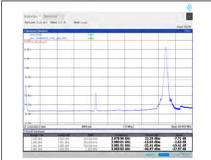
1-N77-3700-3980--30-60-H-2-DFT-PI2BPSK-Edge_1R_B_Right-1@161-Ant1-PASS-see graph
