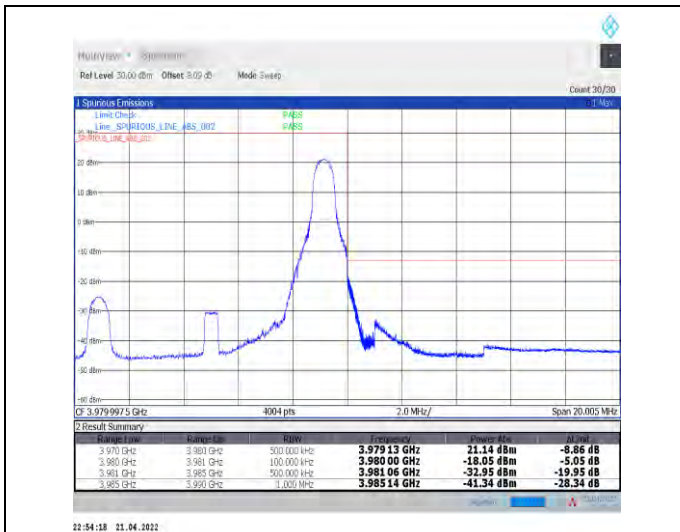
1-N77-3700-3980--30-10-H-2-DFT-PI2BPSK-Edge_1R_B_Right-1@23-Ant1-PASS-see graph
