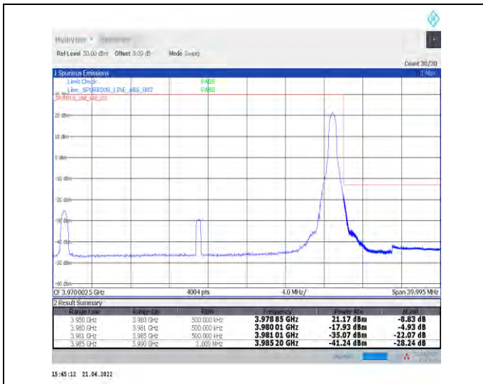
1-N77-3700-3980--30-30-H-2-DFT-PI2BPSK-Edge_1R_B_Right-1@77-Ant1-PASS-see graph
