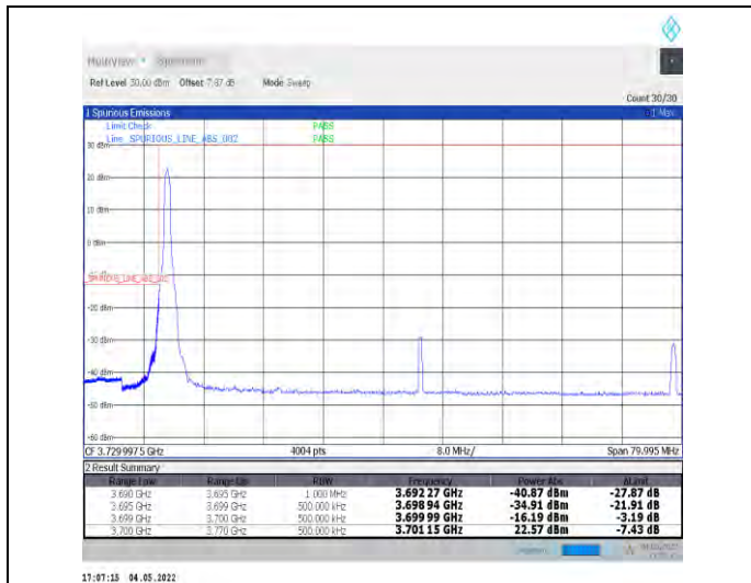
1-N77-3700-3980--30-70-L-1-DFT-PI2BPSK-Edge_1R B_Left-1@0-Ant1-PASS-see graph
