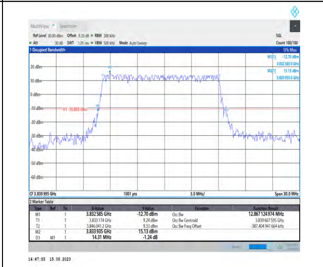
1-N77-3700-3980-PC1-30-15-M-4-DFT-64QAM-Outer_Full-36@0-Ant1-12.867-14.310-≤15-PASS
