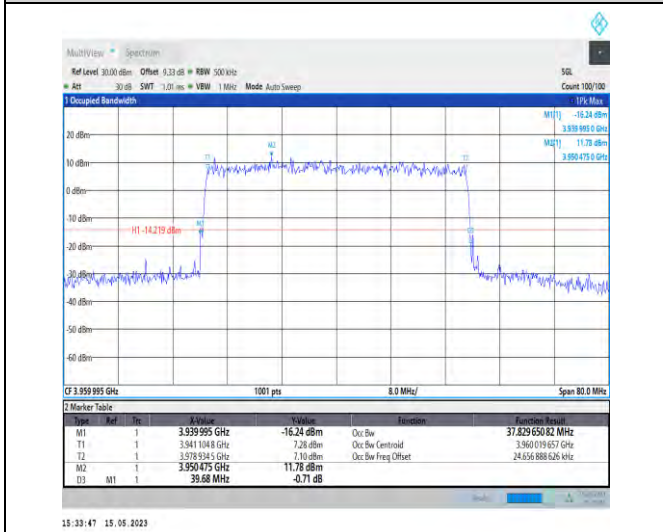
1-N77-3700-3980-PC1-30-40-H-9-CP-256QAM-Outer_Full-106@0-Ant1-37.83-39.680-≤40-PASS
