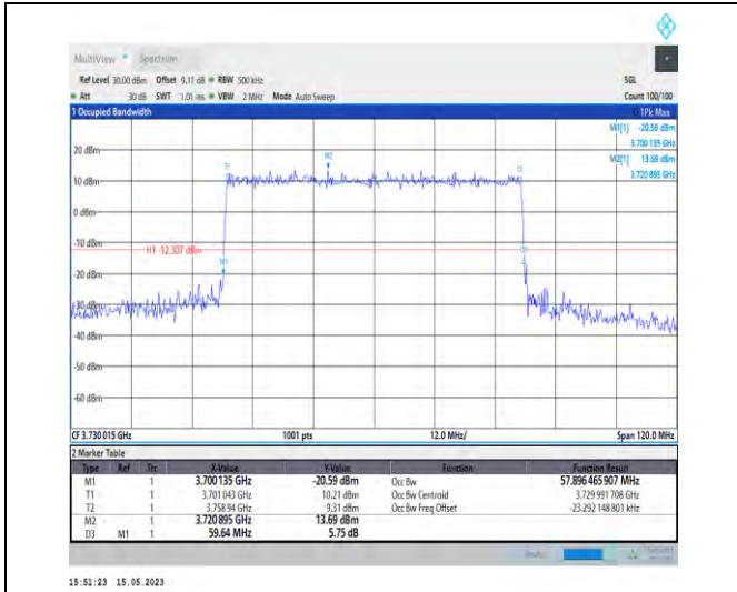
1-N77-3700-3980-PC1-30-60-L-3-DFT-16QAM-Outer_Full-162@0-Ant1-57.896-59.640-≤60-PASS
