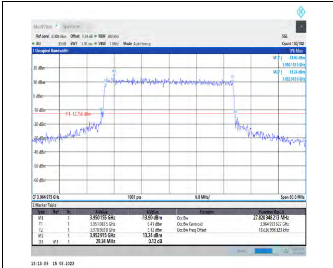
1-N77-3700-3980-PC1-30-30-H-6-CP-QPSK-Outer_Full-78@0-Ant1-27.82-29.340-≤30-PASS
