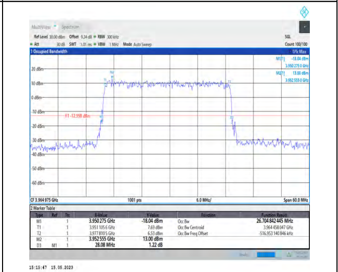
1-N77-3700-3980-PC1-30-30-H-5-DFT-256QAM-Out er_Full-75@0-Ant1-26.705-28.080-≤30-PASS
