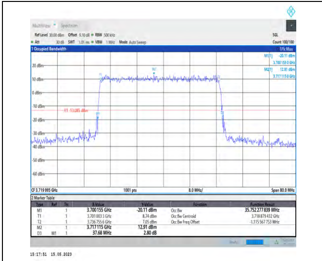
1-N77-3700-3980-PC1-30-40-L-5-DFT-256QAM-Out er_Full-100@0-Ant1-35.752-37.680-≤40-PASS
