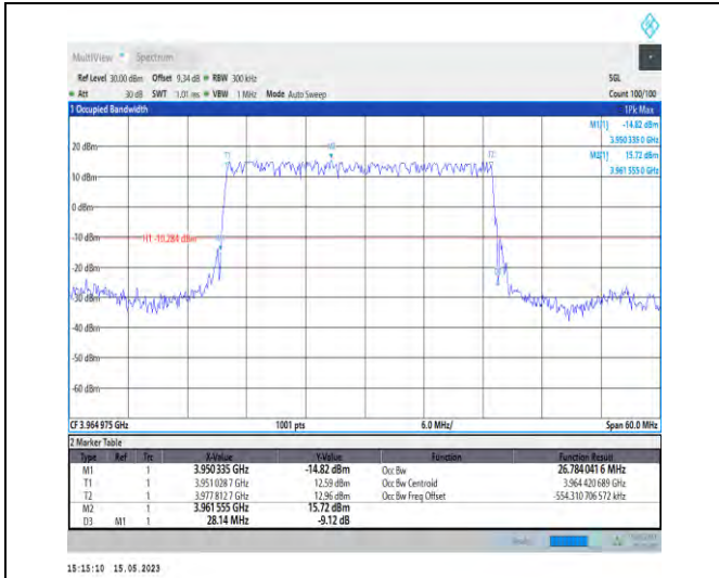
1-N77-3700-3980-PC1-30-30-H-2-DFT-PI2BPSK-Out er_Full-75@0-Ant1-26.784-28.140-≤30-PASS
