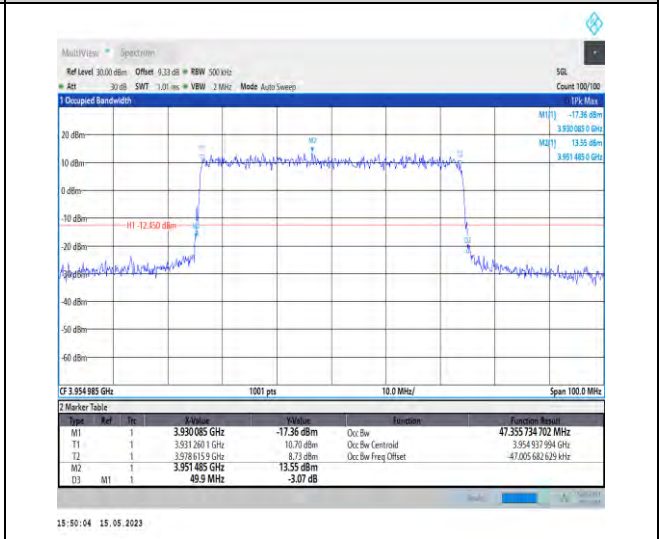
1-N77-3700-3980-PC1-30-50-H-7-CP-16QAM-Outer_Full-133@0-Ant1-47.356-49.900-≤50-PASS
