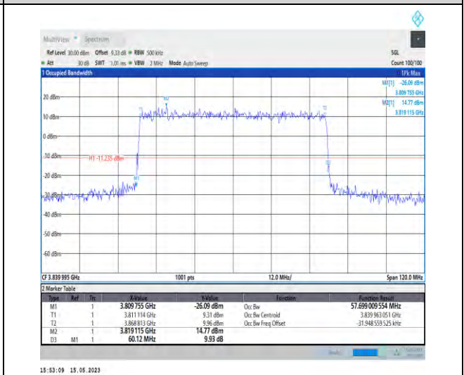
1-N77-3700-3980-PC1-30-60-M-1-DFT-QPSK-Outer_Full-162@0-Ant1-57.699-60.120-≤60-PASS
