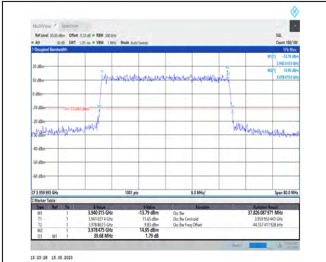
1-N77-3700-3980-PC1-30-40-H-7-CP-16QAM-Outer_Full-106@0-Ant1-37.826-39.680-≤40-PASS
