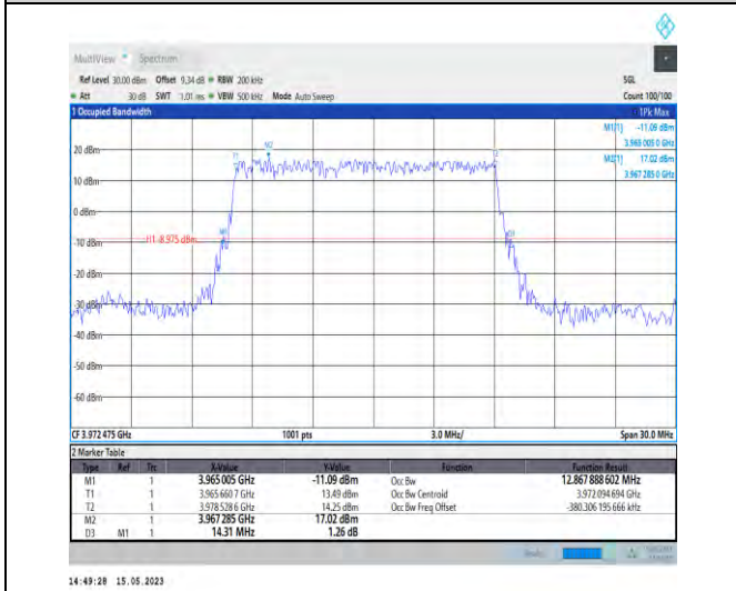
1-N77-3700-3980-PC1-30-15-H-2-DFT-PI2BPSK-Outer_Full-36@0-Ant1-12.868-14.310-≤15-PASS
