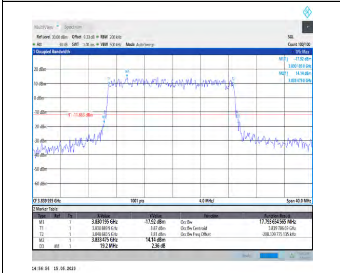
1-N77-3700-3980-PC1-30-20-M-4-DFT-64QAM-Outer_Full-50@0-Ant1-17.794-19.200-≤20-PASS
