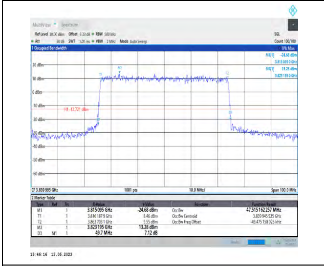
1-N77-3700-3980-PC1-30-50-M-7-CP-16QAM-Outer_Full-133@0-Ant1-47.515-49.700-≤50-PASS
