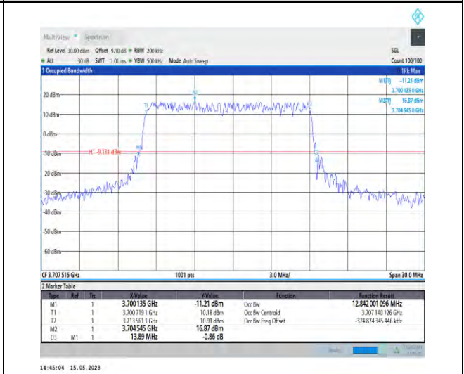
1-N77-3700-3980-PC1-30-15-L-1-DFT-QPSK-Outer_Full-36@0-Ant1-12.842-13.890-≤15-PASS
