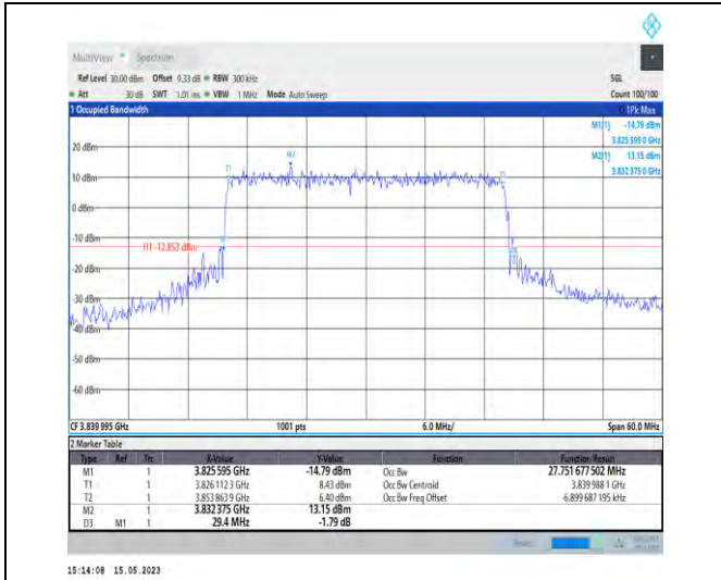
1-N77-3700-3980-PC1-30-30-M-7-CP-16QAM-Outer _Full-78@0-Ant1-27.752-29.400-≤30-PASS
