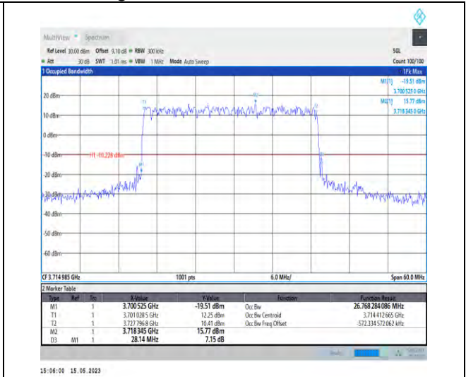
1-N77-3700-3980-PC1-30-30-L-1-DFT-QPSK-Outer_Full-75@0-Ant1-26.768-28.140-≤30-PASS
