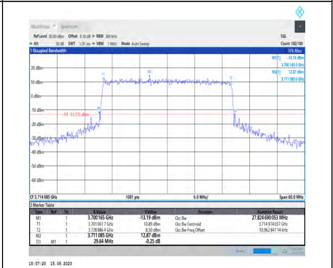
1-N77-3700-3980-PC1-30-30-L-7-CP-16QAM-Outer_Full-78@0-Ant1-27.825-29.640-≤30-PASS
