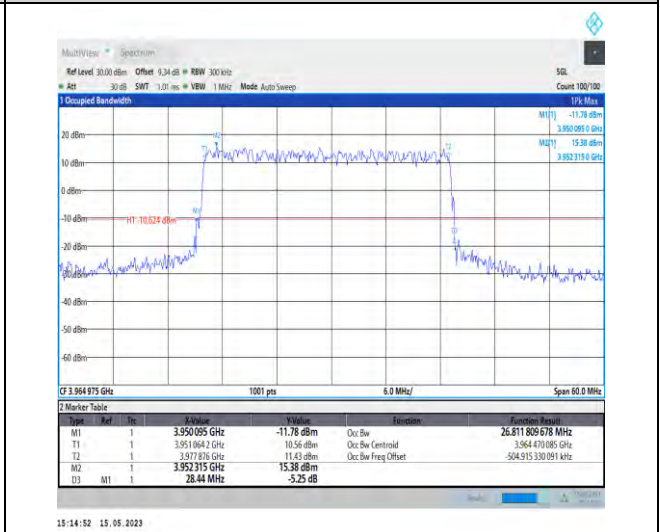
1-N77-3700-3980-PC1-30-30-H-1-DFT-QPSK-Outer _Full-75@0-Ant1-26.812-28.440-≤30-PASS
