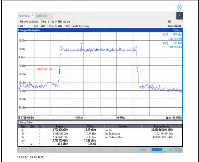
1-N77-3700-3980-PC1-30-50-L-5-DFT-256QAM-Outer_Full-128@0-Ant1-45.63-47.300-<math>\leq 50</math>-PASS
