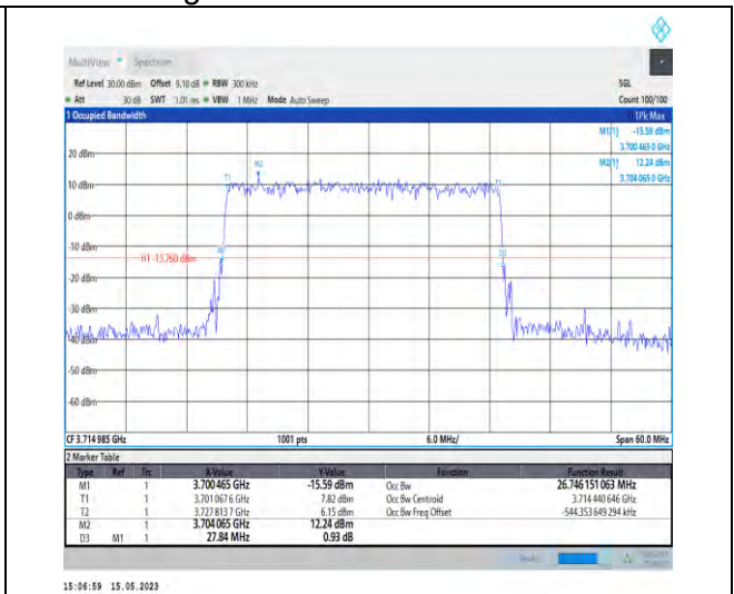
1-N77-3700-3980-PC1-30-30-L-5-DFT-256QAM-Outer_Full-75@0-Ant1-26.746-27.840-≤30-PASS
