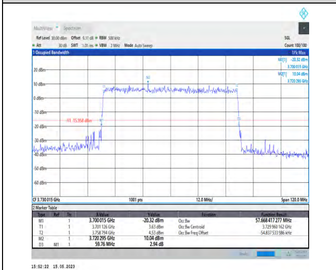
1-N77-3700-3980-PC1-30-60-L-9-CP-256QAM-Outer_Full-162@0-Ant1-57.668-59.760-≤60-PASS
