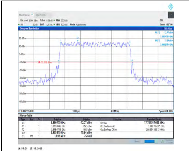
1-N77-3700-3980-PC1-30-20-M-2-DFT-PI2BPSK-Outer_Full-50@0-Ant1-17.782-18.920-≤20-PASS
