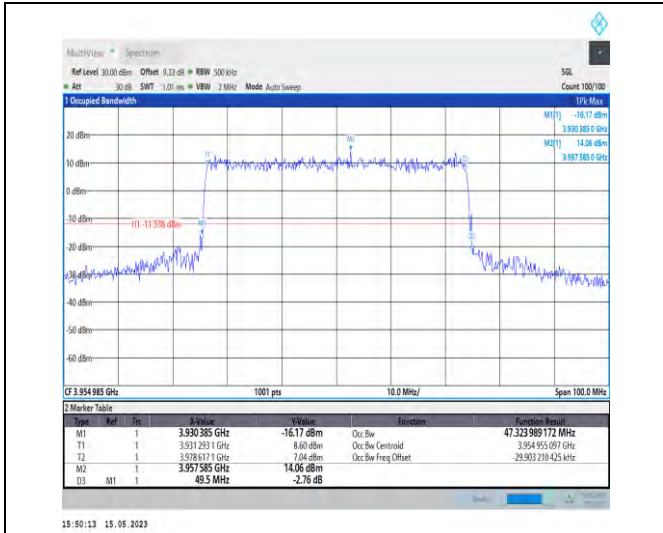
1-N77-3700-3980-PC1-30-50-H-8-CP-64QAM-Outer_Full-133@0-Ant1-47.324-49.500-≤50-PASS
