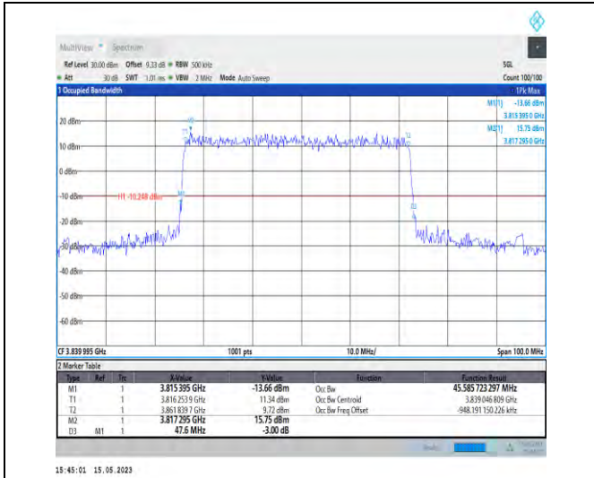
1-N77-3700-3980-PC1-30-50-M-1-DFT-QPSK-Outer_Full-128@0-Ant1-45.586-47.600-≤50-PASS
