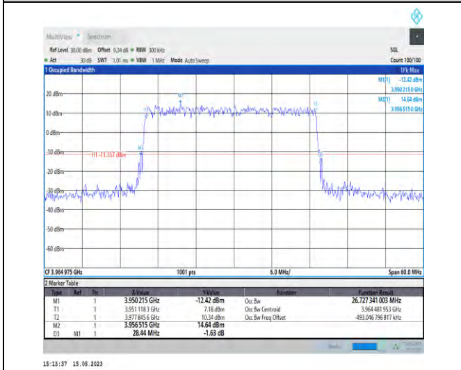
1-N77-3700-3980-PC1-30-30-H-4-DFT-64QAM-Out er_Full-75@0-Ant1-26.727-28.440-≤30-PASS
