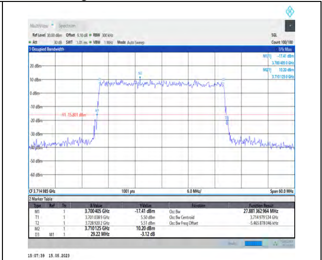
1-N77-3700-3980-PC1-30-30-L-9-CP-256QAM-Outer_Full-78@0-Ant1-27.881-29.220-≤30-PASS
