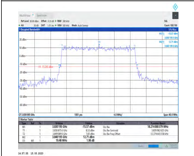
1-N77-3700-3980-PC1-30-20-M-8-CP-64QAM-Outer_Full-51@0-Ant1-18.214-19.480-≤20-PASS
