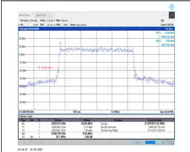
1-N77-3700-3980-PC1-30-30-M-9-CP-256QAM-Outer _Full-78@0-Ant1-27.88-29.100-≤30-PASS
