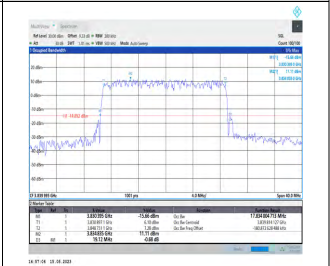
1-N77-3700-3980-PC1-30-20-M-5-DFT-256QAM-Outer_Full-50@0-Ant1-17.834-19.120-≤20-PASS
