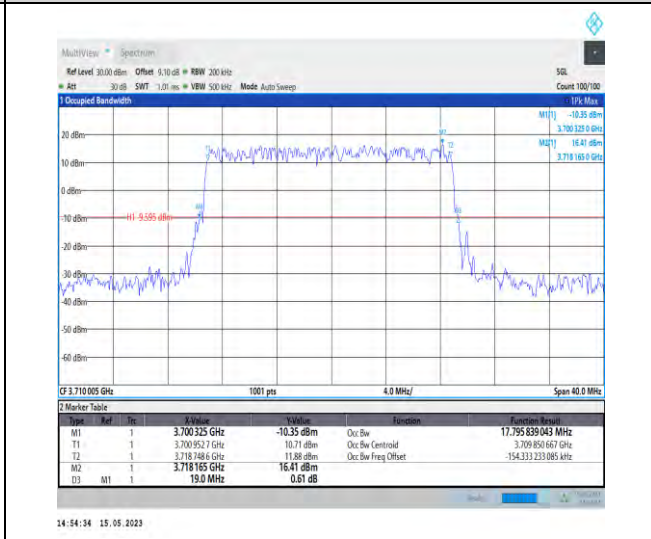
1-N77-3700-3980-PC1-30-20-L-2-DFT-PI2BPSK-Outer_Full-50@0-Ant1-17.796-19.000-≤20-PASS
