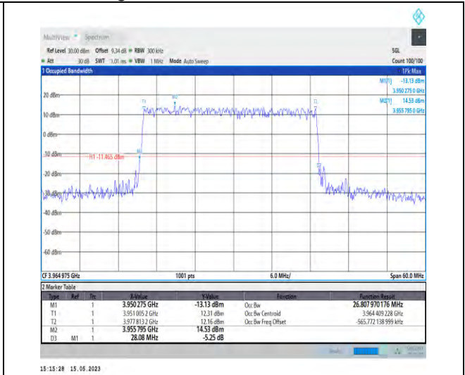
1-N77-3700-3980-PC1-30-30-H-3-DFT-16QAM-Out er_Full-75@0-Ant1-26.808-28.080-≤30-PASS
