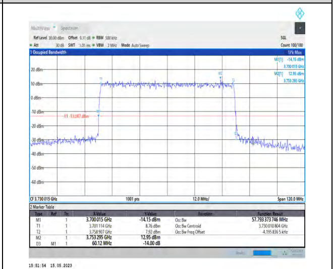
1-N77-3700-3980-PC1-30-60-L-6-CP-QPSK-Outer_Full-162@0-Ant1-57.793-60.120-≤60-PASS
