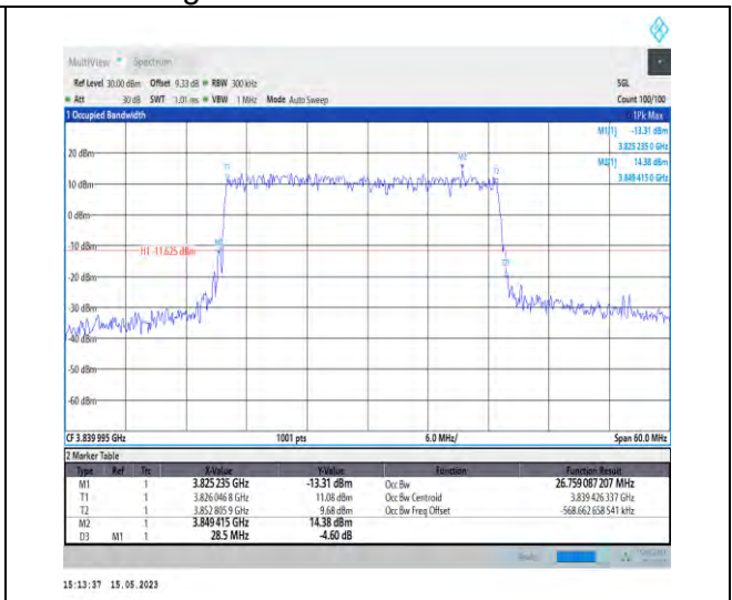
1-N77-3700-3980-PC1-30-30-M-4-DFT-64QAM-Outer_Full-75@0-Ant1-26.759-28.500-≤30-PASS
