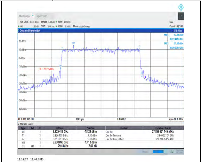
1-N77-3700-3980-PC1-30-30-M-8-CP-64QAM-Outer _Full-78@0-Ant1-27.854-29.400-≤30-PASS
