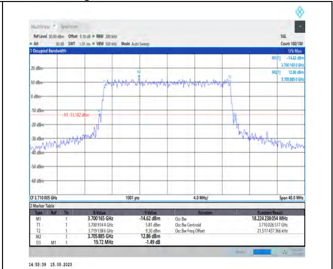
1-N77-3700-3980-PC1-30-20-L-8-CP-64QAM-Outer_Full-51@0-Ant1-18.224-19.720-≤20-PASS
