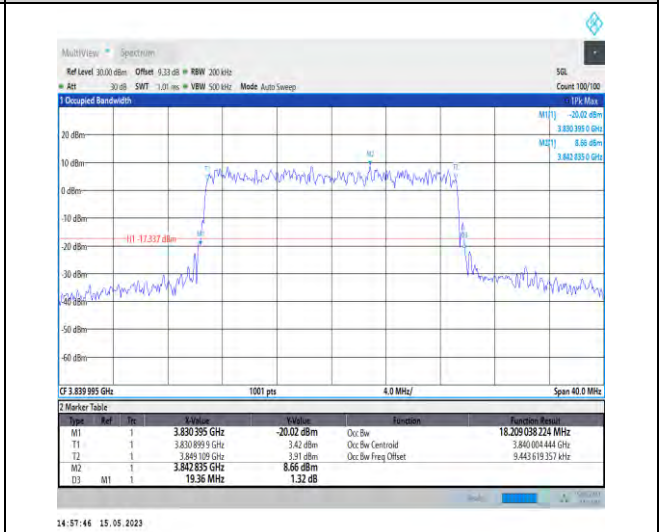
1-N77-3700-3980-PC1-30-20-M-9-CP-256QAM-Outer_Full-51@0-Ant1-18.209-19.360-≤20-PASS
