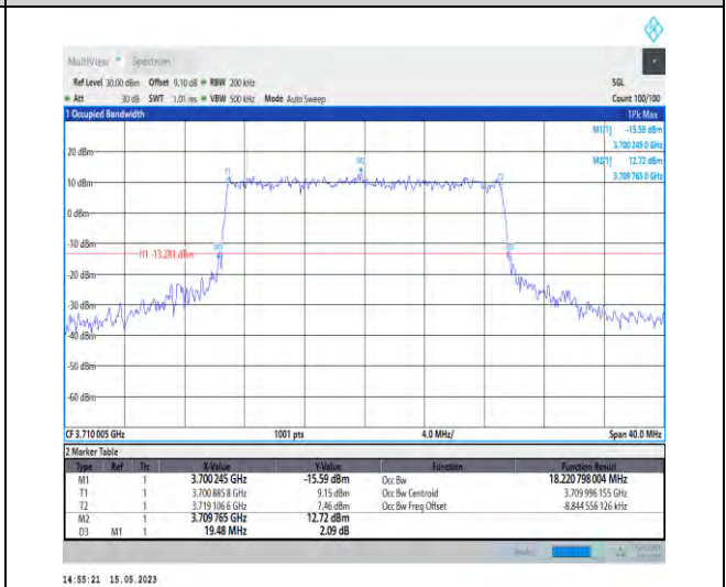
1-N77-3700-3980-PC1-30-20-L-6-CP-QPSK-Outer_Full-51@0-Ant1-18.221-19.480-≤20-PASS
