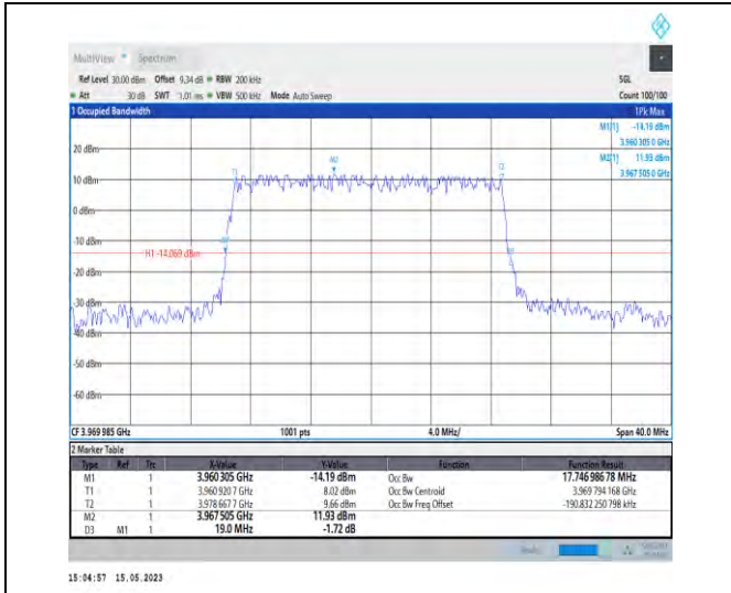
1-N77-3700-3980-PC1-30-20-H-5-DFT-256QAM-Out_er_Full-50@0-Ant1-17.747-19.000-≤20-PASS
