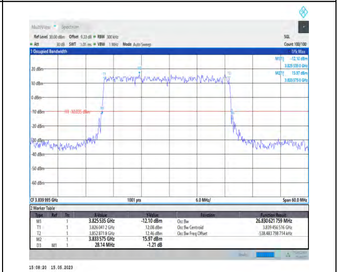
1-N77-3700-3980-PC1-30-30-M-2-DFT-PI2BPSK-Outer_Full-75@0-Ant1-26.831-28.140-≤30-PASS
