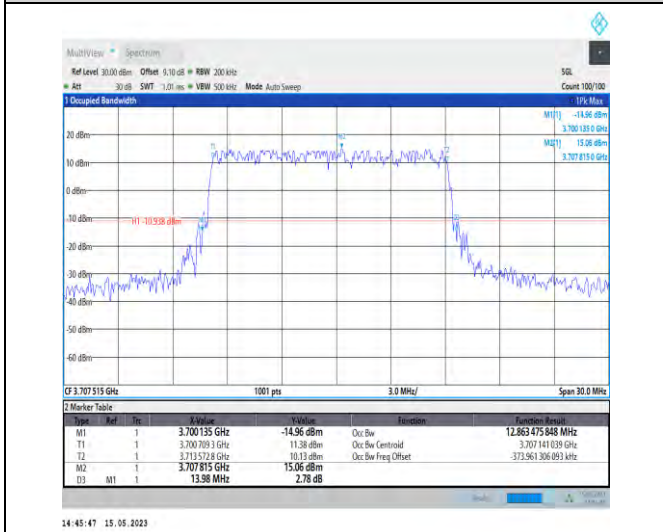
1-N77-3700-3980-PC1-30-15-L-4-DFT-64QAM-Outer_Full-36@0-Ant1-12.863-13.980-≤15-PASS
