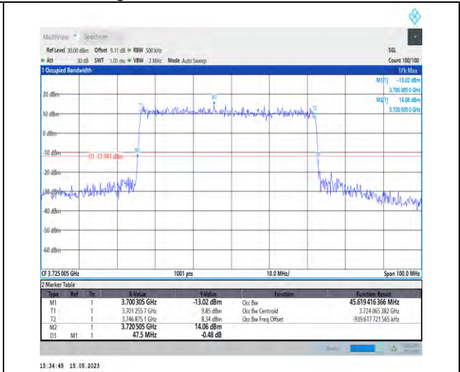
1-N77-3700-3980-PC1-30-50-L-3-DFT-16QAM-Outer_Full-128@0-Ant1-45.619-47.500-<math>\leq 50</math>-PASS
