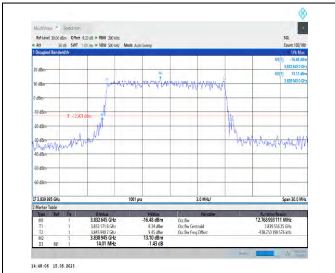
1-N77-3700-3980-PC1-30-15-M-5-DFT-256QAM-Out_er_Full-36@0-Ant1-12.769-14.010-≤15-PASS
