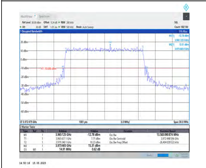
1-N77-3700-3980-PC1-30-15-H-6-CP-QPSK-Outer_Full-38@0-Ant1-13.583-14.910-≤15-PASS
