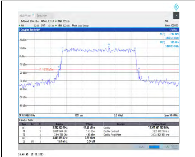
1-N77-3700-3980-PC1-30-15-M-9-CP-256QAM-Outer_Full-38@0-Ant1-13.572-15.000-≤15-PASS
