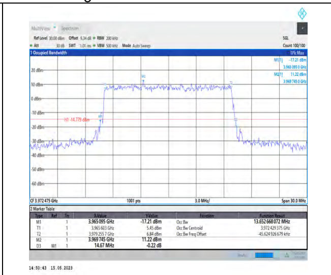
1-N77-3700-3980-PC1-30-15-H-9-CP-256QAM-Outer_Full-38@0-Ant1-13.653-14.670-≤15-PASS
