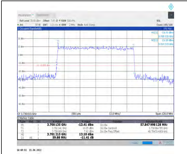
1-N77-3700-3980--30-60-L-3-DFT-16QAM-Outer_Fu II-162@0-Ant1-57.848-59.880-<math>\leq 60</math>-PASS
