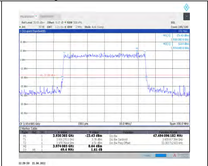
1-N77-3700-3980--30-50-H-9-CP-256QAM-Outer_Fu ll-133@0-Ant1-47.494-49.400-<math>\leq 50</math>-PASS
