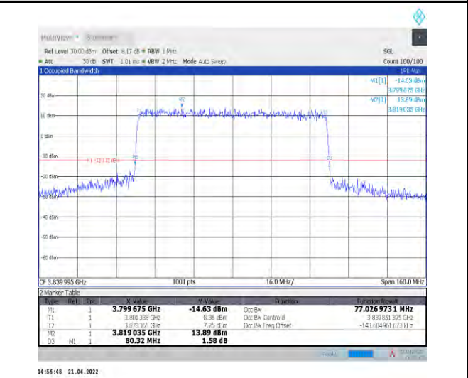
1-N77-3700-3980--30-80-M-3-DFT-16QAM-Outer_Fu II-216@0-Ant1-77.027-80.320-<math>\leq 80</math>-PASS
