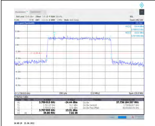
1-N77-3700-3980--30-60-L-1-DFT-QPSK-Outer_Full -162@0-Ant1-57.736-59.880-<math>\leq 60</math>-PASS
