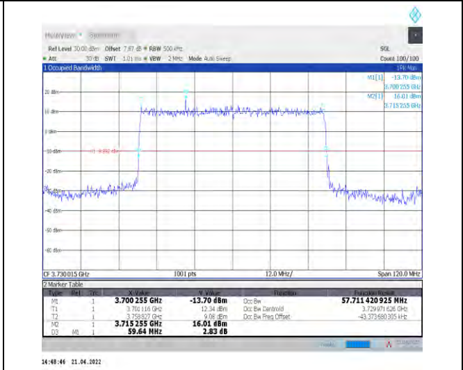
1-N77-3700-3980--30-60-L-2-DFT-PI2BPSK-Outer_F ull-162@0-Ant1-57.711-59.640-<math>\leq 60</math>-PASS
