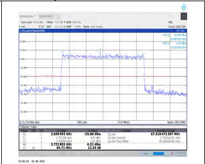
1-N77-3700-3980--30-70-L-9-CP-256QAM-Outer_Ful I-189@0-Ant1-67.518-69.720-<math>\leq 70</math>-PASS
