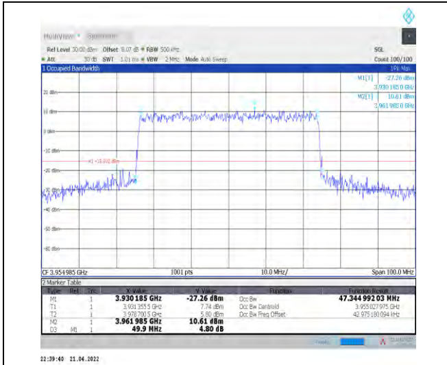
1-N77-3700-3980--30-50-H-8-CP-64QAM-Outer_Full -133@0-Ant1-47.345-49.900-<math>\leq 50</math>-PASS
