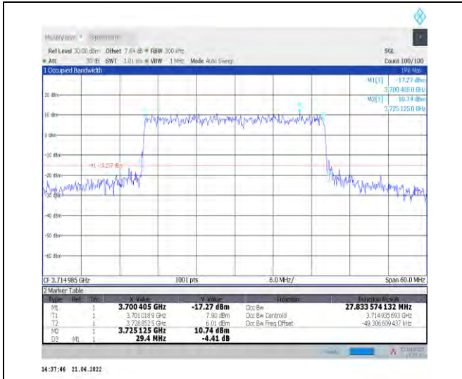
1-N77-3700-3980--30-30-L-8-CP-64QAM-Outer_Full -78@0-Ant1-27.833-29.400-<30-PASS
