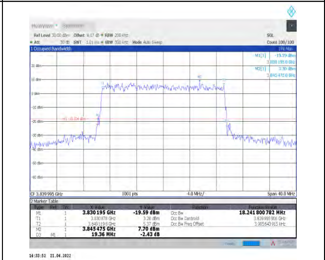
1-N77-3700-3980--30-20-M-9-CP-256QAM-Outer_Full-51@0-Ant1-18.242-19.360-≤20-PASS
