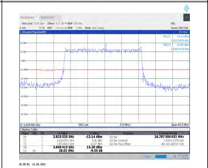
1-N77-3700-3980--30-30-M-2-DFT-PI2BPSK-Outer_Full Full-75@0-Ant1-26.71-28.020-<30-PASS
