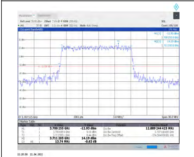
1-N77-3700-3980--30-15-L-4-DFT-64QAM-Outer_Full-36@0-Ant1-12.889-13.740-≤15-PASS
