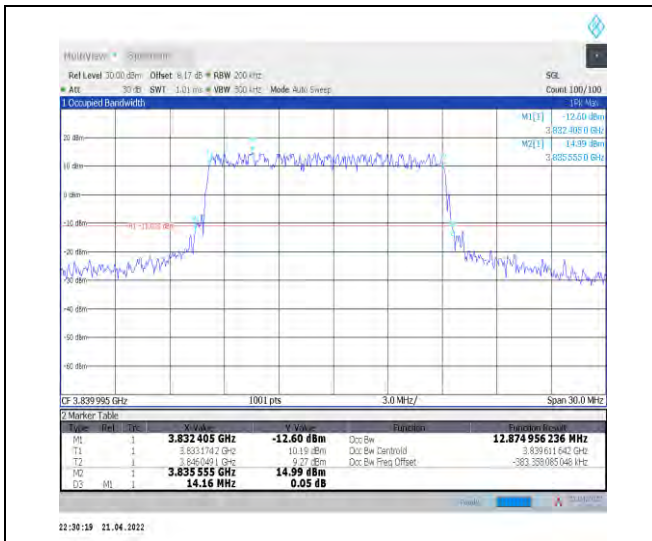
1-N77-3700-3980--30-15-M-1-DFT-QPSK-Outer_Full -36@0-Ant1-12.875-14.160≤15-PASS
