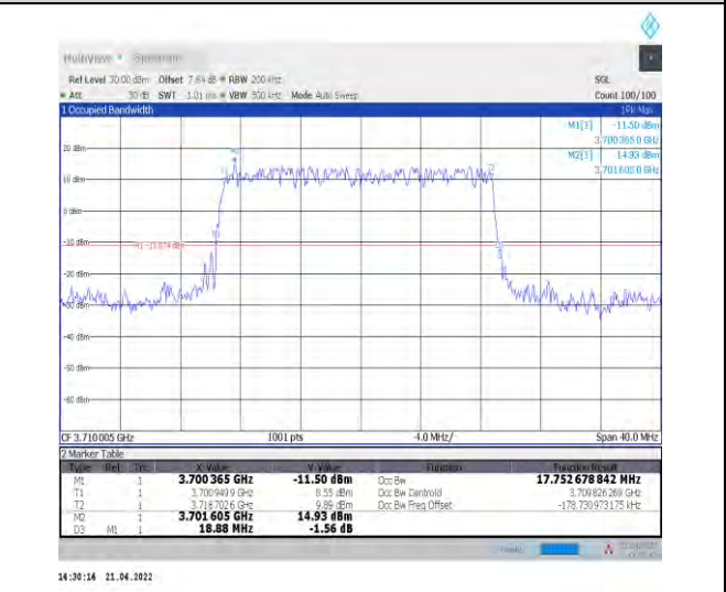
1-N77-3700-3980--30-20-L-2-DFT-PI2BPSK-Outer_Full ull-50@0-Ant1-17.753-18.880-≤20-PASS
