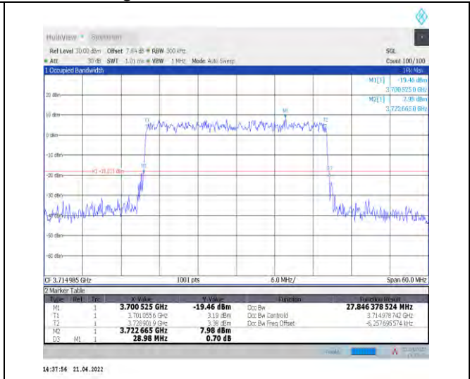
1-N77-3700-3980--30-30-L-9-CP-256QAM-Outer_Ful I-78@0-Ant1-27.852-28.980-<30-PASS
