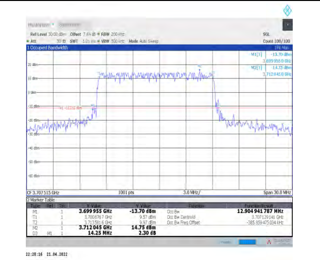
1-N77-3700-3980--30-15-L-1-DFT-QPSK-Outer_Full- 36@0-Ant1-12.905-14.250-≤15-PASS
