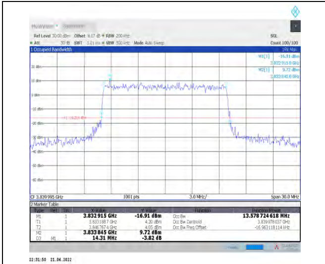
1-N77-3700-3980--30-15-M-9-CP-256QAM-Outer_Full-38@0-Ant1-13.579-14.310-≤15-PASS
