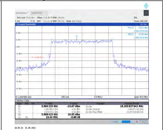
1-N77-3700-3980--30-20-H-6-CP-QPSK-Outer_Full-51@0-Ant1-18.206-19.440-<=20-PASS
