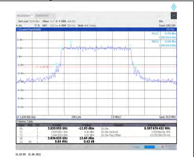
1-N77-3700-3980--30-10-M-1-DFT-QPSK-Outer_Full -24@0-Ant1-8.598-9.840-<=10-PASS
