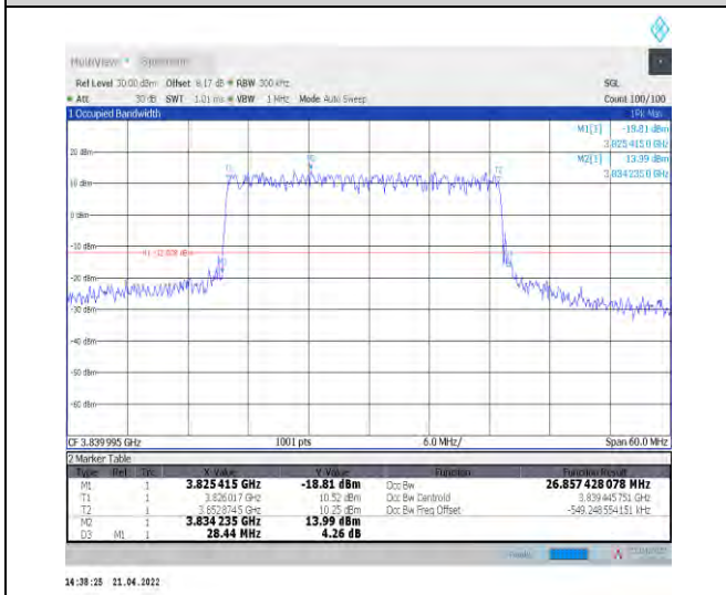
1-N77-3700-3980--30-30-M-1-DFT-QPSK-Outer_Full -75@0-Ant1-26.857-28.440-<30-PASS
