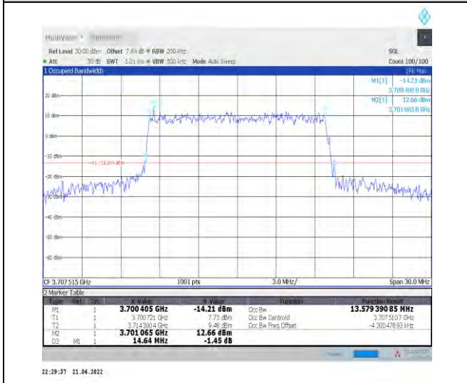
1-N77-3700-3980--30-15-L-8-CP-64QAM-Outer_Full-38@0-Ant1-13.579-14.640-≤15-PASS
