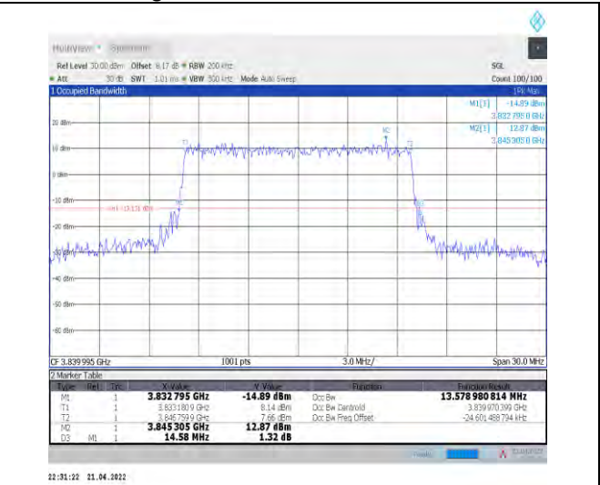
1-N77-3700-3980--30-15-M-6-CP-QPSK-Outer_Full-38@0-Ant1-13.579-14.580-≤15-PASS
