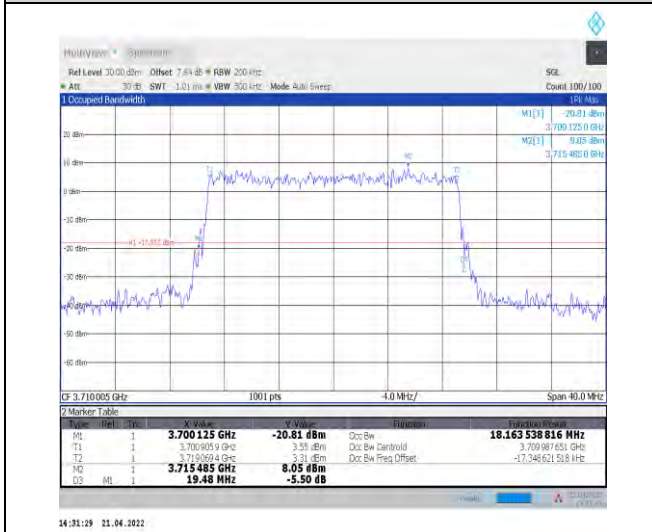
1-N77-3700-3980--30-20-L-9-CP-256QAM-Outer_Fu ll-51@0-Ant1-18.164-19.480-≤20-PASS
