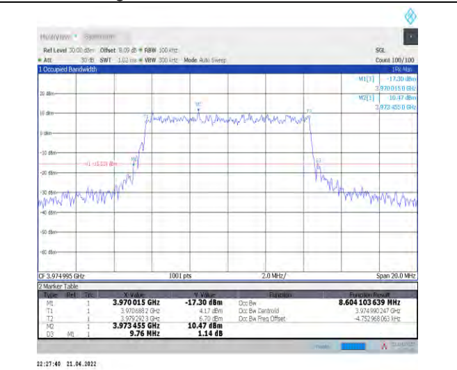
1-N77-3700-3980--30-10-H-8-CP-64QAM-Outer_Full -24@0-Ant1-8.604-9.760-≤10-PASS
