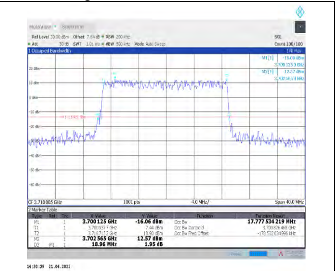
1-N77-3700-3980--30-20-L-4-DFT-64QAM-Outer_Full-50@0-Ant1-17.778-18.960-≤20-PASS
