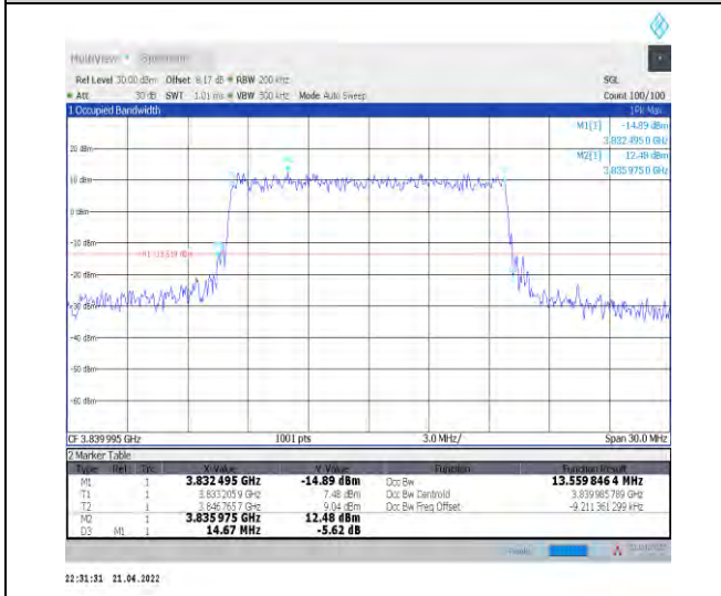
1-N77-3700-3980--30-15-M-7-CP-16QAM-Outer_Full-38@0-Ant1-13.56-14.670-≤15-PASS
