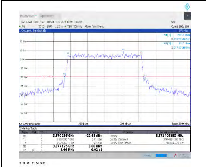
1-N77-3700-3980--30-10-H-9-CP-256QAM-Outer_F ull-24@0-Ant1-8.571-9.460-≤10-PASS
