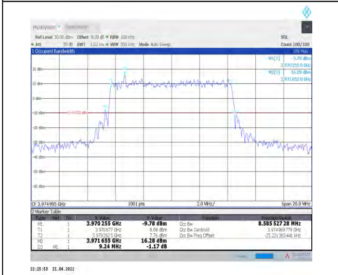
1-N77-3700-3980--30-10-H-1-DFT-QPSK-Outer_Full-24@0-Ant1-8.586-9.240-≤10-PASS
