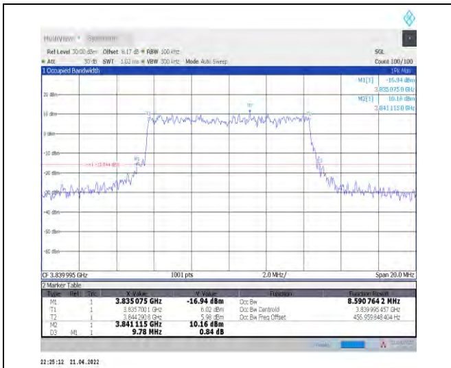
1-N77-3700-3980--30-10-M-8-CP-64QAM-Outer_Ful I-24@0-Ant1-8.591-9.780-≤10-PASS
