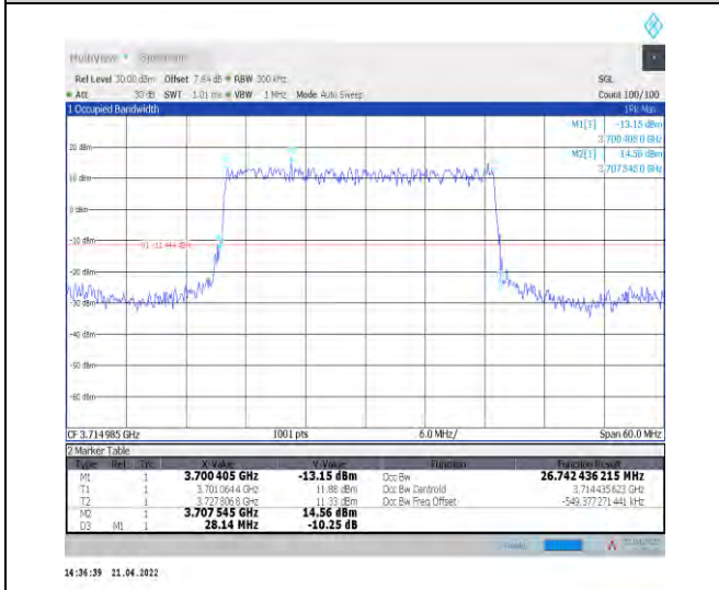
1-N77-3700-3980--30-30-L-2-DFT-PI2BPSK-Outer_Full-75@0-Ant1-26.744-28.140-≤30-PASS
