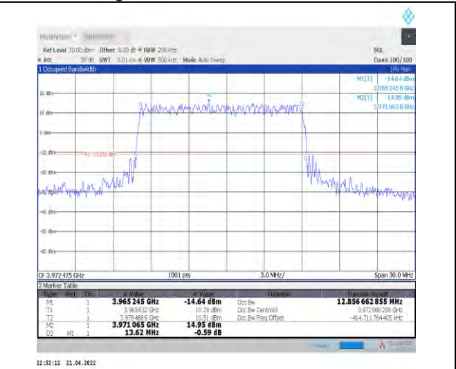
1-N77-3700-3980--30-15-H-1-DFT-QPSK-Outer_Full-36@0-Ant1-12.857-13.620-≤15-PASS
