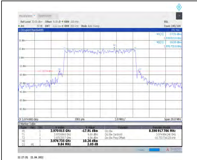
1-N77-3700-3980--30-10-H-7-CP-16QAM-Outer_Full -24@0-Ant1-8.599-9.840-≤10-PASS
