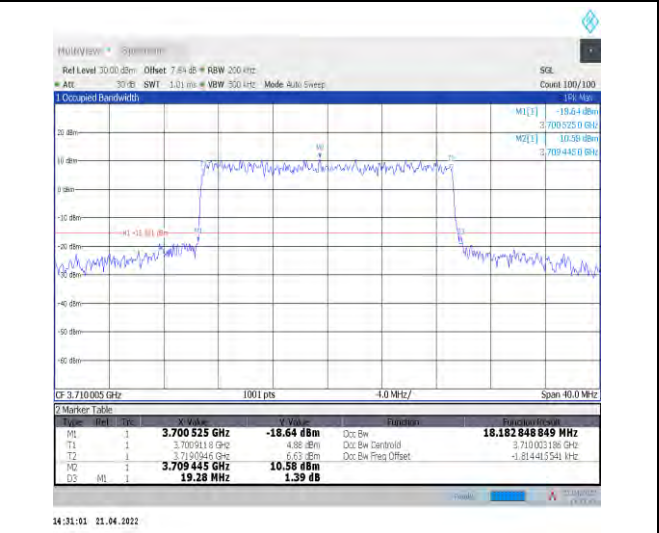
1-N77-3700-3980--30-20-L-6-CP-QPSK-Outer_Full-50@0-Ant1-18.183-19.280-≤20-PASS
