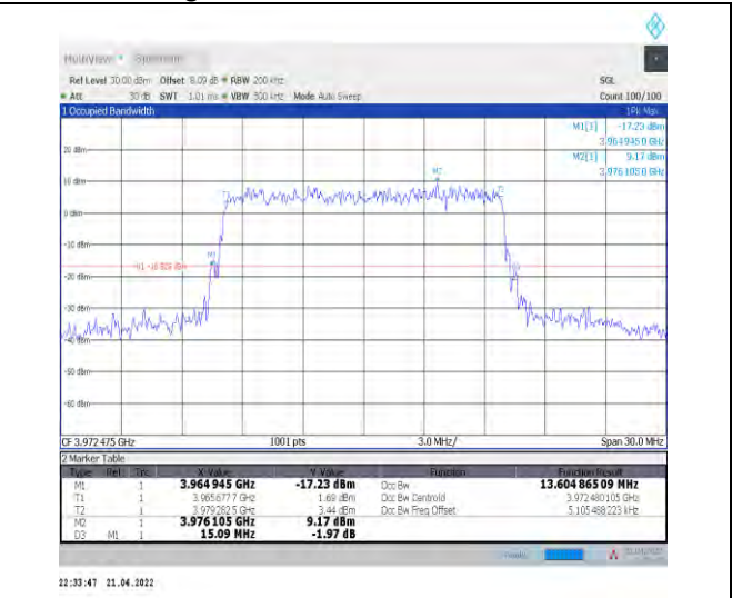
1-N77-3700-3980--30-15-H-9-CP-256QAM-Outer_Fu II-38@0-Ant1-13.605-15.090-≤15-PASS
