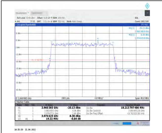
1-N77-3700-3980--30-20-H-9-CP-256QAM-Outer_Full-51@0-Ant1-18.214-19.320-≤20-PASS
