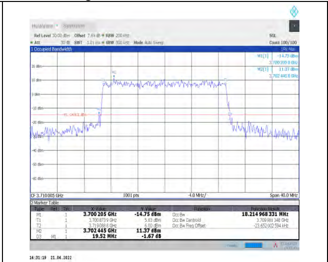
1-N77-3700-3980--30-20-L-8-CP-64QAM-Outer_Full 51@0-Ant1-18.215-19.520-≤20-PASS
