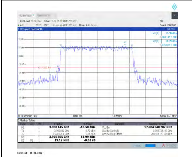
1-N77-3700-3980--30-20-H-3-DFT-16QAM-Outer_Full Full-50@0-Ant1-17.804-19.120-≤20-PASS
