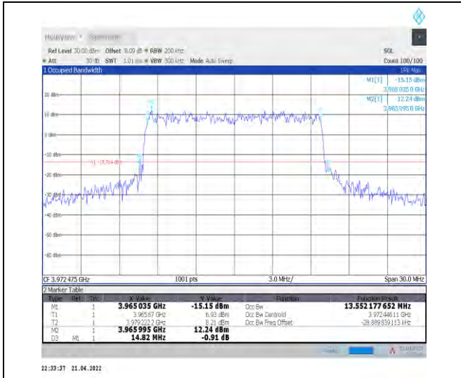
1-N77-3700-3980--30-15-H-8-CP-64QAM-Outer_Full -38@0-Ant1-13.552-14.820-≤15-PASS
