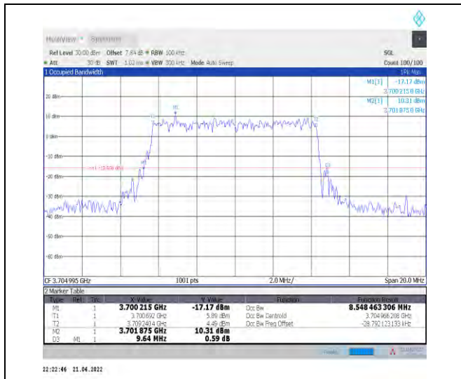
1-N77-3700-3980--30-10-L-5-DFT-256QAM-Outer_Full-24@0-Ant1-8.548-9.640-≤10-PASS
