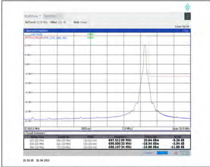
1-N71--15-15-H-2-DFT-PI2BPSK-Edge_1RB_Right-1@78-Ant1-PASS-see graph
