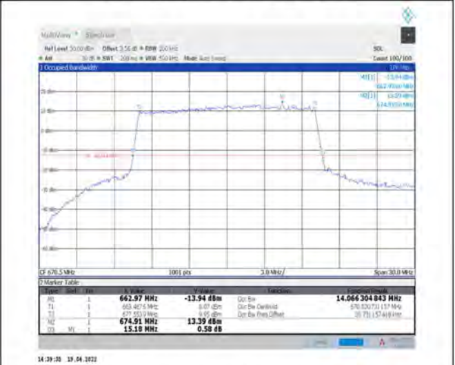
1-N71--15-15-L-6-CP-QPSK-Outer_Full-79@0-Ant1-14.066-15.180-≤15-PASS
