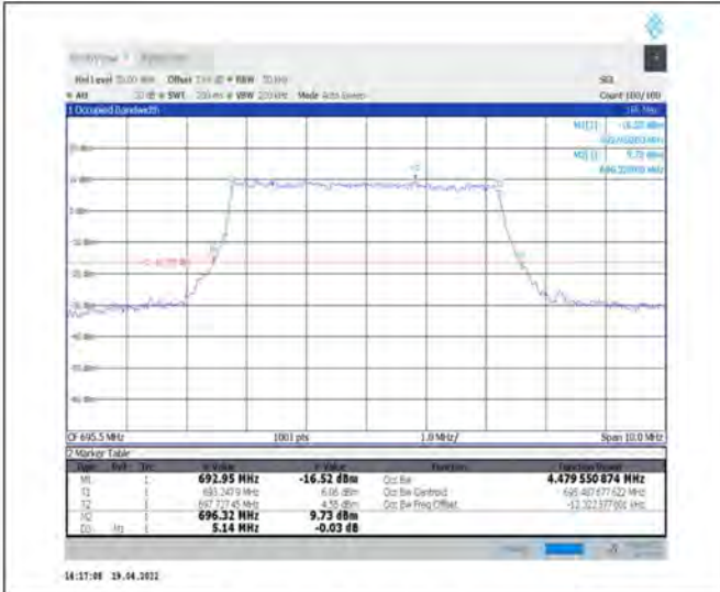
1-N71--15-5-H-7-CP-16QAM-Outer_Full-25@0-Ant1-4.48-5.140-≤5-PASS
