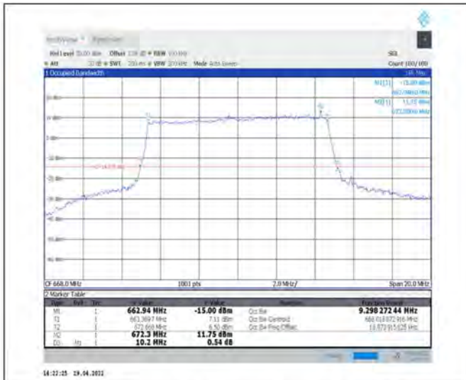
1-N71--15-10-L-6-CP-QPSK-Outer_Full-52@0-Ant1-9.298-10.200-≤10-PASS
