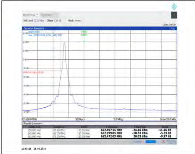
1-N71--15-15-L-1-DFT-PI2BPSK-Edge_1RB_Left-1@0-Ant1-PASS-see graph
