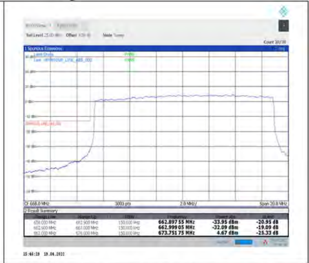
1-N71--15-15-L-3-DFT-PI2BPSK-Outer_Full-75@0-Ant1-PASS-see graph
