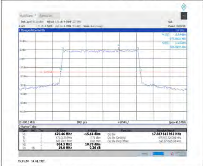
1-N71--15-20-M-5-DFT-256QAM-Outer_Full-100@0-Ant1-17.888-19.000-≤20-PASS
