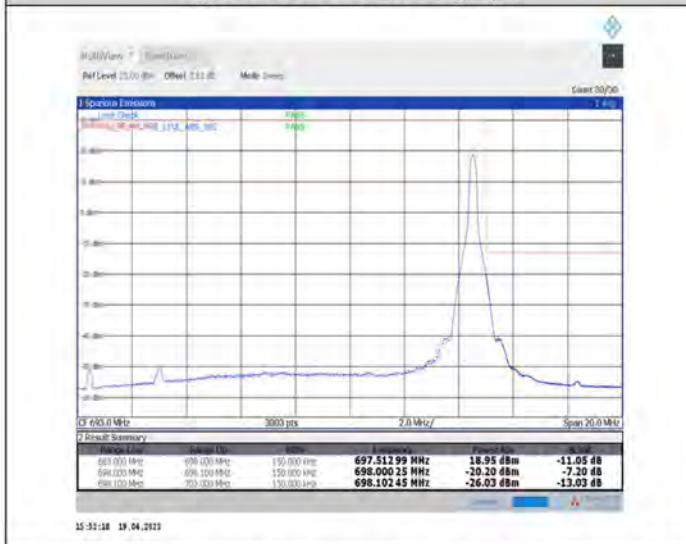
1-N71--15-15-H-5-CP-QPSK-Edge_1RB_Right-1@78-Ant1-PASS-see graph
