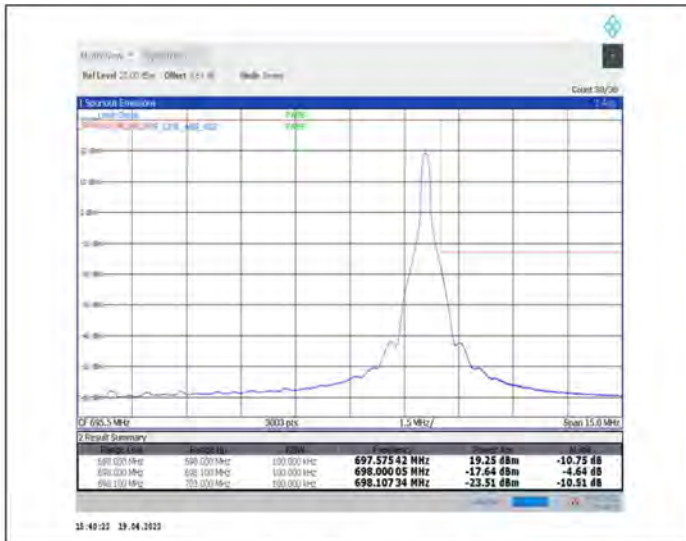
1-N71--15-10-H-2-DFT-PI2BPSK-Edge_1RB_Right-1@51-Ant1-PASS-see graph
