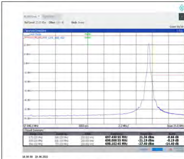
1-N71--15-20-H-2-DFT-PI2BPSK-Edge_1RB_Right-1@105-Ant1-PASS-see graph
