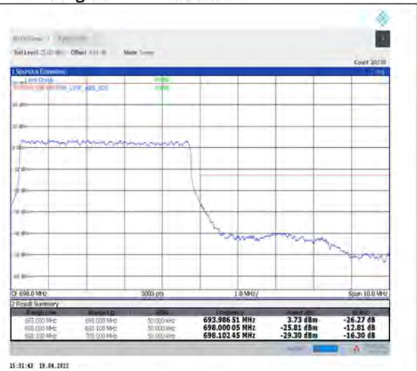
1-N71--15-5-H-3-DFT-PI2BPSK-Outer_Full-25@0-Ant1-PASS-see graph
