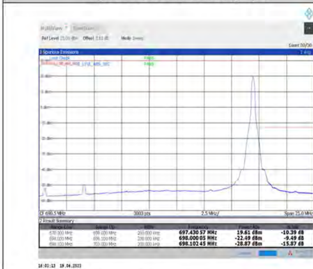
1-N71--15-20-H-5-CP-QPSK-Edge_1RB_Right-1@105-Ant1-PASS-see graph
