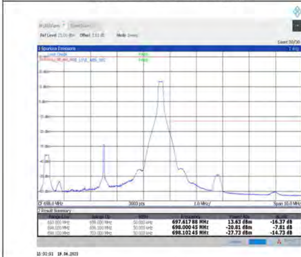
1-N71--15-5-H-5-CP-QPSK-Edge_1RB_Right-1@24-Ant1-PASS-see graph
