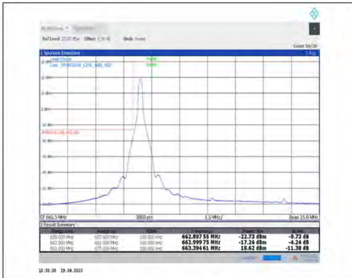
1-N71--15-10-L-1-DFT-PI2BPSK-Edge_1RB_Left-1@0-Ant1-PASS-see graph
