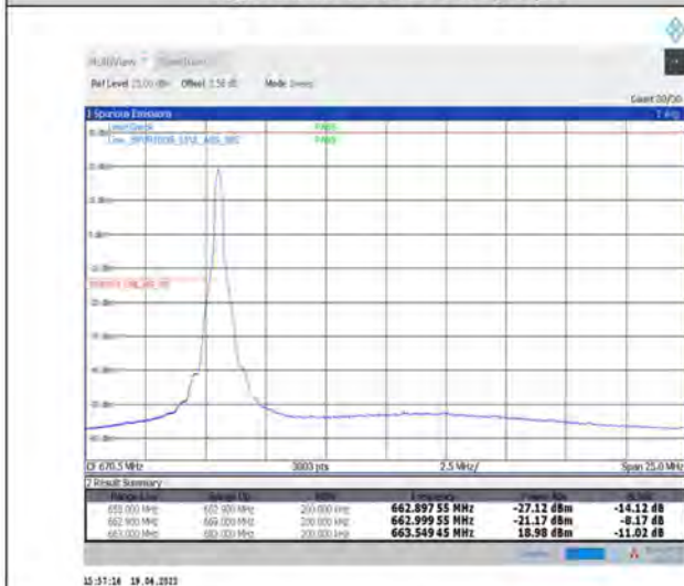
1-N71--15-20-L-4-CP-QPSK-Edge_1RB_Left-1@0-Ant1-PASS-see graph
