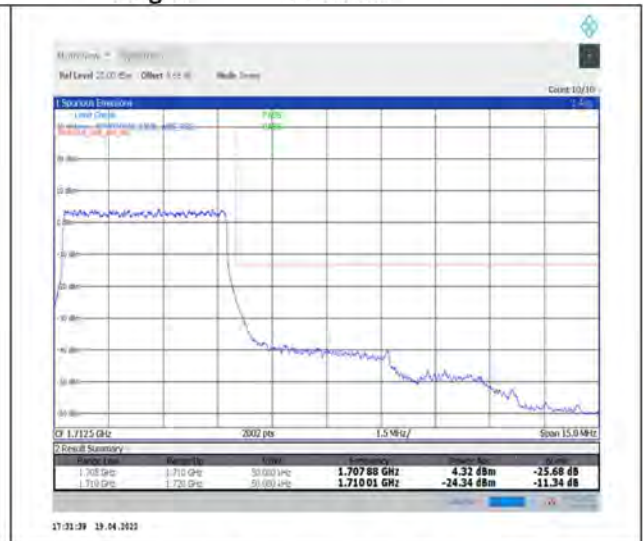
1-N70--15-5-H-3-DFT-PI2BPSK-Outer_Full-25@0-Ant1-seegraph-PASS-see graph
