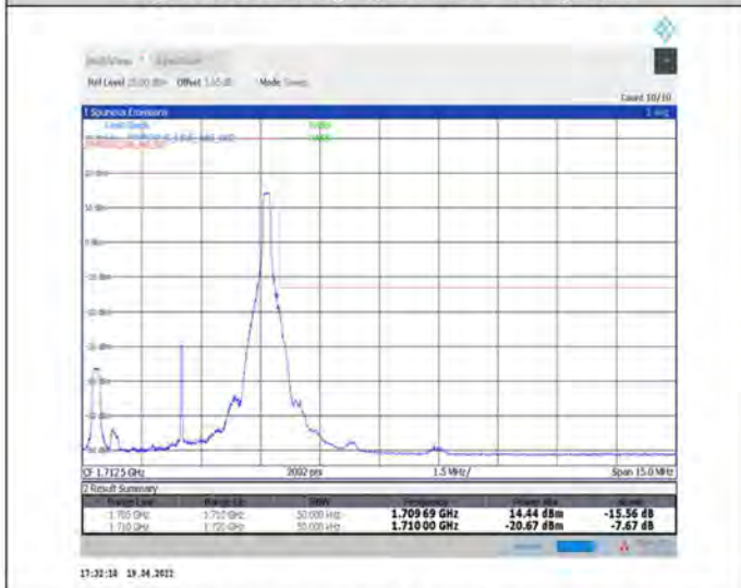
1-N70--15-5-H-5-CP-QPSK-Edge_1RB_Right-1@24-Ant1-seegraph-PASS-see graph
