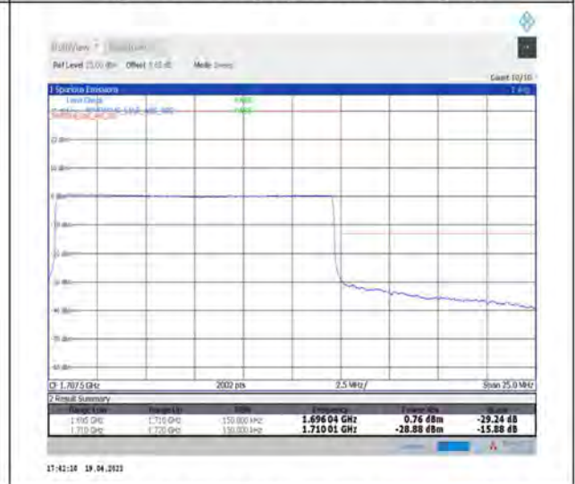
1-N70--15-15-H-6-CP-QPSK-Outer_Full-79@0-Ant1-seegraph-PASS-see graph
