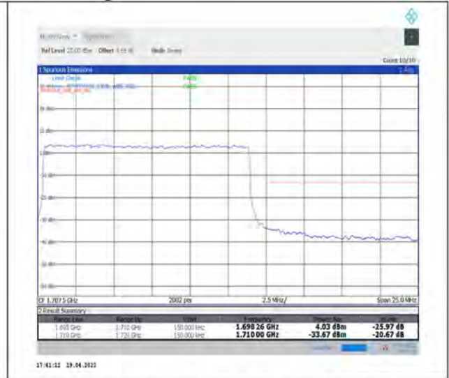
1-N70--15-15-H-3-DFT-PI2BPSK-Outer_Full-75@0-Ant1-seegraph-PASS-see graph
