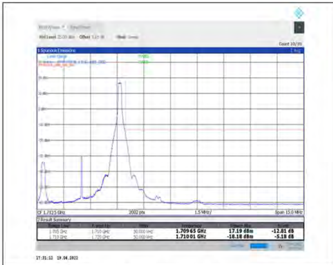
1-N70--15-5-H-2-DFT-PI2BPSK-Edge_1RB_Right-1@24-Ant1-seegraph-PASS-see graph
