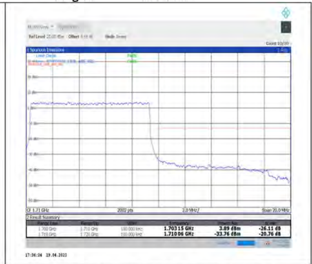
1-N70--15-10-H-3-DFT-PI2BPSK-Outer_Full-50@0-Ant1-seegraph-PASS-see graph
