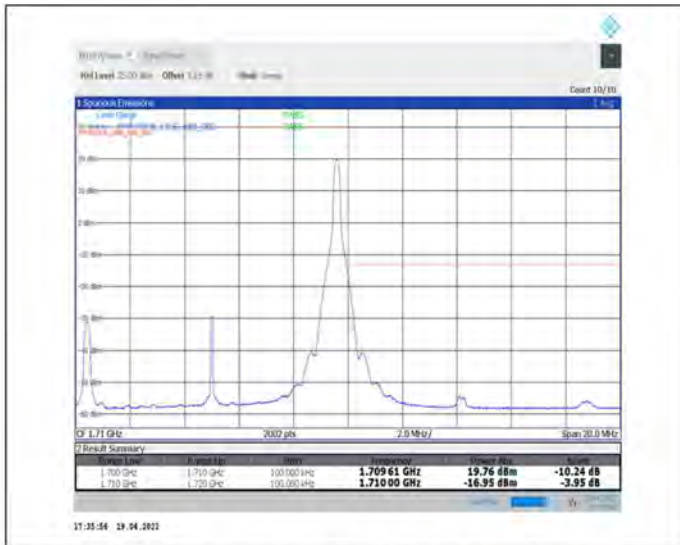
1-N70--15-10-H-2-DFT-PI2BPSK-Edge_1RB_Right-1@51-Ant1-seegraph-PASS-see graph
