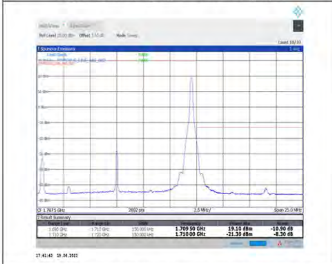
1-N70--15-15-H-5-CP-QPSK-Edge_1RB_Right-1@78-Ant1-seegraph-PASS-see graph
