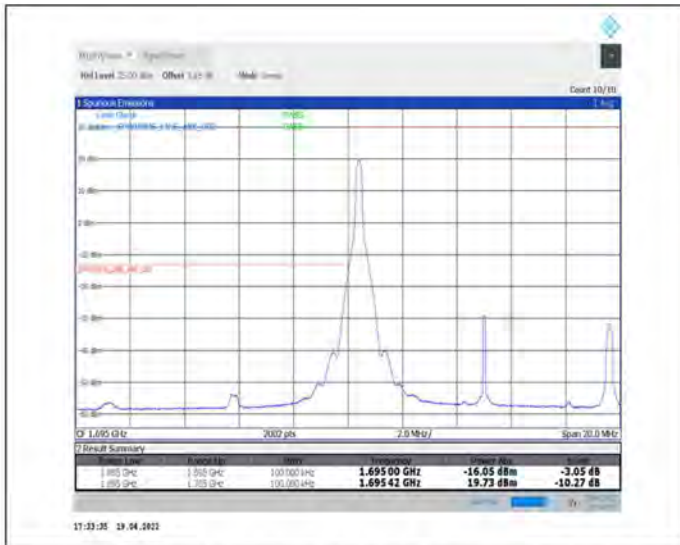
1-N70--15-10-L-1-DFT-PI2BPSK-Edge_1RB_Left-1@0-Ant1-seegraph-PASS-see graph
