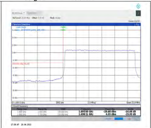
1-N70--15-15-L-3-DFT-PI2BPSK-Outer_Full-75@0-Ant1-seegraph-PASS-see graph
