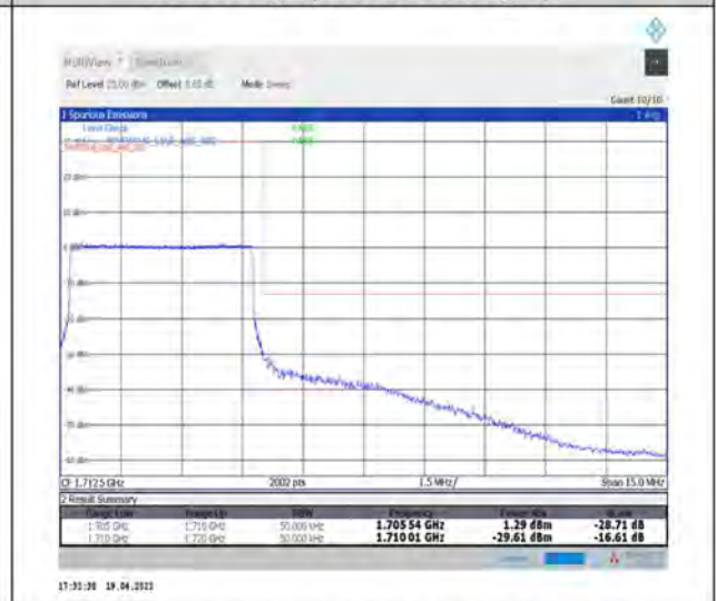
1-N70--15-5-H-6-CP-QPSK-Outer_Full-25@0-Ant1-seegraph-PASS-see graph
