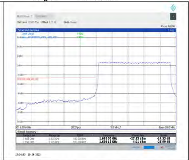
1-N70--15-10-L-3-DFT-PI2BPSK-Outer_Full-50@0-Ant1-seegraph-PASS-see graph
