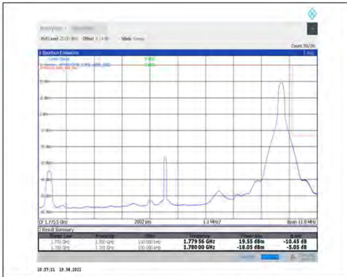
1-N66-PC3-15-10-H-2-DFT-PI2BPSK-Edge_1RB_Right-1@51-Ant1-seegraph-PASS-see graph
