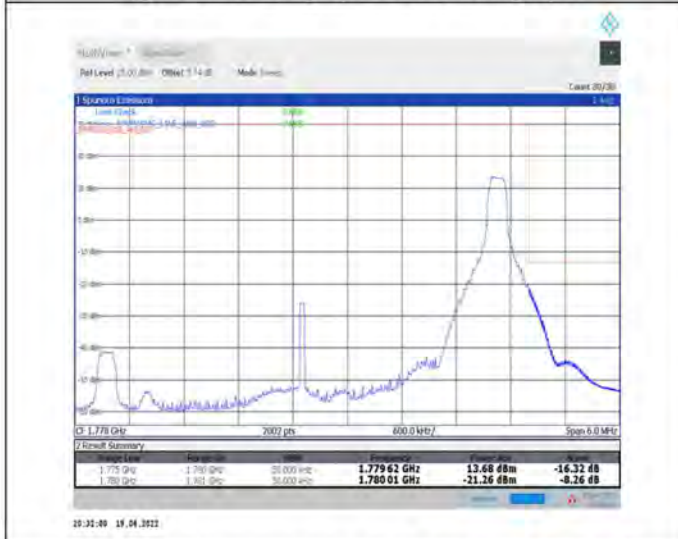
1-N66-PC3-15-5-H-5-CP-QPSK-Edge_1RB_Right-1@24-Ant1-seegraph-PASS-see graph
