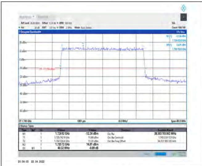
1-N66-PC3-15-40-M-1-DFT-QPSK-Outer_Full-216@0-Ant1-38.584-40.320-≤40-PASS
