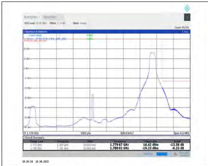
1-N66-PC3-15-5-H-2-DFT-PI2BPSK-Edge_1RB_Right-1@24-Ant1-seegraph-PASS-see graph
