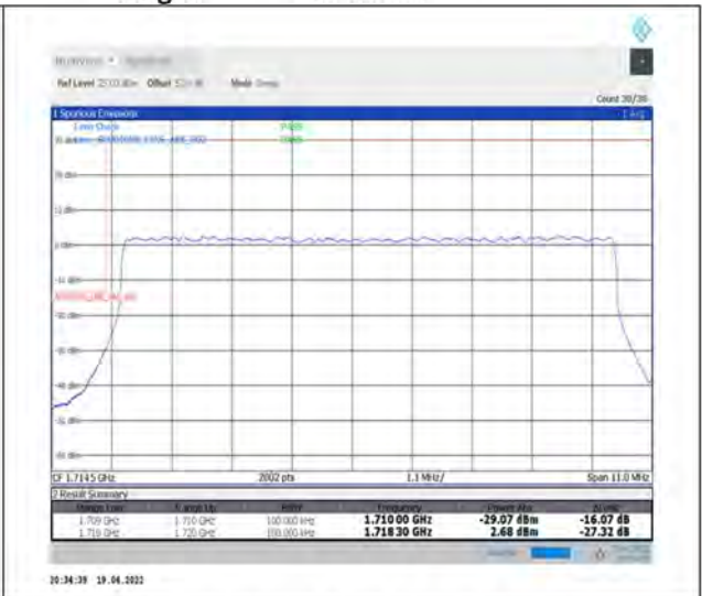
1-N66-PC3-15-10-L-3-DFT-PI2BPSK-Outer_Full-50@0-Ant1-seegraph-PASS-see graph
