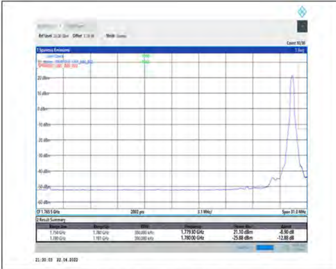
1-N66-PC3-15-30-H-2-DFT-PI2BPSK-Edge_1RB_Right-1@159-Ant1-seegraph-PASS-see graph
