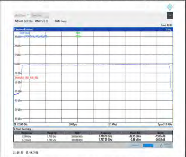
1-N66-PC3-15-30-L-6-CP-QPSK-Outer_Full-160@0-Ant1-seegraph-PASS-see graph
