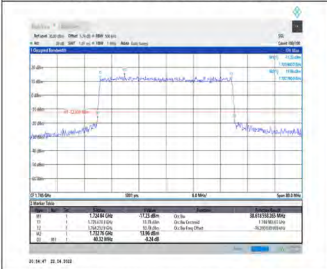
1-N66-PC3-15-40-M-3-DFT-16QAM-Outer_Full-216@0-Ant1-38.619-40.320-≤40-PASS
