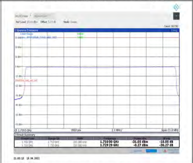
1-N66-PC3-15-20-L-6-CP-QPSK-Outer_Full-106@0-Ant1-seegraph-PASS-see graph
