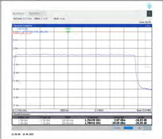
1-N66-PC3-15-20-H-3-DFT-PI2BPSK-Outer_Full-100@0-Ant1-seegraph-PASS-see graph
