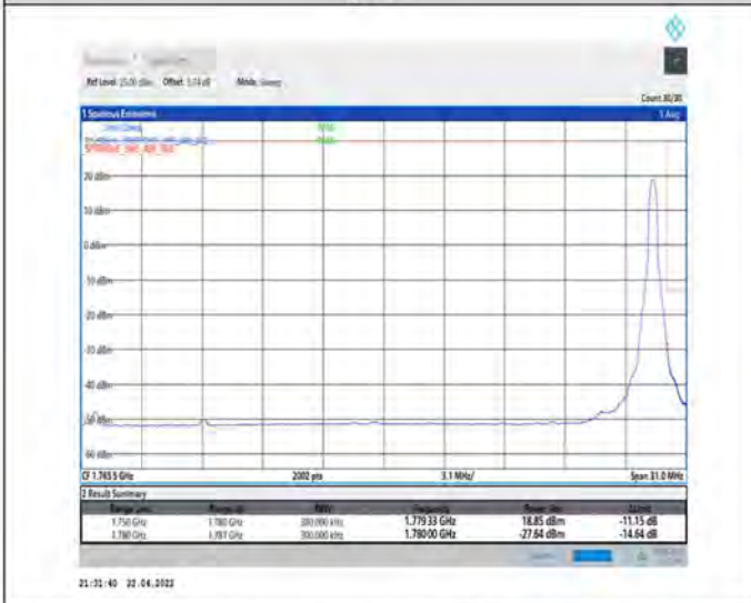
1-N66-PC3-15-30-H-5-CP-QPSK-Edge_1RB_Right-1@159-Ant1-seegraph-PASS-see graph
