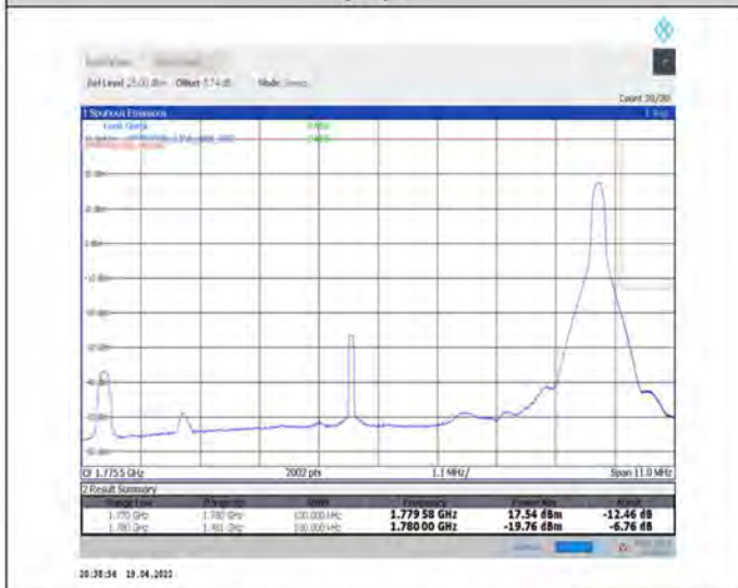
1-N66-PC3-15-10-H-5-CP-QPSK-Edge_1RB_Right-1@51-Ant1-seegraph-PASS-see graph
