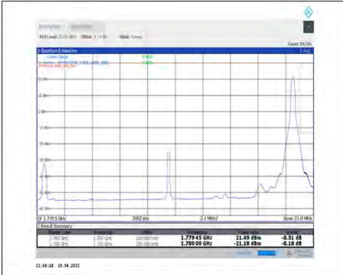
1-N66-PC3-15-20-H-2-DFT-PI2BPSK-Edge_1RB_Right-1@105-Ant1-seegraph-PASS-see graph
