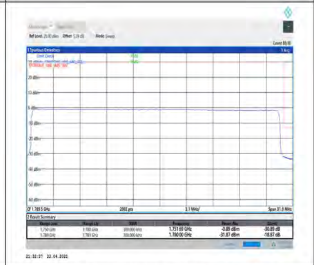
1-N66-PC3-15-30-H-6-CP-QPSK-Outer_Full-160@0-Ant1-seegraph-PASS-see graph
