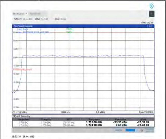
1-N66-PC3-15-20-L-3-DFT-PI2BPSK-Outer_Full-100@0-Ant1-seegraph-PASS-see graph
