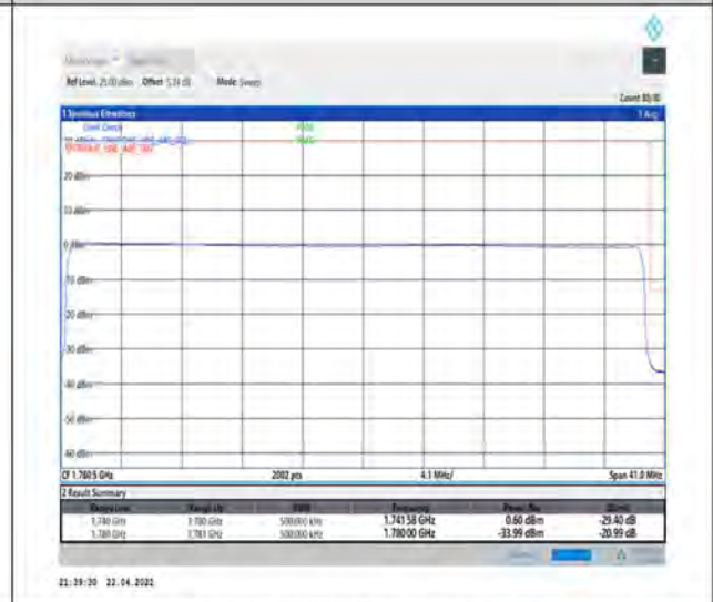
1-N66-PC3-15-40-H-6-CP-QPSK-Outer_Full-216@0-Ant1-seegraph-PASS-see graph
