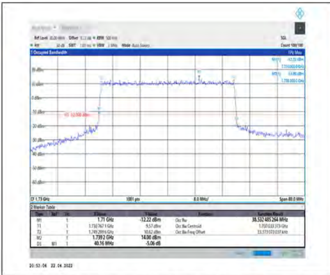
1-N66-PC3-15-40-L-6-CP-QPSK-Outer_Full-216@0-Ant1-38.532-40.160-≤40-PASS
