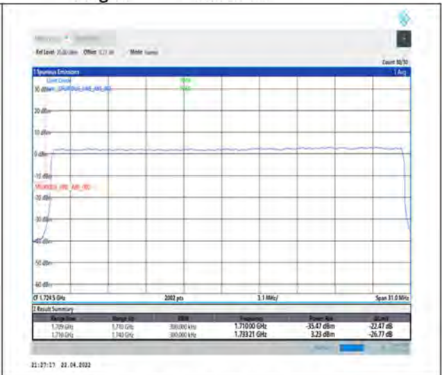
1-N66-PC3-15-30-L-3-DFT-PI2BPSK-Outer_Full-160@0-Ant1-seegraph-PASS-see graph
