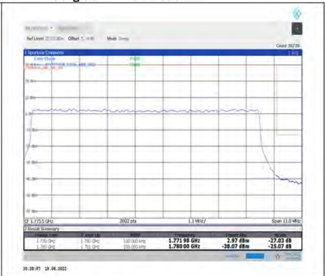
1-N66-PC3-15-10-H-3-DFT-PI2BPSK-Outer_Full-50@0-Ant1-seegraph-PASS-see graph
