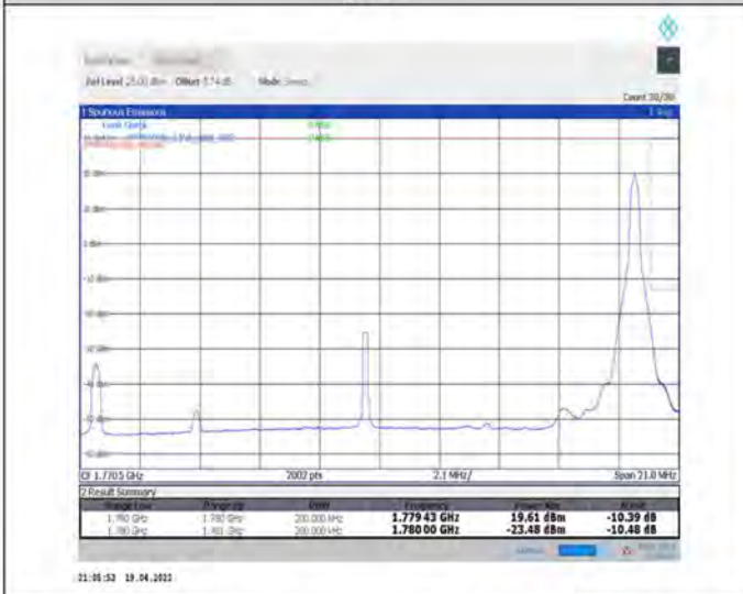
1-N66-PC3-15-20-H-5-CP-QPSK-Edge_1RB_Right-1@105-Ant1-seegraph-PASS-see graph
