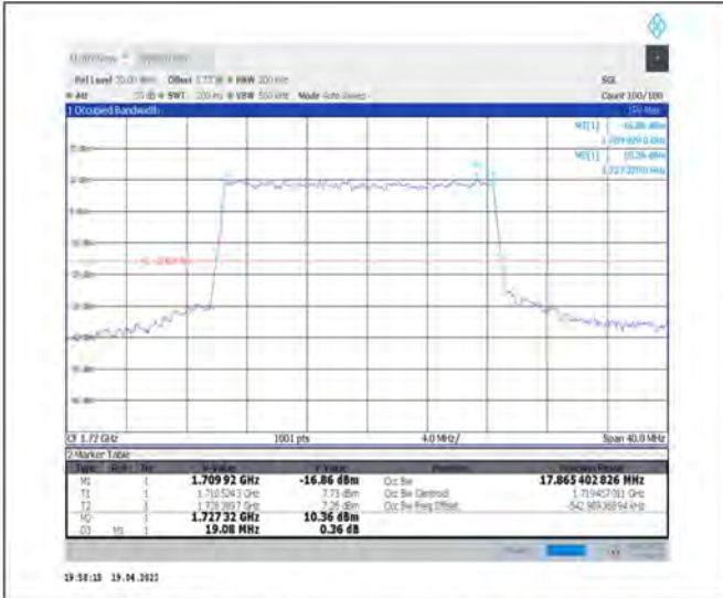
1-N66-PC3-15-20-L-4-DFT-64QAM-Outer_Full-100@0-Ant1-17.865-19.080-≤20-PASS
