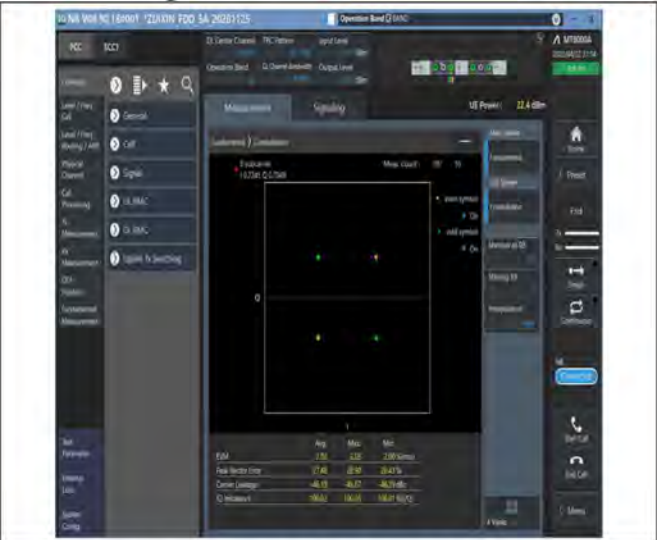
1-N66-PC3-15-40-M-1-DFT-PI2BPSK-Outer_Full-216@0-Ant1-see graph-PASS
