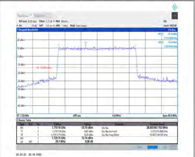
1-N66-PC3-15-30-L-4-DFT-64QAM-Outer_Full-160@0-Ant1-28.604-29.700-≤30-PASS
