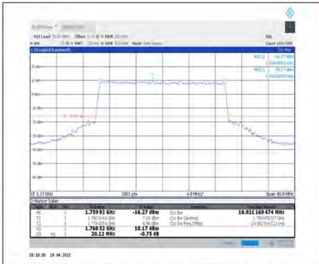
1-N66-PC3-15-20-H-6-CP-QPSK-Outer_Full-106@0-Ant1-18.921-20.120-≤20-PASS
