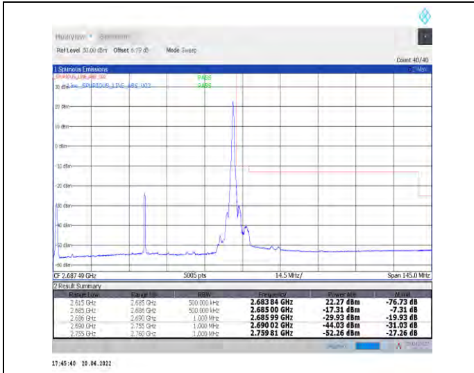
1-N41--30-70-H-2-DFT-PI2BPSK-Edge_1RB_Right-1@188-Ant1-PASS-see graph
