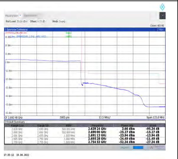
1-N41--30-60-H-6-CP-QPSK-Outer_Full-162@0-A nt1-PASS-see graph
