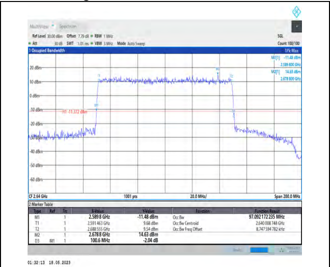
1-N41-PC1-30-100-H-8-CP-64QAM-Outer_Full-273 @0-Ant1-97.092-100.600-≤100-PASS
