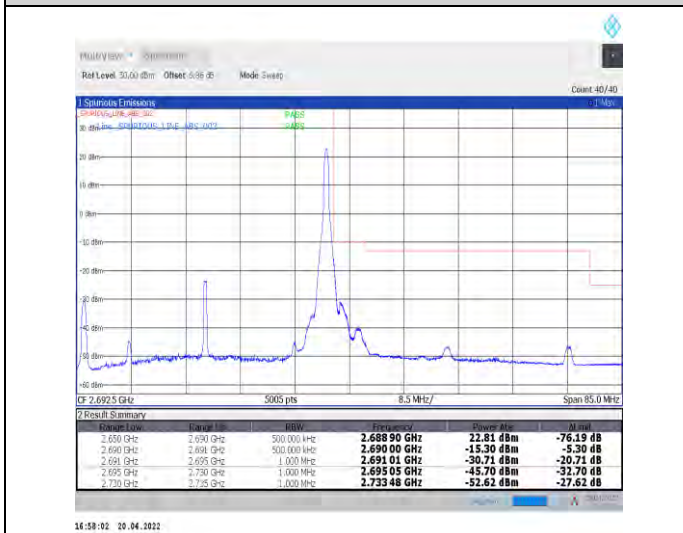
1-N41--30-40-H-5-CP-QPSK-Edge_1RB_Right-1@105-Ant1-PASS-see graph
