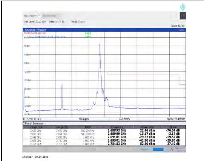
1-N41--30-60-H-2-DFT-PI2BPSK-Edge_1RB_Right-1@ 161-Ant1-PASS-see graph
