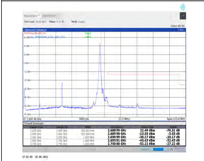
1-N41--30-60-H-5-CP-QPSK-Edge_1RB_Right-1@161 -Ant1-PASS-see graph
