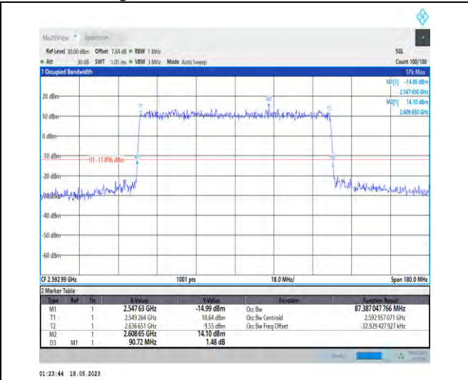
1-N41-PC1-30-90-M-8-CP-64QAM-Outer_Full-245@ 0-Ant1-87.387-90.720-≤90-PASS
