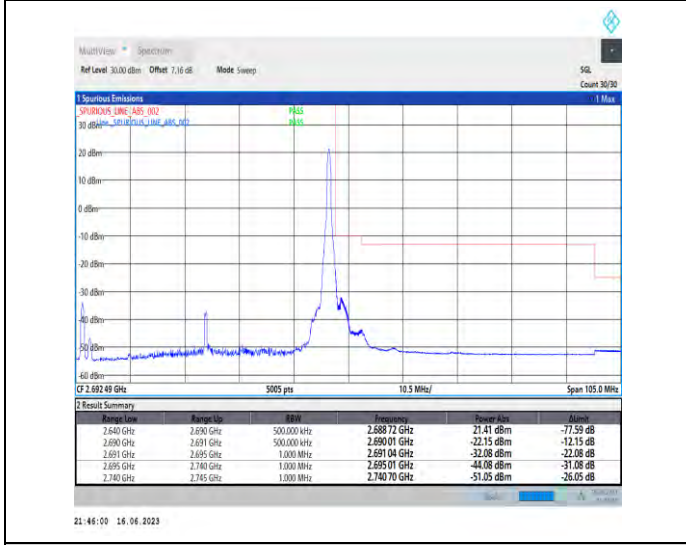
1-N41-PC1-30-50-H-5-CP-QPSK-Edge_1RB_Right-1 @132-Ant1-1--PASS-see graph
