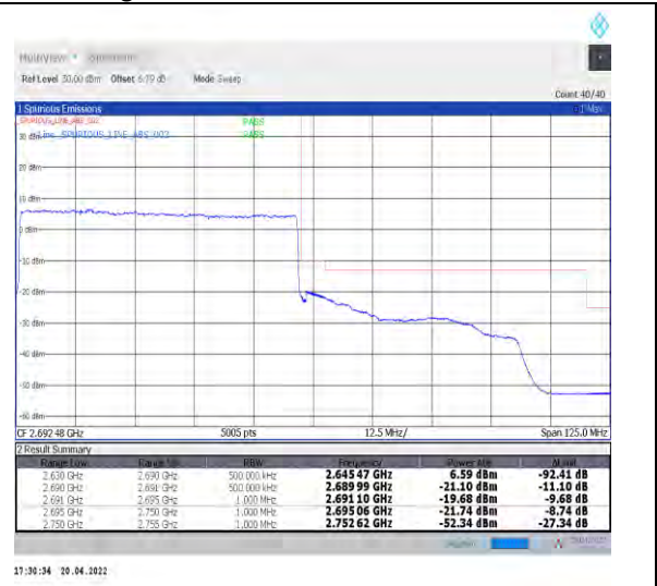
1-N41--30-60-H-3-DFT-PI2BPSK-Outer_Full-162 @0-Ant1-PASS-see graph
