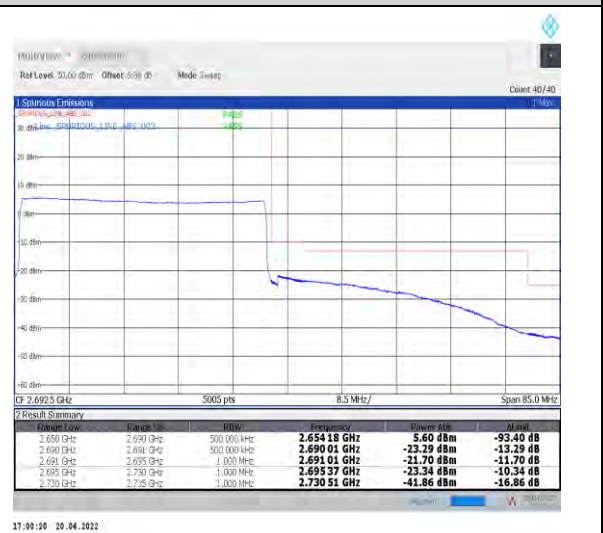
1-N41--30-40-H-6-CP-QPSK-Outer_Full-106@0-Ant1-PASS-see graph
