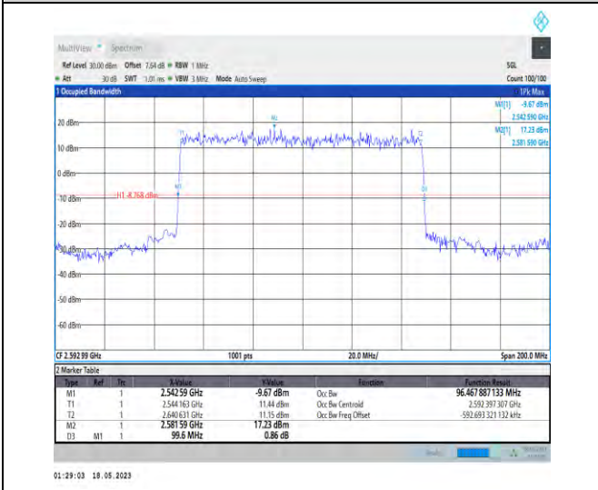
1-N41-PC1-30-100-M-2-DFT-PI2BPSK-Outer_Full-270 @0-Ant1-96.468-99.600-≤100-PASS
