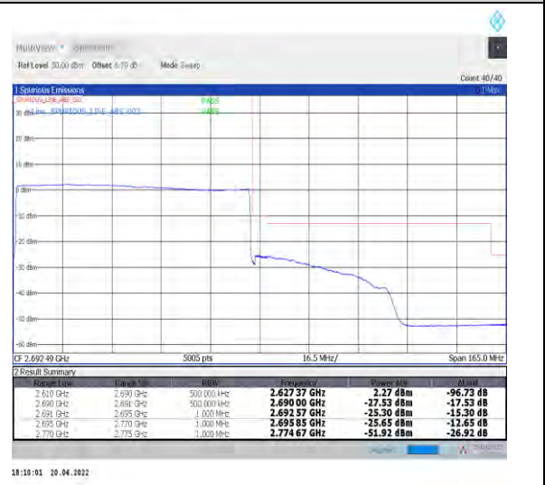
1-N41--30-80-H-6-CP-QPSK-Outer_Full-217@0-Ant1-PASS-see graph
