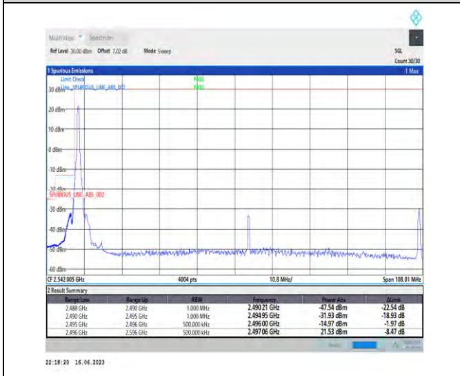
1-N41-PC1-30-100-L-4-CP-QPSK-Edge_1RB_Left-1 @0-Ant1-1--PASS-see graph
