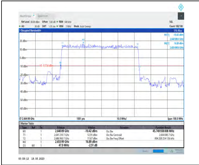
1-N41-PC1-30-50-H-2-DFT-PI2BPSK-Outer_Full-128 @0-Ant1-45.75-47.900-≤50-PASS
