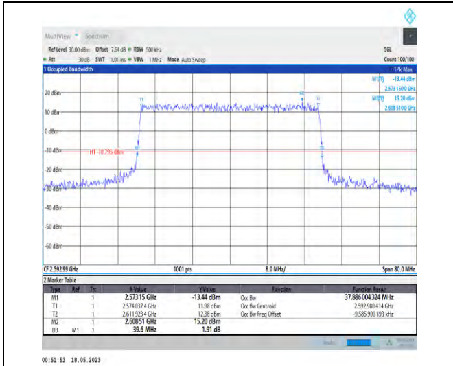
1-N41-PC1-30-40-M-6-CP-QPSK-Outer_Full-106@0 -Ant1-37.886-39.600-≤40-PASS
