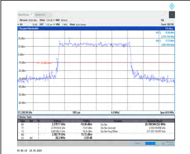
1-N41-PC1-30-30-M-3-DFT-16QAM-Outer_Full-75@0 0-Ant1-26.769-28.200-≤30-PASS
