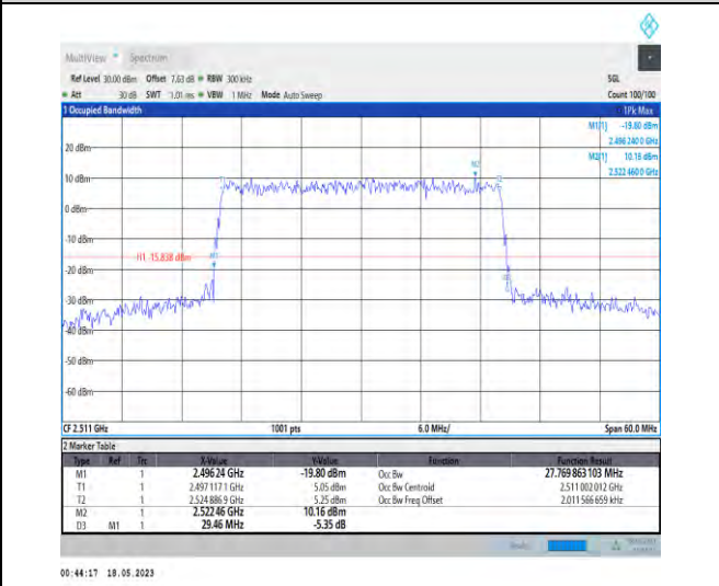
1-N41-PC1-30-30-L-9-CP-256QAM-Outer_Full-78@0-A Ant1-27.77-29.460-≤30-PASS
