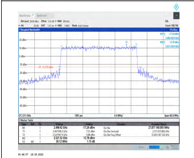
1-N41-PC1-30-30-L-8-CP-64QAM-Outer_Full-78@0-A Ant1-27.871-30.120-≤30-PASS
