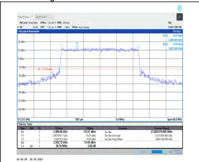
1-N41-PC1-30-30-L-7-CP-16QAM-Outer_Full-78@0-A Ant1-27.82-29.160-≤30-PASS
