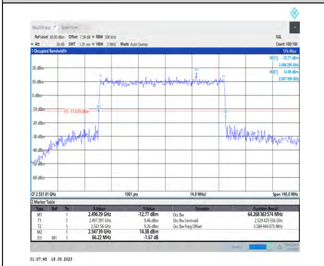
1-N41-PC1-30-70-L-4-DFT-64QAM-Outer_Full-180 @0-Ant1-64.268-66.220-<math>\leq 70</math>-PASS
