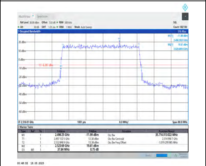
1-N41-PC1-30-40-L-2-DFT-PI2BPSK-Outer_Full-100@0 -Ant1-35.716-37.840-<math>\leq 40</math>-PASS
