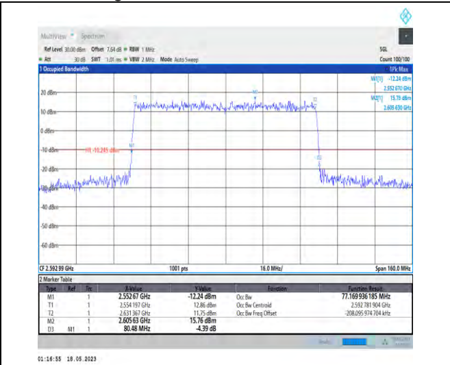
1-N41-PC1-30-80-M-3-DFT-16QAM-Outer_Full-216 @0-Ant1-77.17-80.480-≤80-PASS
