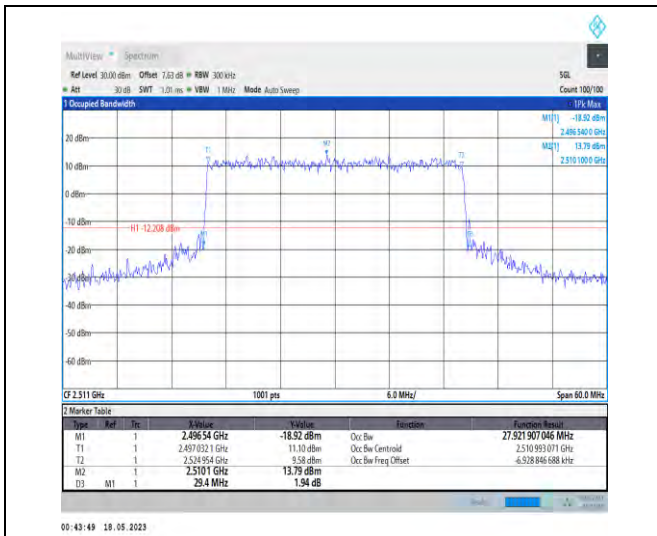
1-N41-PC1-30-30-L-6-CP-QPSK-Outer_Full-78@0-A nt1-27.922-29.400-≤30-PASS
