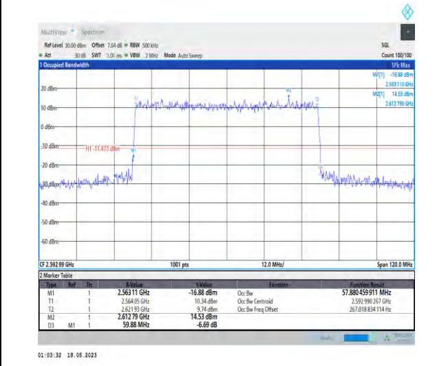
1-N41-PC1-30-60-M-3-DFT-16QAM-Outer_Full-162 @0-Ant1-57.88-59.880-≤60-PASS
