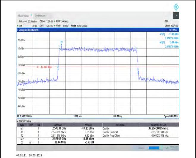
1-N41-PC1-30-40-M-9-CP-256QAM-Outer_Full-106@0 -Ant1-37.865-39.440-≤40-PASS
