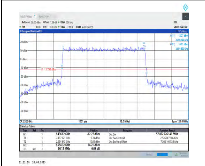
1-N41-PC1-30-60-L-3-DFT-16QAM-Outer_Full-162 @0-Ant1-57.872-60.120-≤60-PASS
