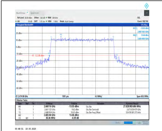
1-N41-PC1-30-30-H-8-CP-64QAM-Outer_Full-78@0 -Ant1-27.829-30.360-<math>\leq 30</math>-PASS
