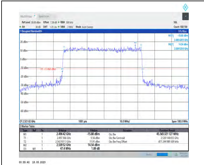
1-N41-PC1-30-50-L-4-DFT-64QAM-Outer_Full-128 @0-Ant1-45.565-47.400-≤50-PASS
