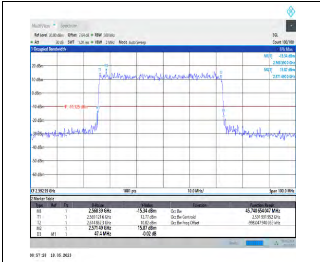
1-N41-PC1-30-50-M-3-DFT-16QAM-Outer_Full-128 @0-Ant1-45.741-47.400-≤50-PASS
