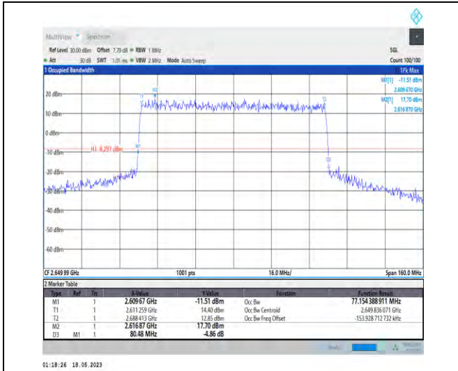
1-N41-PC1-30-80-H-1-DFT-QPSK-Outer_Full-216@ 0-Ant1-77.154-80.480-≤80-PASS
