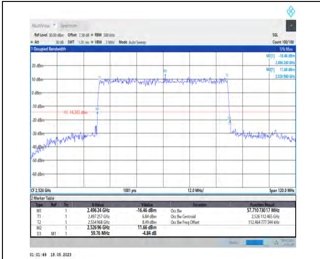
1-N41-PC1-30-60-L-5-DFT-256QAM-Outer_Full-162 @0-Ant1-57.711-59.760-≤60-PASS
