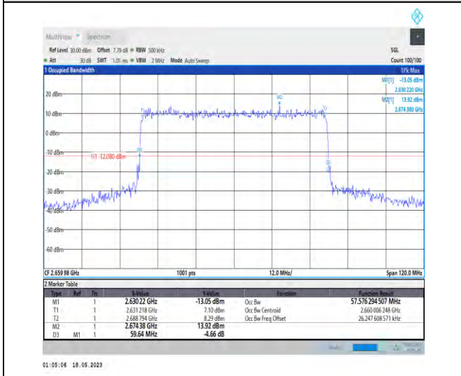
1-N41-PC1-30-60-H-1-DFT-QPSK-Outer_Full-162@ 0-Ant1-57.576-59.640-≤60-PASS
