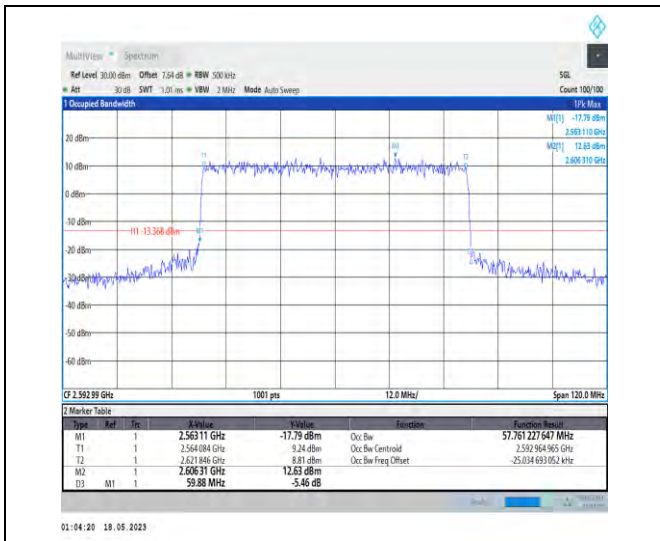
1-N41-PC1-30-60-M-8-CP-64QAM-Outer_Full-162@ 0-Ant1-57.761-59.880-≤60-PASS
