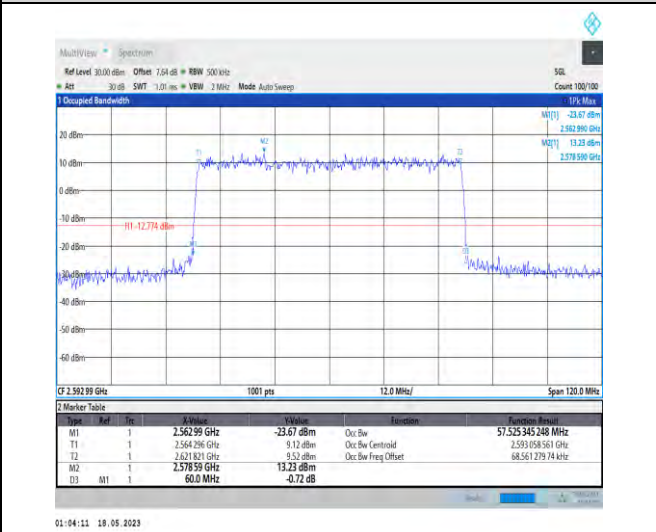
1-N41-PC1-30-60-M-7-CP-16QAM-Outer_Full-162@0 -Ant1-57.525-60.000-≤60-PASS
