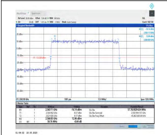
1-N41-PC1-30-60-M-6-CP-QPSK-Outer_Full-162@0 -Ant1-57.764-59.760-≤60-PASS
