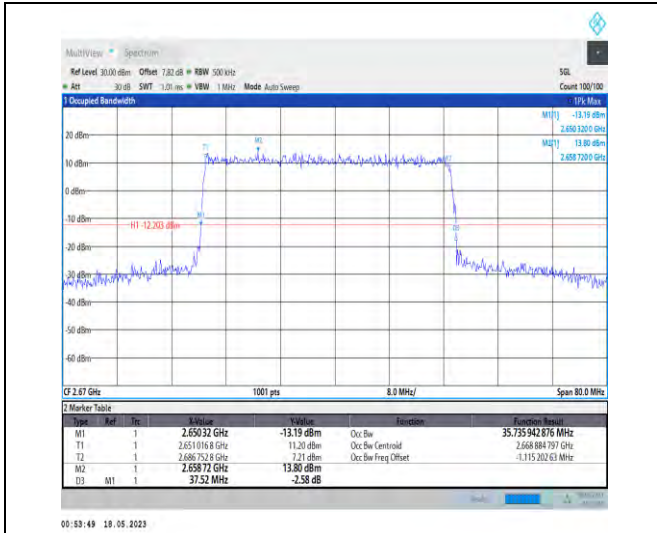
1-N41-PC1-30-40-H-5-DFT-256QAM-Outer_Full-100 @0-Ant1-35.736-37.520-≤40-PASS
