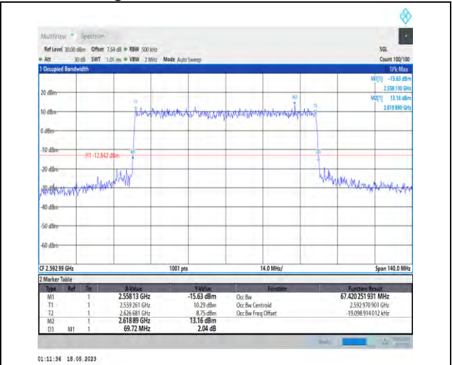
1-N41-PC1-30-70-M-6-CP-QPSK-Outer_Full-189@0 -Ant1-67.42-69.720-<=70-PASS
