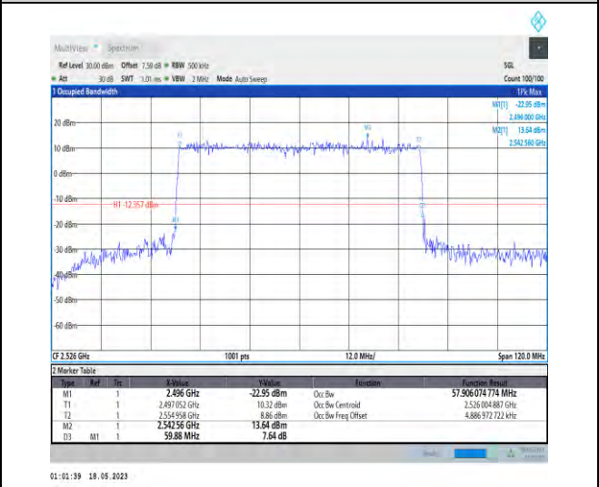
1-N41-PC1-30-60-L-4-DFT-64QAM-Outer_Full-162 @0-Ant1-57.906-59.880-≤60-PASS
