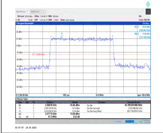
1-N41-PC1-30-50-M-5-DFT-256QAM-Outer_Full-128 @0-Ant1-45.789-47.300-≤50-PASS
