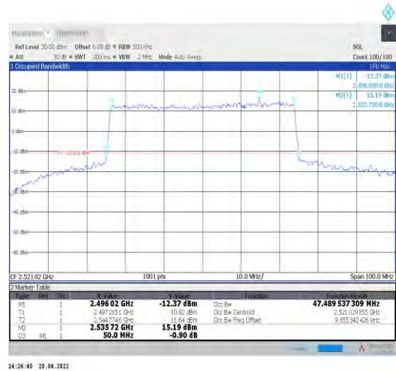
1-N41--30-50-L-7-CP-16QAM-Outer_Full-133@0-Ant t1-47.49-50.000-<math>\leq 50</math>-PASS
