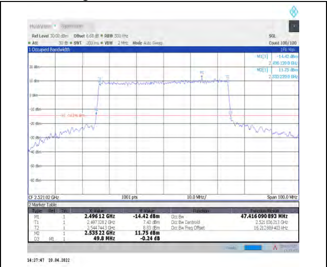
1-N41--30-50-L-9-CP-256QAM-Outer_Full-133@0-Ant nt1-47.416-49.800-≤50-PASS
