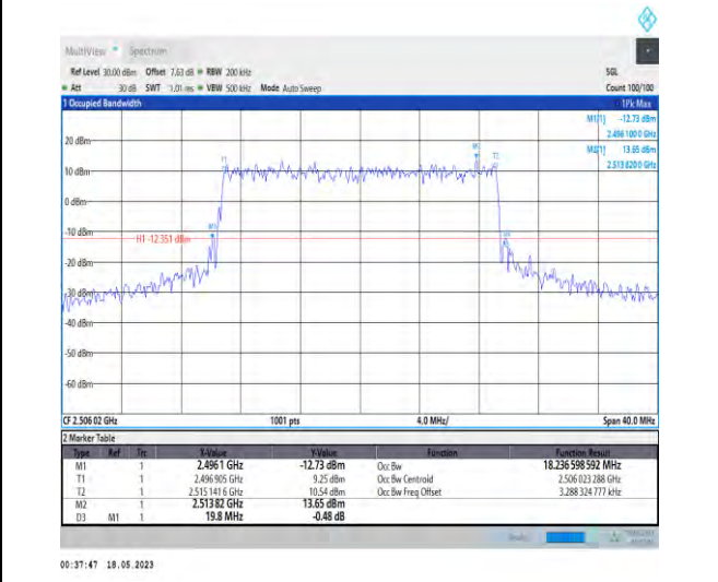
1-N41-PC1-30-20-L-8-CP-64QAM-Outer_Full-51@0-Ant1-18.237-19.800-≤20-PASS
