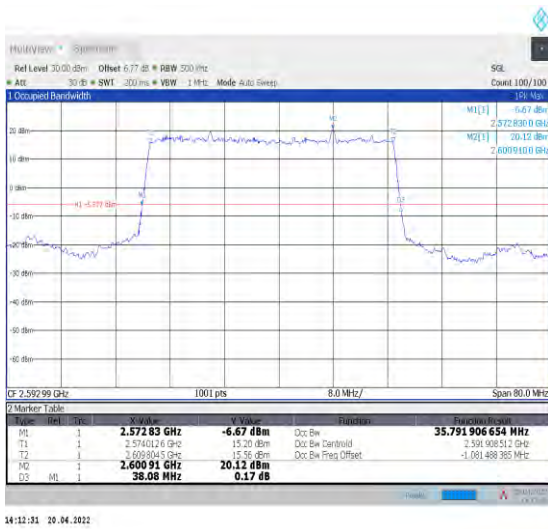
1-N41--30-40-M-2-DFT-PI2BPSK-Outer_Full-100@0-Ant1-35.792-38.080-≤40-PASS
