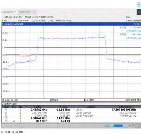
1-N41--30-50-L-6-CP-QPSK-Outer_Full-133@0-Ant1 -47.505-50.200-<math>\leq 50</math>-PASS
