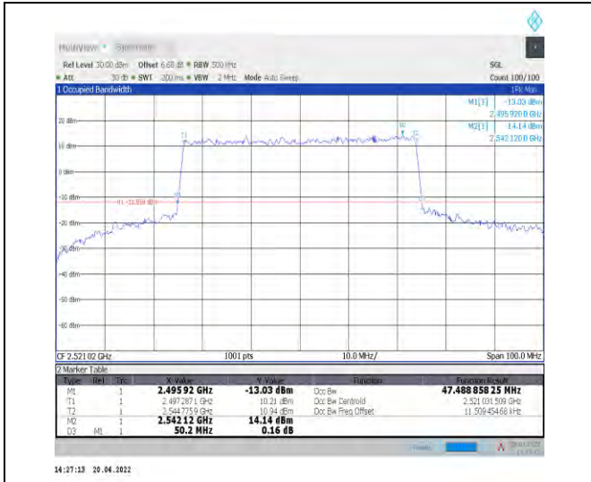
1-N41--30-50-L-8-CP-64QAM-Outer_Full-133@0-Ant 1-47.489-50.200-≤50-PASS
