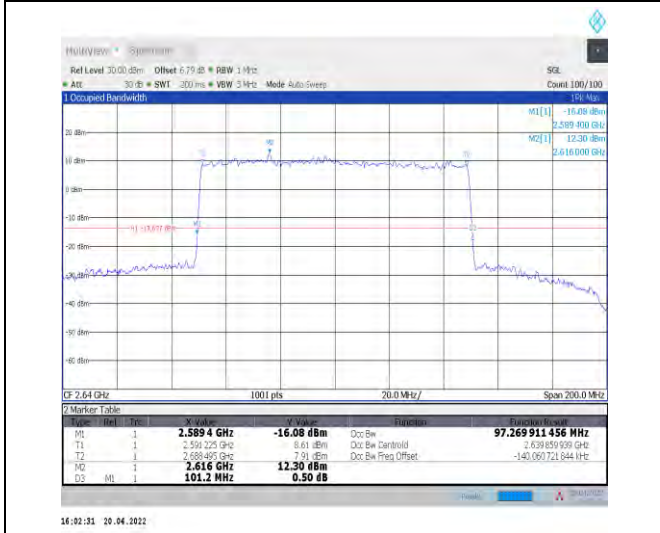
1-N41--30-100-H-9-CP-256QAM-Outer_Full-273@0-A Ant1-97.27-101.200-≤100-PASS
