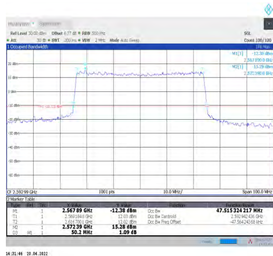
1-N41--30-50-M-6-CP-QPSK-Outer_Full-133@0-Ant 1-47.515-50.200-≤50-PASS
