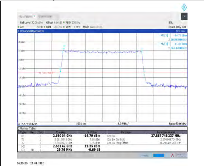
1-N41--30-30-H-9-CP-256QAM-Outer_Full-78@0-An t1-27.888-29.760-≤30-PASS
