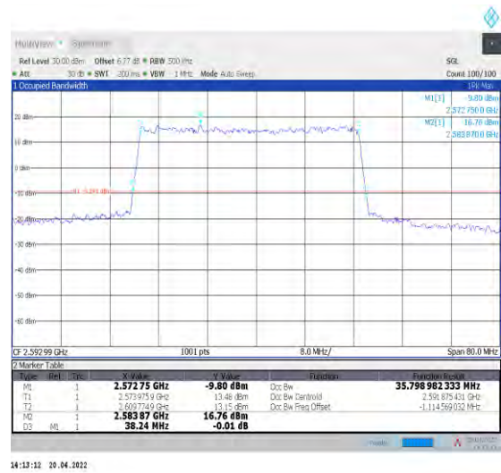
1-N41--30-40-M-3-DFT-16QAM-Outer_Full-100@0-Ant1-35.799-38.240-≤40-PASS
