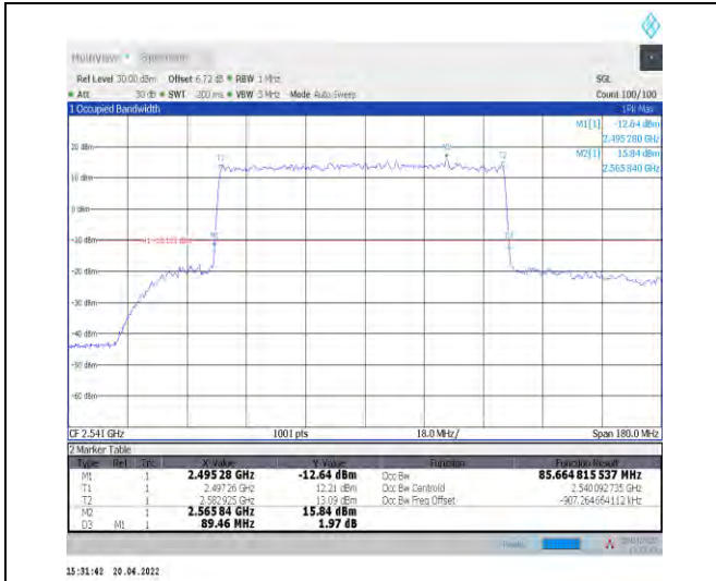
1-N41--30-90-L-4-DFT-64QAM-Outer_Full-240@0-A nt1-85.665-89.460-≤90-PASS
