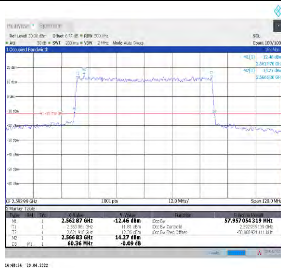
1-N41--30-60-M-7-CP-16QAM-Outer_Full-162@0-A nt1-57.957-60.360-≤60-PASS
