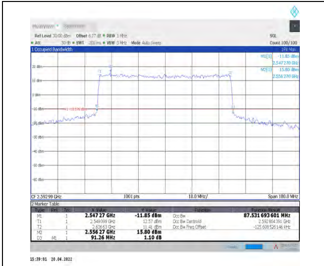
1-N41--30-90-M-7-CP-16QAM-Outer_Full-245@0-An t1-87.532-91.260-<=90-PASS
