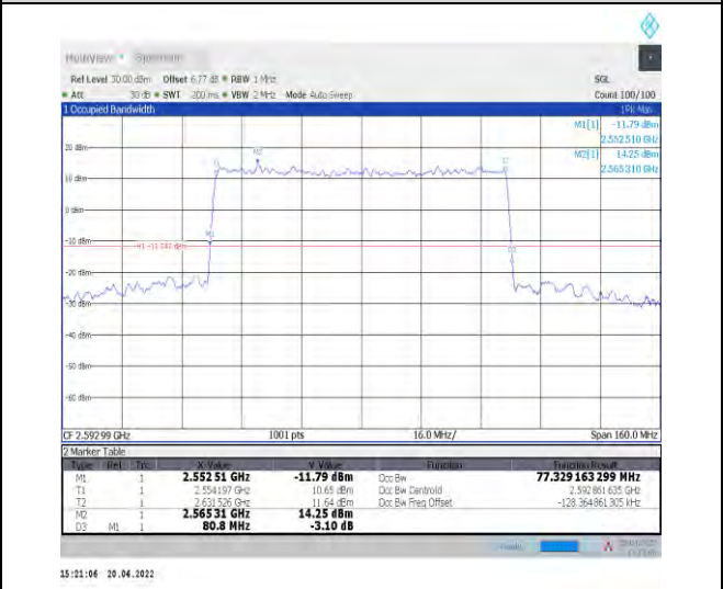
1-N41--30-80-M-5-DFT-256QAM-Outer_Full-216@0-Ant1-77.329-80.800-≤80-PASS
