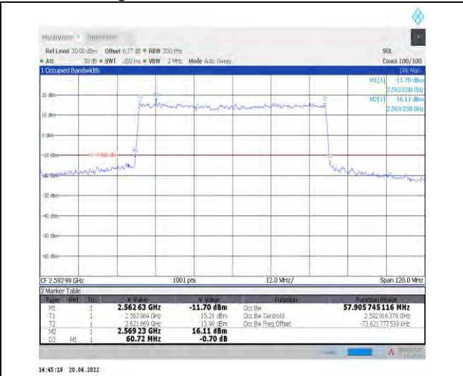
1-N41--30-60-M-1-DFT-QPSK-Outer_Full-162@0-An t1-57.906-60.720-≤60-PASS
