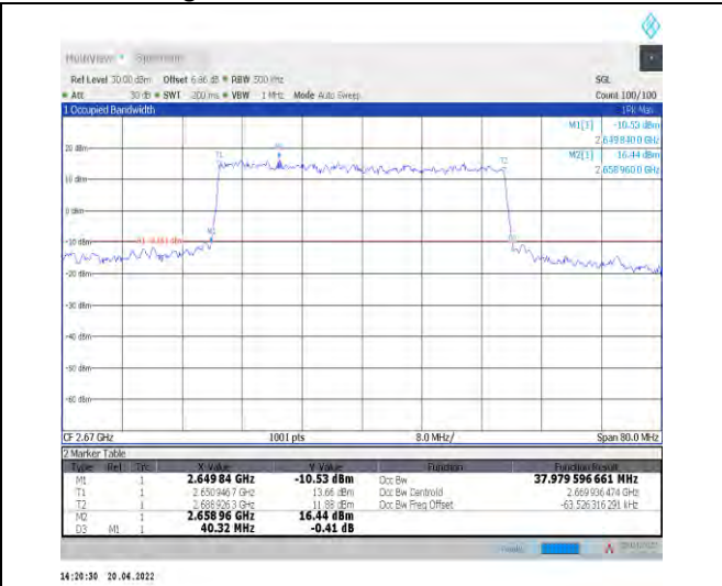
1-N41--30-40-H-6-CP-QPSK-Outer_Full-106@0-Ant 1-37.98-40.320-<math>\leq 40</math>-PASS
