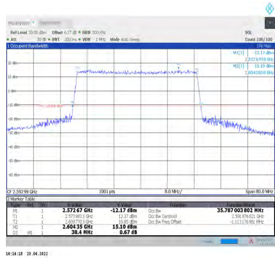
1-N41--30-40-M-5-DFT-256QAM-Outer_Full-100@0-Ant1-35.787-38.400-≤40-PASS
