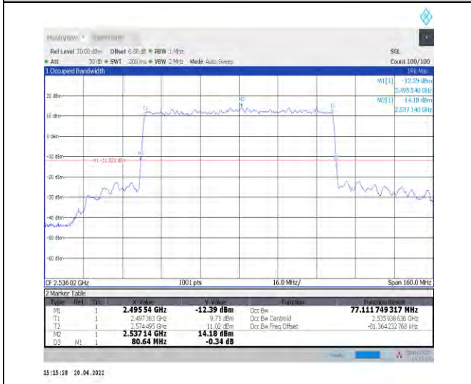
1-N41--30-80-L-5-DFT-256QAM-Outer_Full-216@0-A Ant1-77.112-80.640-<80-PASS
