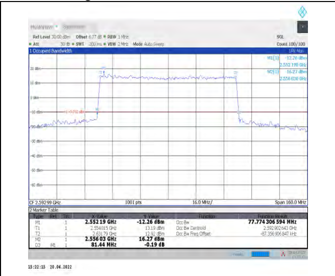
1-N41--30-80-M-7-CP-16QAM-Outer_Full-217@0-Ant 1-77.774-81.440-<80-PASS
