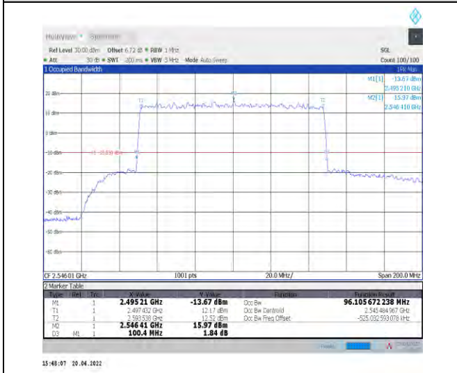
1-N41--30-100-L-3-DFT-16QAM-Outer_Full-270@0-Ant1-96.106-100.400-≤100-PASS
