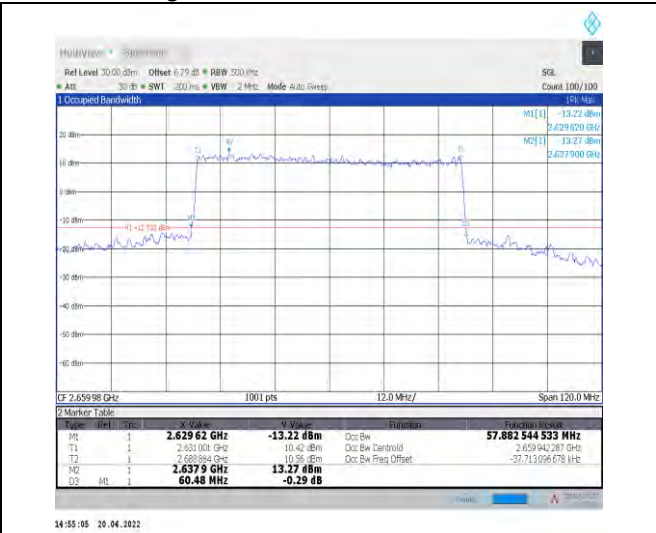
1-N41--30-60-H-8-CP-64QAM-Outer_Full-162@0-An t1-57.883-60.480-≤60-PASS
