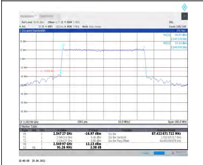
1-N41--30-90-M-9-CP-256QAM-Outer_Full-245@0-A nt1-87.423-91.260-<=90-PASS
