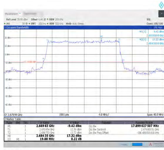
1-N41--30-20-H-2-DFT-PI2BPSK-Outer_Full-50@0- Ant1-17.899-19.880-≤20-PASS
