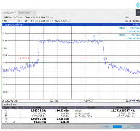
1-N41--30-20-M-8-CP-64QAM-Outer_Full-51@0-Ant 1-18.273-19.240-≤20-PASS
