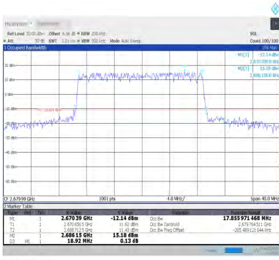
1-N41--30-20-H-1-DFT-QPSK-Outer_Full-50@0-Ant 1-17.856-18.920-≤20-PASS
