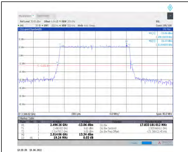
1-N41--30-20-L-5-DFT-256QAM-Outer_Full-50@0-A nt1-17.833-19.240-≤20-PASS
