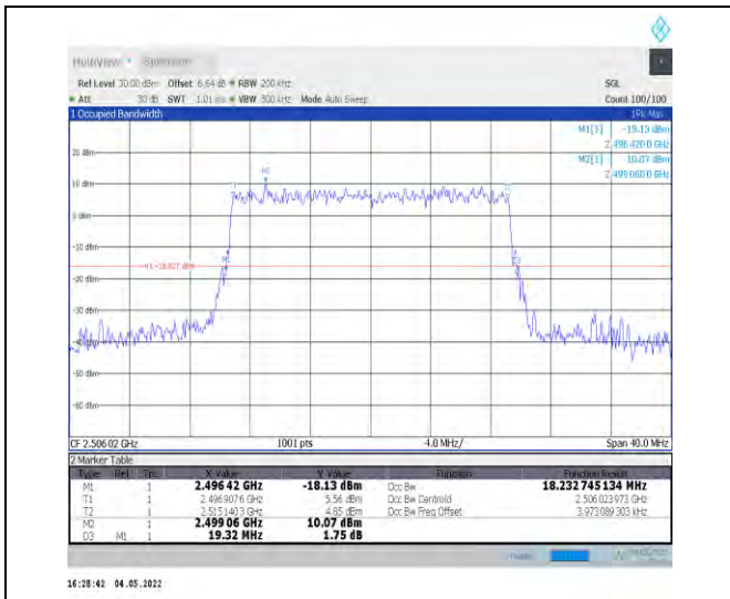
1-N41--30-20-L-9-CP-256QAM-Outer_Full-51@0-Ant 1-18.233-19.320-≤20-PASS
