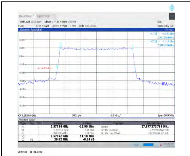
1-N41--30-30-M-9-CP-256QAM-Outer_Full-78@0-Ant t1-27.877-29.820-≤30-PASS
