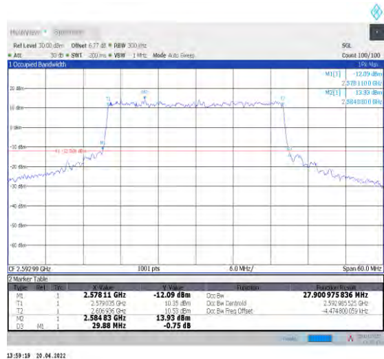
1-N41--30-30-M-8-CP-64QAM-Outer_Full-78@0-Ant 1-27.901-29.880-≤30-PASS
