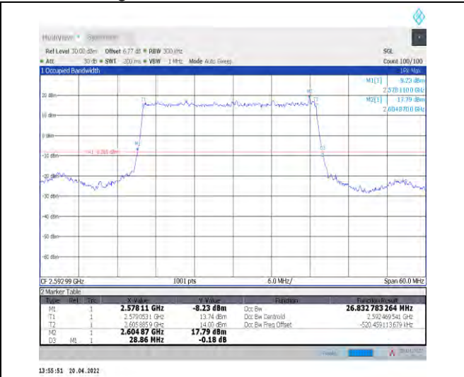
1-N41--30-30-M-2-DFT-PI2BPSK-Outer_Full-75@0-Ant 1-26.833-28.860-≤30-PASS
