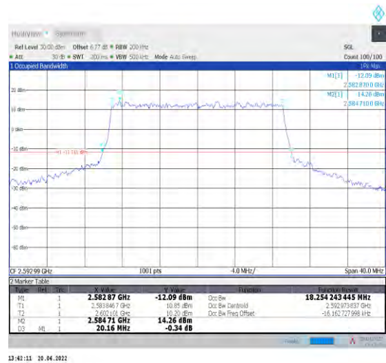
1-N41--30-20-M-7-CP-16QAM-Outer_Full-51@0-Ant 1-18.254-20.160-<=20-PASS
