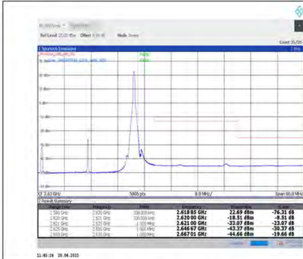
1-N38--30-30-H-2-DFT-PI2BPSK-Edge_1RB_Right-1@77-Ant1-PASS-see graph
