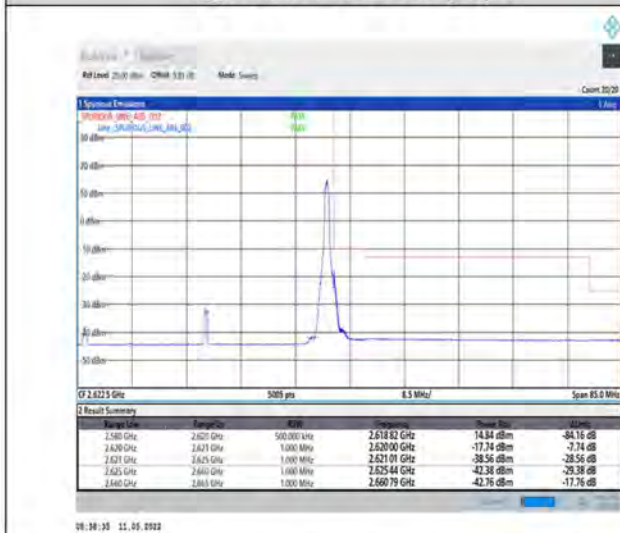
1-N38-PC2-30-40-H-5-CP-QPSK-Edge_1RB_Right-1@105-Ant1-PASS-see graph
