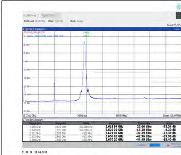
1-N38--30-40-H-2-DFT-PI2BPSK-Edge_1RB_Right-1@105-Ant1-PASS-see graph
