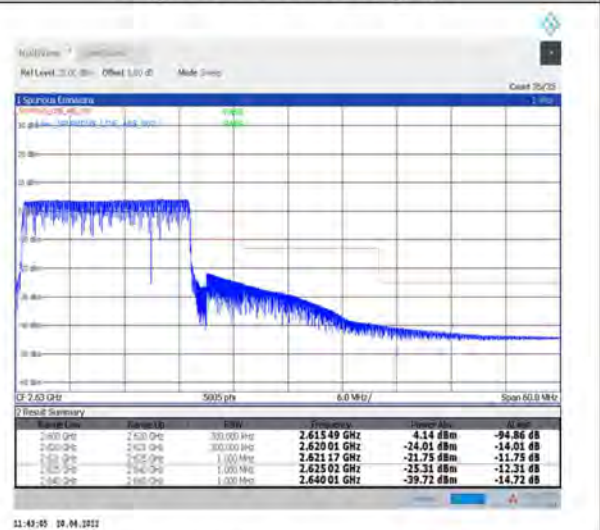
1-N38--30-20-H-6-CP-QPSK-Outer_Full-51@0-Ant1-PASS-see graph
