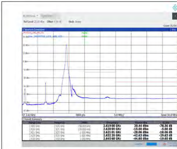
1-N38--30-15-H-2-DFT-PI2BPSK-Edge_1RB_Right-1@37-Ant1-PASS-see graph
