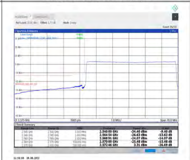
1-N38--30-40-L-6-CP-QPSK-Outer_Full-106@0-Ant1-PASS-see graph
