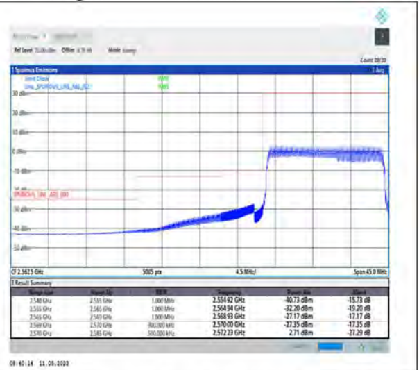
1-N38-PC2-30-15-L-6-CP-QPSK-Outer_Full-38@0-Ant1-PASS-see graph
