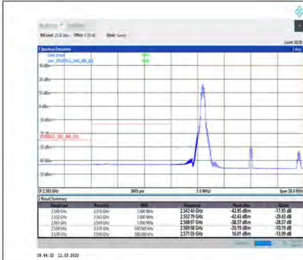
1-N38-PC2-30-20-L-4-CP-QPSK-Edge_1RB_Left-1@0-Ant1-PASS-see graph
