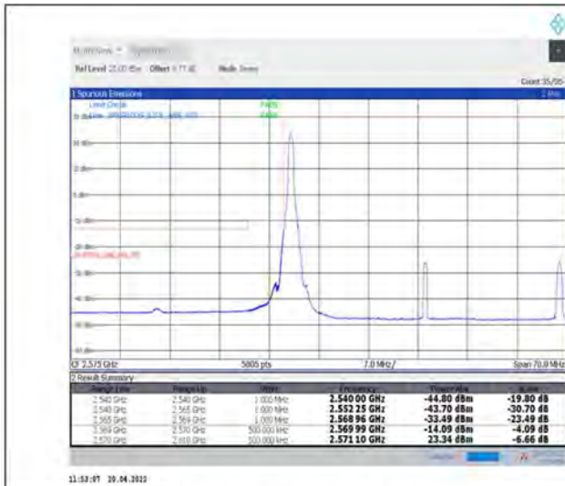
1-N38--30-40-L-1-DFT-PI2BPSK-Edge_1RB_Left-1@0-Ant1-PASS-see graph
