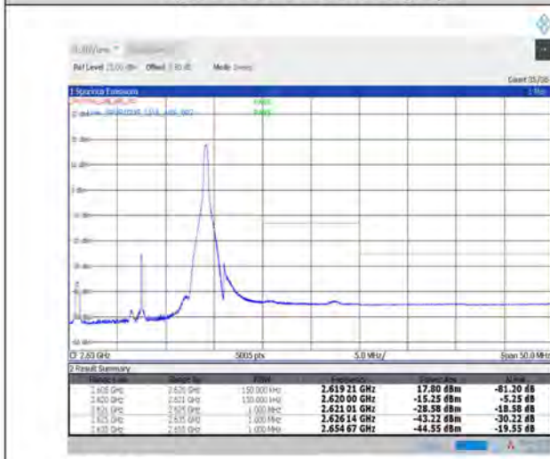
1-N38--30-15-H-2-DFT-PI2BPSK-Edge_1RB_Right-1@37-Ant1-PASS-see graph
