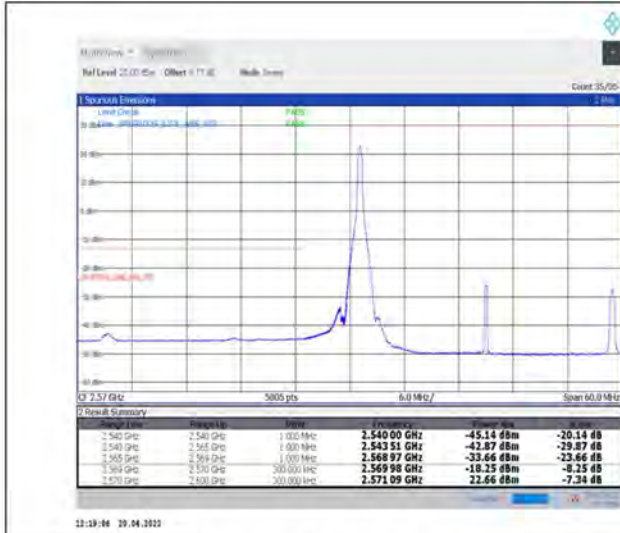
1-N38--30-30-L-1-DFT-PI2BPSK-Edge_1RB_Left-1@0-Ant1-PASS-see graph
