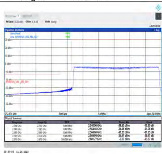
1-N38-PC2-30-40-L-6-CP-QPSK-Outer_Full-106@0-Ant1-PASS-see graph
