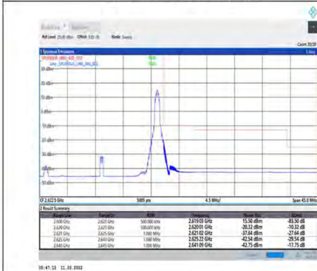
1-N38-PC2-30-20-H-5-CP-QPSK-Edge_1RB_Right-1@50-Ant1-PASS-see graph
