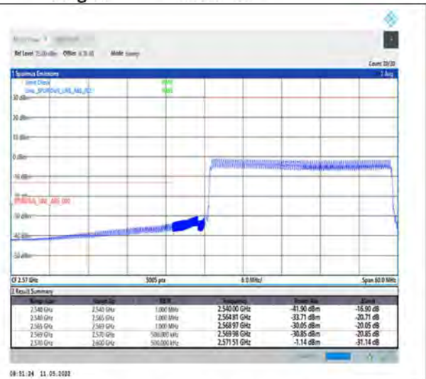
1-N38-PC2-30-30-L-6-CP-QPSK-Outer_Full-78@0-Ant1-PASS-see graph
