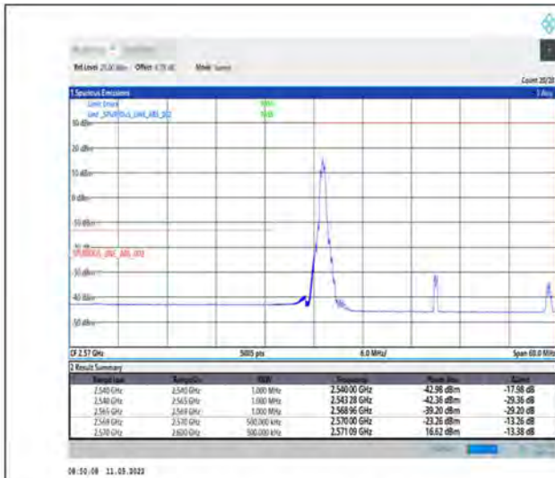
1-N38-PC2-30-30-L-4-CP-QPSK-Edge_1RB_Left-1@0-Ant1-PASS-see graph
