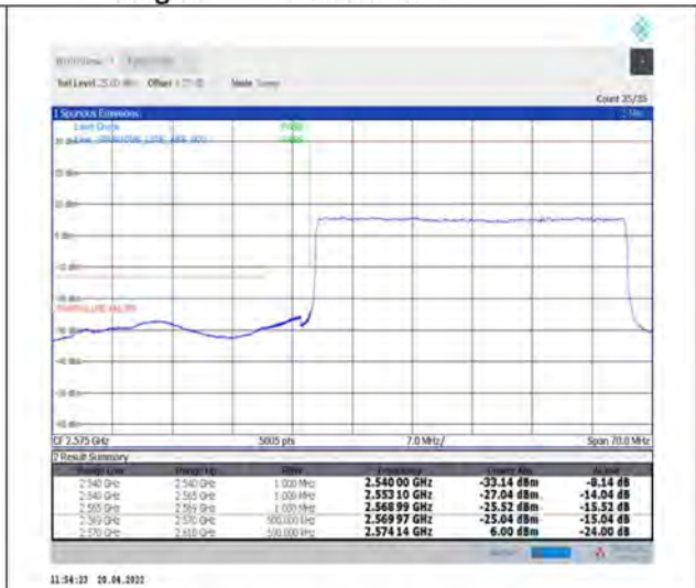
1-N38--30-40-L-3-DFT-PI2BPSK-Outer_Full-100@0-Ant1-PASS-see graph
