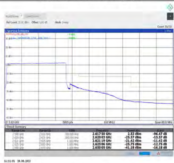
1-N38--30-30-H-6-CP-QPSK-Outer_Full-78@0-Ant1-PASS-see graph
