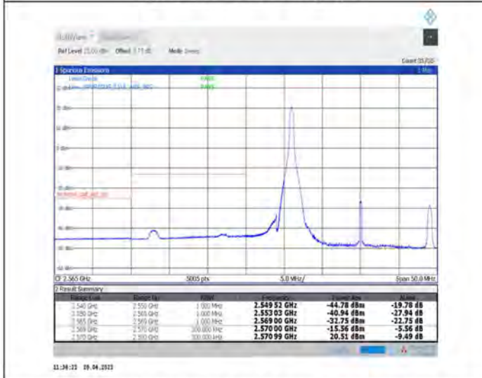
1-N38--30-20-L-4-CP-QPSK-Edge_1RB_Left-1@0-Ant1-PASS-see graph
