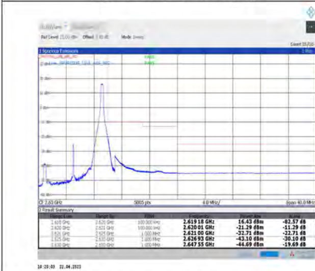
1-N38--30-10-H-5-CP-QPSK-Edge_1RB_Right-1@23-Ant1-PASS-see graph
