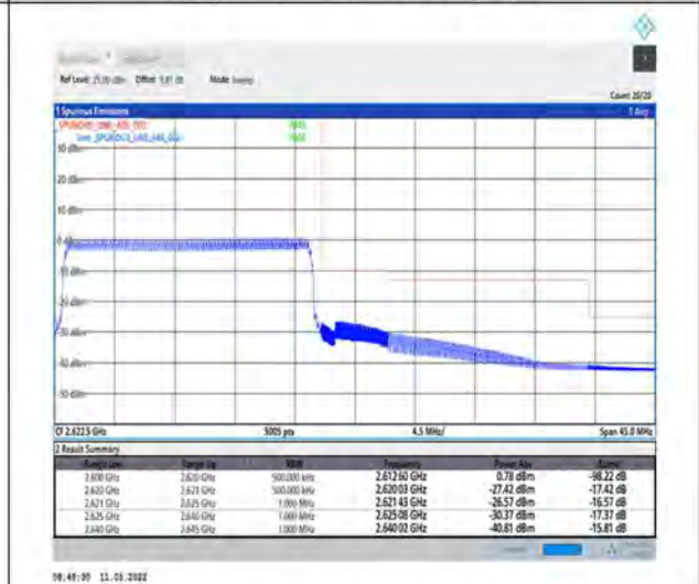
1-N38-PC2-30-20-H-6-CP-QPSK-Outer_Full-51@0-Ant1-PASS-see graph
