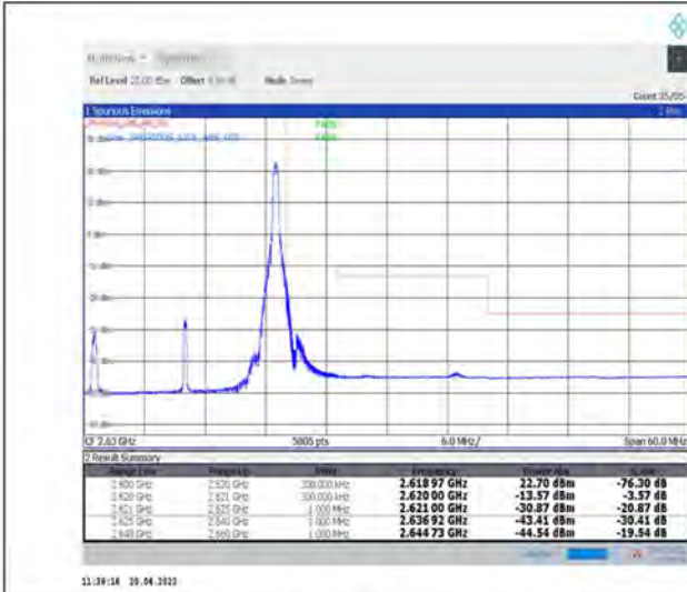
1-N38--30-20-H-2-DFT-PI2BPSK-Edge_1RB_Right-1@50-Ant1-PASS-see graph
