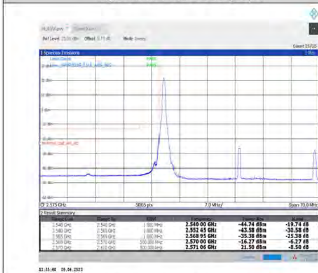
1-N38--30-40-L-4-CP-QPSK-Edge_1RB_Left-1@0-Ant1-PASS-see graph
