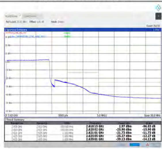
1-N38--30-15-H-3-DFT-PI2BPSK-Outer_Full-36@0-Ant1-PASS-see graph
