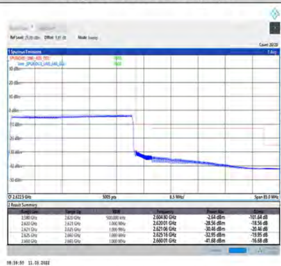
1-N38-PC2-30-40-H-6-CP-QPSK-Outer_Full-106@0-Ant1-PASS-see graph
