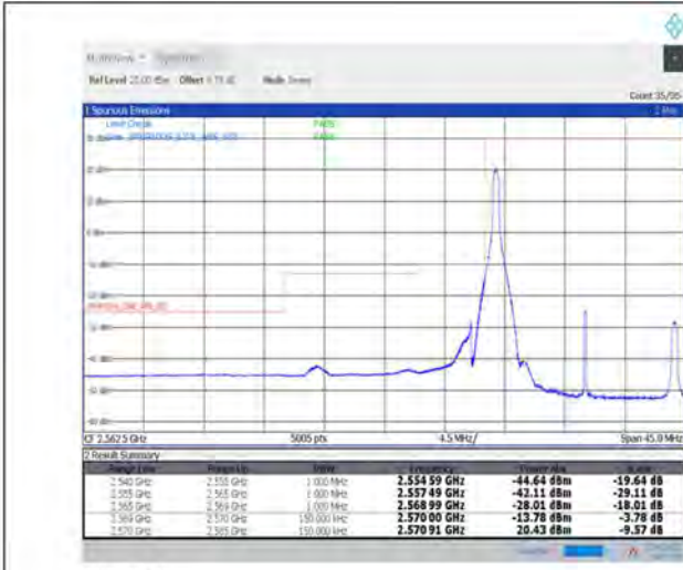
1-N38--30-15-L-1-DFT-PI2BPSK-Edge_1RB_Left-1@0-Ant1-PASS-see graph
