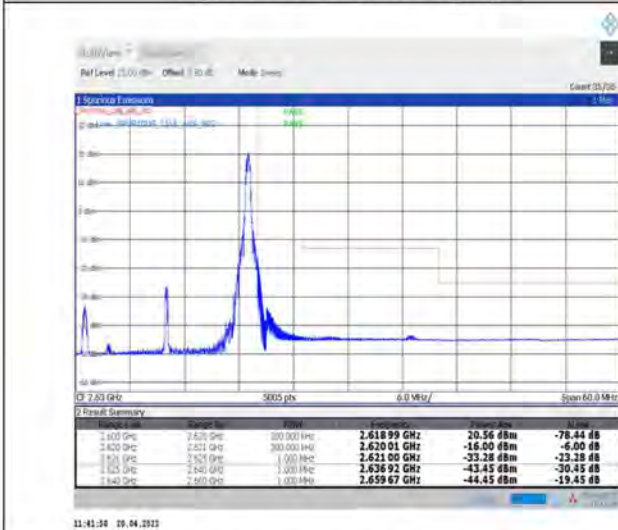
1-N38--30-20-H-5-CP-QPSK-Edge_1RB_Right-1@50-Ant1-PASS-see graph
