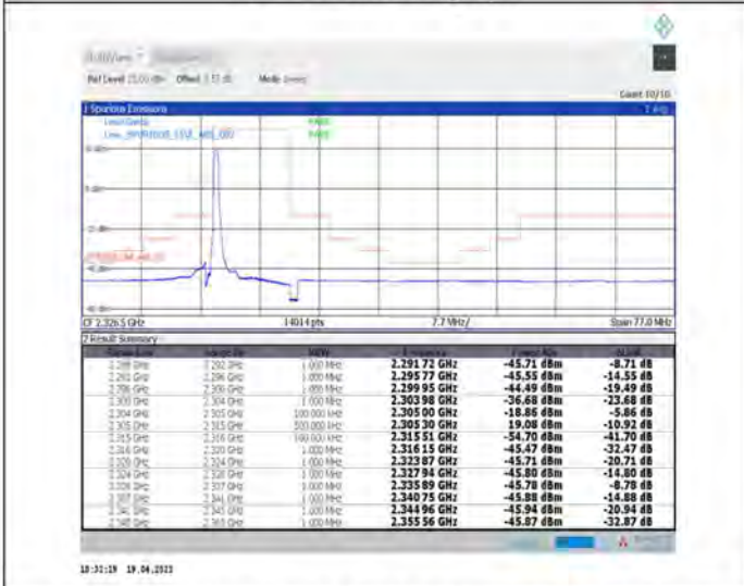
1-N30--30-10-L-4-CP-QPSK-Edge_1RB_Left-1@0-Ant1-PASS-see graph
