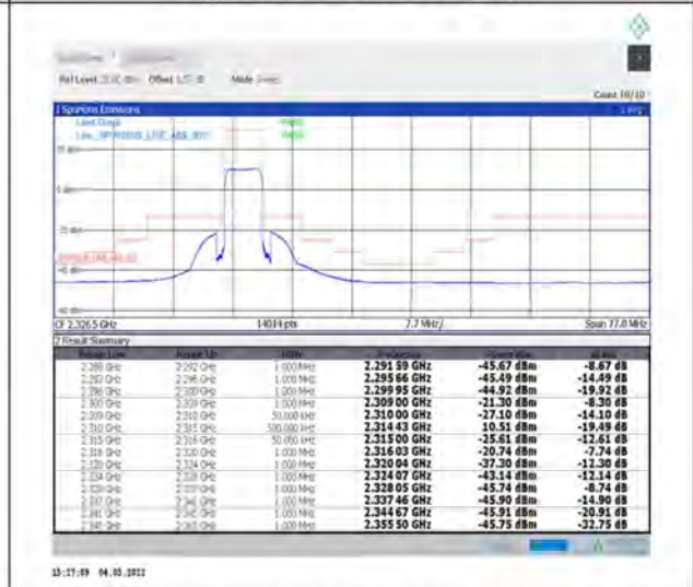
1-N30--15-5-H-6-CP-QPSK-Outer_Full-25@0-Ant1-PASS-see graph
