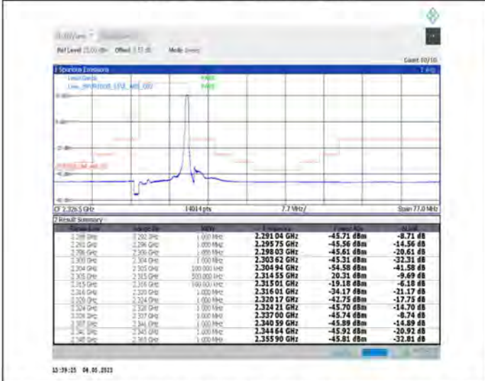
1-N30-15-10-H-5-CP-QPSK-Edge_1RB_Right-1@51-Ant1-PASS-see graph
