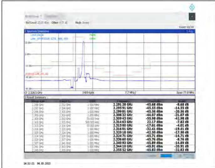
1-N30--15-5-H-2-DFT-PI2BPSK-Edge_1RB_Right-1@24-Ant1-PASS-see graph
