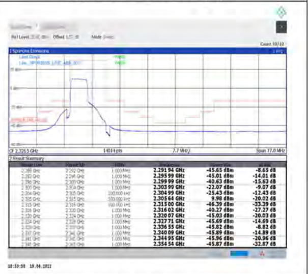
1-N30--30-10-L-6-CP-QPSK-Outer_Full-24@0-Ant1-PASS-see graph
