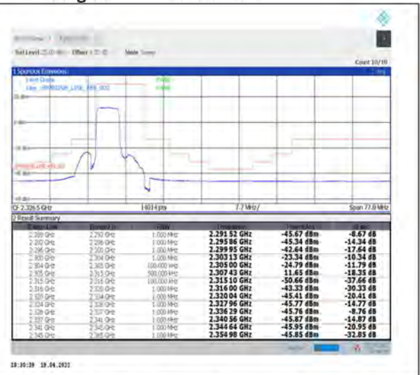
1-N30--30-10-L-3-DFT-PI2BPSK-Outer_Full-24@0-Ant1-PASS-see graph
