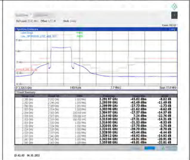
1-N30-15-10-H-6-CP-QPSK-Outer_Full-52@0-Ant1-PASS-see graph
