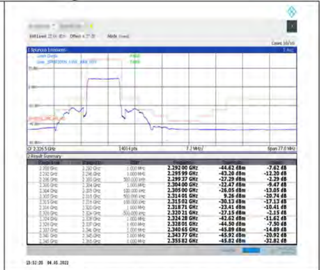
1-N30-15-10-H-3-DFT-PI2BPSK-Outer_Full-50@0-Ant1-PASS-see graph
