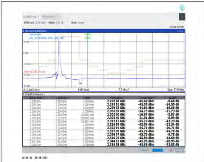
1-N30--30-10-L-1-DFT-PI2BPSK-Edge_1RB_Left-1@0-Ant1-PASS-see graph
