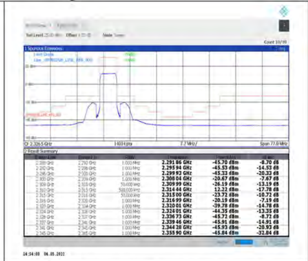
1-N30--15-5-H-3-DFT-PI2BPSK-Outer_Full-25@0-Ant1-PASS-see graph
