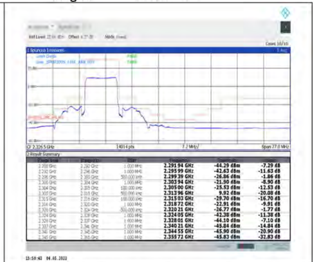
1-N30--15-10-L-3-DFT-PI2BPSK-Outer_Full-50@0-Ant1-PASS-see graph
