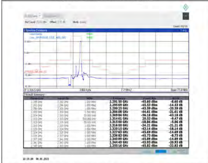
1-N30--15-5-H-5-CP-QPSK-Edge_1RB_Right-1@24-Ant1-PASS-see graph
