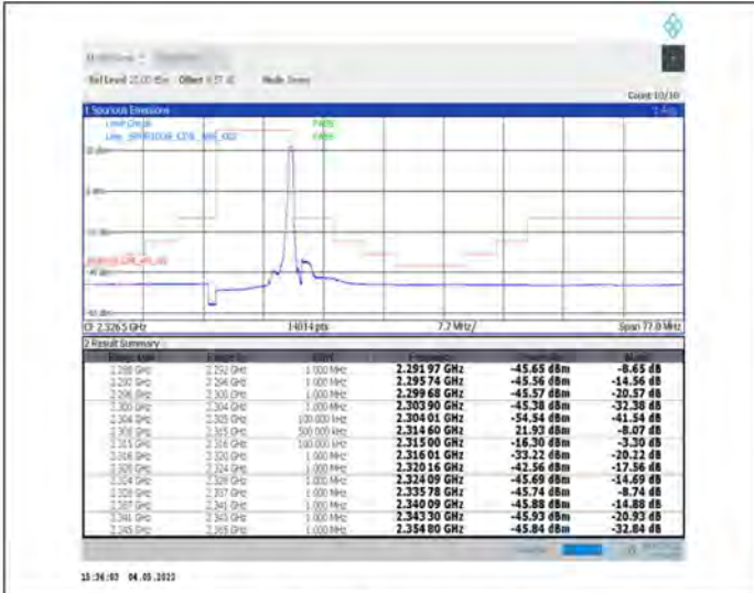
1-N30-15-10-H-2-DFT-PI2BPSK-Edge_1RB_Right-1@51-Ant1-PASS-see graph
