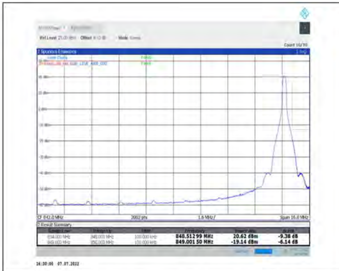
1-N26-824-849--15-15-H-2-DFT-PI2BPSK-Edge_1RB_Right-1@78-Ant1-seegraph-PASS-see graph
