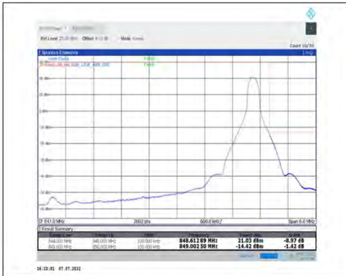
1-N26-824-849--15-5-H-2-DFT-PI2BPSK-Edge_1RB_Right-1@24-Ant1-seegraph-PASS-see graph
