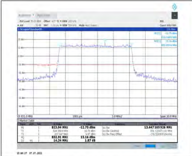
1-N26-824-849--15-15-L-3-DFT-16QAM-Outer_Full-75@0-Ant1-13.447-14.340-≤15-PASS
