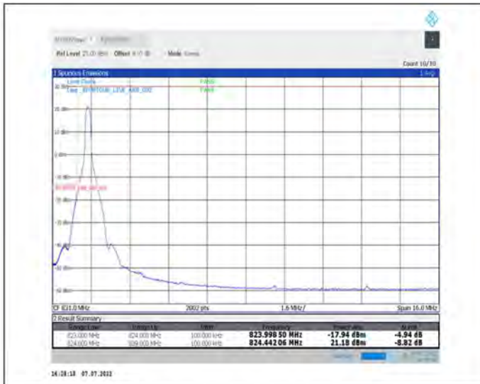
1-N26-824-849--15-15-L-1-DFT-PI2BPSK-Edge_1RB_Left-1@0-Ant1-seegraph-PASS-see graph
