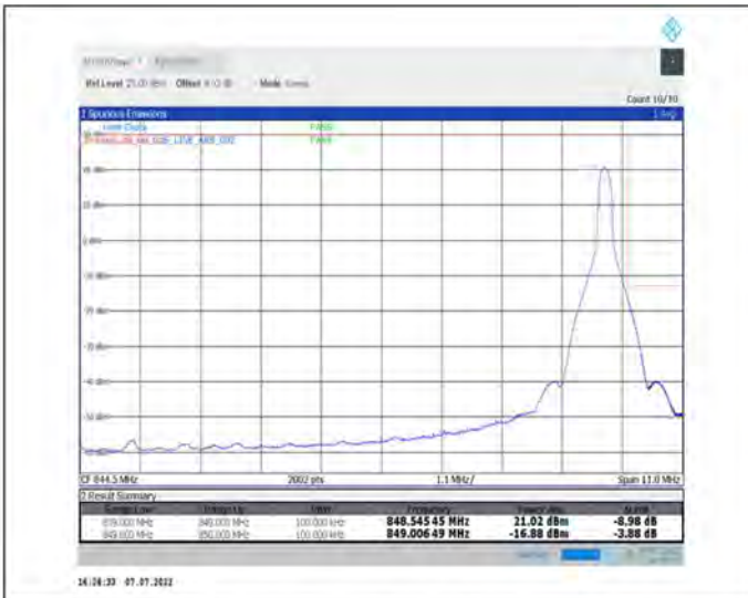
1-N26-824-849--15-10-H-2-DFT-PI2BPSK-Edge_1RB_Right-1@51-Ant1-seegraph-PASS-see graph
