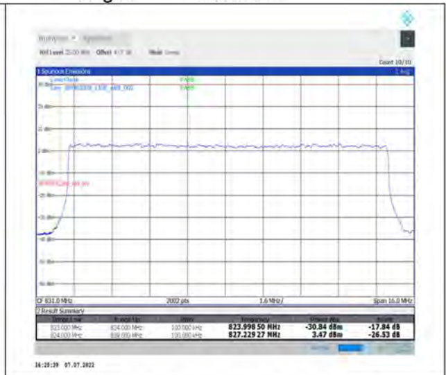
1-N26-824-849--15-15-L-3-DFT-PI2BPSK-Outer_Full-75@0-Ant1-seegraph-PASS-see graph
