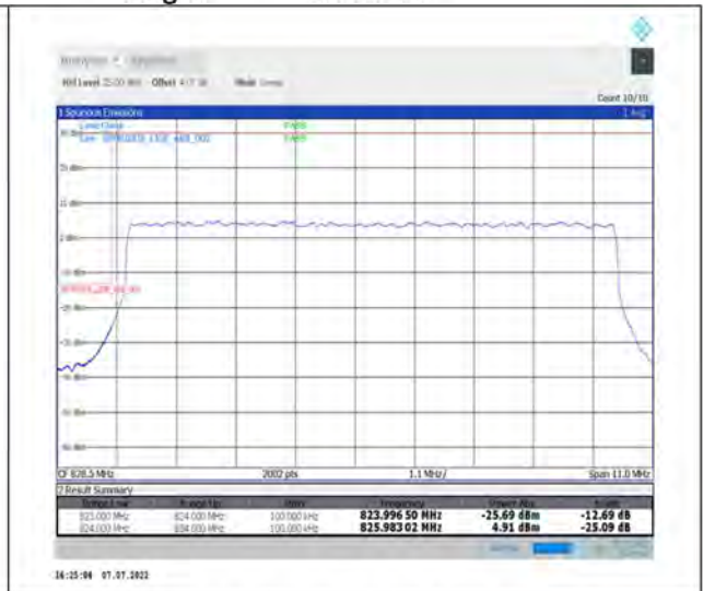
1-N26-824-849--15-10-L-3-DFT-PI2BPSK-Outer_Full-50@0-Ant1-seegraph-PASS-see graph
