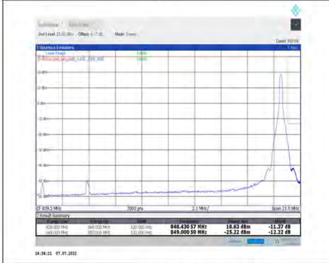
1-N26-824-849--15-20-H-5-CP-QPSK-Edge_1RB_Right-1@105-Ant1-seegraph-PASS-see graph
