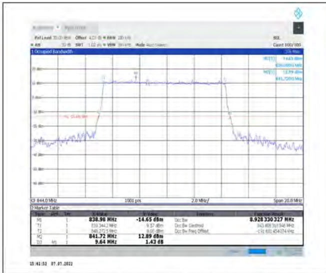
1-N26-824-849--15-10-H-4-DFT-64QAM-Outer_Full-50@0-Ant1-8.928-9.640-≤10-PASS
