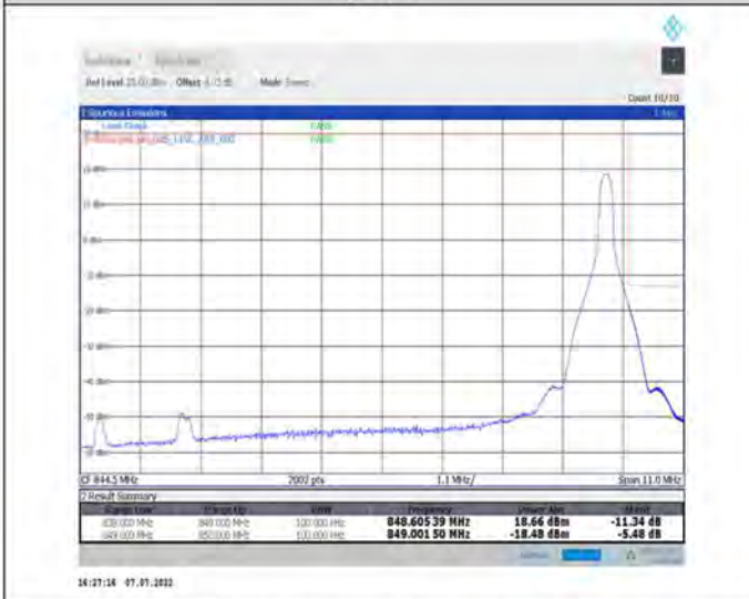
1-N26-824-849--15-10-H-5-CP-QPSK-Edge_1RB_Right-1@51-Ant1-seegraph-PASS-see graph
