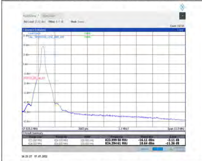
1-N26-824-849--15-10-L-4-CP-QPSK-Edge_1RB_Left-1@0-Ant1-seegraph-PASS-see graph
