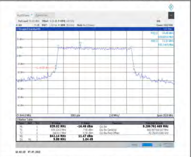
1-N26-824-849--15-10-H-7-CP-16QAM-Outer_Full-52@0-Ant1-9.287-9.880-≤10-PASS
