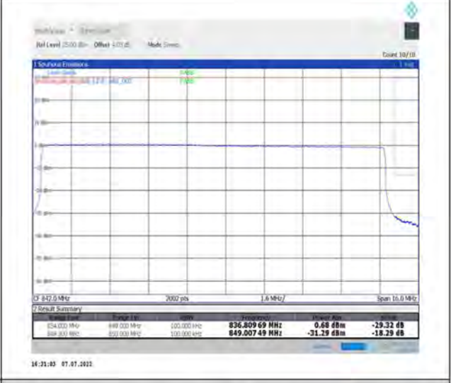
1-N26-824-849--15-15-H-6-CP-QPSK-Outer_Full-79@0-Ant1-seegraph-PASS-see graph
