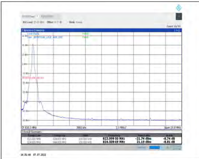
1-N26-824-849--15-20-L-1-DFT-PI2BPSK-Edge_1RB_Left-1@0-Ant1-seegraph-PASS-see graph
