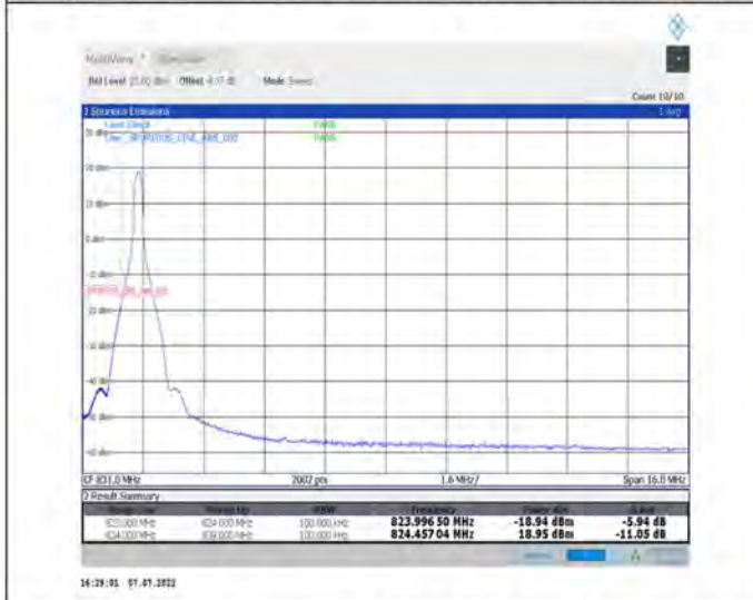
1-N26-824-849--15-15-L-4-CP-QPSK-Edge_1RB_Left-1@0-Ant1-seegraph-PASS-see graph
