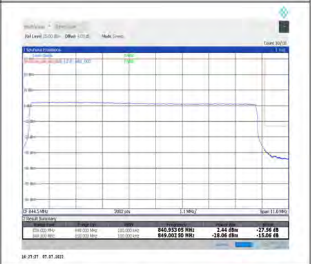
1-N26-824-849--15-10-H-6-CP-QPSK-Outer_Full-52@0-Ant1-seegraph-PASS-see graph
