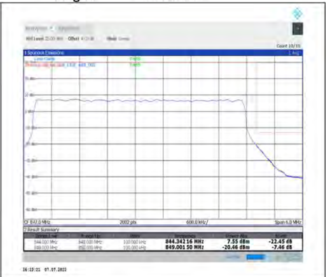
1-N26-824-849--15-5-H-3-DFT-PI2BPSK-Outer_Full-25@0-Ant1-seegraph-PASS-see graph
