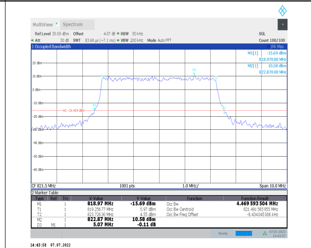
1-N26-814-824--15-5-H-6-CP-QPSK-Outer_Full-25 @0-Ant1-4.47-5.070-≤5-PASS
