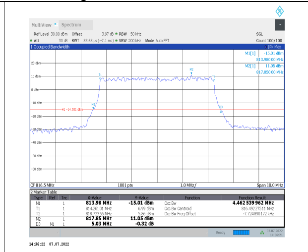
1-N26-814-824--15-5-L-6-CP-QPSK-Outer_Full-25@ 0-Ant1-4.463-5.030-≤5-PASS
