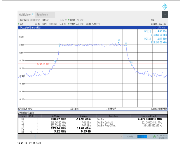
1-N26-814-824--15-5-H-3-DFT-16QAM-Outer_Full-2 5@0-Ant1-4.473-5.120-≤5-PASS
