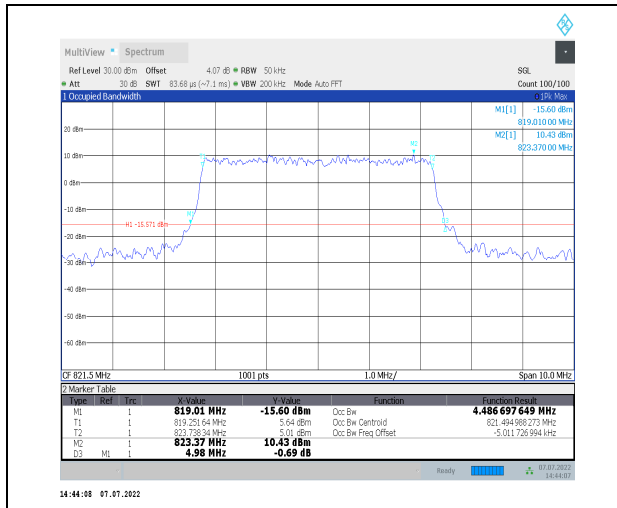
1-N26-814-824--15-5-H-7-CP-16QAM-Outer_Full-25 @0-Ant1-4.487-4.980-<math>\leq 5</math>-PASS
