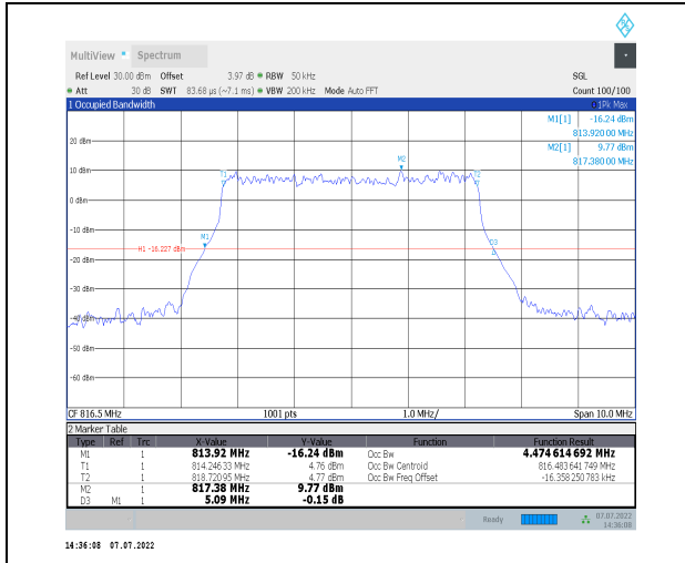
1-N26-814-824--15-5-L-5-DFT-256QAM-Outer_Full-2 @0-Ant1-4.475-5.090-≤5-PASS
