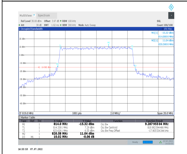
1-N26-814-824--15-10-M-8-CP-64QAM-Outer_Full-5 2@0-Ant1-9.288-10.020-≤10-PASS
