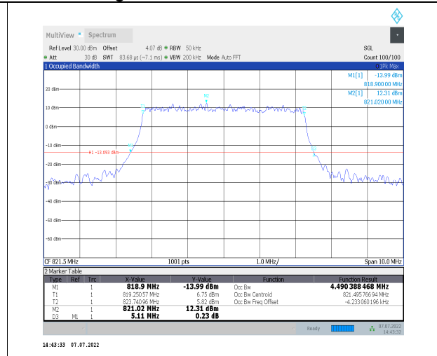
1-N26-814-824--15-5-H-4-DFT-64QAM-Outer_Full-2 5@0-Ant1-4.49-5.110-≤5-PASS
