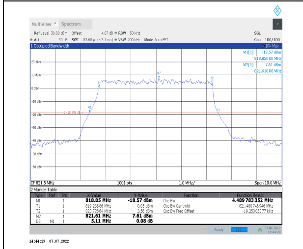
1-N26-814-824--15-5-H-9-CP-256QAM-Outer_Full-2 5@0-Ant1-4.49-5.110-<math>\leq 5</math>-PASS
