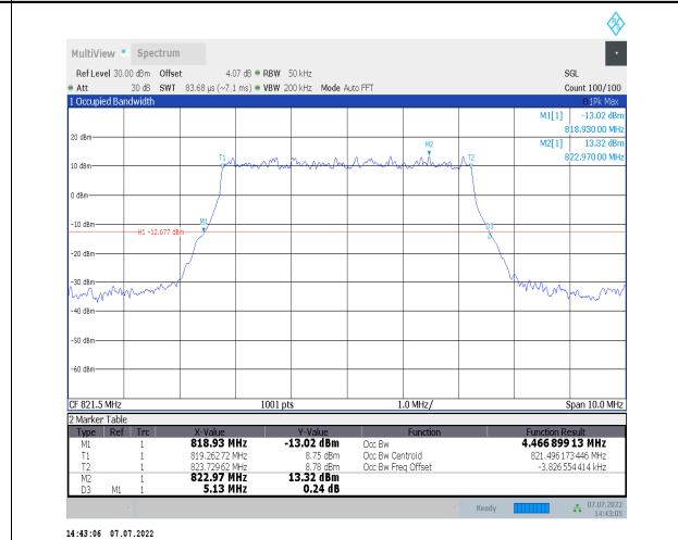
1-N26-814-824--15-5-H-2-DFT-PI2BPSK-Outer_Full-25 @0-Ant1-4.467-5.130-<math>\leq</math>5-PASS
