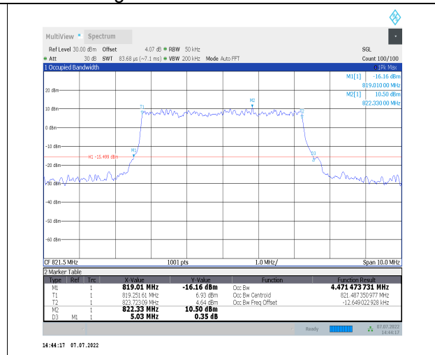
1-N26-814-824--15-5-H-8-CP-64QAM-Outer_Full-25 @0-Ant1-4.471-5.030-<math>\leq 5</math>-PASS
