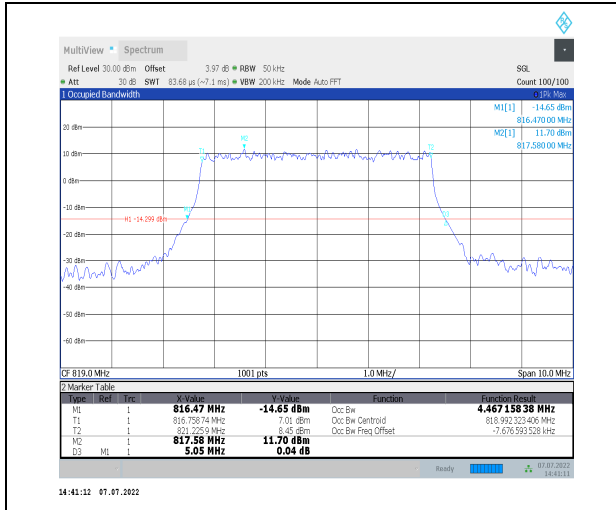
1-N26-814-824--15-5-M-4-DFT-64QAM-Outer_Full-2 5@0-Ant1-4.467-5.050-≤5-PASS
