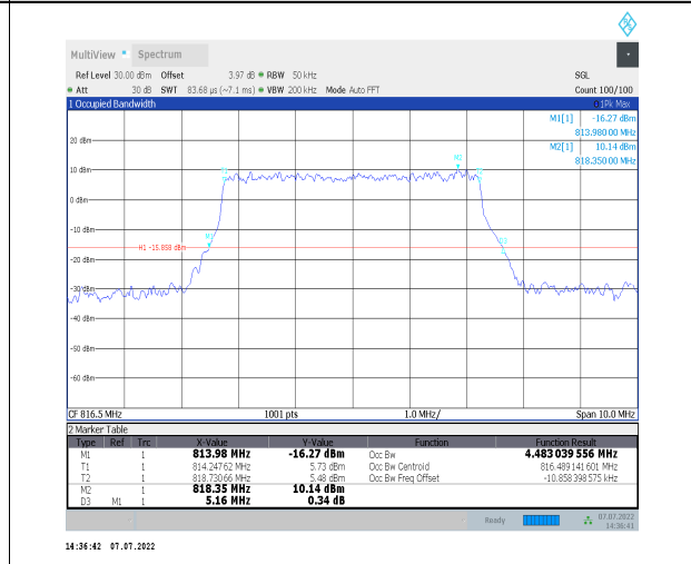
1-N26-814-824--15-5-L-8-CP-64QAM-Outer_Full-25 @0-Ant1-4.483-5.160-≤5-PASS
