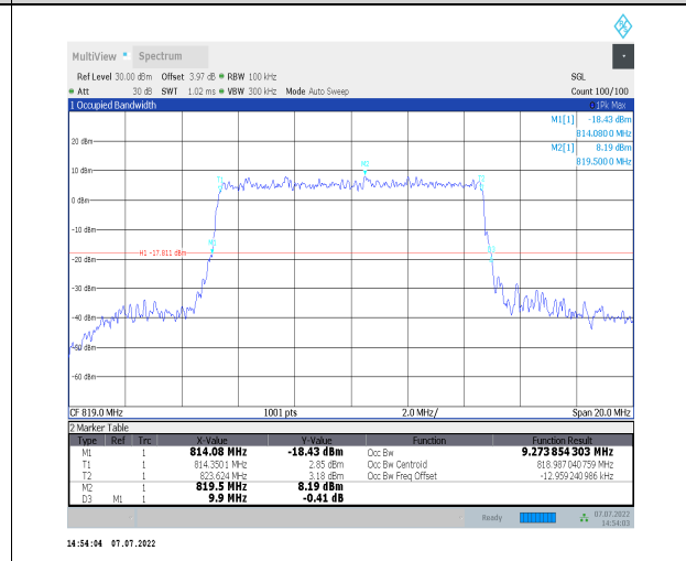
1-N26-814-824--15-10-M-9-CP-256QAM-Outer_Full- 52@0-Ant1-9.274-9.900-≤10-PASS
