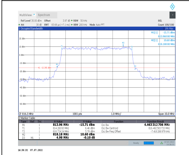
1-N26-814-824--15-5-L-7-CP-16QAM-Outer_Full-25 @0-Ant1-4.463-4.980-≤5-PASS
