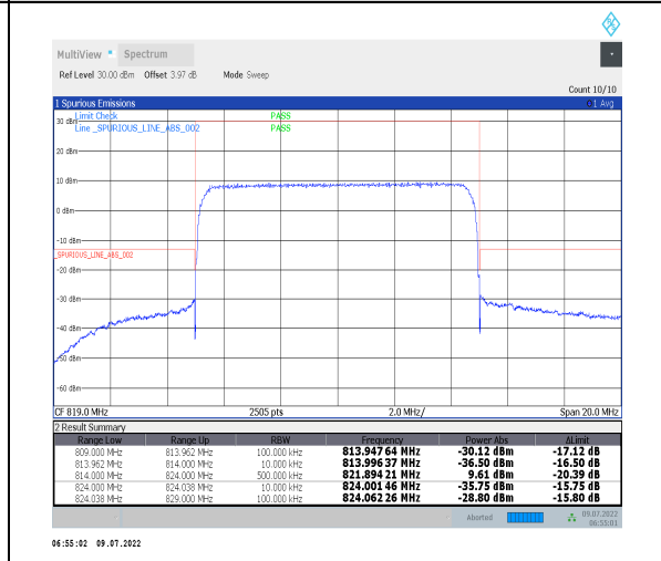
1-N26-814-824--15-10-M-6-CP-QPSK-Outer_Full-52@0-Ant1-PASS-see graph
