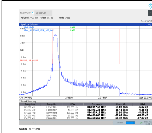
1-N26-814-824--15-10-M-4-CP-QPSK-Edge_1RB_Left-1@0-Ant1-PASS-see graph
