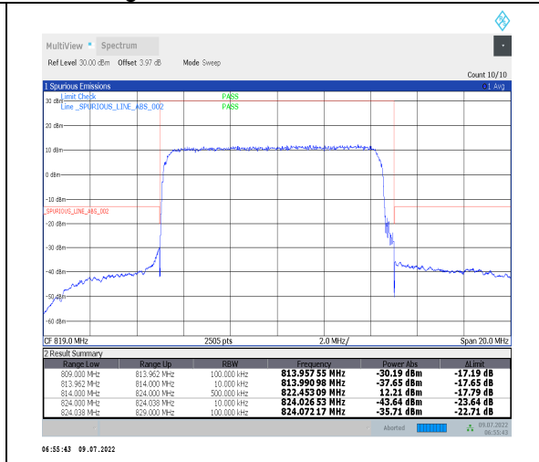
1-N26-814-824--15-10-M-3-DFT-PI2BPSK-Outer_Full-50@0-Ant1-PASS-see graph
