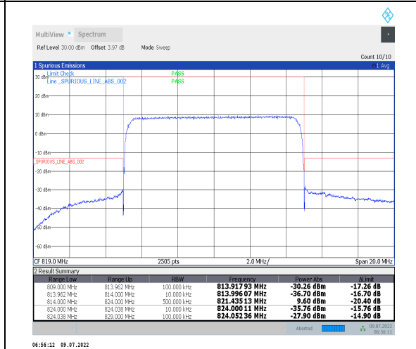
1-N26-814-824--15-10-M-6-CP-QPSK-Outer_Full-52@0-Ant1-PASS-see graph
