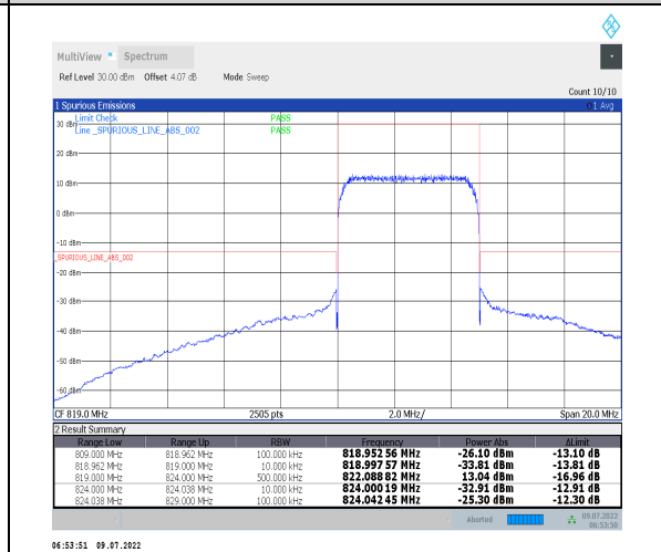
1-N26-814-824--15-5-H-6-CP-QPSK-Outer_Full-25@0-Ant1-PASS-see graph
