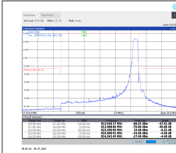
1-N26-814-824--15-10-M-2-DFT-PI2BPSK-Edge_1RB_Right-1@51-Ant1-PASS-see graph
