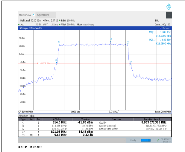
1-N26-814-824--15-10-M-2-DFT-PI2BPSK-Outer_Full-I-50@0-Ant1-8.953-9.680-<=10-PASS
