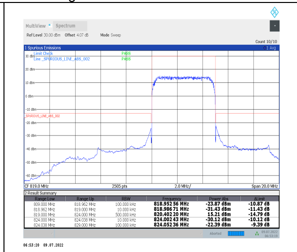
1-N26-814-824--15-5-H-3-DFT-PI2BPSK-Outer_Full-25@0-Ant1-PASS-see graph
