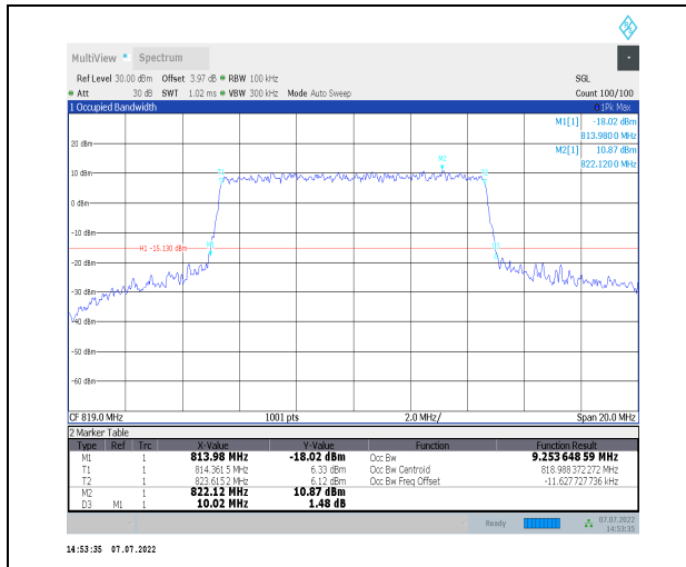
1-N26-814-824--15-10-M-6-CP-QPSK-Outer_Full-52 @0-Ant1-9.254-10.020-≤10-PASS
