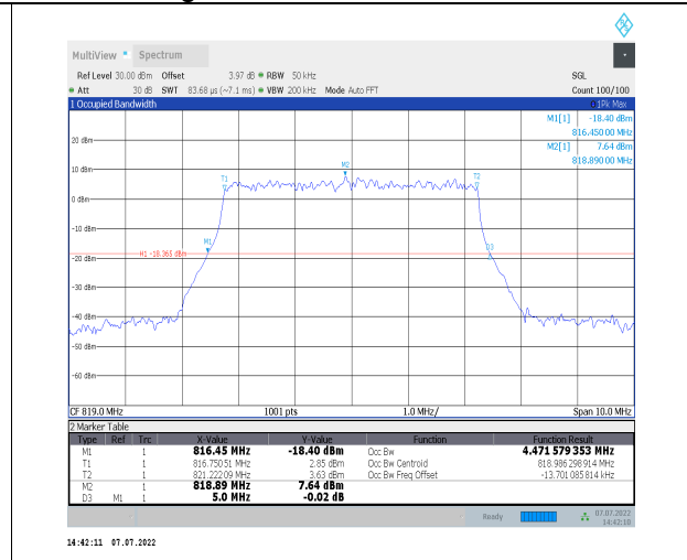
1-N26-814-824--15-5-M-9-CP-256QAM-Outer_Full-2 5@0-Ant1-4.472-5.000-<math>\leq</math>5-PASS
