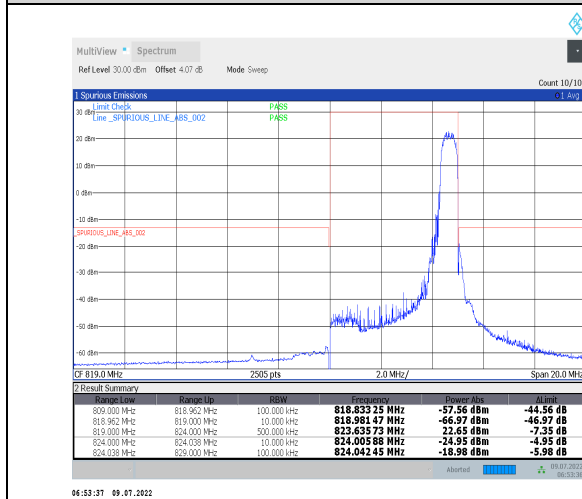
1-N26-814-824--15-5-H-5-CP-QPSK-Edge_1RB_Right-1@24-Ant1-PASS-see graph
