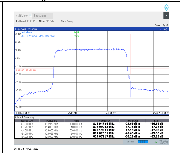
1-N26-814-824--15-10-M-3-DFT-PI2BPSK-Outer_Full-50@0-Ant1-PASS-see graph
