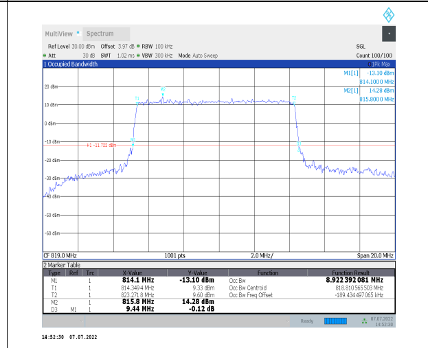
1-N26-814-824--15-10-M-1-DFT-QPSK-Outer_Full-5 0@0-Ant1-8.922-9.440-<math>\leq 10</math>-PASS
