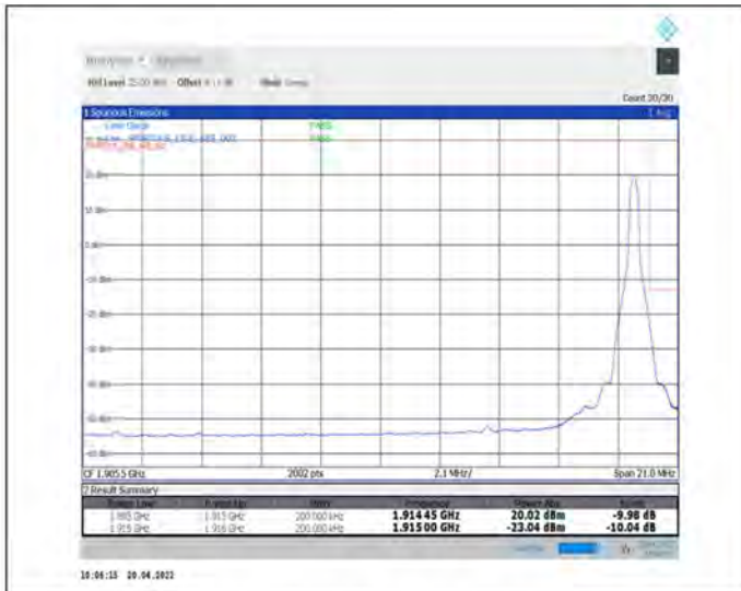
1-N25--15-20-H-2-DFT-PI2BPSK-Edge_1RB_Right-1@105-Ant1-seegraph-PASS-see graph
