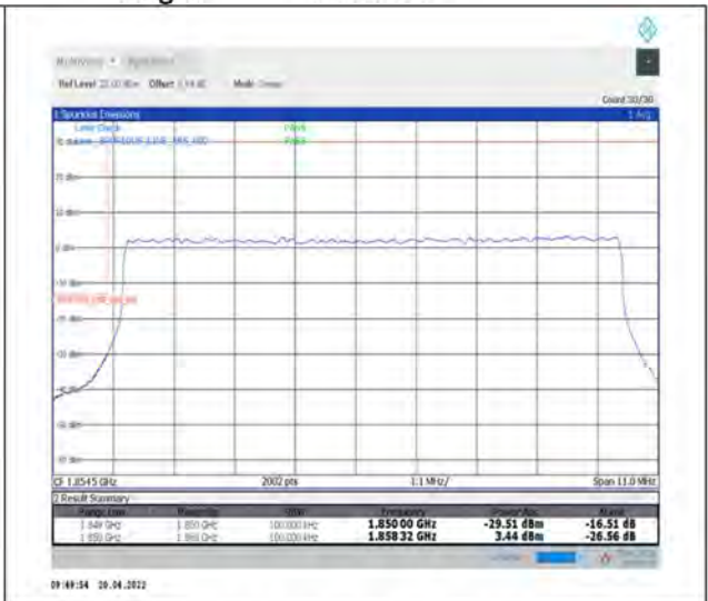
1-N25--15-10-L-3-DFT-PI2BPSK-Outer_Full-50@0-Ant1-seegraph-PASS-see graph
