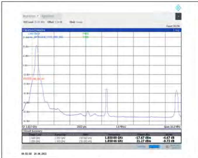
1-N25--15-15-L-1-DFT-PI2BPSK-Edge_1RB_Left-1@0-Ant1-seegraph-PASS-see graph
