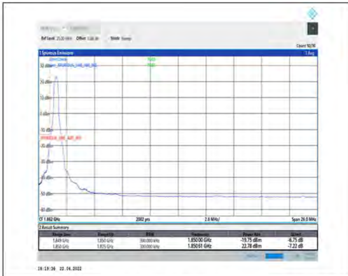
1-N25--15-25-L-1-DFT-PI2BPSK-Edge_1RB_Left-1@0-Ant1-seegraph-PASS-see graph
