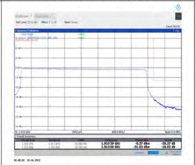
1-N25--15-5-H-6-CP-QPSK-Outer_Full-25@0-Ant1-seegraph-PASS-see graph
