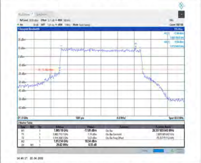
1-N25--15-30-H-7-CP-16QAM-Outer_Full-160@0-Ant1-28.558-29.820-≤30-PASS
