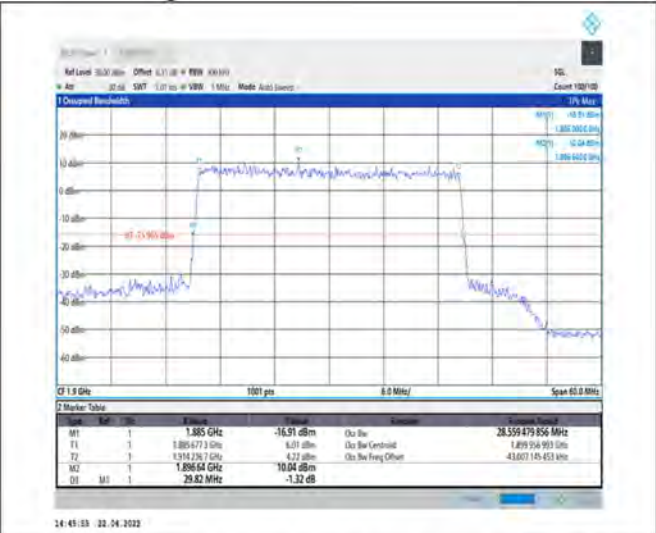
1-N25--15-30-H-5-DFT-256QAM-Outer_Full-160@0-Ant1-28.559-29.820-≤30-PASS
