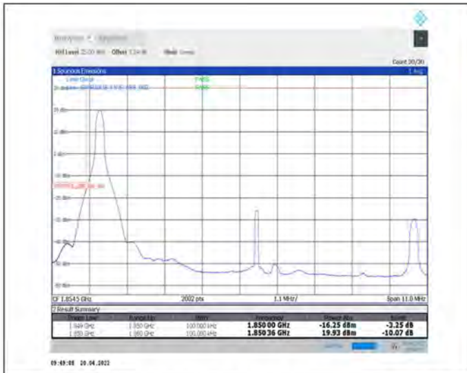
1-N25--15-10-L-1-DFT-PI2BPSK-Edge_1RB_Left-1@0-Ant1-seegraph-PASS-see graph
