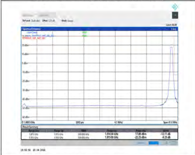
1-N25--15-40-H-5-CP-QPSK-Edge_1RB_Right-1@215-Ant1-seegraph-PASS-see graph
