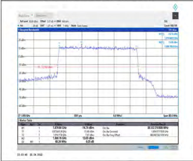
1-N25--15-40-H-3-DFT-16QAM-Outer_Full-216@0-Ant1-38.532-40.240-≤40-PASS
