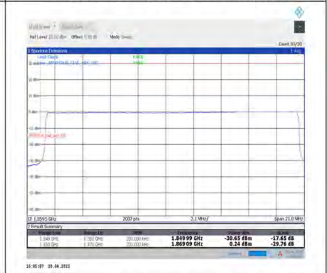
1-N25--15-20-L-6-CP-QPSK-Outer_Full-106@0-Ant1-seegraph-PASS-see graph
