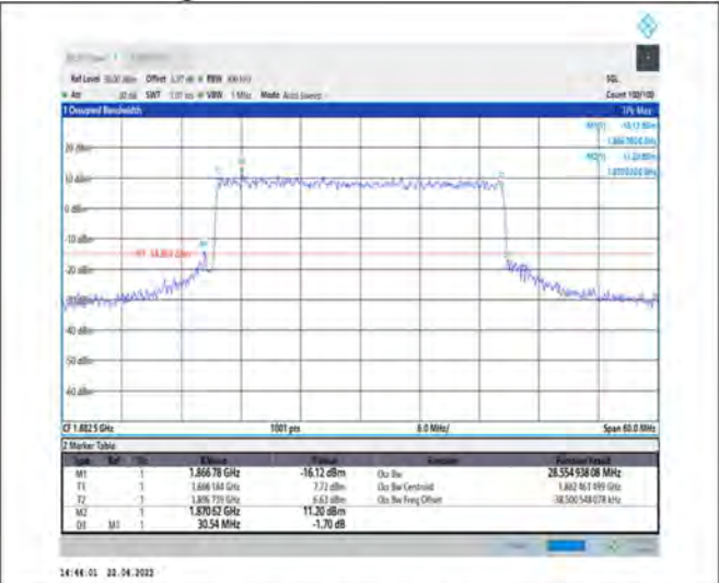
1-N25--15-30-M-6-CP-QPSK-Outer_Full-160@0-Ant1-28.555-30.540-≤30-PASS
