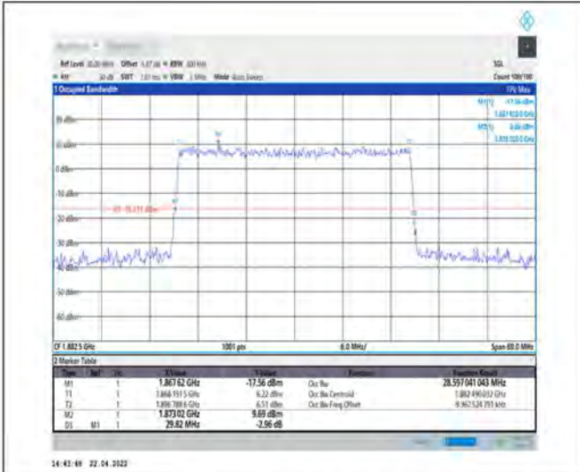
1-N25--15-30-M-5-DFT-256QAM-Outer_Full-160@0-Ant1-28.597-29.820-≤30-PASS
