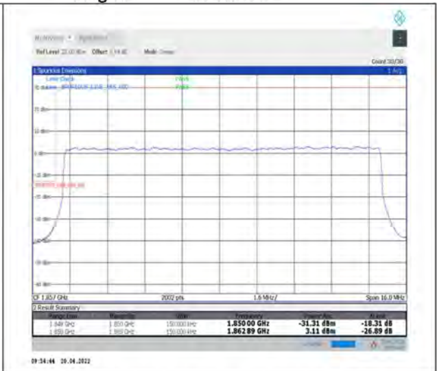
1-N25--15-15-L-3-DFT-PI2BPSK-Outer_Full-75@0-Ant1-seegraph-PASS-see graph
