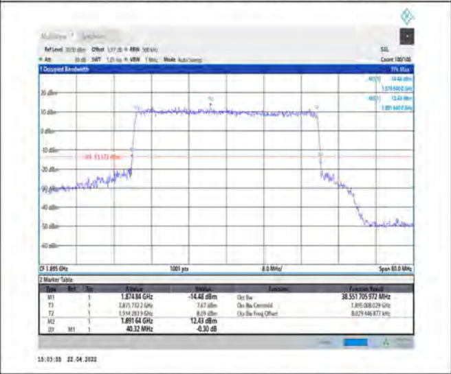
1-N25--15-40-H-4-DFT-64QAM-Outer_Full-216@0-Ant1-38.552-40.320-≤40-PASS
