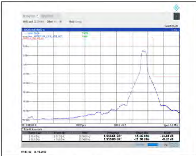
1-N25--15-5-H-2-DFT-PI2BPSK-Edge_1RB_Right-1@24-Ant1-seegraph-PASS-see graph
