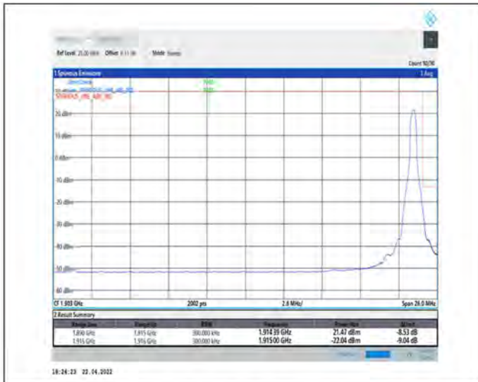
1-N25--15-25-H-2-DFT-PI2BPSK-Edge_1RB_Right-1@132-Ant1-seegraph-PASS-see graph
