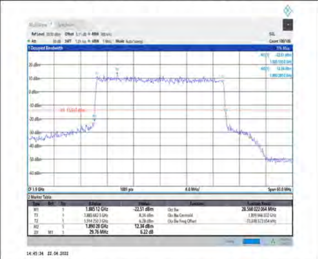
1-N25--15-30-H-3-DFT-16QAM-Outer_Full-160@0-Ant1-28.568-29.760-≤30-PASS
