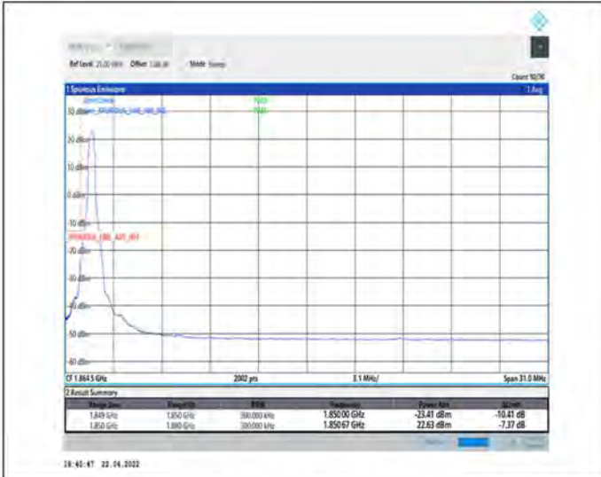
1-N25--15-30-L-1-DFT-PI2BPSK-Edge_1RB_Left-1@0-Ant1-seegraph-PASS-see graph
