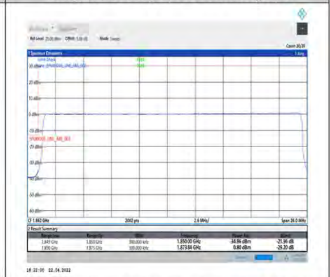
1-N25--15-25-L-6-CP-QPSK-Outer_Full-133@0-Ant1-seegraph-PASS-see graph
