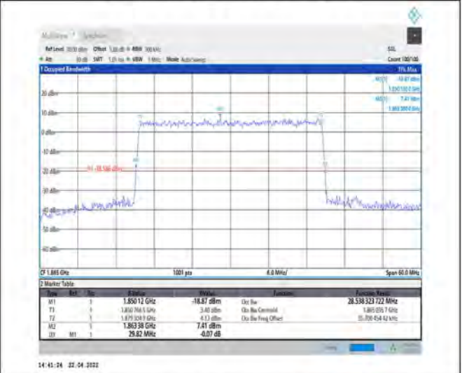
1-N25--15-30-L-9-CP-256QAM-Outer_Full-160@0-Ant1-28.538-29.820-≤30-PASS
