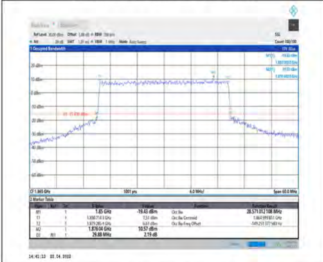
1-N25--15-30-L-8-CP-64QAM-Outer_Full-160@0-Ant1-28.571-29.880-≤30-PASS
