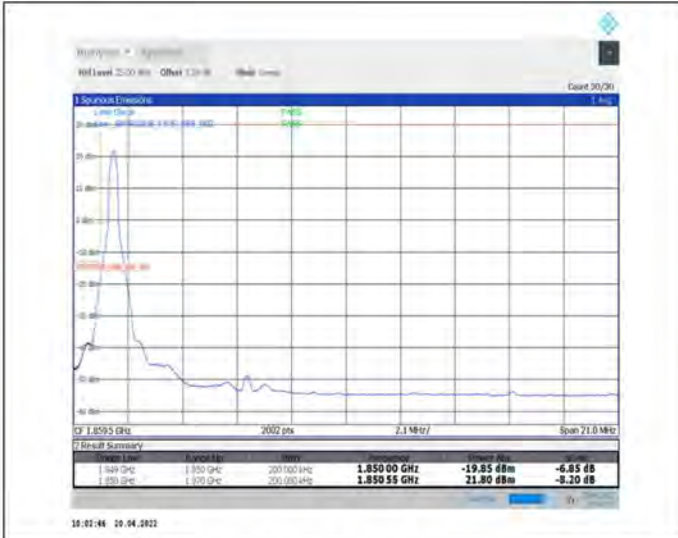
1-N25--15-20-L-1-DFT-PI2BPSK-Edge_1RB_Left-1@0-Ant1-seegraph-PASS-see graph
