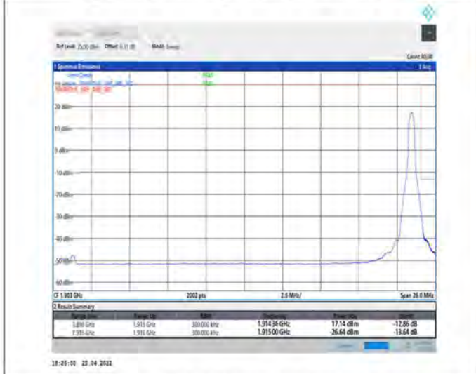
1-N25--15-25-H-5-CP-QPSK-Edge_1RB_Right-1@132-Ant1-seegraph-PASS-see graph
