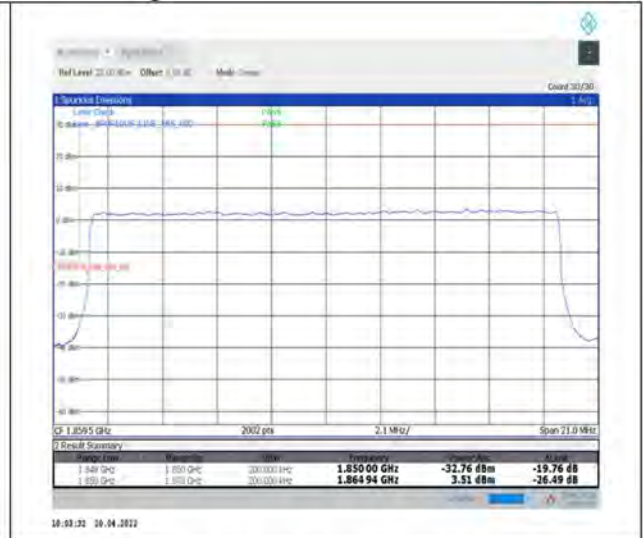
1-N25--15-20-L-3-DFT-PI2BPSK-Outer_Full-100@0-Ant1-seegraph-PASS-see graph
