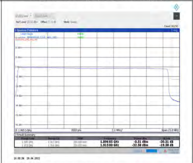
1-N25--15-20-H-6-CP-QPSK-Outer_Full-106@0-Ant1-seegraph-PASS-see graph
